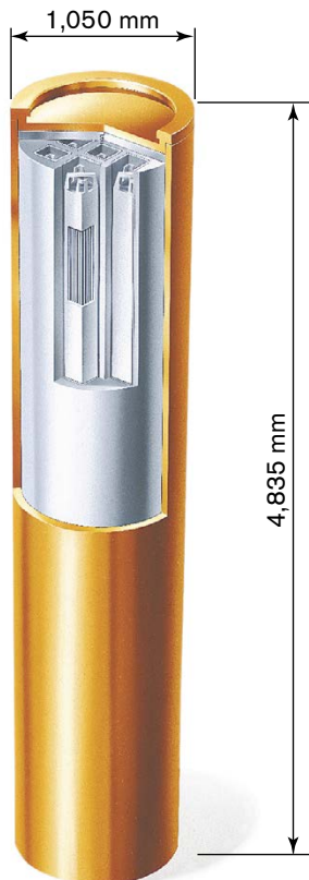
Figure 1-5. The reference design with a corrosion resistant outer copper shell and a load-bearing insert of nodular cast iron.
