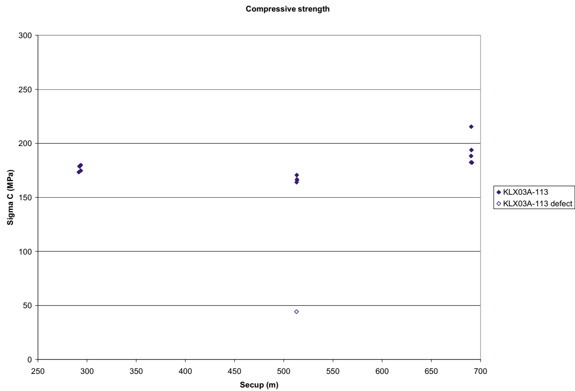
Figure 5-2. Uniaxial compressive strength versus sampling depth in the borehole.
