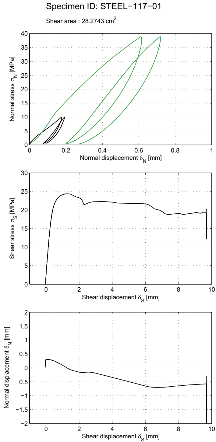
Figure A-1. Results from reference test 1 with a steel specimen cast in concrete.
