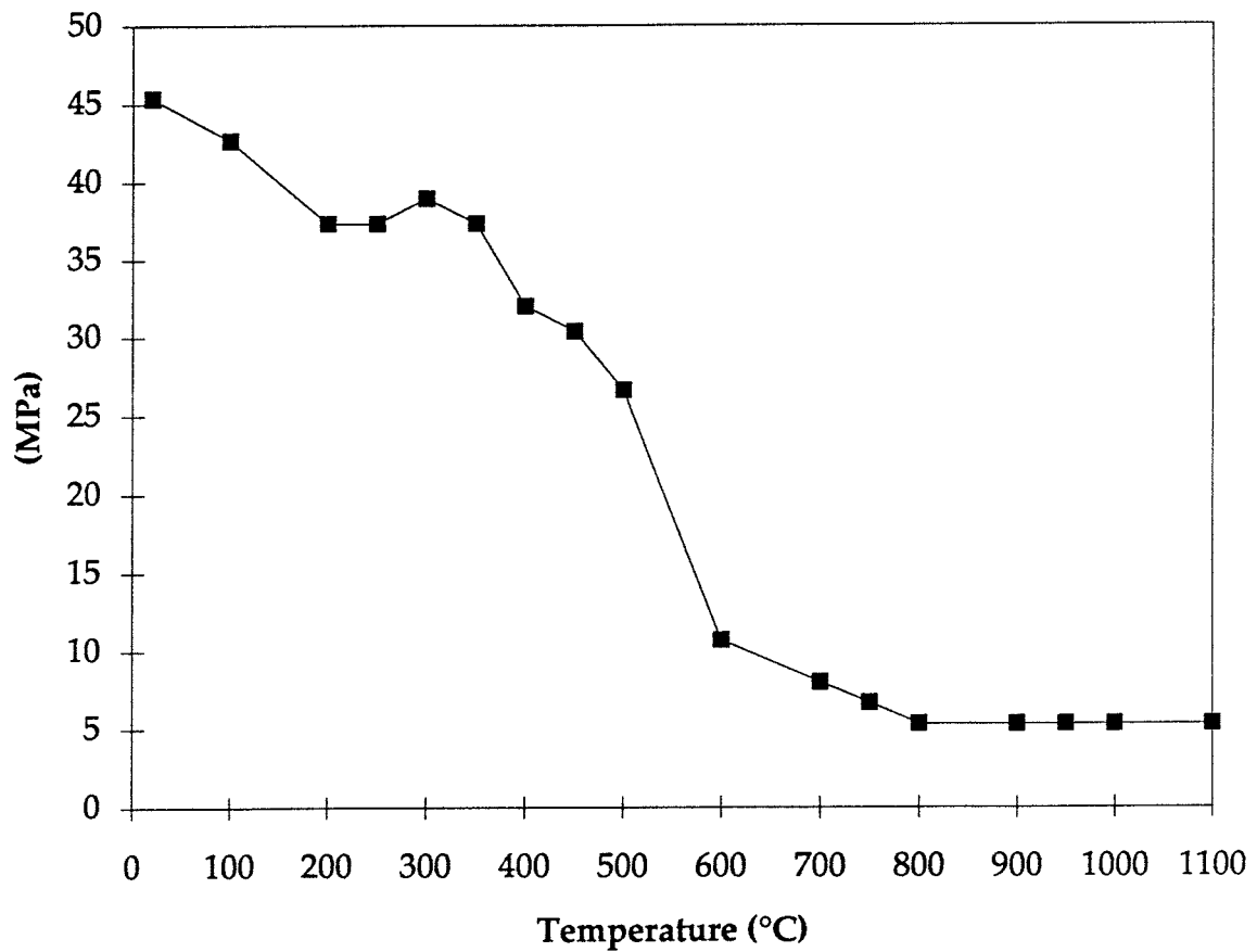
Fig 5 Yield stress as function of temperature for the copper material.
