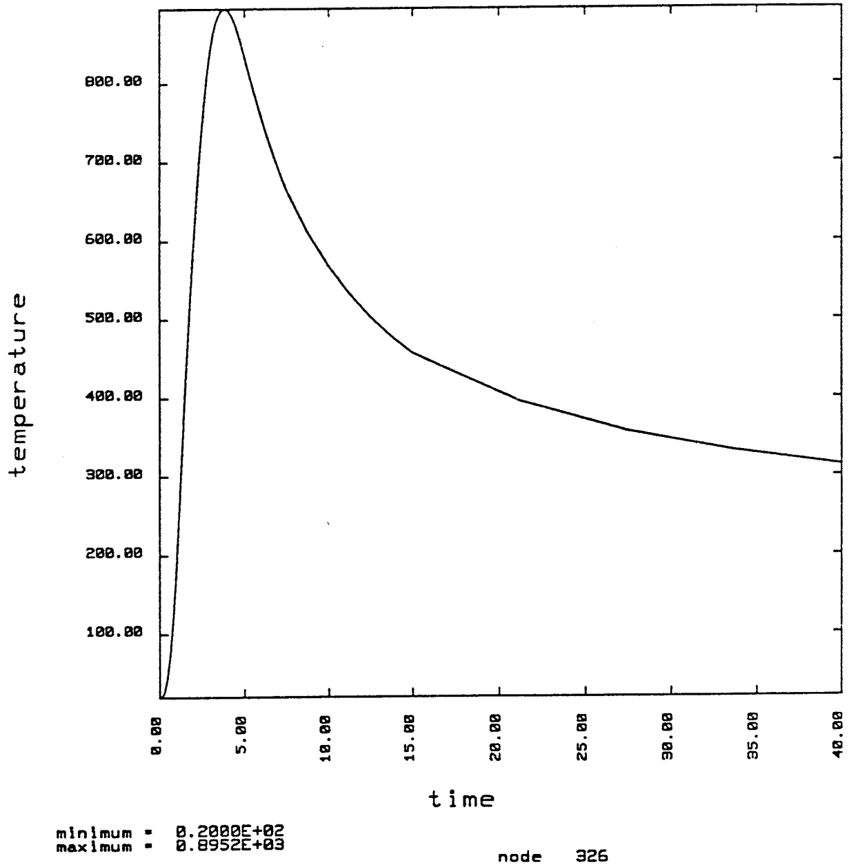
Fig 19 Calculated time history of temperature at a point in the backing ring close to inner surface (same point as in Fig 18).
