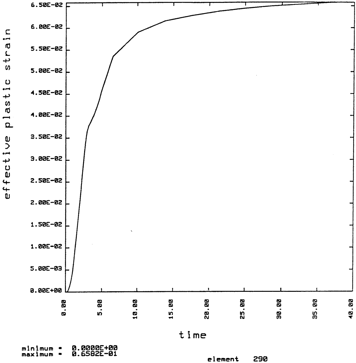
Fig 18 Calculated time history of effective plastic strain for large gap 2.0 mm at a point in the backing ring close to inner surface ( r = 0.38 m, z = 0.92 m).
