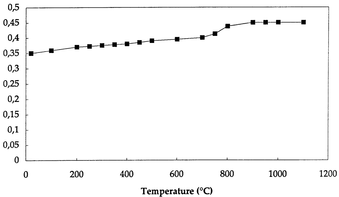
Fig 7 Poisson's ratio as function of temperature for the copper material.
