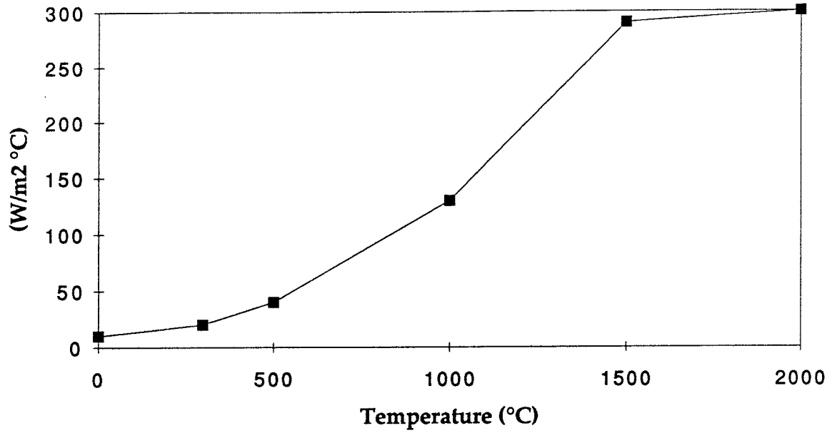
Fig 4 Convective surface heat transfer coefficient as function of temperature.
