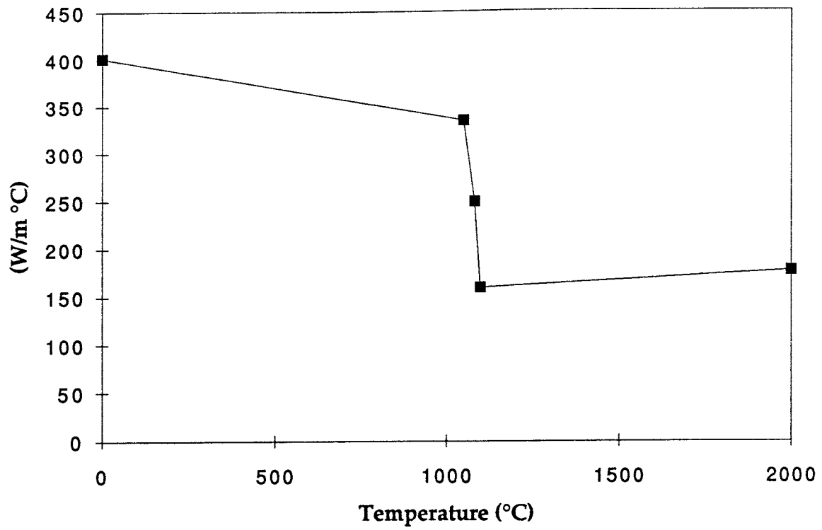
Fig 3a Thermal conductivity as function of temperature for the copper material.
