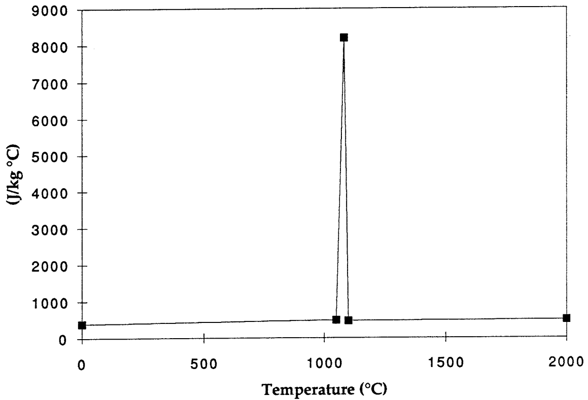
Fig 3b Heat capacity as function of temperature for the copper material.
