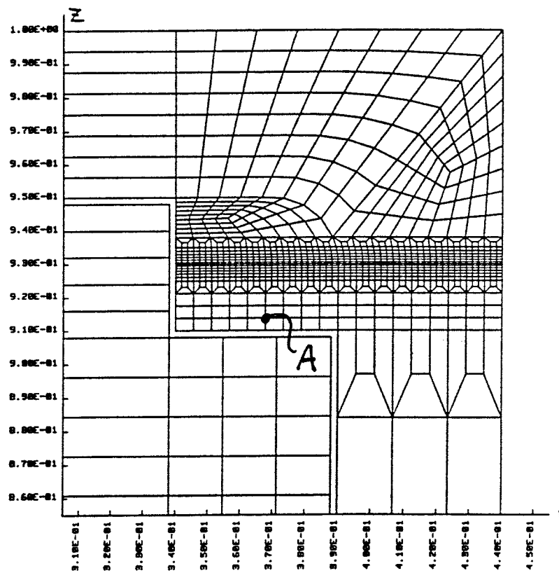
Fig 2 Finite element mesh used in both thermal and mechanical analyses. Point A is used for result presentations.
