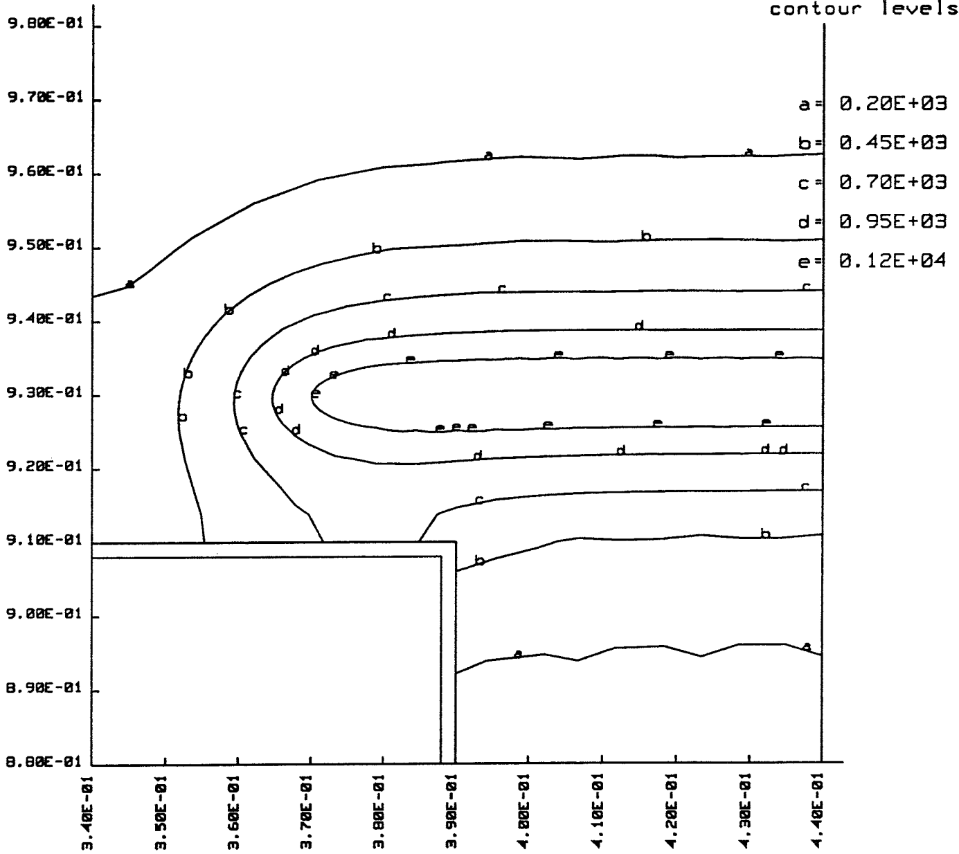
Fig 10 Calculated isotherms during early stage of cooling. Figure is valid for large gap.
