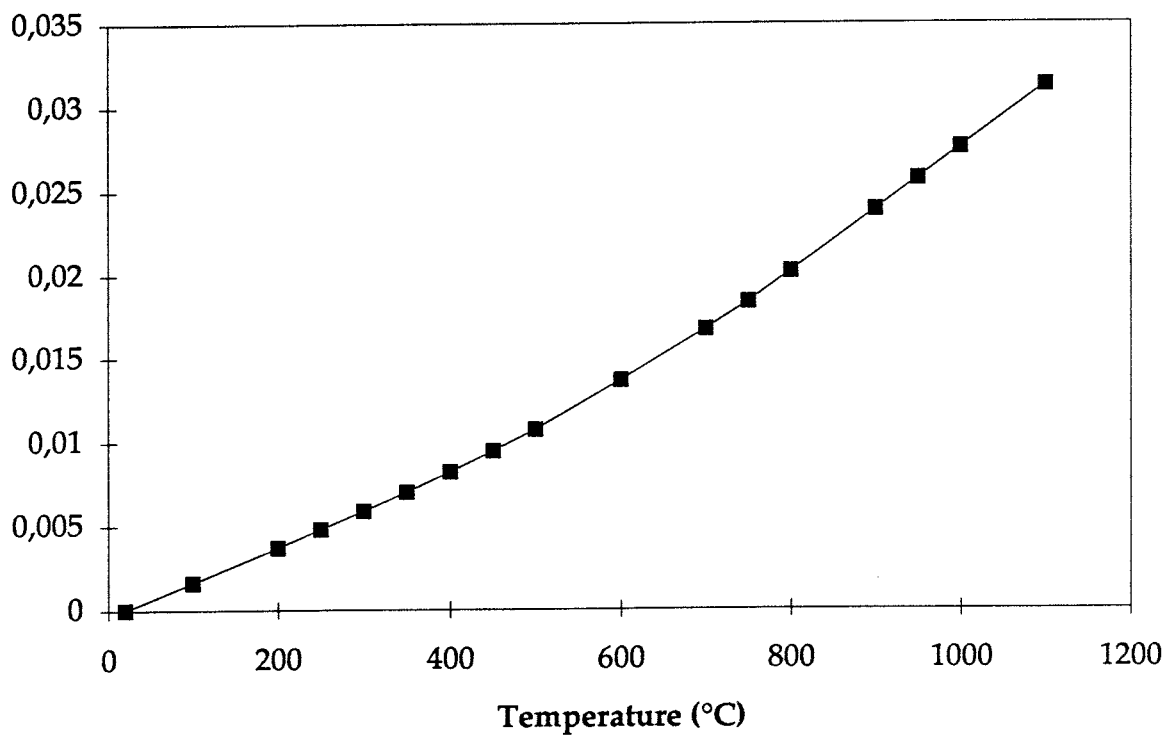
Fig 9 Thermal strain as function of temperature for the copper material.
