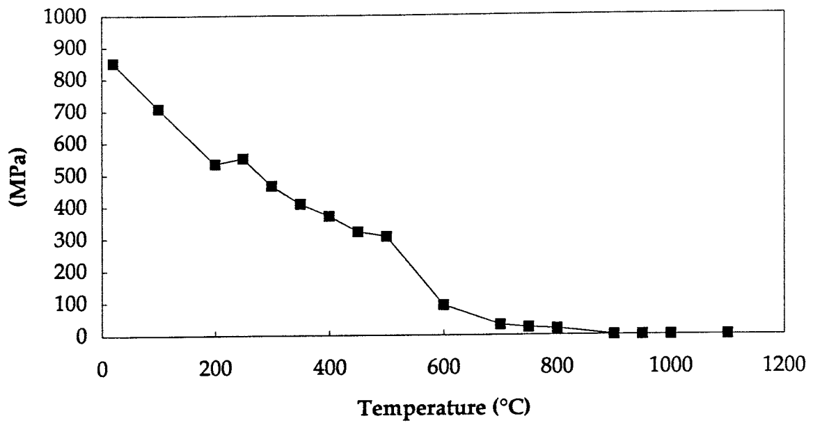
Fig 8 Hardening modulus as function of temperature for the copper material.
