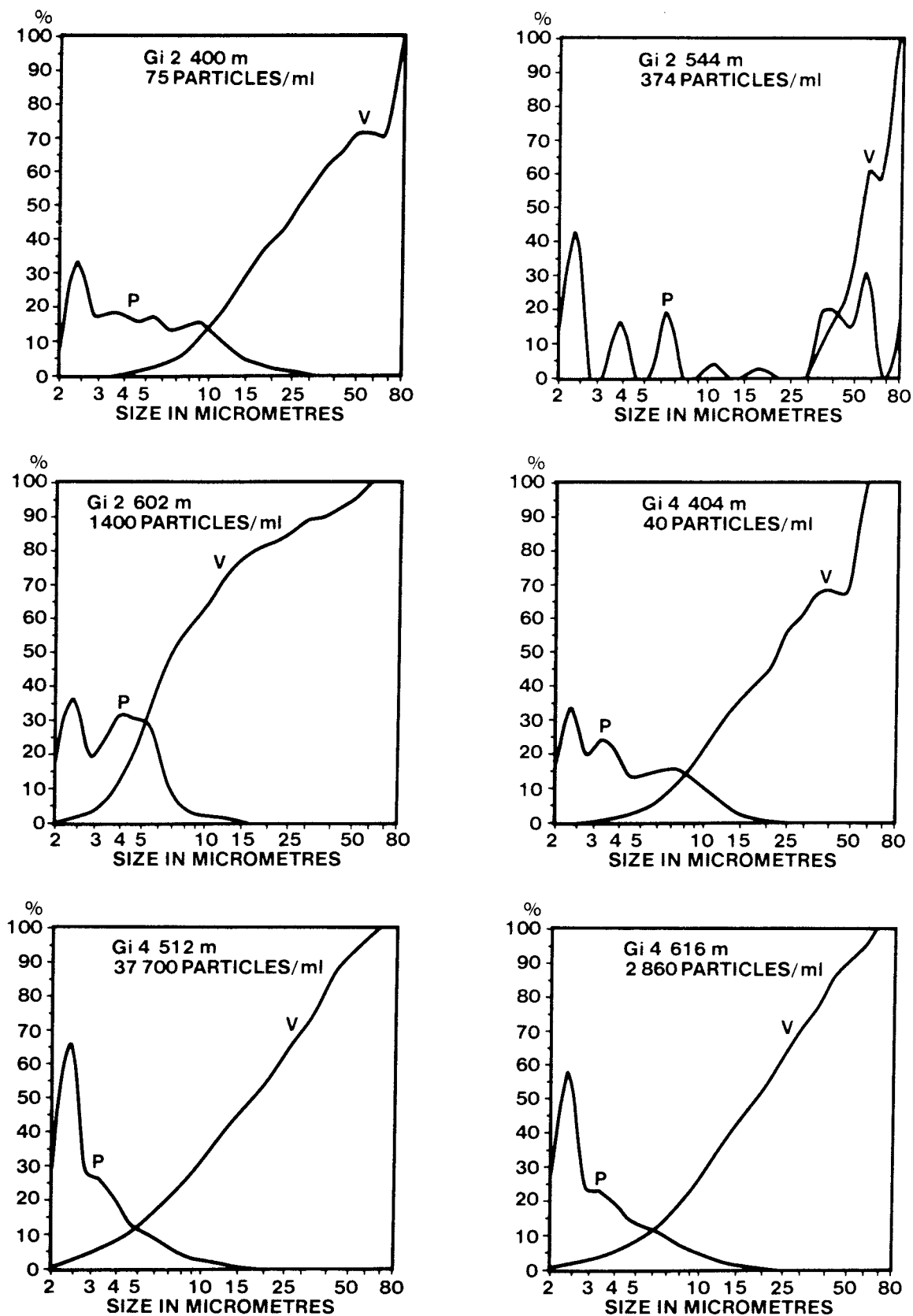
Figure 2. Particle size distribution analysis in the region 2-80 \mu\text{m} . An HIAC PA 500 instrument is used. P represents the percent of the total number of particles with a certain particle size. V represents the percent of the total particle volume less than a certain particle size.
