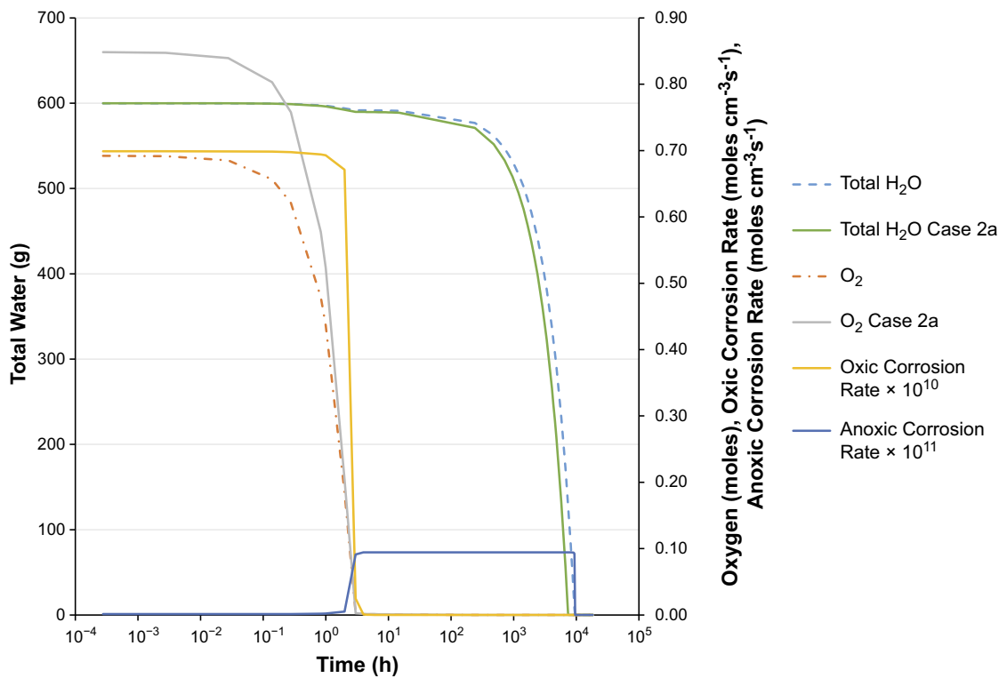
Figure 3-12. Model outputs of canister water, oxygen, and corrosion rates versus time for Case 2b. Also plotted are the O_2 and total H_2O for Case 2a.
