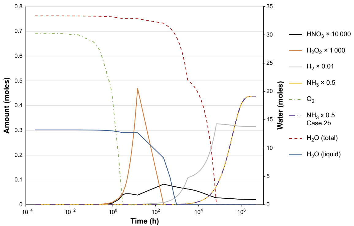
Figure 3-15. Calculated major species amounts for Case 2c. Also plotted NH_3 concentration from Case 2b, results overlap Case 2c.
