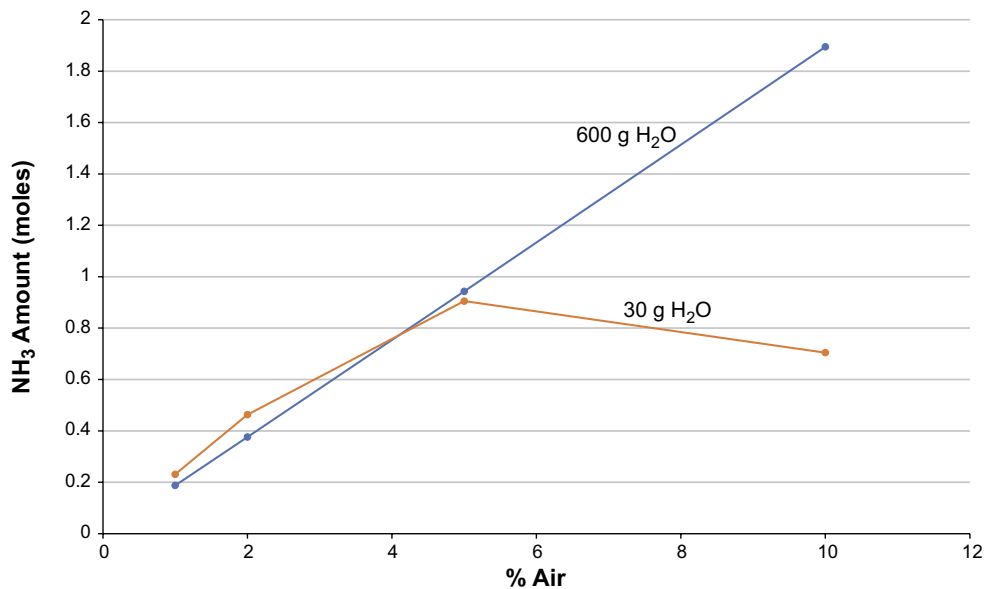
Figure 3-32. Calculated final amounts of NH 3 for Cases 13a, 14, 15, 16, 17, 18, 19, 20 against initial air content of the canister.
