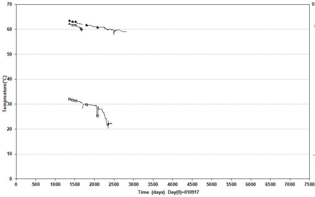
PrototypelHole 1\Cyl.1 (20010917-20220101) Temprature - Geokon
