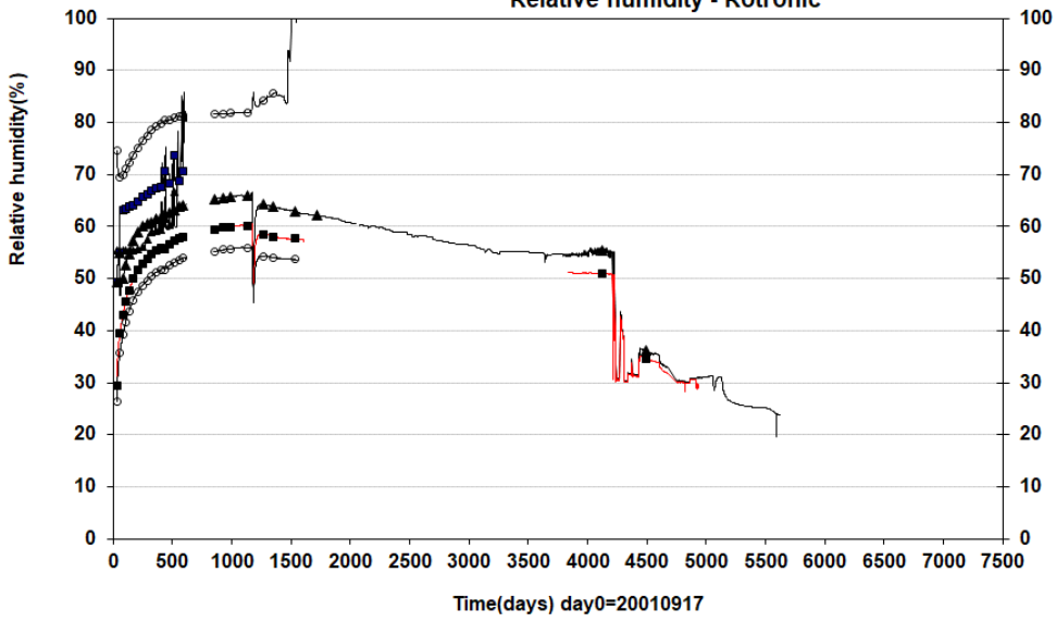
Prototype\Hole 3\Cyl.1 (20010917-20220101) Relative humidity - Rotronic
