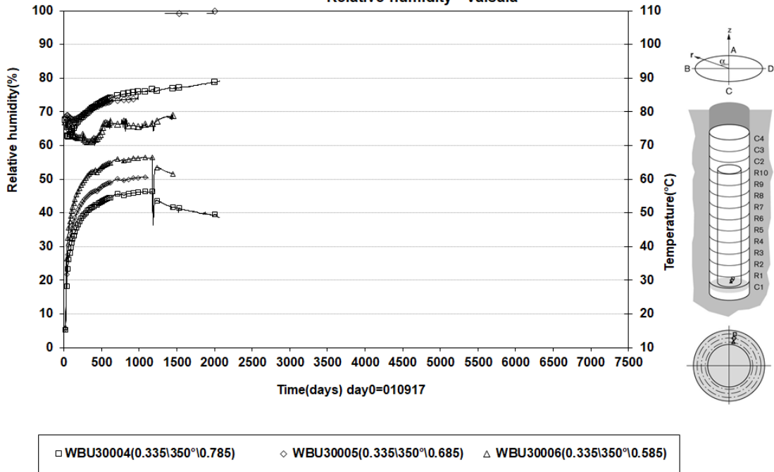
Prototype\Hole 3\Cyl.1 (20010917-20220101) Relative humidity - Vaisala
