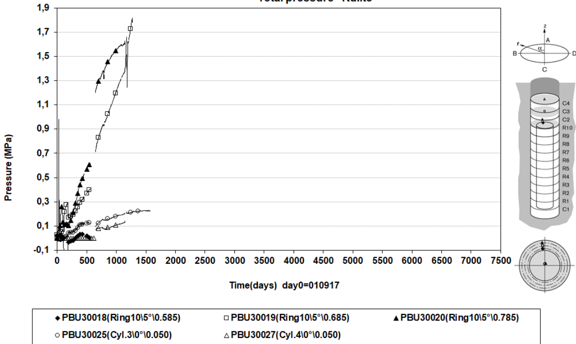
Prototype\Hole 3\Ring10 and Cyl.3-4 (010917-20220101) Total pressure - Kulite
