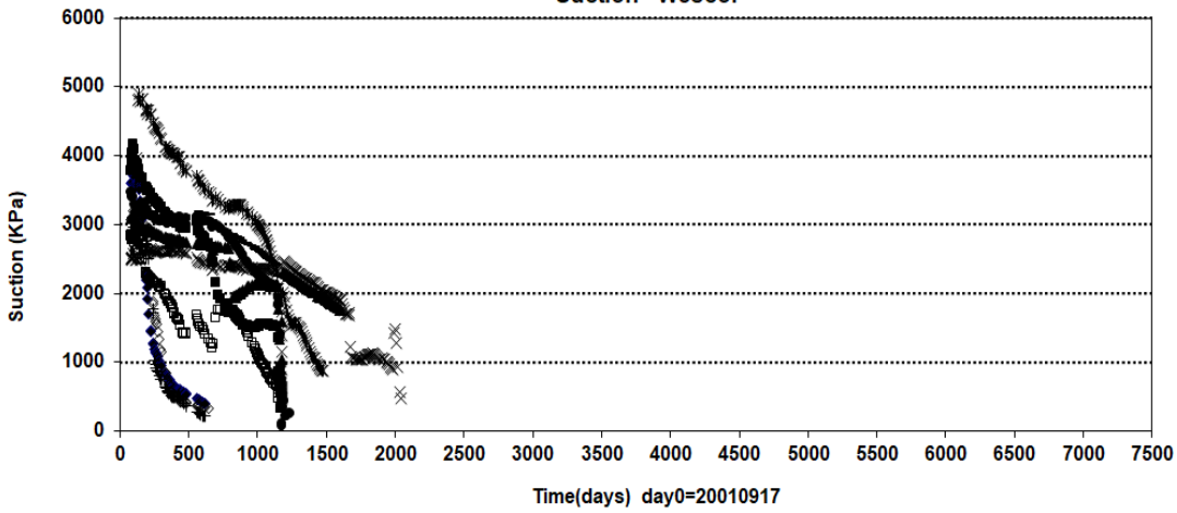
Prototype\Backfill Above dep.hole 3 (20010917-20220101) Suction - Wescor
