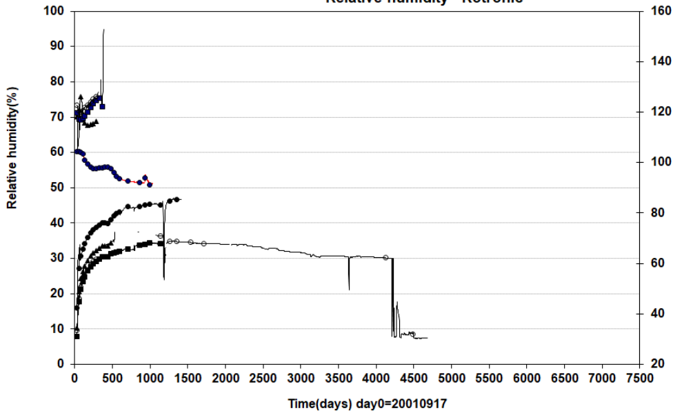
Prototype\Hole 3\Ring 5 (20010917-20220101) Relative humidity - Rotronic
