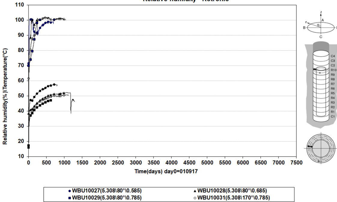
PrototypHole 1\Ring10 (20010917-20220101) Relative humidity - Rotronic
