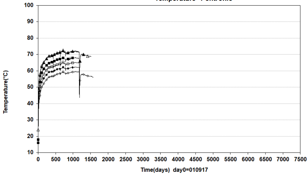
Prototype\Hole 1 \Ring5 (20010917-20220101) Temperature - Pentronic
