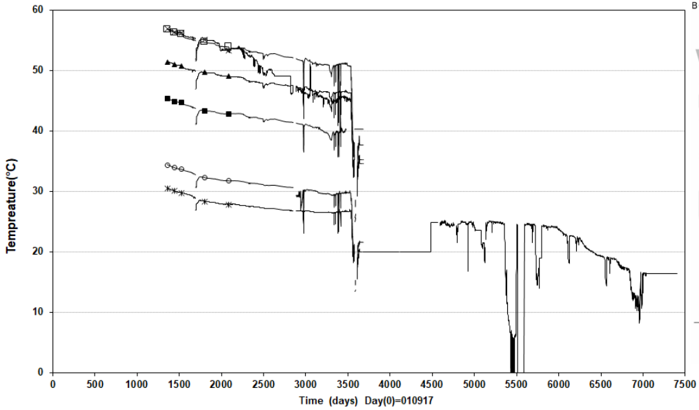
PrototypelHole 1 (20010917-20220101) Temprature - Geokon
