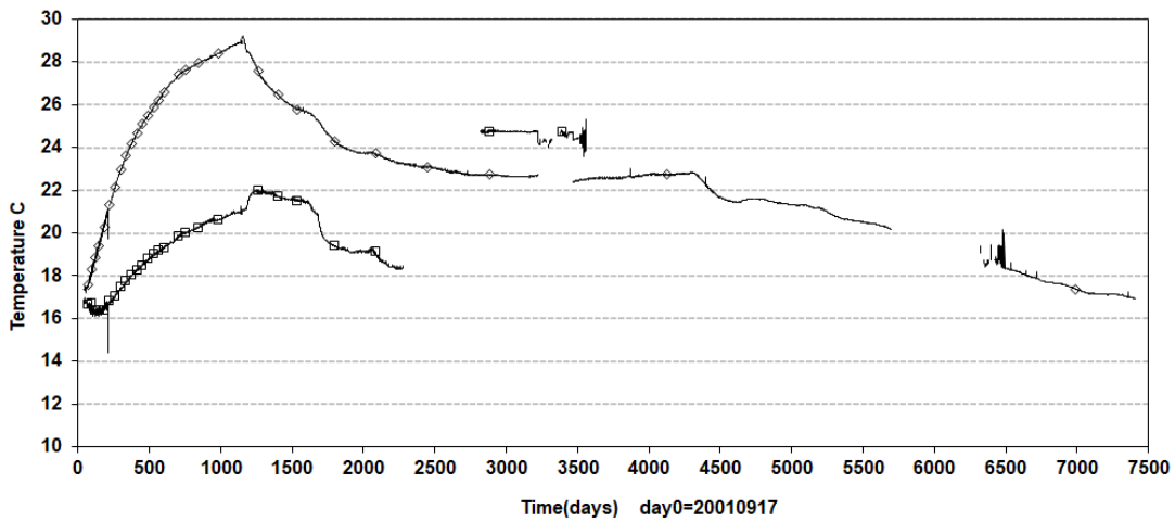
Prototype\ Backfill \ Between dep.hole 2-3 (20010917-20220101) Temperature - Pentronic
