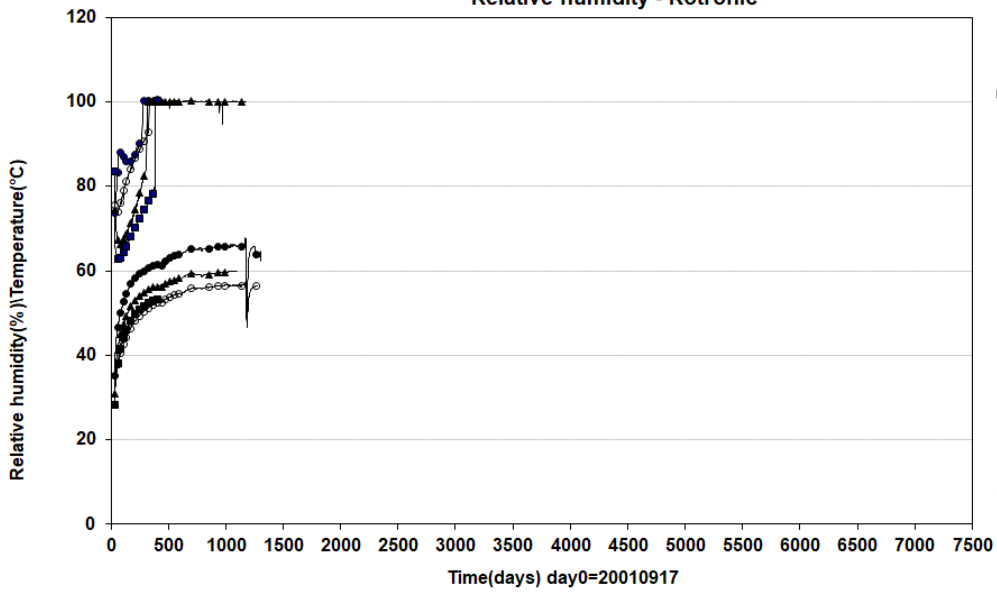
Prototype\Hole 3\Ring 10 (20010917-20220101) Relative humidity - Rotronic
