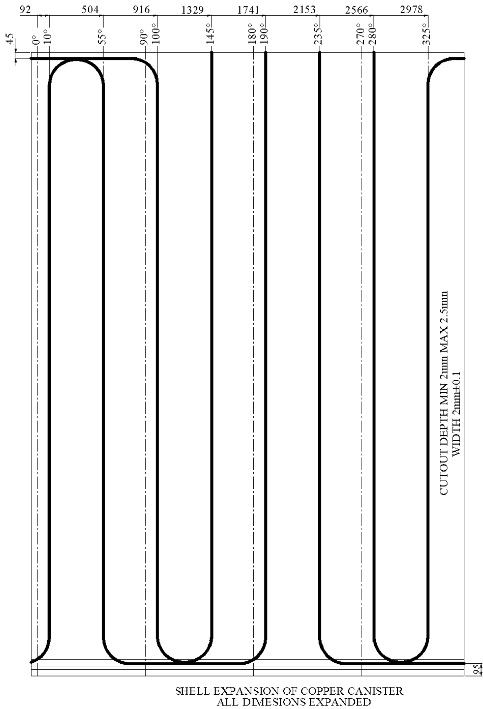
Figure 4-2 Laying of the optical fibre cables with protection tube of Inconel 625 (outer diameter 2 mm) for measurement of the canister surface temperature (surface unfolded).
