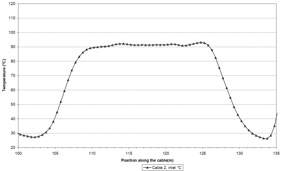
Prototype\ Hole 3 \Canister (050601) Temperature profile on the canister surface - Optical fiber cables
