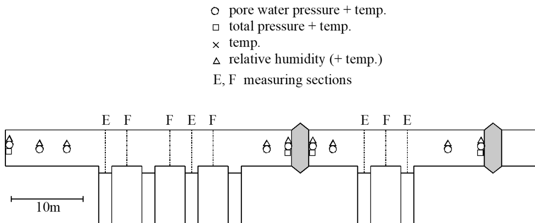
Figure 4-5 Schematic view over the instrumentation of the backfill.
