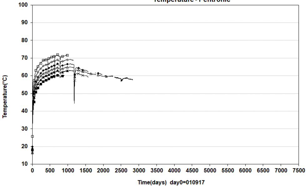
Prototype\Hole 1 \Ring5 (20010917-20220101) Temperature - Pentronic
