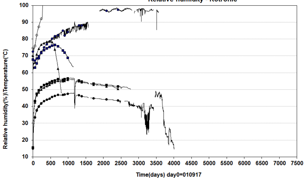
Prototyp\Hole 1\Cyl.1 (20010917-20220101) Relative humidity - Rotronic
