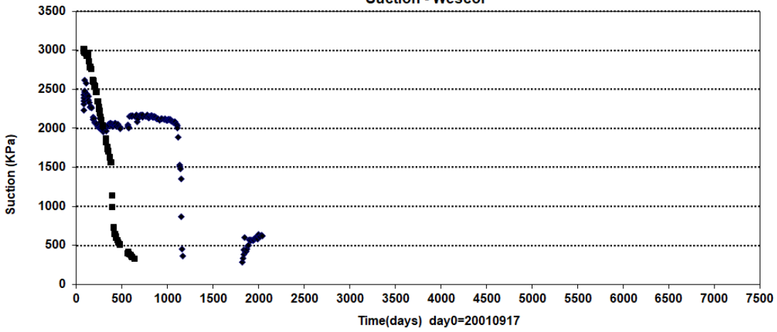
Prototype\Backfill \ In front of plug (20010917-20220101) Suction - Wescor
