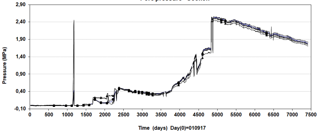
Prototype\Backfill\Section 1 (20010917-20220101) Pore pressure - Geokon
