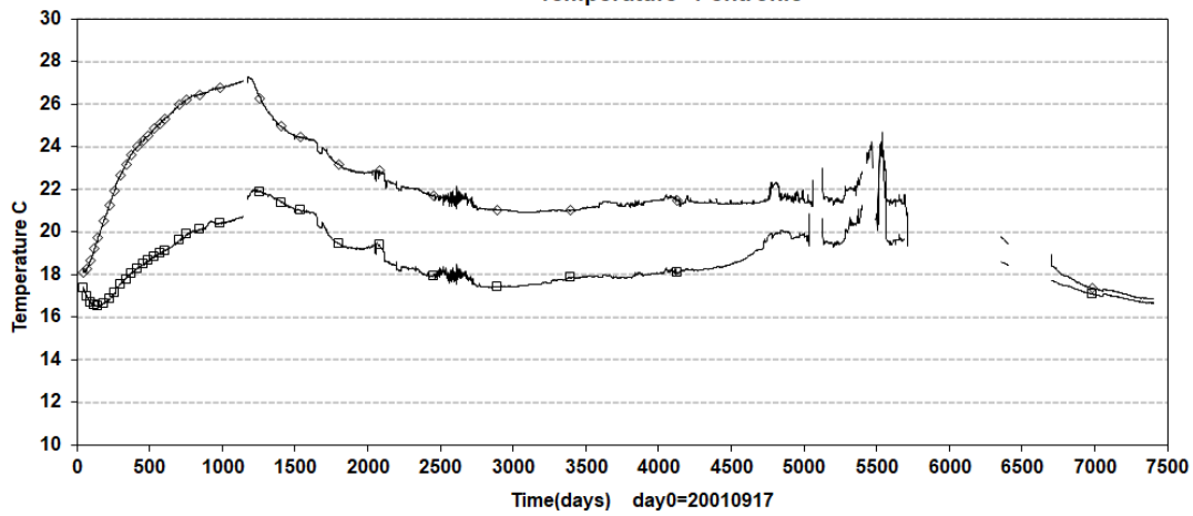
Prototype\ Backfill \ Between dep.hole 1-2 (20010917-20220101) Temperature - Pentronic
