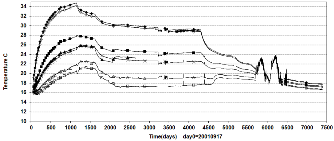
Prototype\ Backfill \ Above dep.hole3 (20010917-20220101) Temperature - Pentronic
