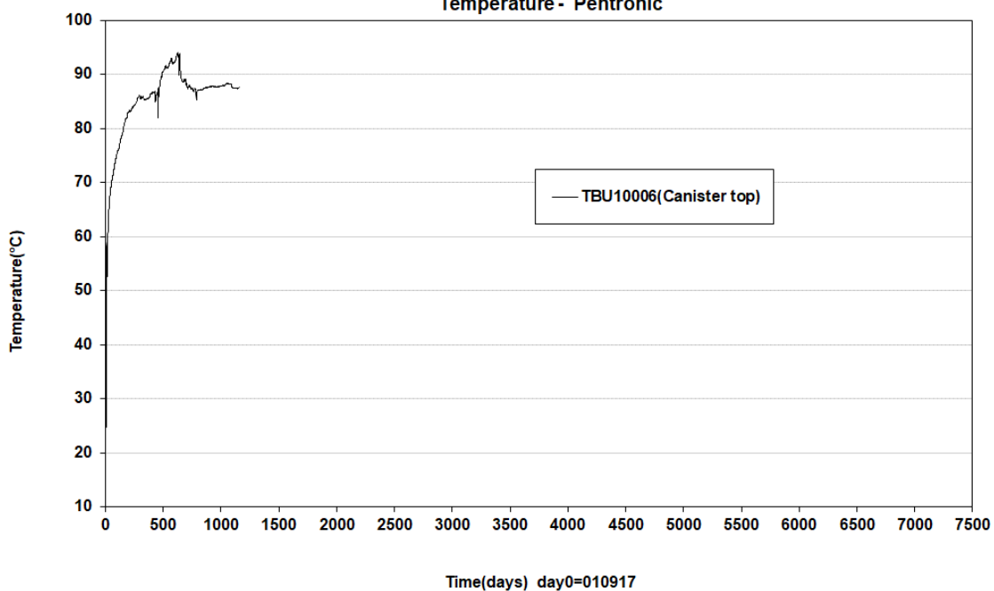
Prototype\Hole 2 \Canister top (20010917-20220101) Temperature - Pentronic
