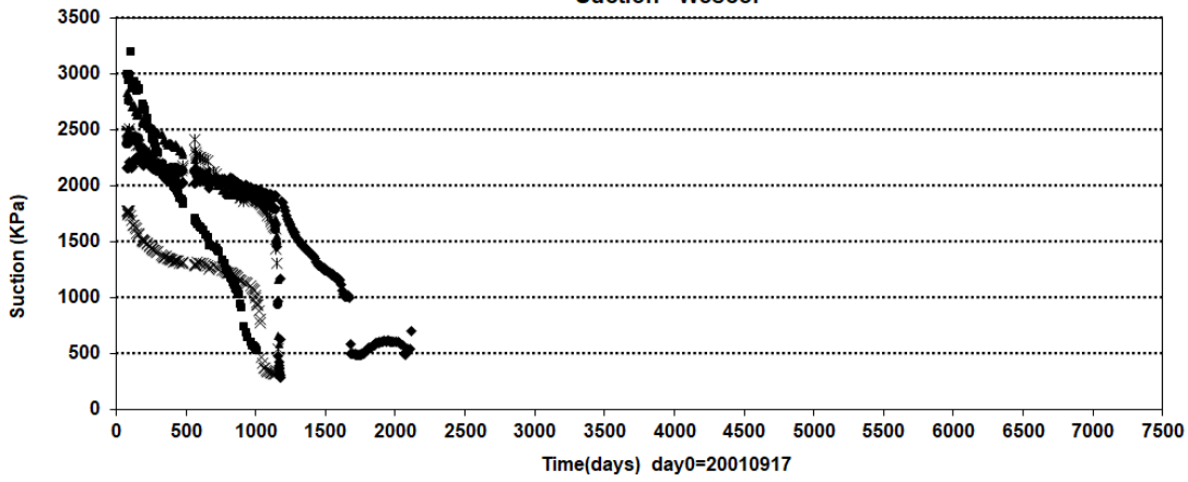
PrototypelBackfill \ Between dep.hole 1 and hole 2 (20010917-20220101) Suction - Wescor
