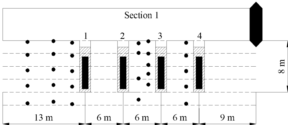
Figure 4-3 Overview of the temperature sensors in the rock. Length section.
