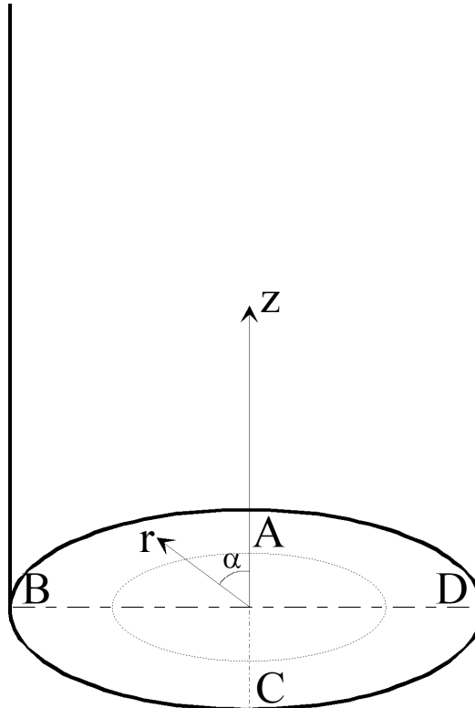
Figure 2-1 Figure describing the instrument planes (A-D) and the coordinate system used when describing the instrument positions(A headed against the end of the tunnel).
