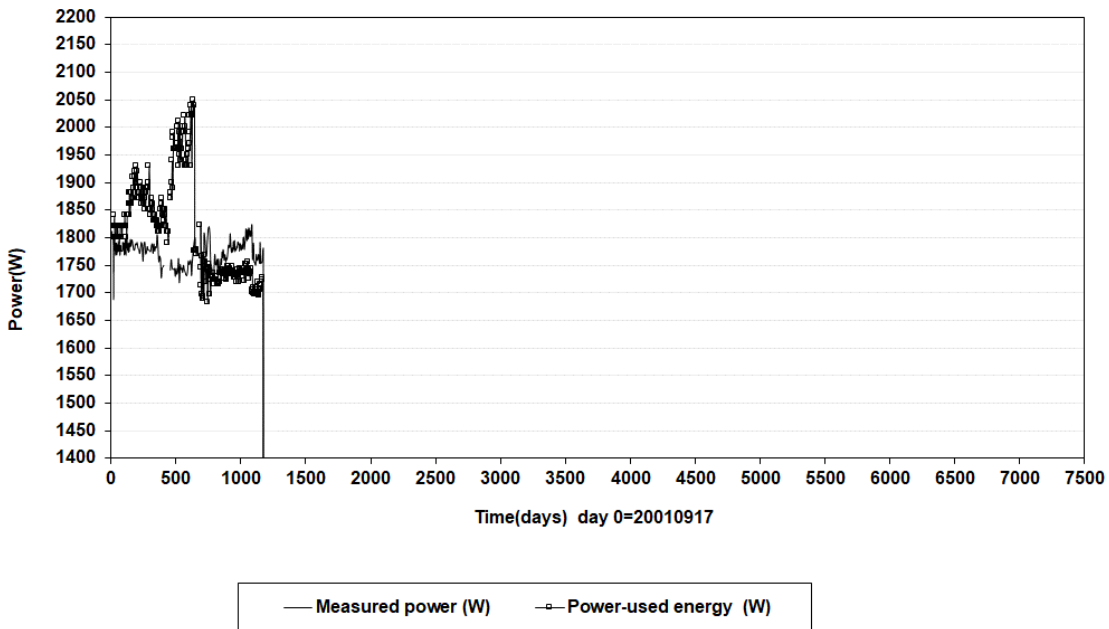
Prototype\Hole 2 (20010917-20220101) Canister power
