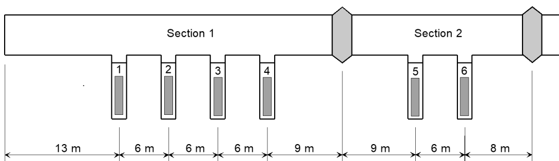
Figure 1-1 Schematic view of the Prototype Repository.
