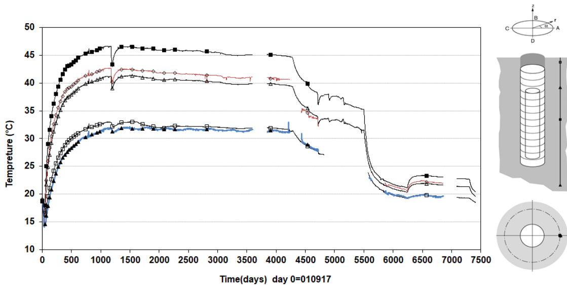
Prototype\Rock\Hole 4 (20010917-20220101) Temperature - Pentronic
