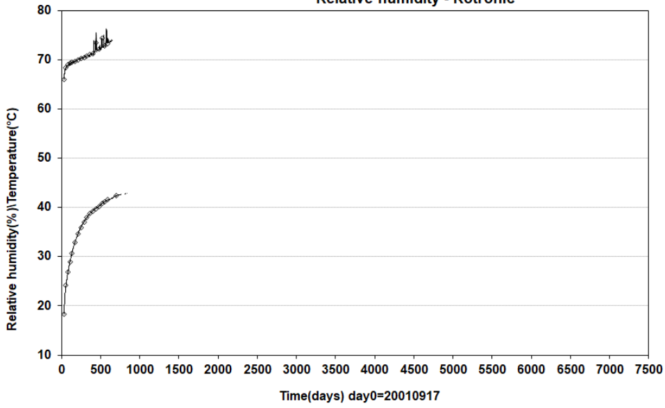
Prototype\Hole 3\Cyl.3 (20010917-202210101) Relative humidity - Rotronic
