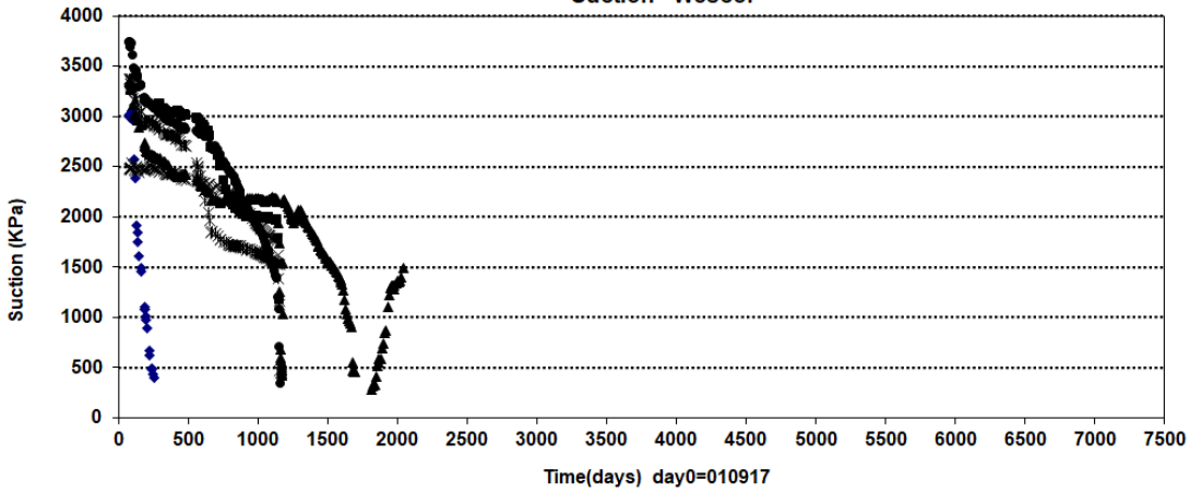
Prototype\Backfill \ Between dep.hole 3 and hole 4 (20010917-20220101) Suction - Wescor
