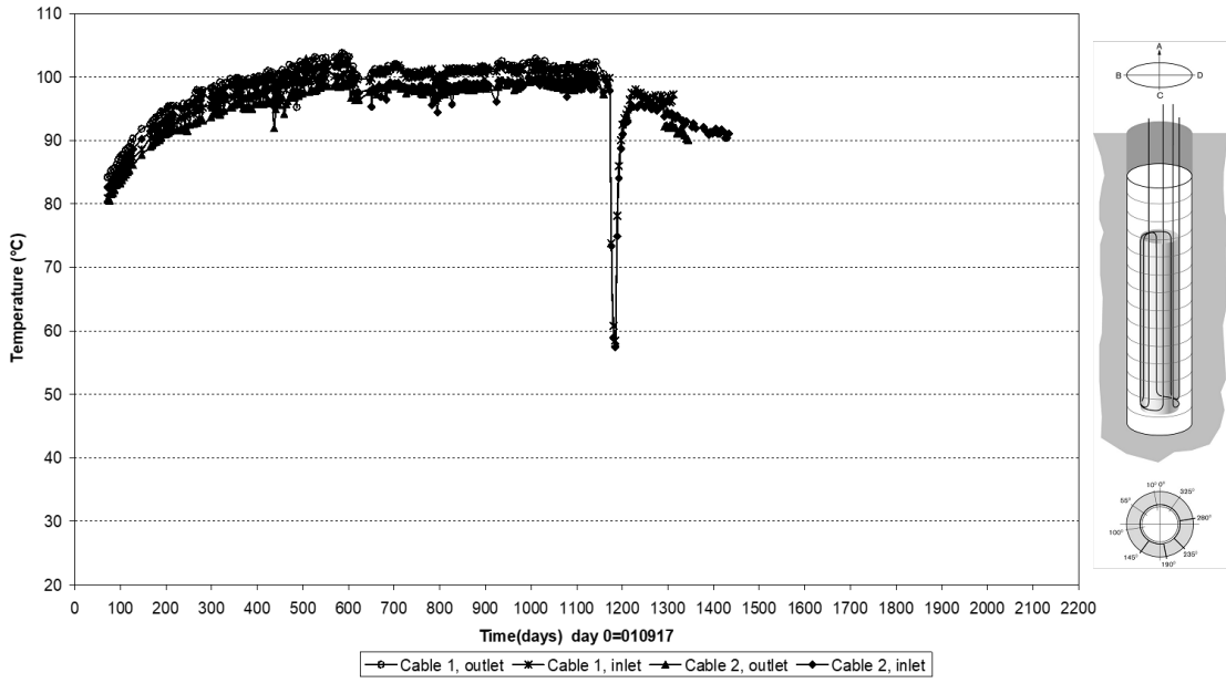
Prototype\ Hole 3 \Canister (050601) Temperature profile on the canister surface - Optical fiber cables
