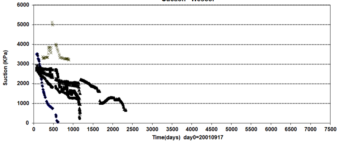
PrototypelBackfill \ Between dep.hole 2 and hole 3 (20010917-20220101) Suction - Wescor
