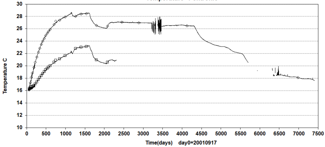
Prototype\ Backfill \ Between dep.hole 3-4 (20010917-20220101) Temperature - Pentronic
