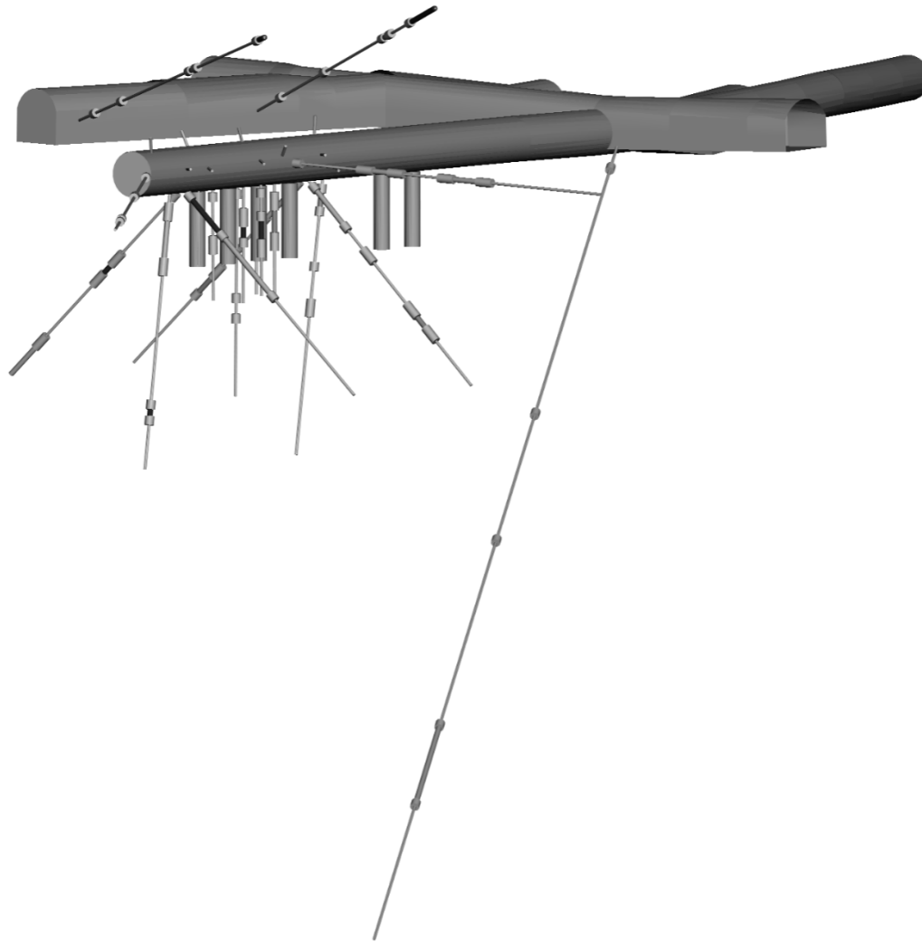
Figure A5-0-1. View of the drilled core holes in the Prototype Repository Section I. The length from the I-tunnel to the end of the TBM-tunnel is 90 m. The diameter of the TBM tunnel is 5m and the diameter of the deposition holes is 1.75 m. The depth of the deposition holes is holes is 8.37 m in the centre and 8.15 m along the deposition hole wall. The diameter of the core holes is 76 mm except for the short core holes in the roof of the TBM tunnel that have a diameter of 56 mm. The monitoring boreholes used in the presentation in this report are located in the inner part of the tunnel surrounding the area with the four innermost canister holes. Also included are two holes drilled from the G-tunnel and the long hole KA3510A drilled from the main tunnel.
