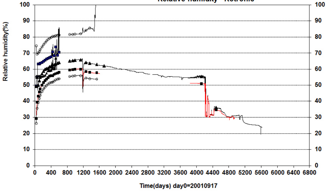
Prototype\Hole 3\Cyl.1 (20010917-20200101) Relative humidity - Rotronic
