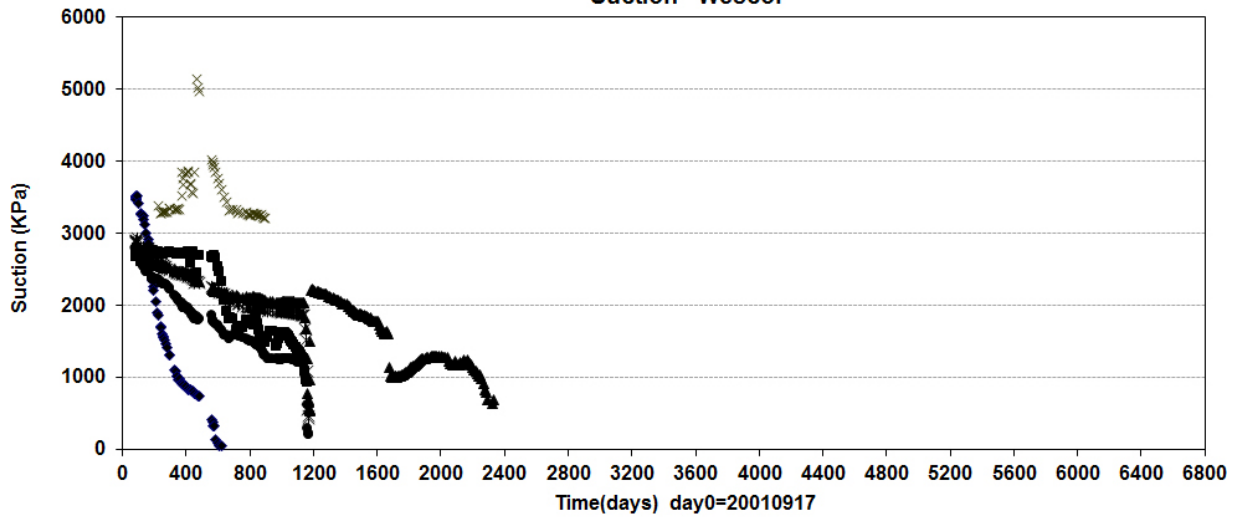
Prototype\Backfill \ Between dep.hole 2 and hole 3 (20010917-20200101) Suction - Wescor
