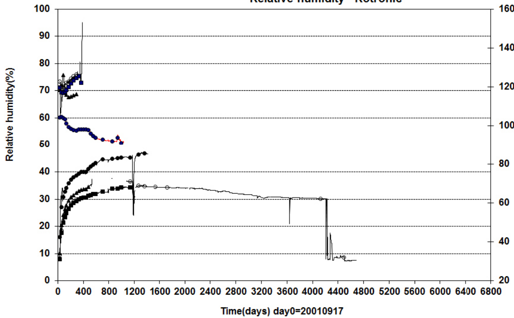
Prototype\Hole 3\Ring 5 (20010917-20200101) Relative humidity - Rotronic
