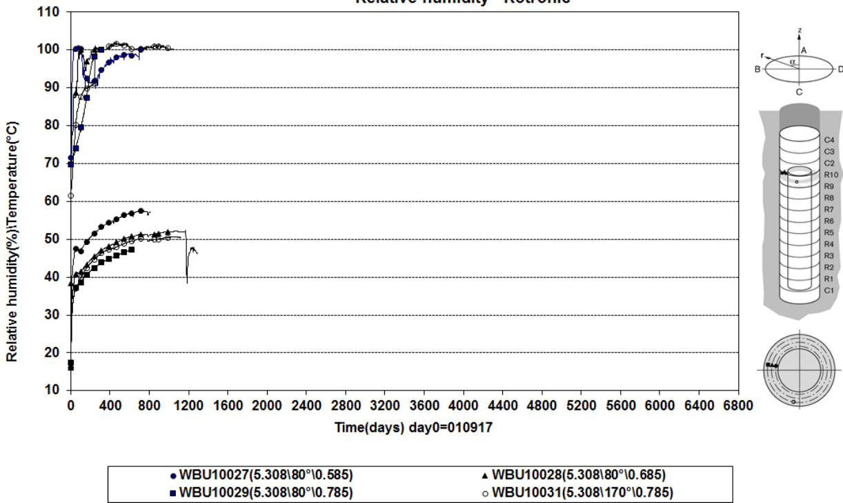
Prototyp\Hole 1\Ring10 (20010917-20200101) Relative humidity - Rotronic
