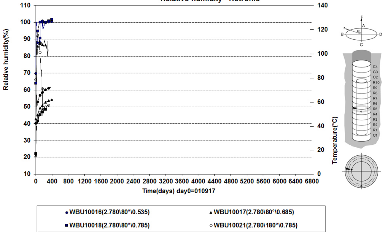
Prototyp\Hole 1\Ring.5 (20010917-20200101) Relative humidity - Rotronic
