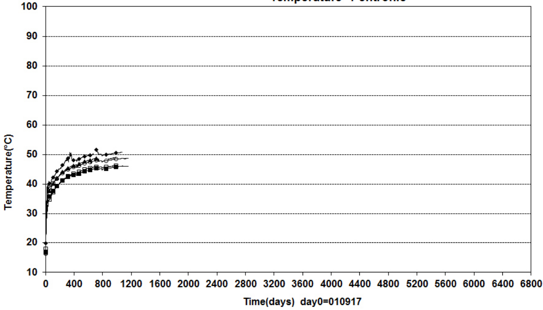
Prototype\Hole 1 \Ring10 (20010917-20200101) Temperature - Pentronic
