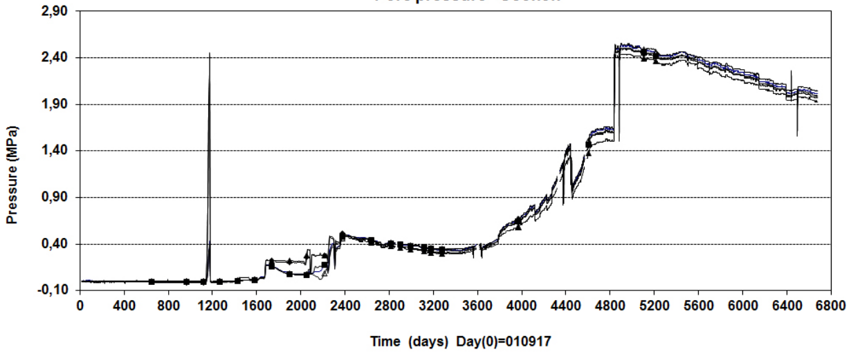
Prototype\Backfill\Section 1 (20010917-20200101) Pore pressure - Geokon
