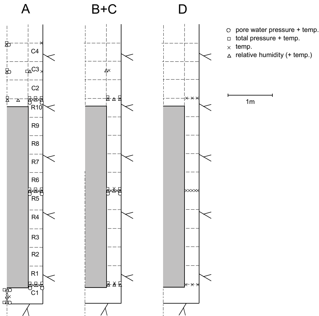
Figure 4-1. Schematic view over the instruments in four vertical sections and the block designation.
