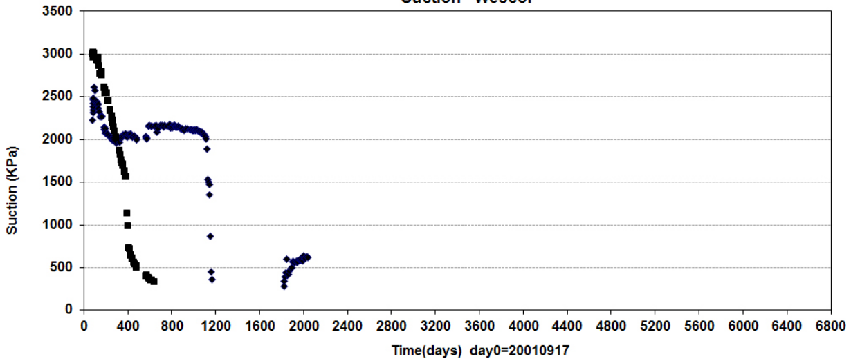
Prototype\Backfill \ In front of plug (20010917-20200101) Suction - Wescor
