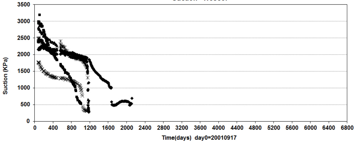
Prototype\Backfill \ Between dep.hole 1 and hole 2 (20010917-20200101) Suction - Wescor
