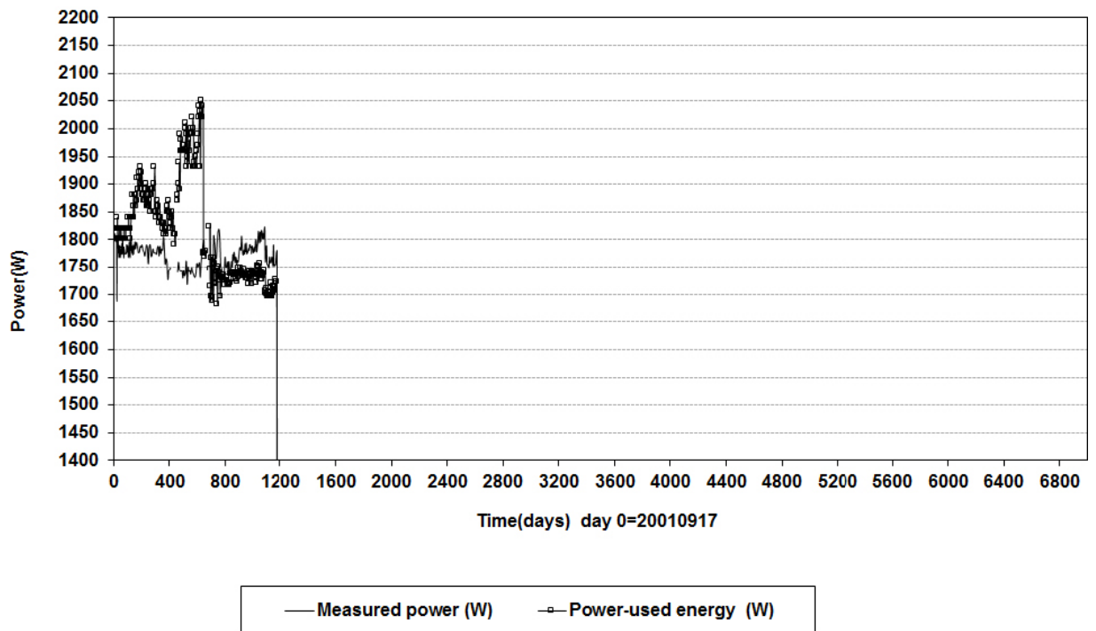
Prototype\Hole 2 (20010917-20200101) Canister power
