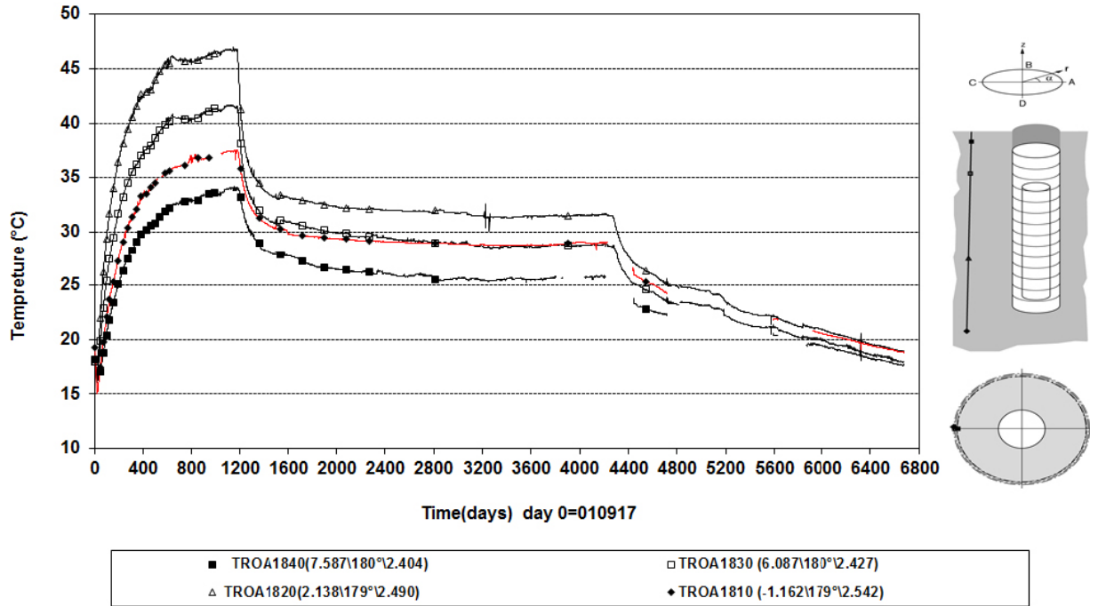
Prototype\Rock\Hole 2 (20010917-20200101) Temperature - Pentronic
