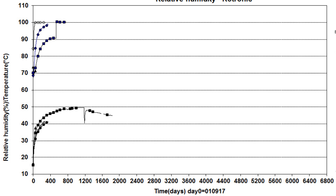
Prototyp\Hole 1\Cyl.1 (20010917-20200101) Relative humidity - Rotronic
