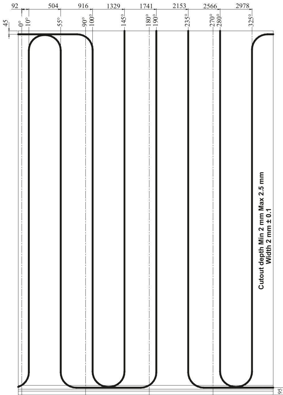
Shell expansion of copper canister All dimesions expanded
