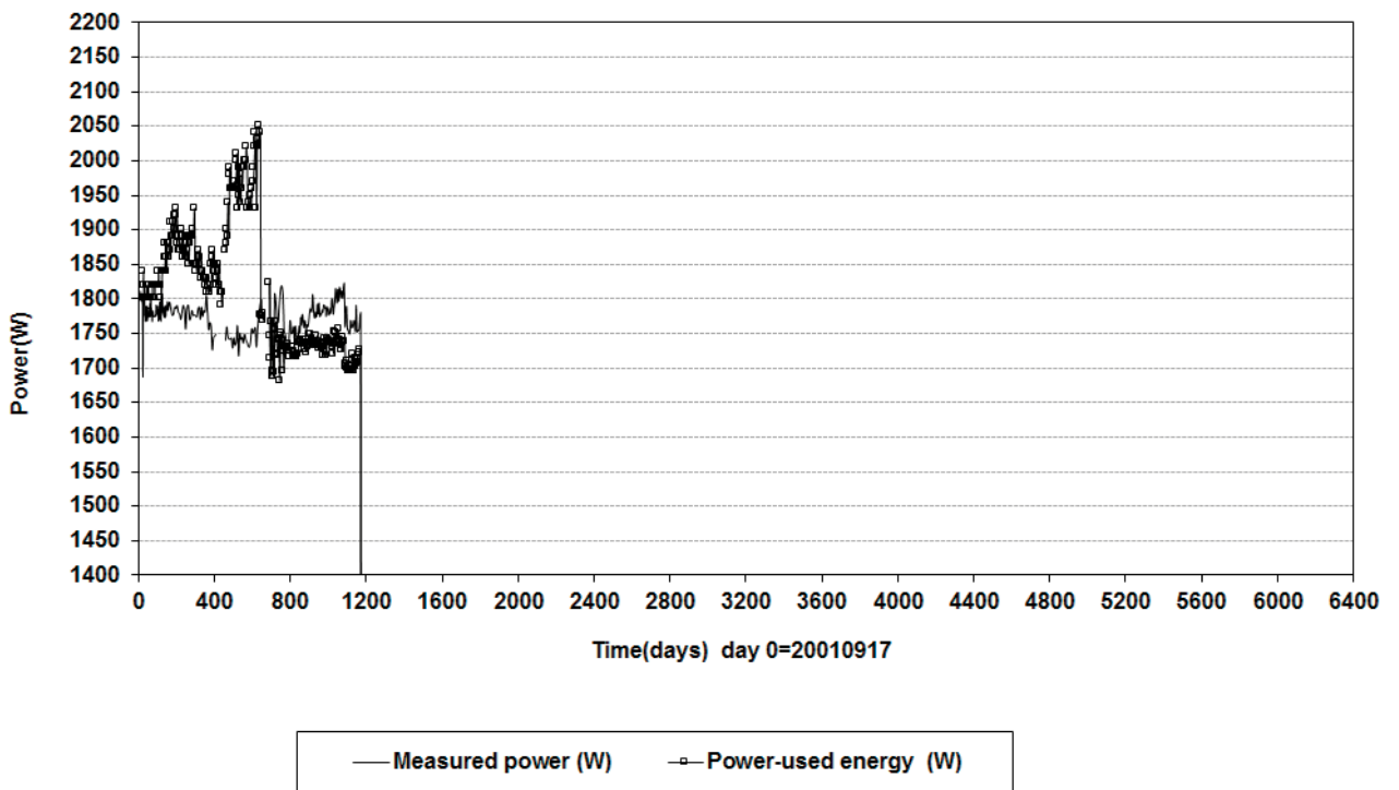
Prototype\Hole 2 (20010917-20190101) Canister power
