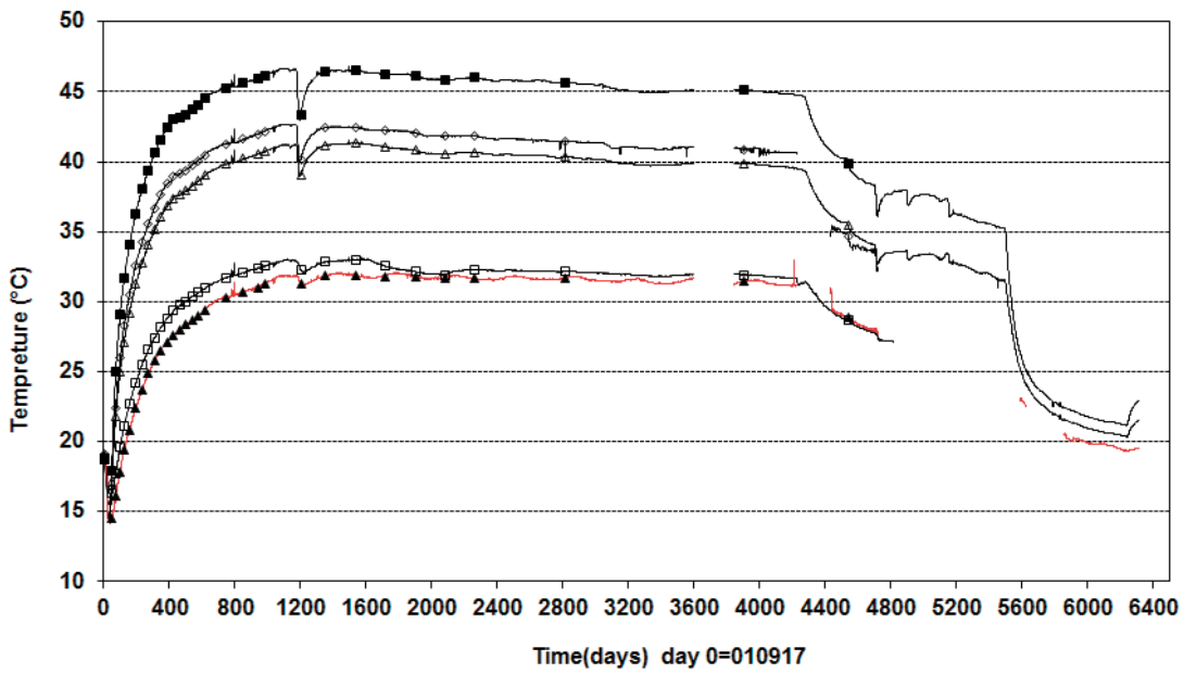
Prototype\Rock\Hole 4 (20010917-20190101) Temperature - Pentronic
