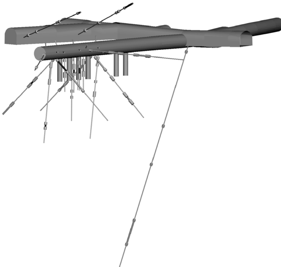
Figure A5-1. View of the drilled core holes in the Prototype Repository Section 1. The length from the I-tunnel to the end of the TBM-tunnel is 90 m. The diameter of the TBM-tunnel is 5m and the diameter of the deposition holes is 1.75 m. The depth of the deposition holes is 8.37 m in the centre and 8.15 m along the deposition hole wall. The diameter of the core holes is 76 mm except for the short core holes in the roof of the TBM tunnel that have a diameter of 56 mm. The monitoring boreholes used in the presentation in this report are located in the inner part of the tunnel surrounding the area with the four innermost canister holes. Also included are two holes drilled from the G-tunnel and the long hole KA3510A drilled from the main tunnel.
