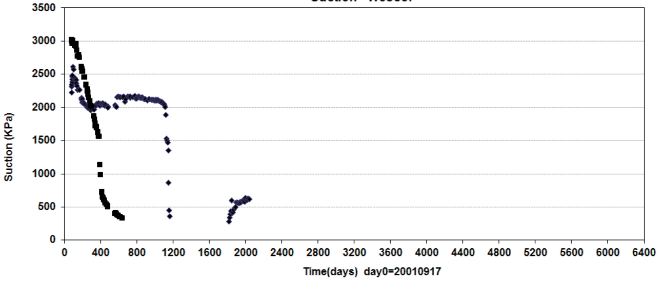
Prototype\Backfill \ In front of plug (20010917-20190101) Suction - Wescor
