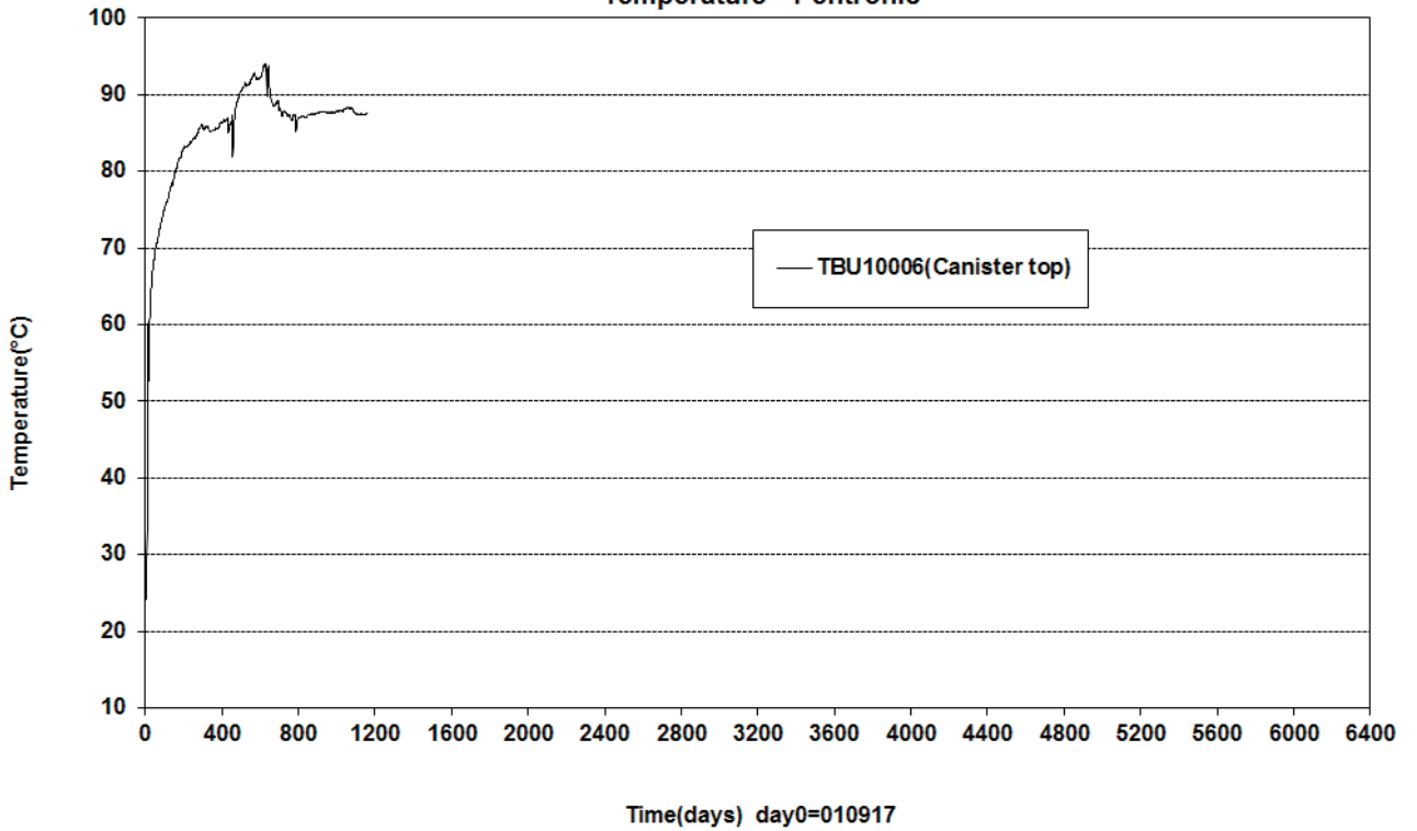
Prototype\Hole 2 \Canister top (010917-20190101) Temperature - Pentronic
