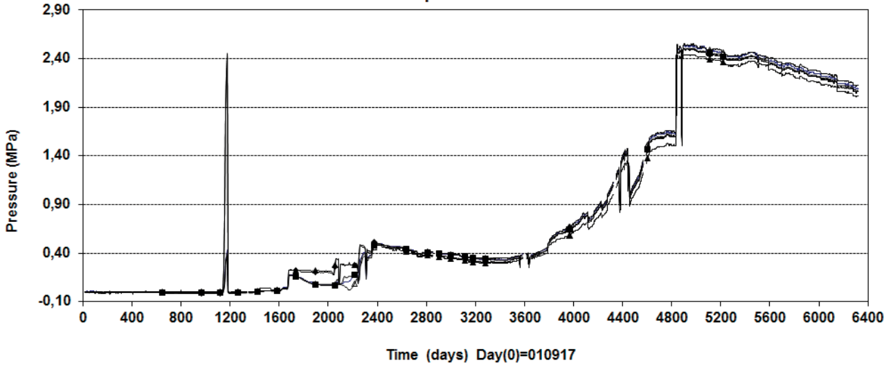
Prototype\Backfill\Section 1 (010917-20190101) Pore pressure - Geokon
