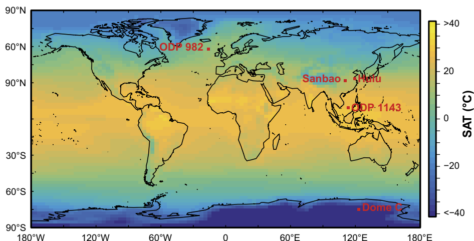
Figure 3-11. Map highlighting the source locations of the proxy data records. Temperature records are from Antarctica (Dome C), the South China Sea (ODP 1143), and the North Atlantic (ODP 982). East Asian Monsoon records are from central (Sanbao Cave) and eastern China (Hulu Cave). Background shading illustrates pre-industrial SAT ( ^{\circ}\text{C} ) taken from a HadCM3 control simulation.
