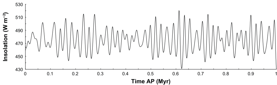
Figure 3-16. Evolution of summer insolation ( W m^{-2} ) at 65^{\circ}N for the next million years, calculated using the method of Laskar et al. (2004).
