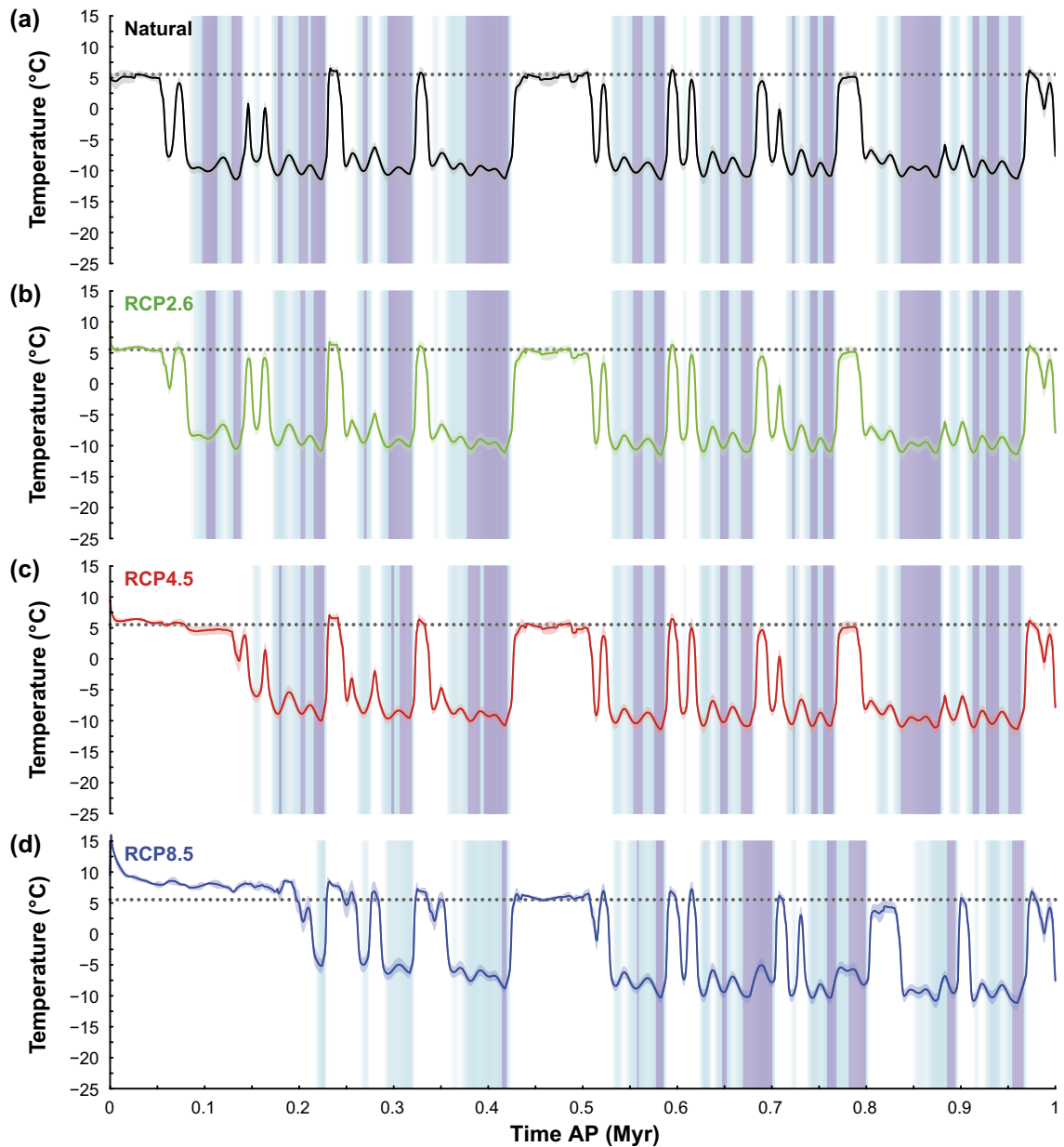
Figure 4-14. Time series of emulated downscaled mean annual SAT (°C) for the next 1 Myr assuming no ice cover during glacial conditions at the Forsmark site, for the natural (a), RCP2.6 (b), RCP4.5 (c), and RCP8.5 (d) emissions scenarios, downscaled using the bias-correction technique. During glacial periods, GSL is allowing to reach a minimum of -46 m and is then held constant until it increases towards interglacial conditions. SAT is modelled every 1 kyr. Error bands represent the emulated grid box posterior variance (1 SD). Vertical bands represent periods when the Fennoscandian ice sheet is covering the site, with purple shading indicating higher confidence ( GSL < -93 m) and cyan shading indicating lower confidence ( -93 \text{ m} < GSL < -53 m) ice coverage. A higher degree of cyan shading indicates lower uncertainty. The grey dotted line represents present-day mean annual SAT at the site ( 5.5 °C) taken from the CRU 0.5^\circ gridded climatology for the period 1961–1990 (New et al. 1999).
