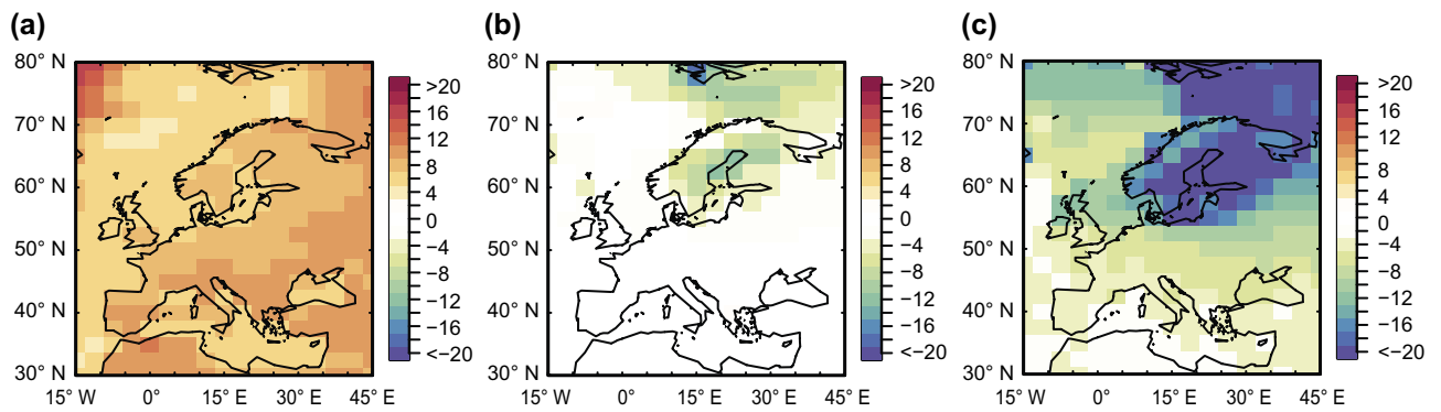
Figure 4-5. Emulated mean annual SAT anomaly ( ^{\circ}\text{C} ) for the region of Europe for the RCP8.5 emissions scenario. Snapshots have GSL values of: (a) +24 m (5 kyr AP), (b) -46 m (215 kyr AP), and (c) -122 m (796 kyr AP).
