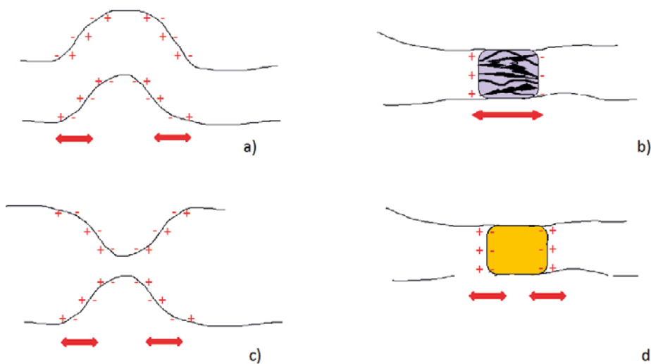
Figure 5-1. Illustrations of microscale features of the rock's porous system that may cause dielectric behaviour. The red arrows indicate zones of capacitance effects.
