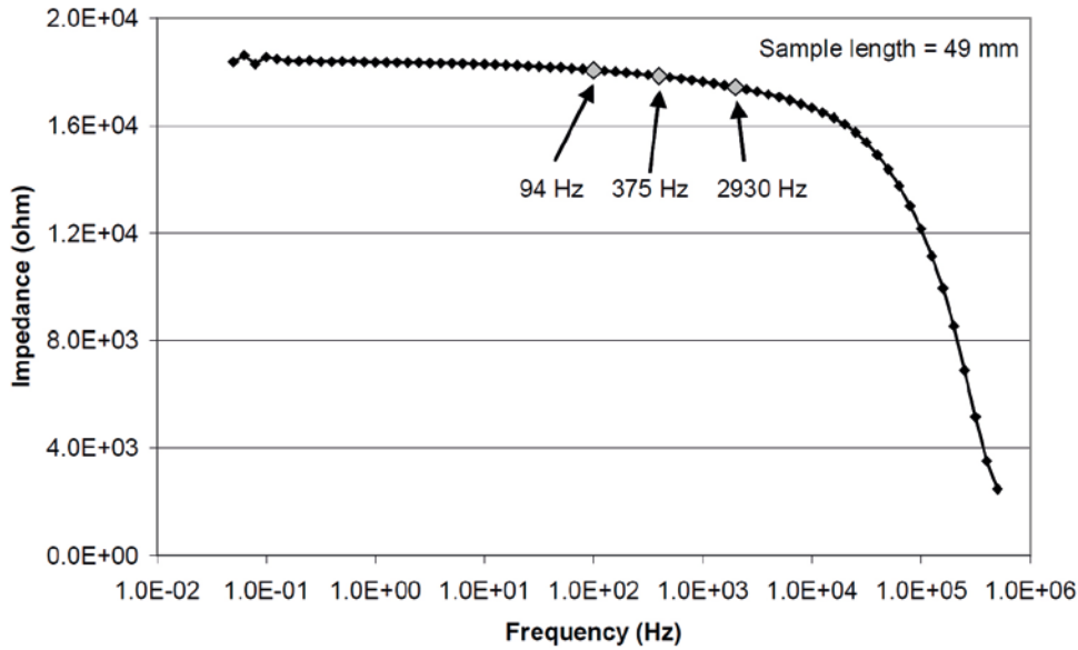
Figure 5-7. Impedance spectroscopy of Laxemar sample saturated with 1 M NaCl. Reproduced from Löfgren (2001, Figure 5-15).
