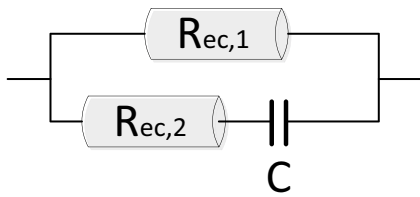
Figure 5-2. Electric circuit representation of rock, incorporating capacitance effects in the electric double layer.
