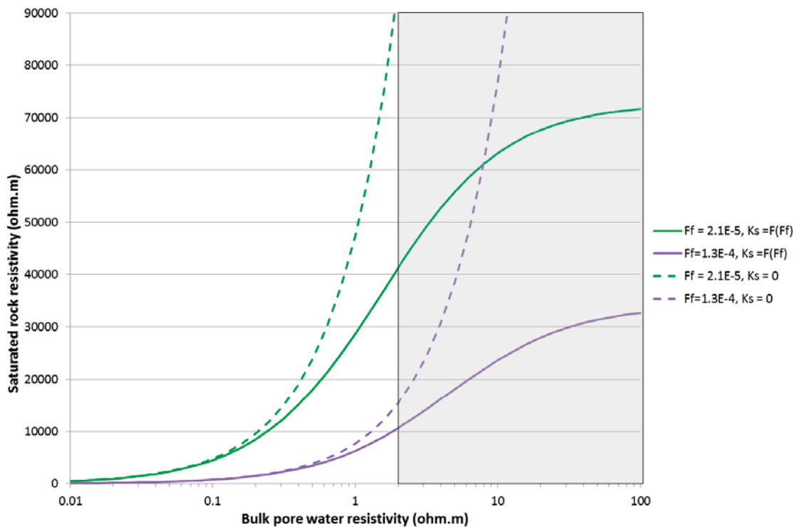
Figure 4-5. Saturated rock resistivity vs. bulk pore water resistivity. The solid lines correspond to calculations by Equation 4-7, where the surface conduction is a function of the formation factor. The dashed lines correspond to calculations by Equation 1-2, neglecting surface conduction. The shaded area shows pore water resistivities from which no formation factor has been derived in SR-Site.
