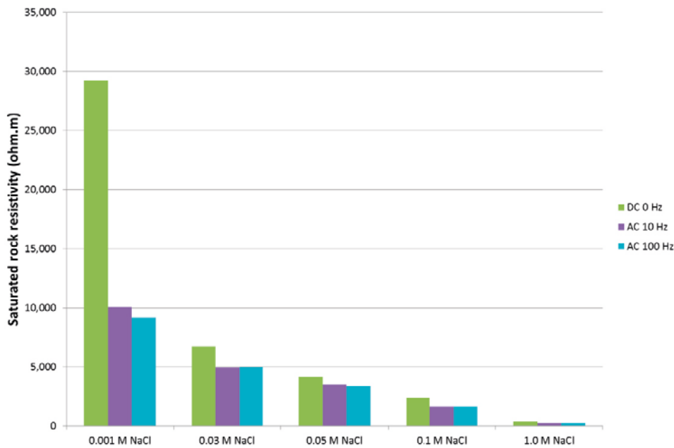
Figure 5-10. Saturated rock resistivities of Sample 1 from Forsmark (cf. Table 4-1) at different frequencies, as saturated by different pore water solutions.
