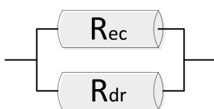
Figure 3-1. Parallel coupled resistors where R_{ec} represents the resistance associated with electrolytic conduction in the pore water and R_{dr} is the resistance of the dry rock.
