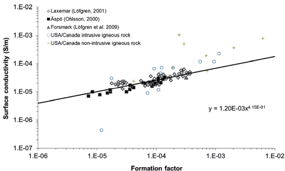
Figure 4-4. Surface conductivity vs. formation factor. Data from Ohlsson (2000) and Löfgren (2001), as well as the correlation, are the same as in Figure 4-3. Added data points come from reinterpretations of experimental data in Brace et al. (1965) and Brace and Orange (1968). Data point from Forsmark is reinterpreted, based on Figure 4-2.
