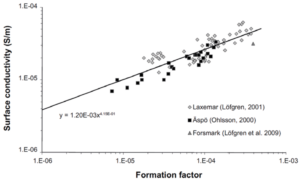
Figure 4-3. Surface conductivity vs. formation factor. Based on measurements on crystalline rock samples from the Oskarshamn and Forsmark sites. Reproduced from SKB (2010a, Figure 6-72).
