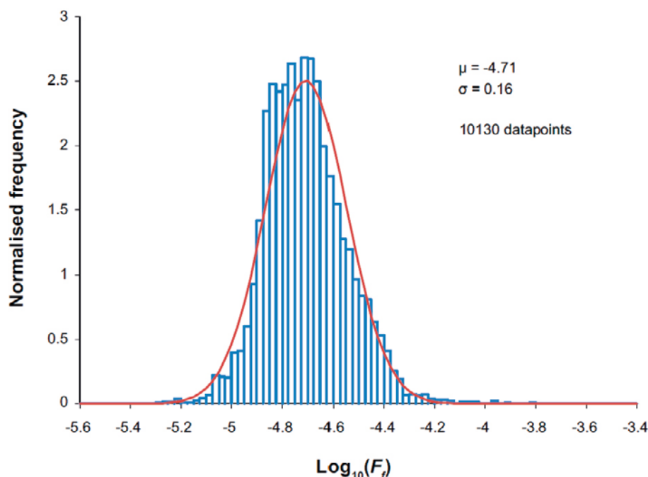
Figure 2-2. Histogram of all in situ formation factor data from boreholes KFM01D, KFM06A, and KFM08C, for the non-fractured rock matrix, together with the best fit \log_{10} -normal distribution. It should be noted that corrections have been made and accordingly the histogram does not reflect the apparent formation factor but the formation factor. Image reproduced from SKB (2010a, Figure 6-78).
