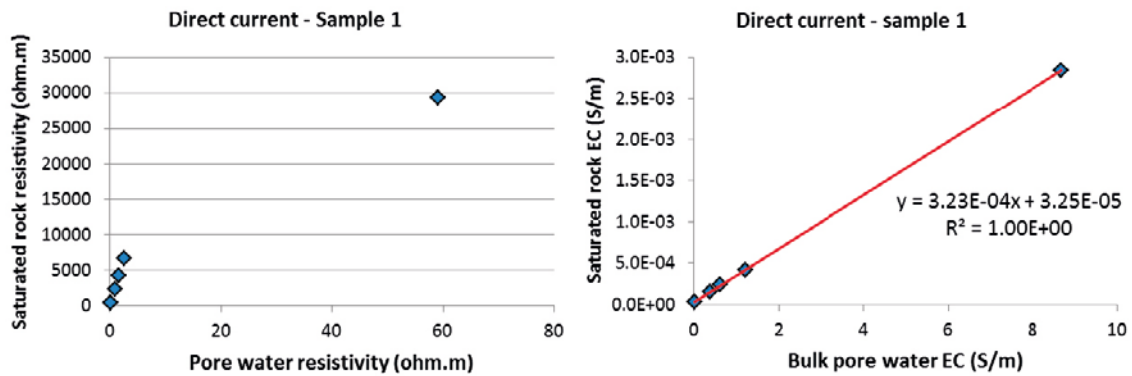
Figure 4-2. Left: DC saturated rock resistivity plotted vs. the bulk pore water resistivity of Table 4-1. Right: DC saturated rock conductivity vs. bulk pore water EC of Table 4-1. Red curve represents a linear fitting according to Equation 4-4, where the fitting parameters are shown. The data are obtained on a drill core sample from Forsmark (cf. Table 3-6).
