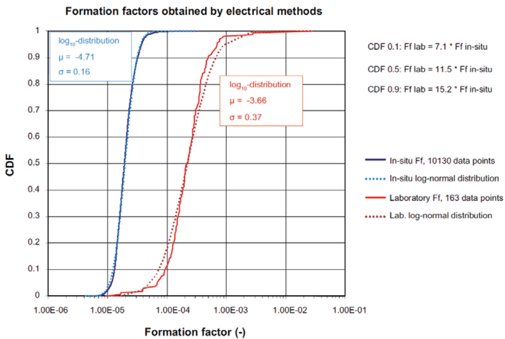
Figure 2-4. Blue curves: CDF and best fit log-normal distribution of in situ formation factors for borehole KFM01D, KFM06A, and KFM08C. Red curves: CDF and best fit log-normal distribution of laboratory formation factors obtained by the electrical resistivity method. Image reproduced from SKB (2010a, Figure 6-80).
