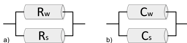
Figure 4-1. a) Parallel coupled resistors where R_w (ohm) represents the resistance associated with electrolytic conduction in the bulk part of the pore water and R_s (ohm) represents the resistance associated with surface conduction. b) Parallel coupled conductors where C_w (S) is the conductance associated with electrolytic conduction in the bulk part of the pore water and C_s (S) is the conductance associated with surface conduction.
