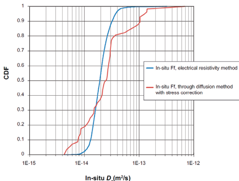
Figure 2-5. Comparison of CDFs of in situ effective diffusivity obtained by the two approaches of analysing data. The blue curve represents approach 1 and the red curve approach 2. Image reproduced from SKB (2010a, Figure 6-81).
