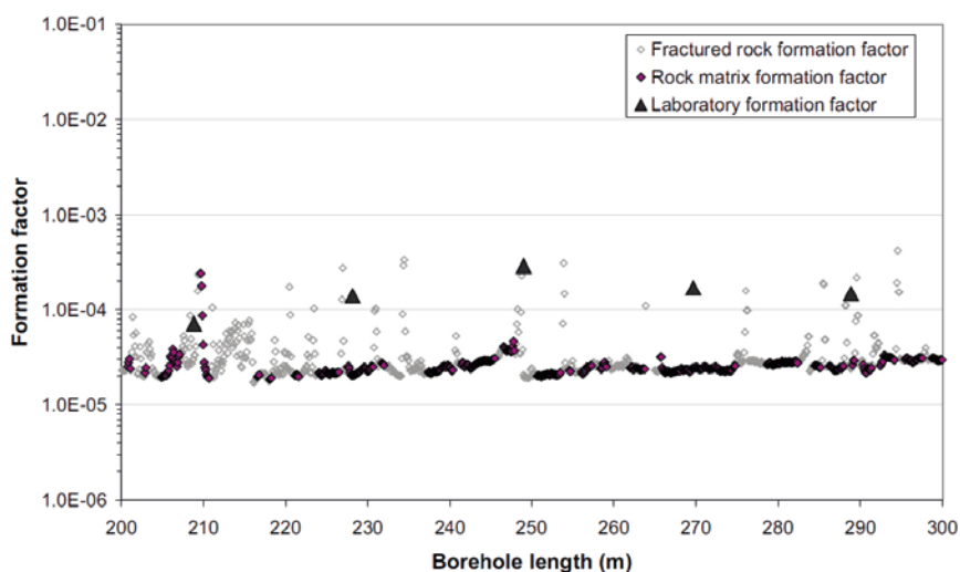
Figure 2-1. In situ apparent formation factors (diamonds) and laboratory apparent formation factors (triangles) obtained by electrical methods for borehole KFM05A. For what is labelled rock matrix formation factors in the figure, in situ data from drill core sections that are intersected by open fractures, detected in the drill core mapping, have been discarded. This is to assure that the electrical properties of the non-fractured rock matrix are reflected. The electrical conductivity of the groundwater in the displayed borehole section is \sim 1 S/m. Image reproduced from Löfgren et al. (2006, Appendix C1). When composing Löfgren et al. (2006), the term formation factor was (erroneously) used for the apparent formation factor, as long as the difference between the two parameters was estimated to be small.
