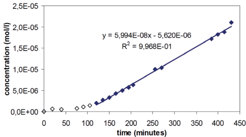
Figure 6-1. TEM experiment: Iodide breakthrough curve for sample AD-1 (10 mm length). Full diamonds represent steady state conditions. Tracer injection occurs at 0 minutes. Figure reproduced from Vecernik et al. (2012, Figure 6).
