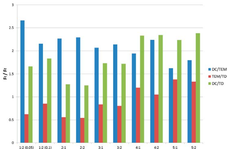
Figure 6-3. Ratios of the DC, TEM and through-diffusion (TD) formation factors, for the Forsmark samples of Löfgren et al. (2009).
