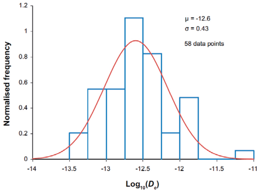
Figure 2-3. Histogram of all effective diffusivities from laboratory through-diffusion measurements in Forsmark, except for those of samples with porosities over 10% that are considered as outliers at the site. Image reproduced from SKB (2010a, Figure 6-79).
