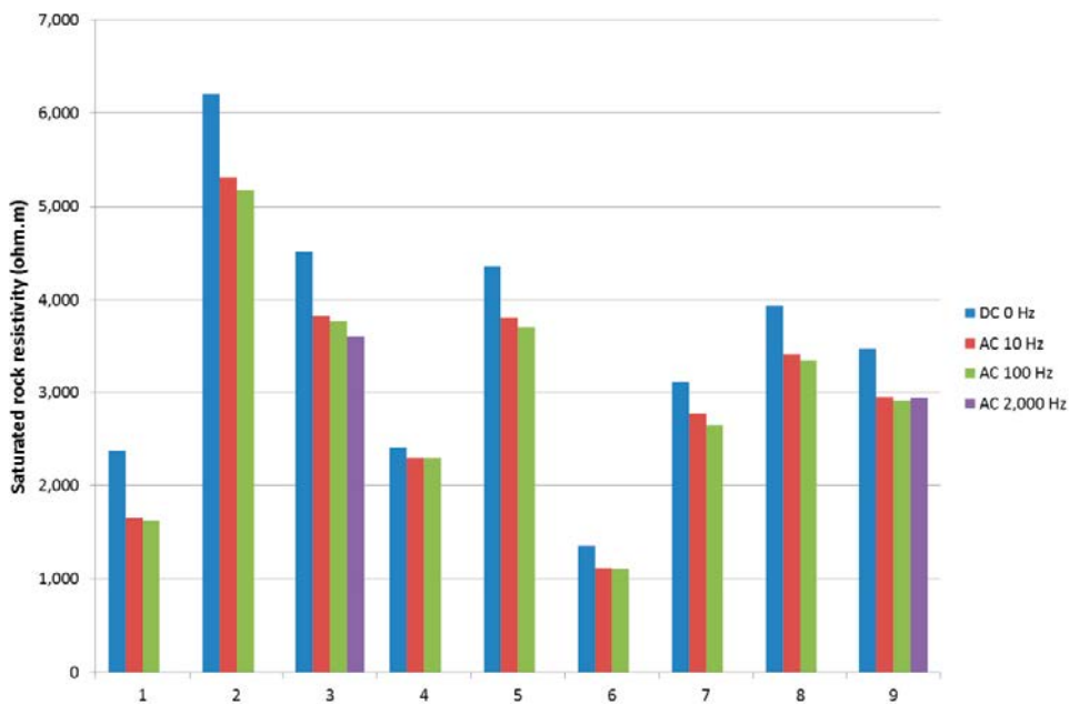
Figure 5-9. Saturated rock resistivities of nine Forsmark and Oskarshamn rock samples (cf. Table 3-8) at different frequencies. The saturation solution is 0.1 M NaCl for samples of odd numbers, and 0.05 M NaCl for samples of even numbers.
