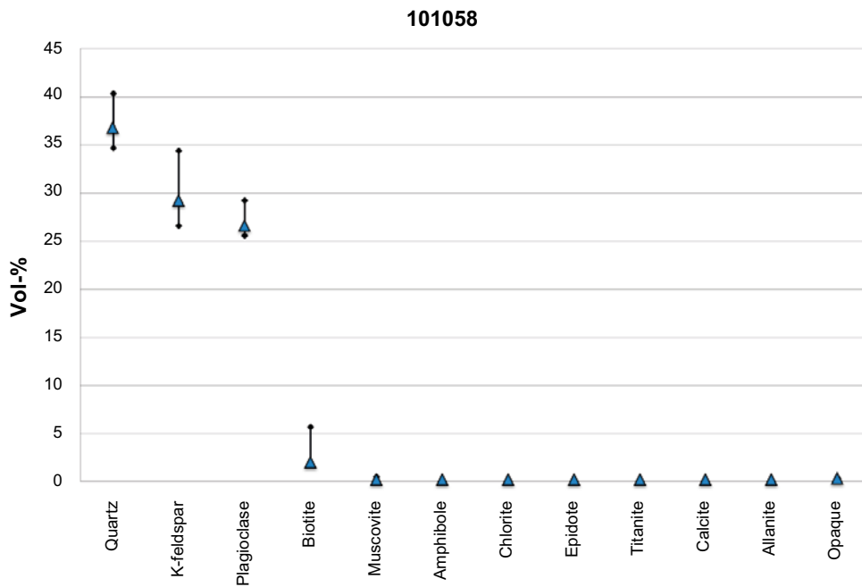
Figure 3-5. Mineral composition of rock type 101058 – Metamorphosed, aplitic granite. The whiskers show the upper and lower quartiles. Data taken from Sandström and Stephens (2009, Table 3-11).
