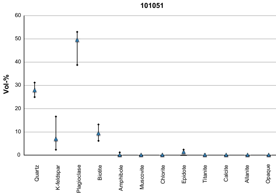
Figure 3-6. Mineral composition of rock type 101051 – metamorphosed, fine- to medium-grained granitoid. The whiskers show the upper and lower quartiles. Data taken from Sandström and Stephens (2009, Table 3-3).
