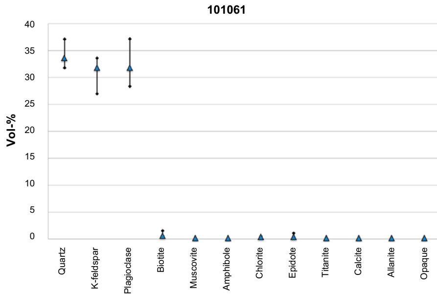
Figure 3-4. Mineral composition of rock type 101061 – pegmatite or pegmatitic granite. The whiskers show the upper and lower quartiles. Data taken from Sandström and Stephens (2009, Table 3-12).
