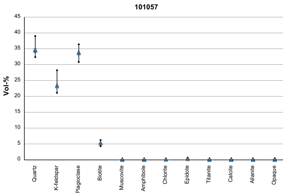
Figure 3-3. Mineral composition of rock type 101057 – metamorphosed, medium-grained granite to granodiorite. The whiskers show the upper and lower quartiles. Data taken from Sandström and Stephens (2009, Table 3-7).
