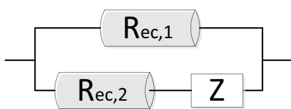
Figure 5-3. Electric circuit representation of rock, internalising frequency dependent impedance effects in the pores. Adapted from Telford et al. (1990, Figure 9.3).
