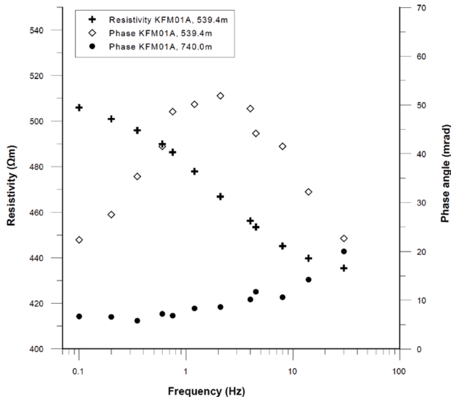
Figure 5-6. Resistivity (ohm.m) and phase angle (mrad) plotted versus measurement frequency for an anomalous sample (KFM01A, 539.39–539.42 m). Phase angle results for a normal sample (KFM01A, 740.01–740.04 m) are shown for reference. Figure reproduced from Thunehed (2007a, Figure 5-3).
