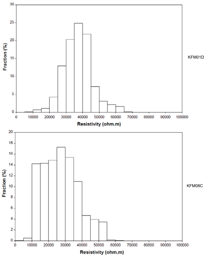
Figure 3-2. Upper and lower images show histograms of the saturated in situ rock matrix resistivities of KFM01D and KFM08C, respectively. Reproduced from Löfgren (2007, Figures 4-2 and 4-4).
