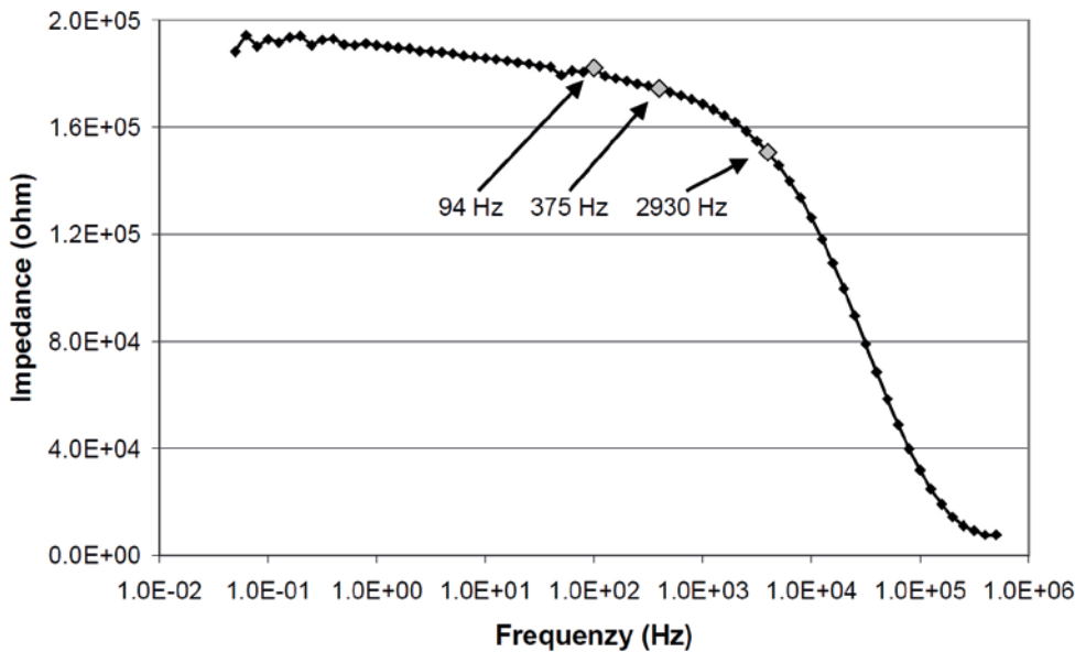
Figure 5-8. Impedance spectroscopy of Laxemar sample leached in deionised water. Reproduced from Löfgren (2001, Figure A5-15).
