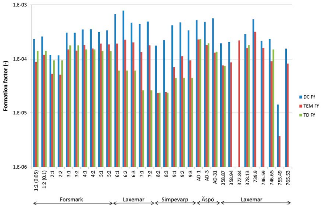
Figure 6-2. Formation factors obtained by the through-electromigration method, using the anionic tracer iodide, the through-diffusion (TD) method using HTO as the tracer, and the DC rock resistivity method. Data are based on Löfgren (2004), Löfgren and Neretnieks (2006), Löfgren et al. (2009) and Vecernik et al. (2012). Sample labelling is explained in Appendix C.
