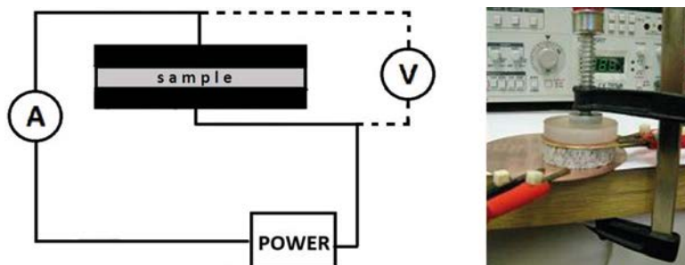
Figure 3-7. The dry rock resistivity of the cylindrical drill core sample is measured by directly pressing copper electrodes to its end surfaces, connected to an AC/DC power supply providing constant potential drop, and an Ampere-meter. Images by P. Večerník.
