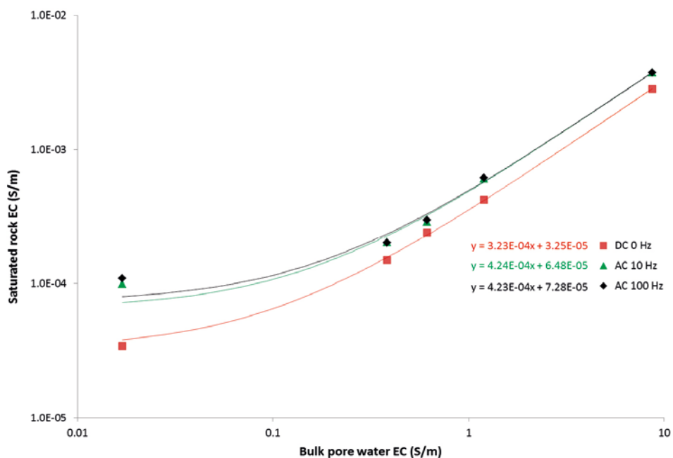
Figure 5-11. Saturated rock ECs of Sample 1 from Forsmark (cf. Table 4-1) at different frequencies, as saturated by pore water solutions of different EC. The fittings correspond to Equation 4-4.
