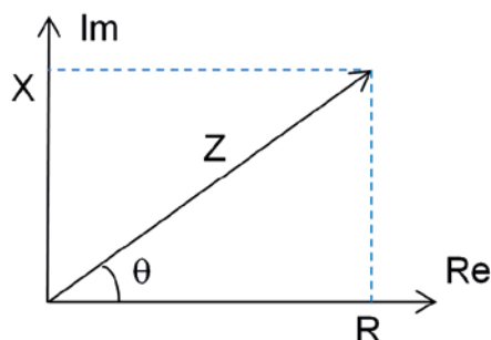
Figure 5-4. The relations between impedance Z , resistance R , reactance X , and phase angle \theta .
