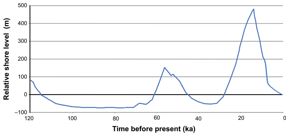
Figure 3-20. Reconstructed shore-level displacement at Forsmark for the last glacial cycle using GIA modelling (Section 2.2.4) and Holocene data (Påsse 2001). Positive values mean that the area is submerged under the contemporary level of the Baltic Sea. Note that during periods of maximum isostatic depression, the area is situated under the ice sheet.
