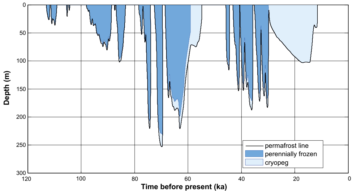
Figure 3-18. Evolution of permafrost and perennially frozen ground depth for the reconstruction of last glacial cycle conditions in Forsmark (spent nuclear fuel repository site). The results were obtained using a 1D permafrost model (Section 2.1.4). Due to the high sub-glacial pressure, a thick unfrozen cryopeg exists within the permafrost (defined by the 0°C isotherm) after 60 ka and after 30 ka before present (including the LGM). For the corresponding 2D modelling results see Figure 3-69 in SKB (2010a).
