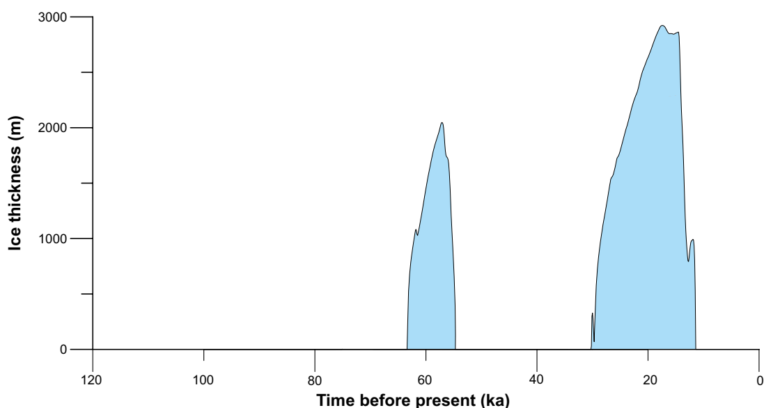
Figure 3-21. Reconstructed ice-sheet thickness over Forsmark for the last glacial cycle (Section 2.3.4).
