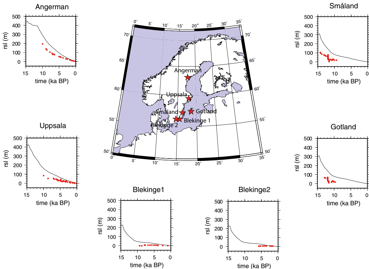
Figure 2-20. Comparison between predicted relative sea-level (black lines) from the GIA model, using the ice loading from the Weichselian glacial cycle (model 1 in Table 2-4), and observations from relative sea-level markers (red points) at six sites in Fennoscandia (red stars) for the last 15 ka. Data compiled from Lambeck et al. (1998).
