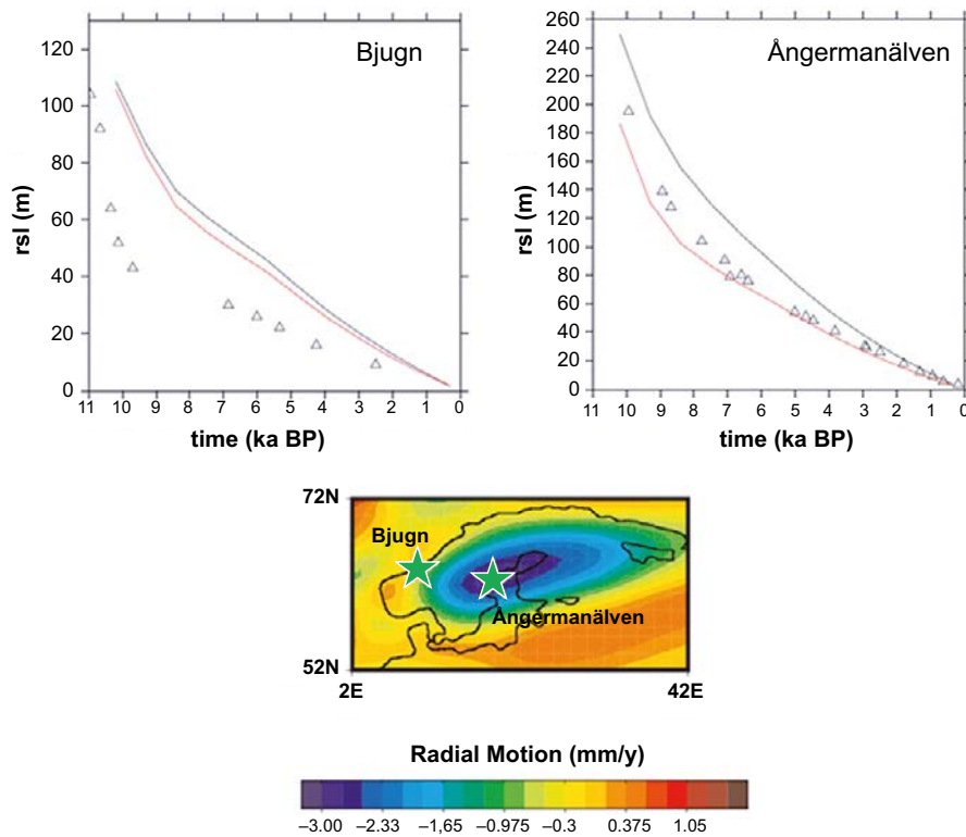
Figure 2-35. Top left: Predicted relative sea-level history at Bjugn for the last 10 ka. Black line: 1D model. Red line: 3D model. Top right: Predicted relative sea-level history at Ångermanälven for the last 10 ka. Line colours are as for Bjugn. Relative sea-level data are shown as triangles; see Lambeck et al. (1998) for references. Bottom plot: Location map for Bjugn and Ångermanälven overlaid upon the misfit in uplift rates (as for Figure 2-32a).
