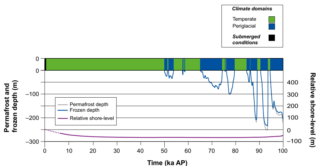
Figure 4-3. Evolution of climate-related conditions at Forsmark as a time series of climate domains and submerged periods for the global warming climate case .
