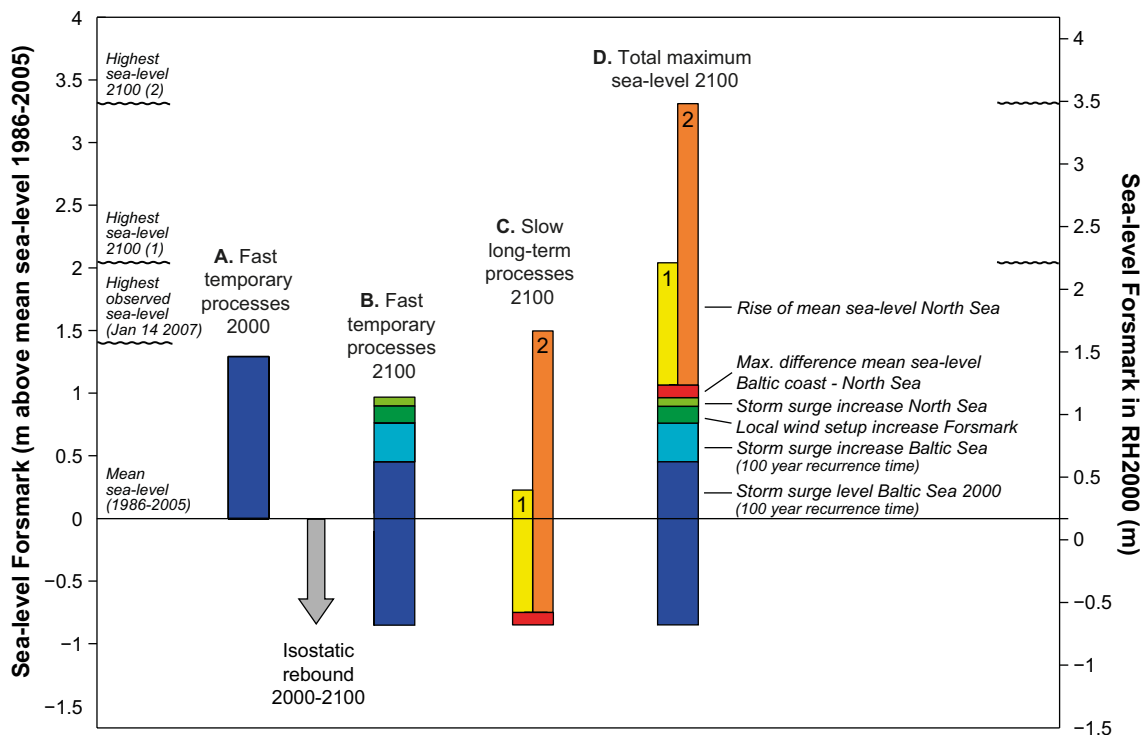
Figure 3-23. Estimated maximum possible sea level at Forsmark at 2100 AD (from Table 3-2). A: present day maximum sea-level rise due to fast temporary processes (e.g. storm surges), B: maximum sea-level rise in 2100 AD due to fast temporary processes, in part compensated for by isostatic rebound, C: sea-level rise at 2100 AD due to slow long-term processes, i.e. rise of mean sea level. (1: process-based projections (IPCC 2013), 2: from other methods (Srifer et al. 2012)), D: total maximum sea-level rise in the year 2100 when considering both the fast temporary processes and the slow long-term processes. The C2 value of Srifer et al. (2012) represents the upper, worst-case, value in a range of values estimated by non-process based models, e.g. semi-empirical models and kinematic constraints on ice-sheet melting. The isostatic rebound for the period 2000 to 2100 AD at the Forsmark site (0.84 m) compensates for a significant portion of the sea-level rise. The sea level is given in m above the present day mean sea level for the period 1986-2005 (corresponding to +0.19 m in RH2000) and in RH2000.
