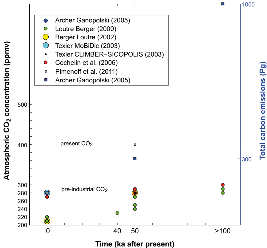
Figure 3-30. Approximate timing of glacial inception versus atmospheric CO 2 concentration in the studies summarised in Table 3-8 (circles and asterisk) and an approximate timing of glacial inception versus total carbon emissions (squares).
