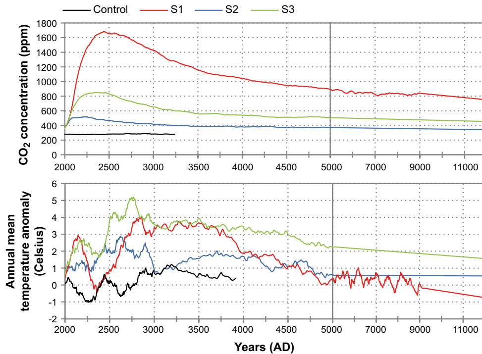
Figure 3-29. Evolution of the atmospheric CO 2 concentration (upper panel) and the annual mean temperature relative to Rauma Kuuskajaskari during 1961–1990 (4.8°C) (lower panel). Note the non-constant scale of the x-axis. Modified from Figure 15 of Pimenoff et al. (2012).
