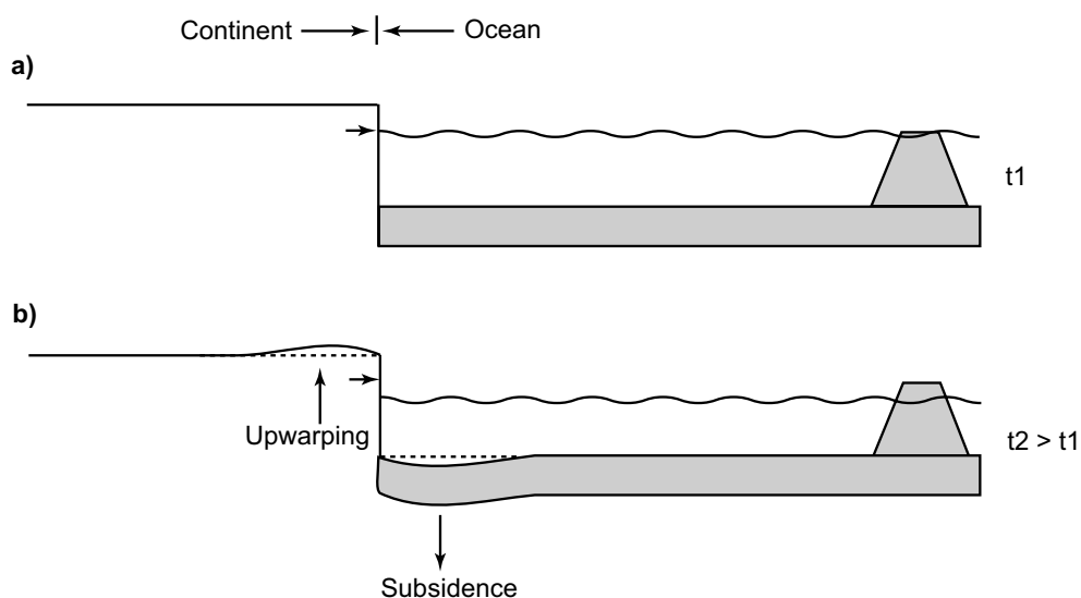
Figure 2-14. Continental levering: the migration of water into offshore regions following deglaciation results in offshore subsidence and onshore upwarping. Ocean floor subsidence results in sea-level fall at far-field sites.
