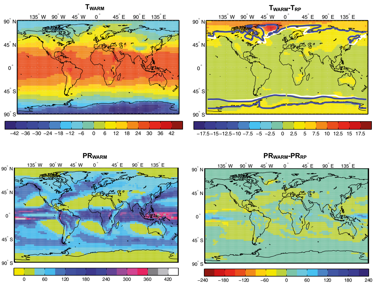
Figure 3-31. Upper panels: Simulated near-surface air temperature in the global warming simulation ( T_{WARM} ) and the difference compared with the simulated present climate ( T_{RP} ) (1961–2000). Units are °C. Also shown by isolines in the rightmost panels is the extent of sea-ice in the simulation of the present climate (white) and in the global warming simulation (blue). Lower panels: Precipitation in the global warming simulation ( PR_{WARM} ) and the difference compared with the simulated present climate ( PR_{RP} ). Units are mm/month. From Kjellström et al. (2009).
