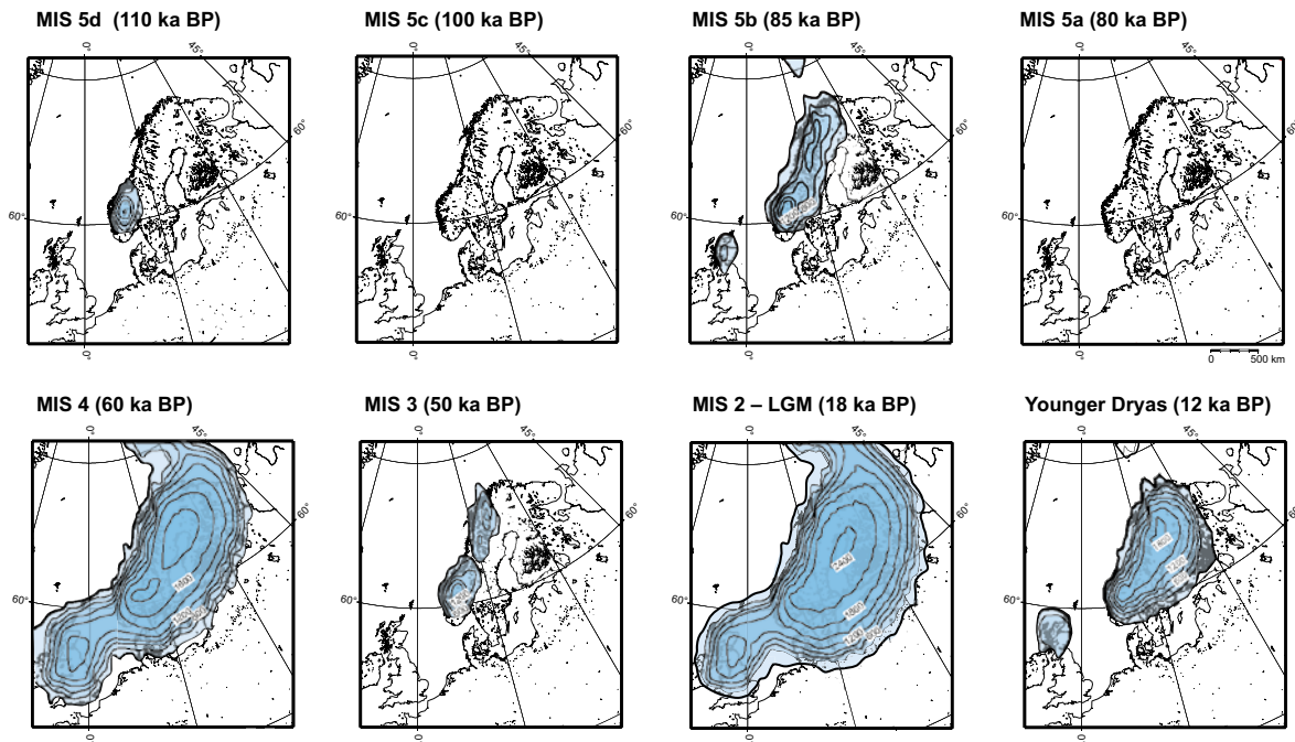
Figure 2-52. Selected maps of ice-sheet surface topography for the reconstructed Weichselian ice sheet. The ice sheet grows to its full LGM configuration in progressive phases of increasing maximum extent, with intervening periods of more restricted ice coverage. Contour lines show ice-surface elevation with a 300 m contour interval. All maps show present-day shoreline position.
