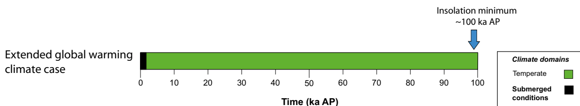
Figure 4-7. Evolution of climate-related conditions at Forsmark as a time series of climate domains and submerged periods for the extended global warming climate case.
