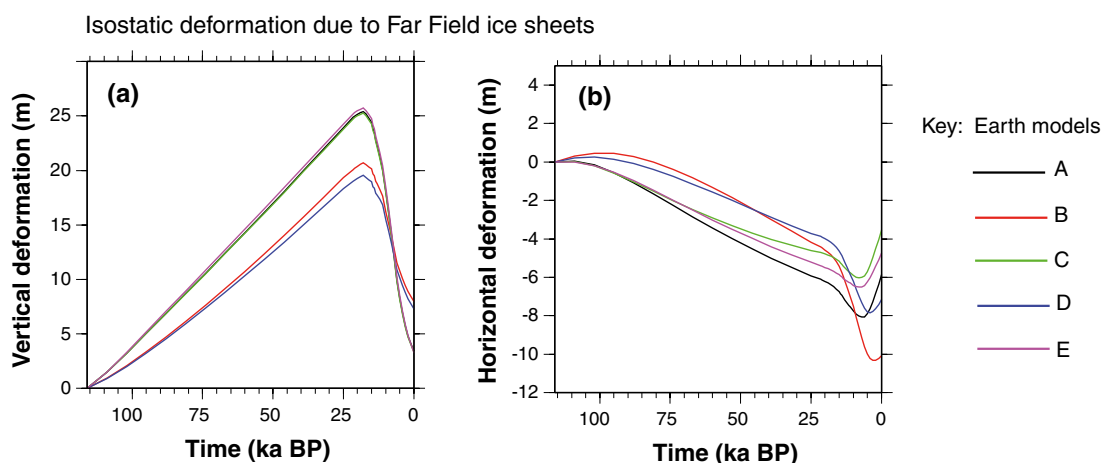
Figure 2-28. Solid surface deformation at Forsmark due to far-field ice loading. See Table 2-5 for a description of the Earth models used. a) vertical deformation, b) horizontal deformation.
