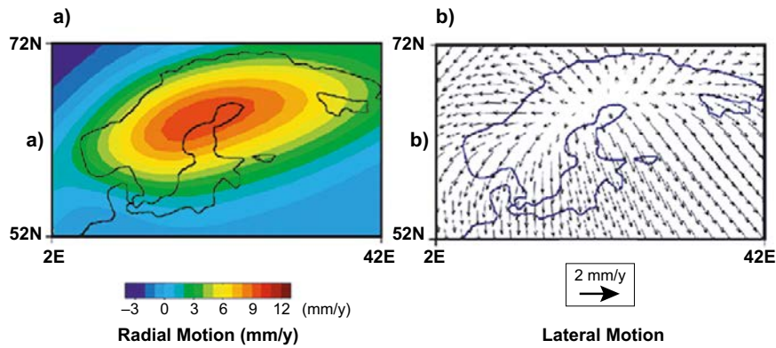
Figure 2-31. Predicted present-day uplift rates (a) and tangential rates (b) generated using the best-fitting 1D Earth model for Fennoscandia and the ice model discussed in the text. Tangential rates are given relative to a point on the north coast of the Gulf of Bothnia.
