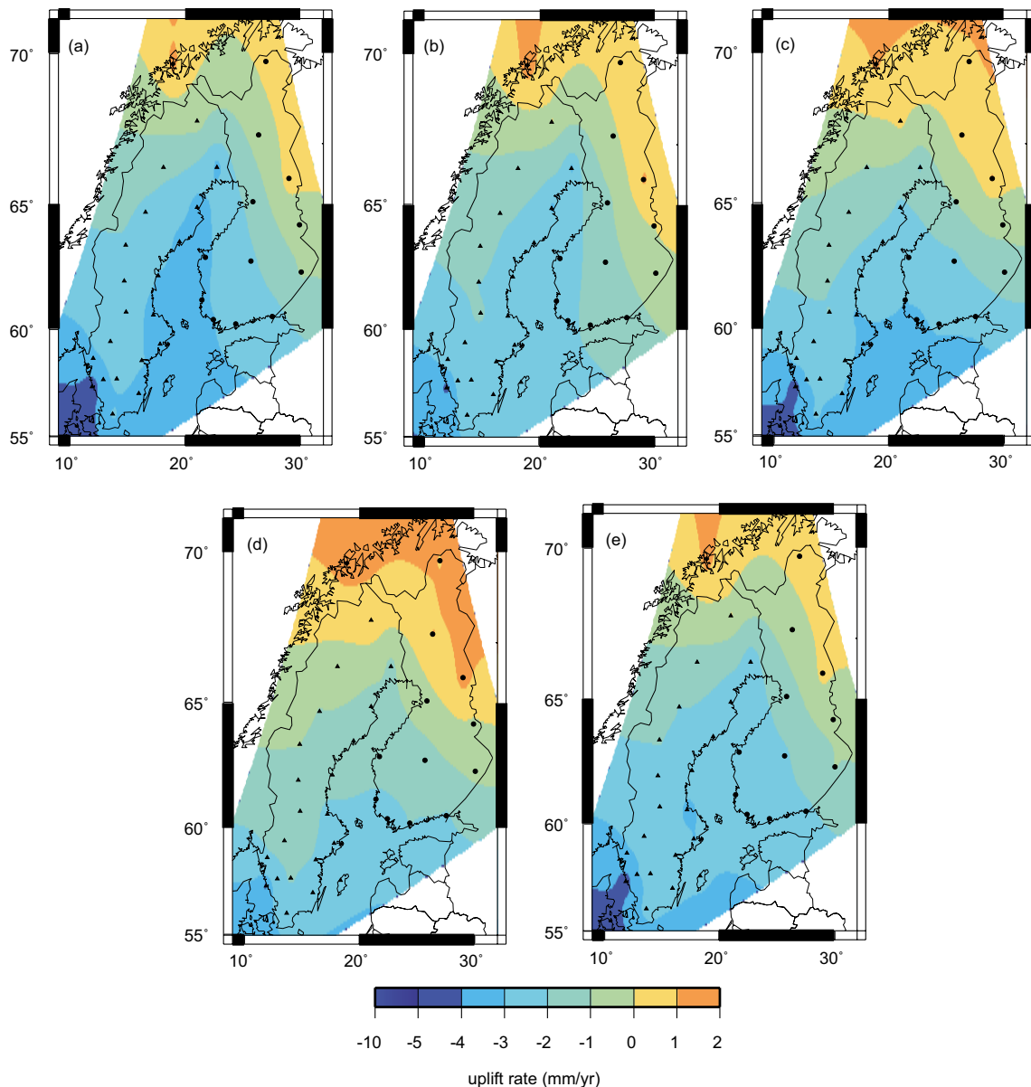
Figure 2-24. Residual present-day uplift rates (misfit between observations and predictions) throughout Fennoscandia for the five Earth models under consideration. The predictions of Figure 2-23 are interpolated at the BIFROST GPS sites and then subtracted from the observed signal (see Figure 2-25). Loading and Earth models as in Figure 2-23.
