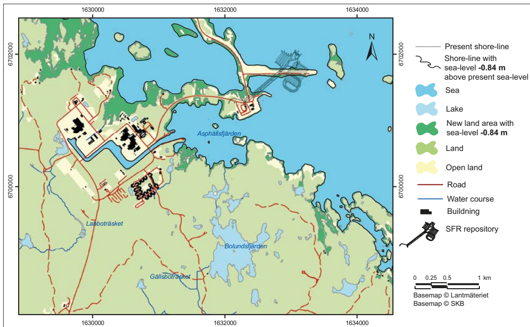
Figure 3-27. Areas at Forsmark which will have emerged from the sea at 2100 AD if the mean sea-level would remain unchanged compared to the present day and only isostatic rebound would influence the shoreline displacement at Forsmark. This map serves to illustrate the lower limit of the uncertainty range for mean sea-level change in Forsmark until 2100 AD. In this case, the sea-level reaches −0.84 m below the present-day mean sea-level (corresponding to −0.65 m in the RH2000 height system) (Table 3-3). The present shore line is based on the Lantmäteriet Property map ( www.lantmateriet.se ). Note that the mean sea level rises by c 1.1 mm/yr at Forsmark at present (see Section 2.2.3), why the assumption of no future mean sea-level rise is unrealistic.
