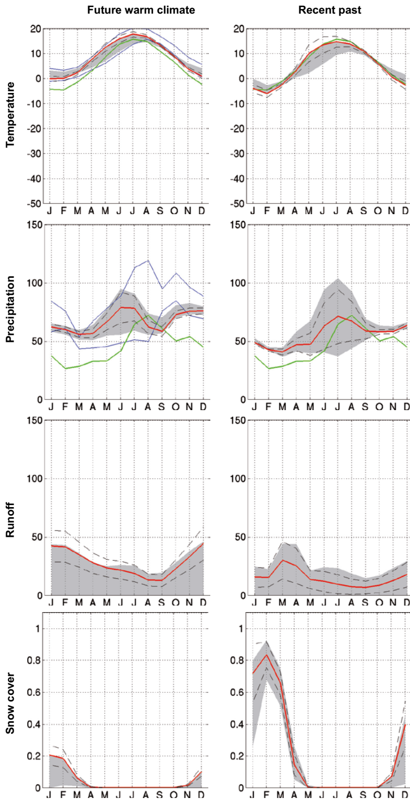
Figure 3-36. Simulated seasonal cycles of temperature ( ^{\circ}\text{C} ), precipitation (mm/month), runoff (mm/month) and snow fraction (dimensionless ranging from 0 to 1) at the grid box closest to the Forsmark site (red line). The spatial variability in the 3 \times 3 -grid (Figure 3-35) is displayed with the dashed lines representing \pm 1 standard deviation calculated from the 9 grid boxes, and the grey area representing the absolute maximum and minimum, of the 9 grid boxes. The green line for temperature and precipitation is the observed seasonal cycle from the CRU data set in the period 1961–1990. In the exemplified future warm climate (left column), an additional uncertainty range defined by \pm 1 standard deviations of the data calculated from the 9 surrounding grid boxes from three additional simulations for the 21st century with RCA3 is shown with blue full lines. From Kjellström et al. (2009).
