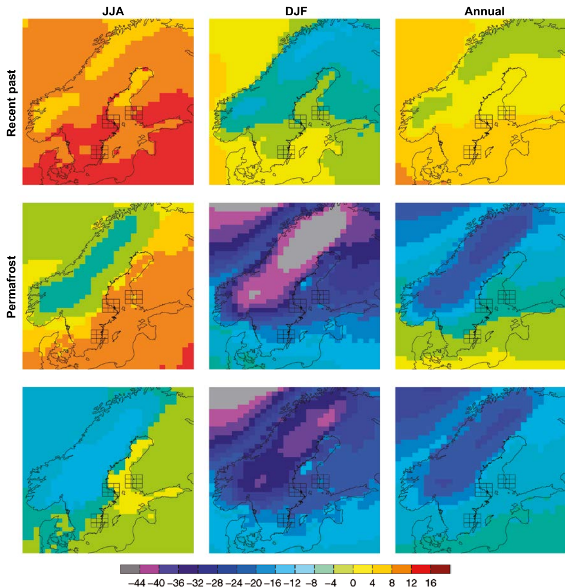
Figure 3-12. Seasonal and annual mean temperature for the present (1961–2000) (upper row) and MIS 3 (middle row) climate simulations. The lower row shows the difference between the two. Units are °C. From Kjellström et al. (2009).
