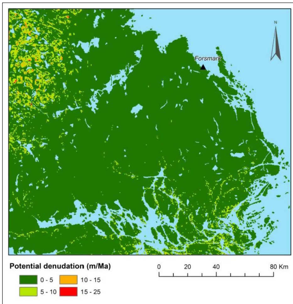
Figure 2-54. Calculated potential future non-glacial denudation in the Forsmark region. At Forsmark, calculated values of the non-glacial denudation component are low, up to 5 m/Ma. From Olvmo (2010).
