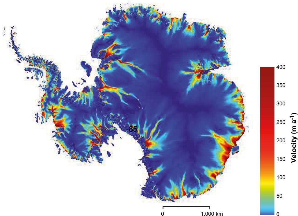
Figure 2-47. Modelled Antarctic ice-surface velocities. Fast-flowing ice streams (red/yellow/green) reach far into the ice-sheet interior. From Johnson (2004) with numerical methods described in Staiger et al. (2005).
