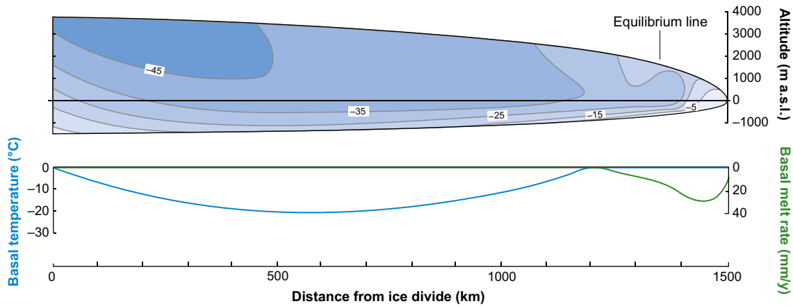
Figure 2-41. Example of modelled ice-sheet temperature distribution along a flow line. Ice temperatures are in °C. Basal melt rates are high near the terminus because of the strain heating effect from rapid ice flow in the region around the equilibrium line. Modified from Hooke (1977).
