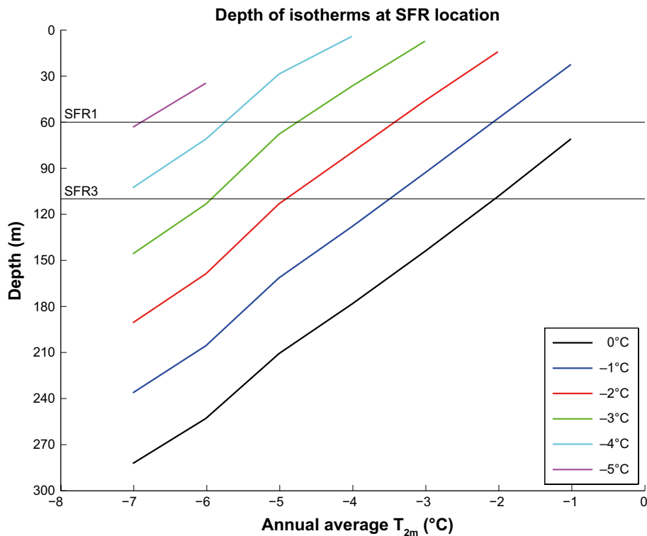
Figure 2-11. Depth (m) of the 0, -1, -2, -3, -4° and -5°C isotherms as a function of the annual average Forsmark T_{2m} . The depths of the existing SFR1 repository (c 60 m) and planned SFR3 repository (c 110 m) are indicated with black lines. The Forsmark annual average T_{2m} was c +5°C in the period 1961–1990 (Johansson et al. 2005).
