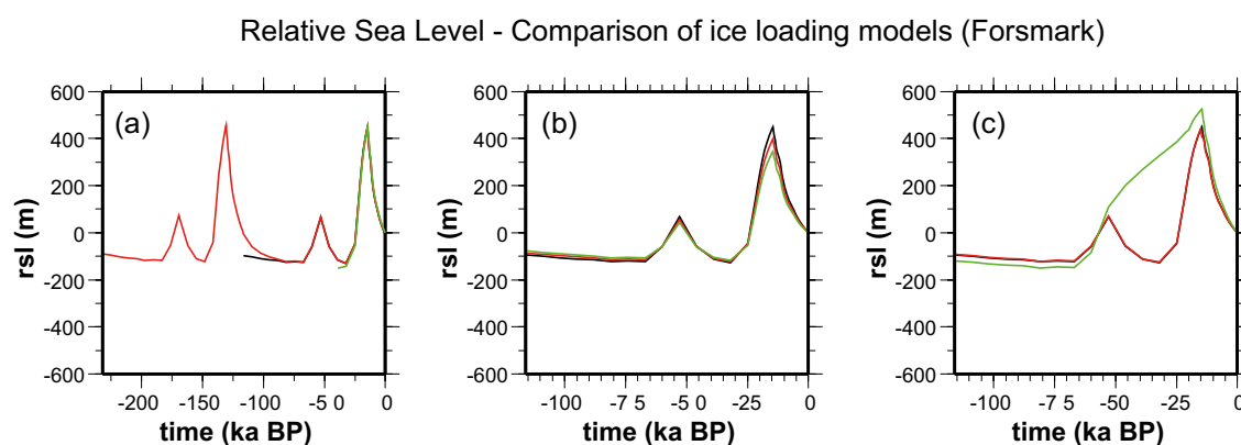
Figure 2-18. Predicted relative sea-level for Forsmark. See Table 2-4 for details of the ice loading models. An Earth model with a thin lithosphere and low upper mantle viscosity has been used in all cases (Model A, Table 2-5). a) black: model 1, red: model 2, green: model 3. b) black: model 1, red: model 4, green: model 5. c) black: model 1, red: model 6, green: model 7.
