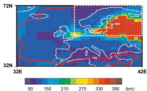
Figure 2-29. Lithospheric thickness derived from the elastic thickness model of Watts (2001) and Pérez-Gussinyé et al. (2004). This is part of a global model where the thicknesses have been scaled to ensure a global mean lithospheric thickness of 120 km. The red lines define plate boundaries. The dashed area is used to define a Fennoscandian regional model studied in Whitehouse (2009) (see text).
