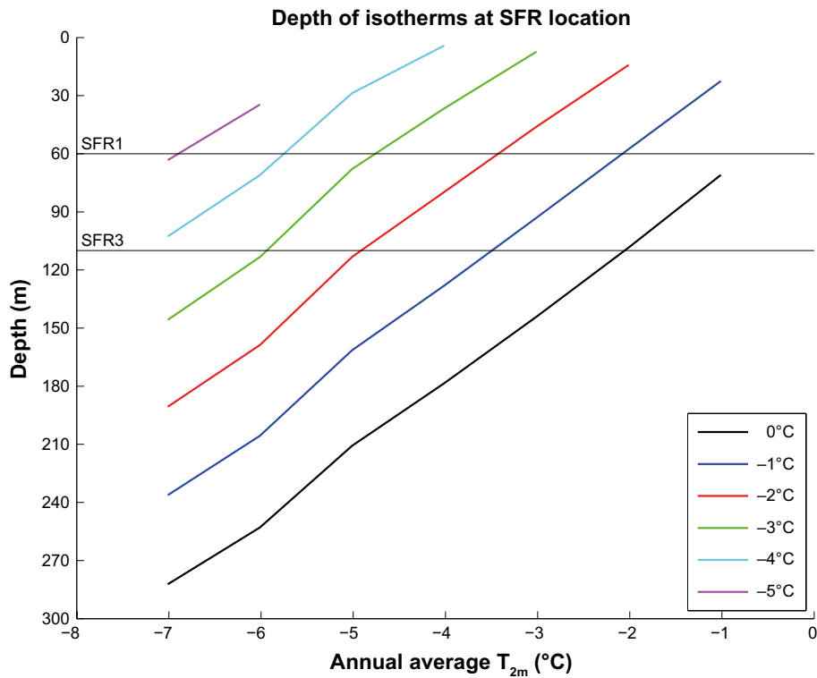
Figure 4-4. Depth (m) of the 0, -1, -2, -3, -4° and -5°C isotherms as a function of the annual average near-surface air temperature ( T_{2m} ) in Forsmark. The depths of the existing SFR1 repository (c 60 m) and planned SFR3 repository (c 110 m) are indicated with black lines.
