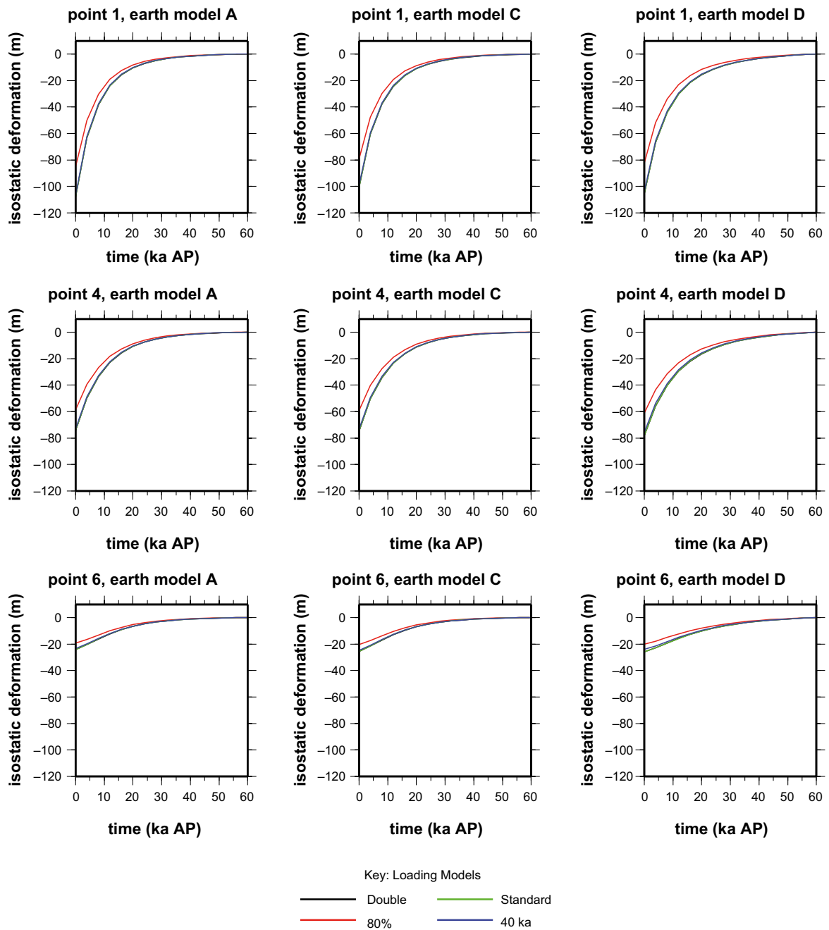
Figure 2-27. Isostatic deformation sensitivity tests. Solid Earth deformation projections between the present day and 60 ka AP at sites 1, 4 and 6 (see Figure 2-25) for the four loading models and three Earth models described in the isostatic recovery sensitivity tests.
