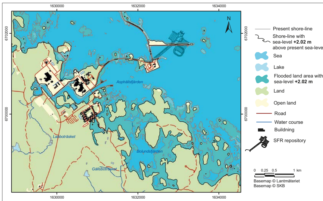
Figure 3-25. Areas at Forsmark which will be temporarily flooded at 2100 AD if the sea-level reaches the maximum possible level of +2.02 m above the present-day mean sea-level (corresponding to +2.21 m in the RH2000 height system). This level represents the sum of the maximum possible mean sea-level rise due to slow long-term processes as projected by process-based methods (+1.07 m; Table 3-3) and the maximum sea-level rise due to fast temporary processes (1.79 m; Table 3-3), compensated for the isostatic rebound (−0.84 m; Table 3-3). The present shore line is based on the Lantmäteriet Property map ( www.lantmateriet.se ). Note that the results describe a situation assuming cumulative worst-case effects of possible future processes spanning the global, regional and local scales, and that the number only applies for occasions of short duration during heavy storms.
