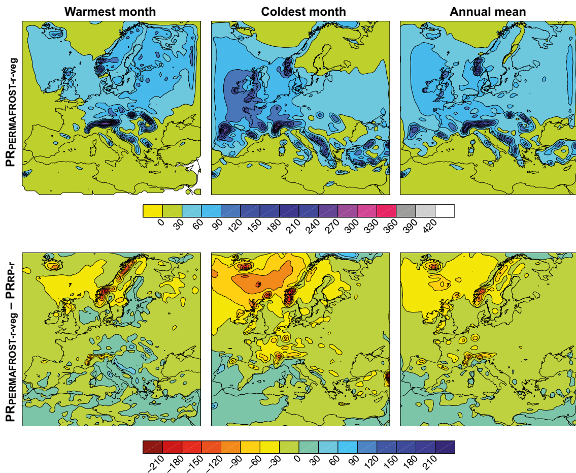
Figure 3-9. Mean precipitation of the warmest month, coldest month and annual mean in the MIS 3 climate simulation (upper row). Also shown are differences between MIS 3 simulation and the simulation of the present (1961–2000) climate. Units are mm/month. From Kjellström et al. (2009).
