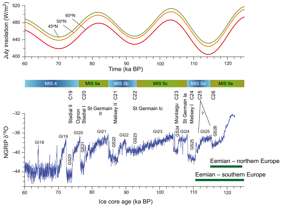
Figure 3-3. Summer insolation at 60°, 50° and 45° N (Berger 1978, Loutre M F, personal communication) compared to the NGRIP \delta^{18}O record (NorthGRIP community members 2004). The North Atlantic sea surface cooling episodes (C26 to C19) and the terrestrial vegetation zones are according to Sánchez Goñi (2007). The correlation between marine and terrestrial events and the NGRIP record was inferred from Figure 13.1 in Sánchez Goñi (2007). The correlation between marine isotope stages (MIS 5e–4) and the NGRIP isotope record is tentative and partly follows Sánchez Goñi (2007) and partly Chapman and Shackleton (1999). The end of the terrestrial Eemian is according to Müller and Kukla (2004) and Sánchez Goñi (2007). GS = Greenland stadials; GI = Greenland interstadials. Note that the correlation of C25 and C26 to Greenland stadials is not entirely clear. C26 likely corresponds to GS26. From Wohlfarth (2013).
