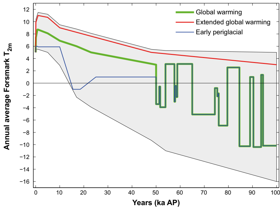
Figure 4-1. Generalised time evolution of annual average near-surface temperature (°C) in Forsmark in the first three climate cases, i.e. global warming, early periglacial and extended global warming climate cases. The grey shading indicates the uncertainty interval for the climate evolution in the next 100 ka. A motivation for the temperature evolution for each case is given in the respective Sections (4.1, 4.2 and 4.3).
