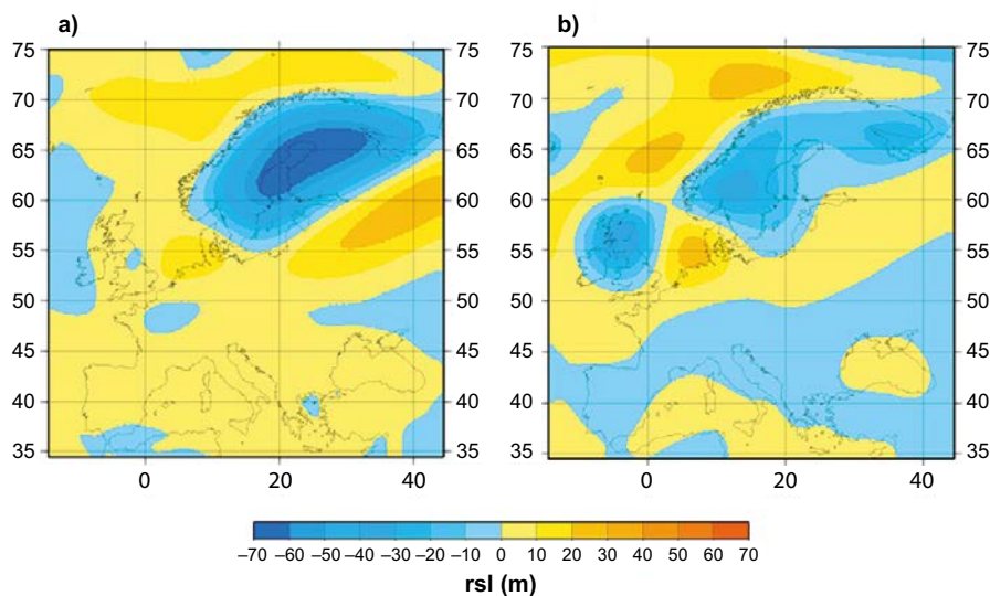
Figure 2-34. Difference in relative sea-level predictions at 10 ka BP. (a) 3D model minus 1D model. (b) 3D model minus 'regional' 1D model (see text).
