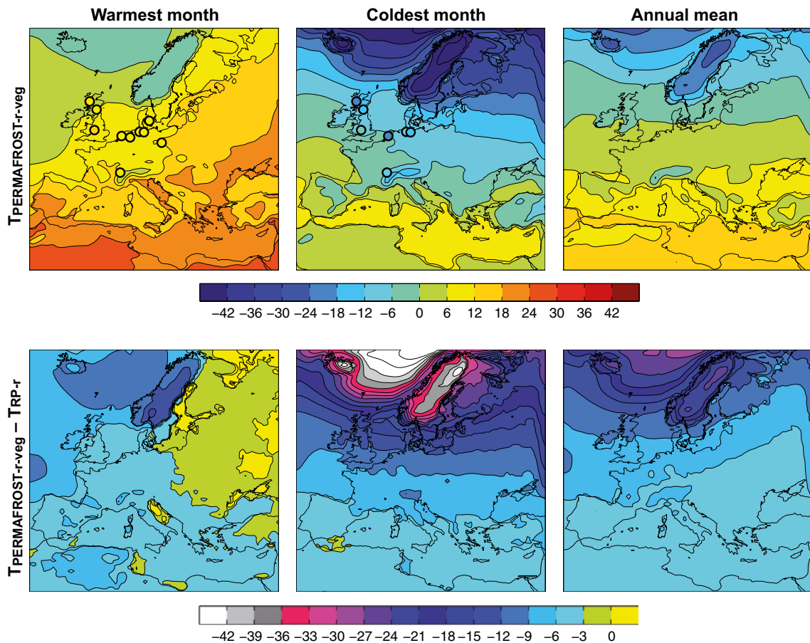
Figure 3-7. Mean air temperatures of the warmest month, coldest month and annual mean in the MIS 3 simulation (top). Shown also are temperature estimates based on proxy data as described in Kjellström et al. (2009, Section 2.4) (coloured circles). The lower row shows the differences between the simulated MIS 3 climate and a recent-past climate simulated for the period 1961–2000. From Kjellström et al. (2009).
