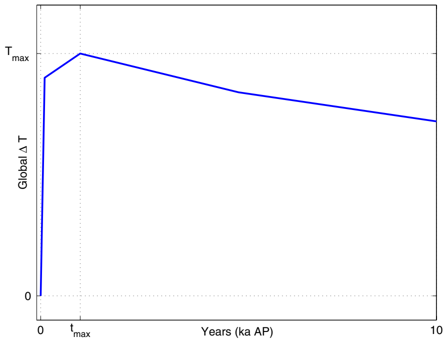
Figure 3-28. Generalised evolution of the global annual average surface air temperature displayed as the anomaly with respect to the year 2000 AD ( \Delta T ). T_{max} is the maximum increase, which occurs at t_{max} ka AP.
