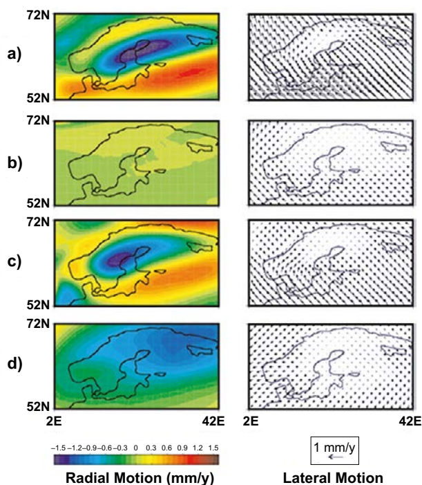
Figure 2-33. (a) Misfit due to lateral variations in lithospheric thickness. (b) Misfit due to the inclusion of weak plate boundary zones. (c) Misfit due to lateral variations in upper mantle viscosity. (d) Misfit due to lateral variations in lower mantle viscosity. Left column: difference in uplift rates. Right column: difference in horizontal rates. All plots show 3D predictions minus 1D predictions.
