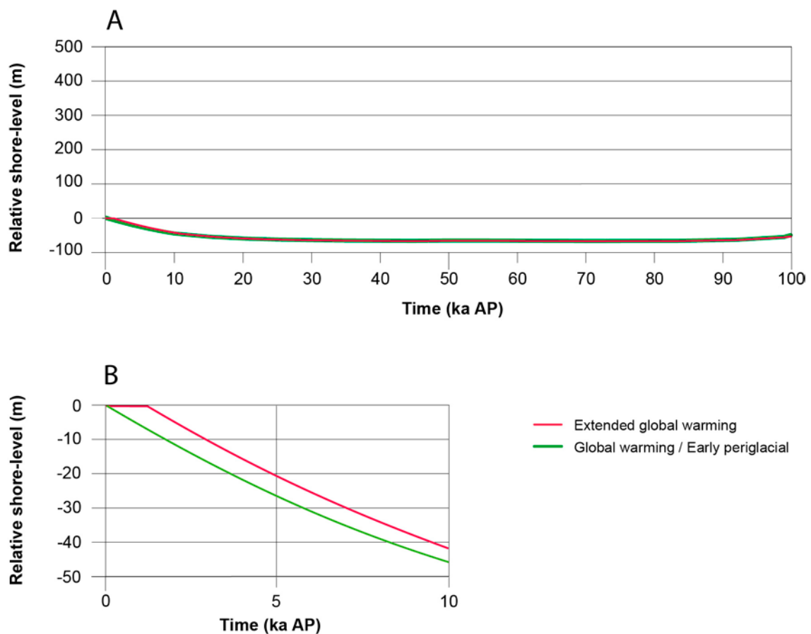
Figure 4-6. Shore-level evolution data from the present (A.) to 100,000 years after present and (B.) to 10,000 years after present for the global warming and early periglacial climate cases (green line) and the extended global warming climate case (red line).
