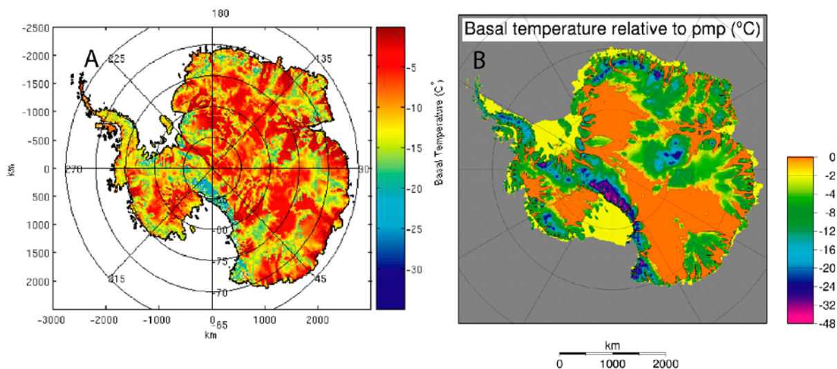
Figure 2-46. Two examples of modelled present-day Antarctic ice sheet basal temperatures. Temperatures are expressed relative to the pressure melting point (pmp). Figure a) is from Johnson (2004) and b) from Huybrechts (2006).
