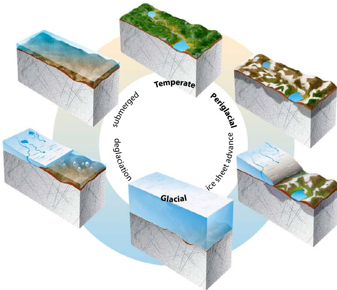
Figure I-3. Simplified glacial cycle constructed from the climate domains (bold text) relevant for assessments of long-term repository safety at Forsmark. In addition to the climate domains, the illustration also depicts a terrestrial glacial advance and a marine deglaciation with subsequent submerged conditions (regular text), in line with the last glacial phase at the Forsmark site. Modified from Selroos et al. (2013).
