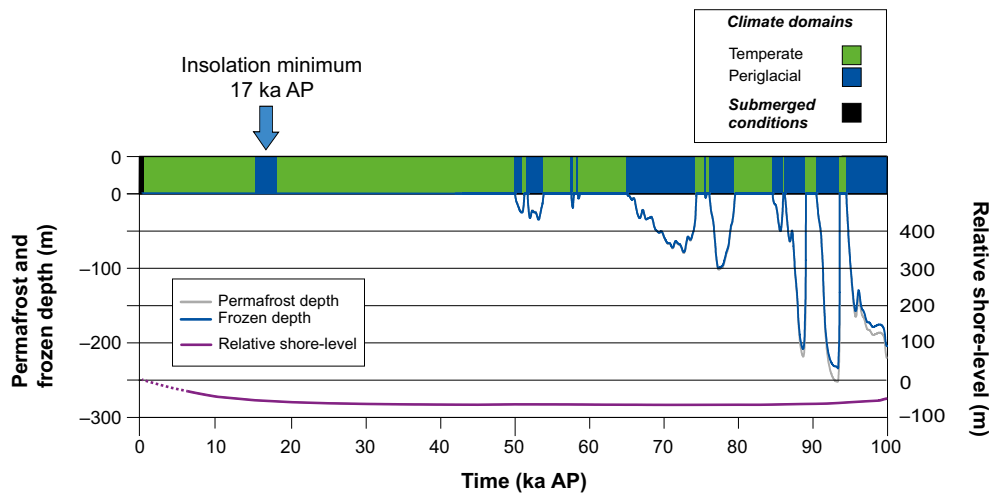
Figure 4-5. Evolution of climate-related conditions at Forsmark as a time series of climate domains and submerged periods for the early periglacial climate case. Note that permafrost and frozen ground evolution is not shown for the period 0 to 50 ka AP. Permafrost and frozen ground can however not be excluded to a depth of about 150 m for the periglacial period from 15.5 to 18.5 ka AP (see Section 4.2.4).
