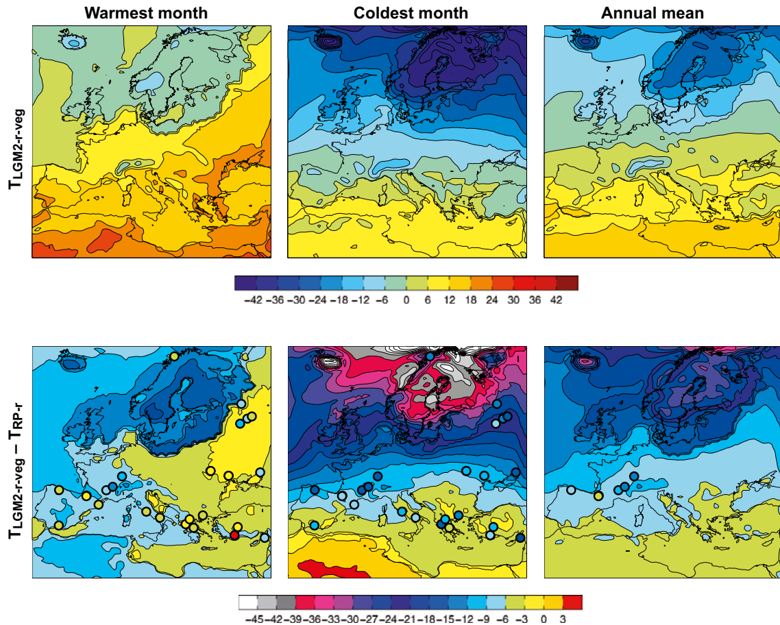
Figure 3-16. Mean temperatures of the warmest and coldest month and annual mean for the LGM simulation (denoted LGM2-r-veg) (upper row). Also shown are differences between the LGM simulation and the simulation of the present climate (years 1961–2000) (denoted RP-r) (lower row). Climate proxy based temperature reconstructions are denoted in the filled circles. Units are °C. From Kjellström et al. (2009).
