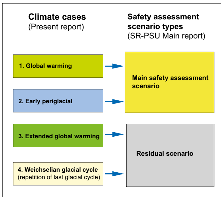
Figure I-4. Relationship between the climate cases identified and described in the present report for the SR-PSU assessment, and the associated safety assessment scenario types analysed in the SR-PSU main report (SKB 2014a).
