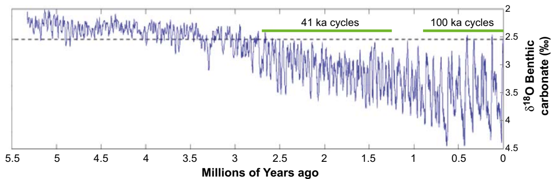
Figure 1-2. Variations of \delta^{18}\text{O} in deep-sea sediments over the last 5.5 Ma (Lisiecki and Raymo 2005). High \delta^{18}\text{O} values indicate large global ice volume and low sea water temperature, i.e. colder climate conditions, whereas low \delta^{18}\text{O} values indicate the opposite. The last 900 ka have been dominated by 100 ka long glacial cycles. Modified from Global Warming Art (2007), after Lisiecki and Raymo (2005).
