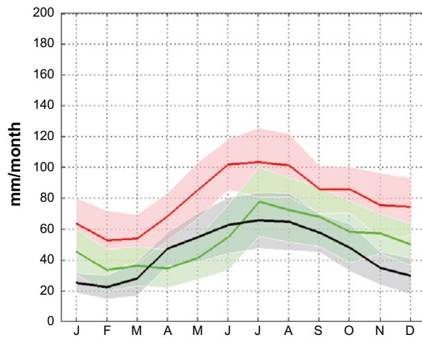
Figure 3-10. Annual precipitation range in Sweden in the MIS 3 simulation (black), present climate simulation (1961–2000) (red) and according to the CRU observational data (green). Shaded areas in corresponding colours indicate the \pm 1 standard deviation range of individual monthly averages in the three data sets. From Kjellström et al. (2009).
