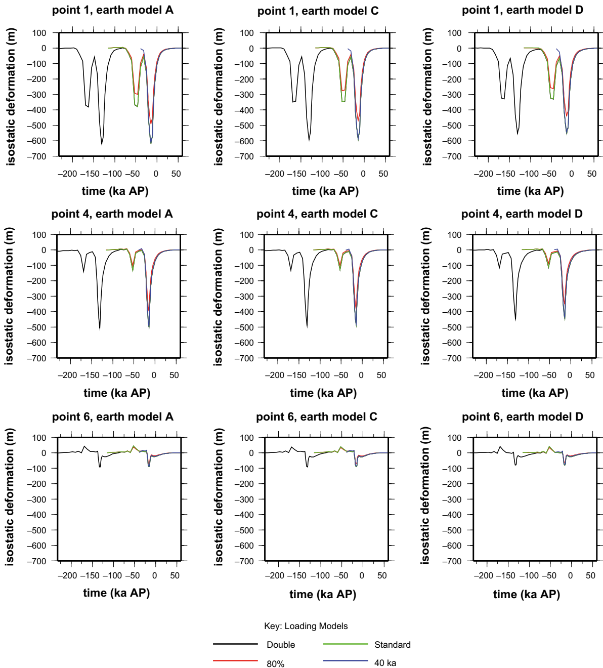
Figure 2-26. Isostatic deformation sensitivity tests. Solid Earth deformation at sites 1, 4 and 6 (see Figure 2-25) for the four loading models and three Earth models described in the isostatic recovery sensitivity tests.
