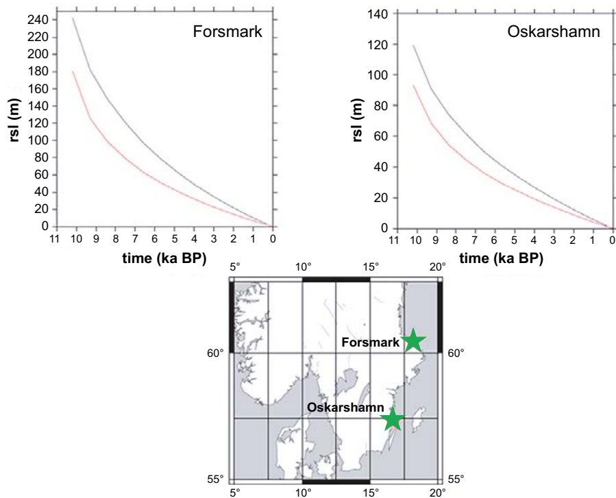
Figure 2-36. Predicted relative sea-level for Forsmark and Oskarshamn calculated using 1D (black line) and 3D (red line) Earth models. Note that both the 1D and 3D GIA simulations used for this plot use another ice load history than the 1D GIA simulations in the previous parts of Section 2.2.4. The results should only be used to exemplify the error introduced by using 1D instead of 3D GIA modelling. At Forsmark, the difference at 10 ka BP is ~60 m.
