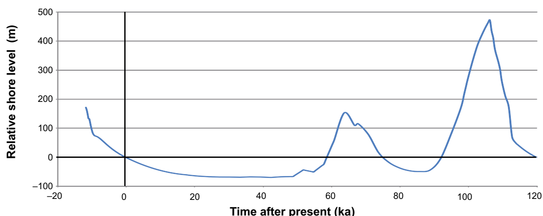
Figure 4-11. Shore-level evolution at Forsmark during the Weichselian glacial cycle climate case . The first c 8 ka of the future period is based on observed relative sea-level data (Påsse 2001) whereas the following part of the time series is constructed from Glacial Isostatic Adjustment modelling (Section 2.2.4). The shore-level is expressed relative to the contemporary Baltic sea-level. Positive numbers indicate that the site is submerged and vice versa. Note that for most of the time when the figure shows submerged conditions, the site is covered by an ice sheet (Figure 4-10). The figure also includes the relative shore-level from the time of deglaciation up to present, used in e.g. the SR-Site biosphere programme.
