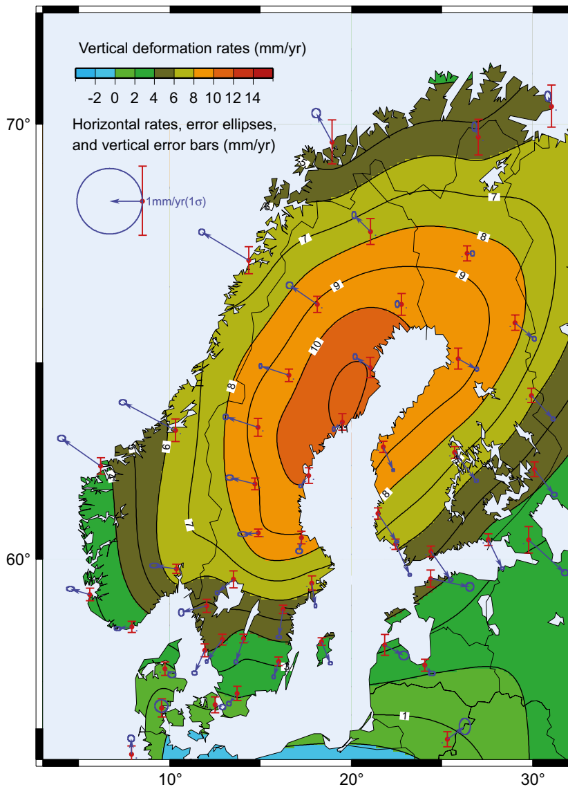
Figure 2-16. Present-day crustal deformation over Fennoscandia as observed by continuous GPS measurements within the BIFROST project (e.g. Scherneck et al. 2001). The rebound displays a concentric pattern with a maximum rebound rate of \sim 11 mm/yr located approximately in the area of the former maximum ice-sheet thickness. In the post-glacial upwarping process, a horizontal component of crustal deformation is also present (blue arrows), directed outward from the area of maximum depression. Modified from Lidberg (2007).
