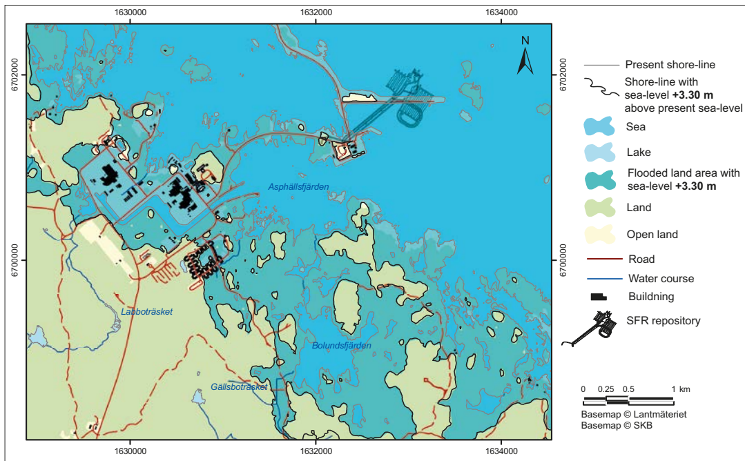
Figure 3-26. Areas at Forsmark which will be temporarily flooded at 2100 AD if the sea-level reaches the maximum possible level of +3.30 m above the present-day mean sea-level (corresponding to +3.49 m in the RH2000 height system). This level represents the sum of the maximum possible mean sea-level rise due to slow long-term processes as projected by non-process based methods (+2.35 m; Table 3-3) and the maximum sea-level rise due to fast temporary processes (1.79 m; Table 3-3), compensated for the isostatic rebound (−0.84 m; Table 3-3). The present shore line is based on the Lantmäteriet Property map ( www.lantmateriet.se ). Note that the results describe a situation assuming cumulative worst-case effects of possible future processes spanning the global, regional and local scales, and that the number only applies for occasions of short duration during heavy storms.
