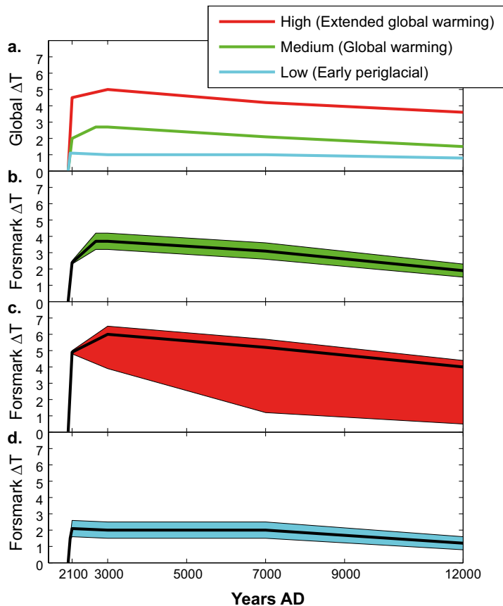
Figure 4-2. Plate (a) shows projected future global annual average near-surface temperature evolution for low (blue), medium (green) and high (red) cumulative carbon emissions. The low, medium and high scenarios correspond to the early periglacial, global warming and extended global warming climate cases respectively. Plate (b) shows the corresponding estimated temperature evolution for the Forsmark region for the global warming climate case (medium emission case), whereas plate (c) and (d) show the corresponding estimated Forsmark temperature evolution for the extended global warming climate case (high emission case) and the early periglacial climate case (low emission case). The temperature is expressed as an increase from the present annual air temperature. The figure also includes the uncertainty interval estimated for each case.
