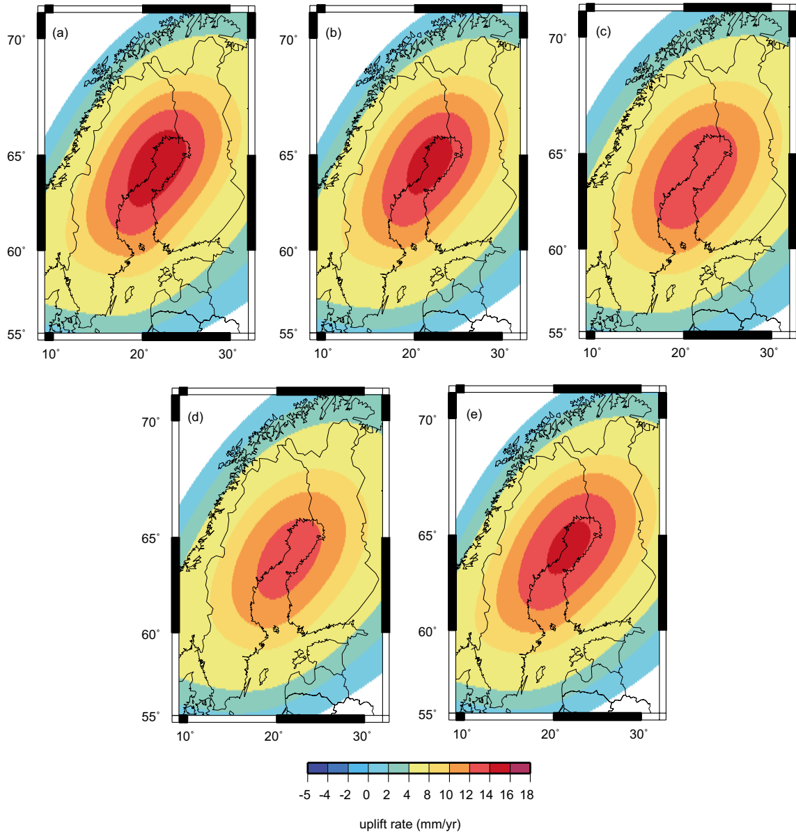
Figure 2-23. Comparison of Earth models. Predicted present-day uplift rates throughout Fennoscandia for the five Earth models under consideration. The loading model is defined to be a single Weichselian glacial cycle (Model 1) in all cases. a) Earth model A. b) Earth model B. c) Earth model C. d) Earth model D. e) Earth model E.
