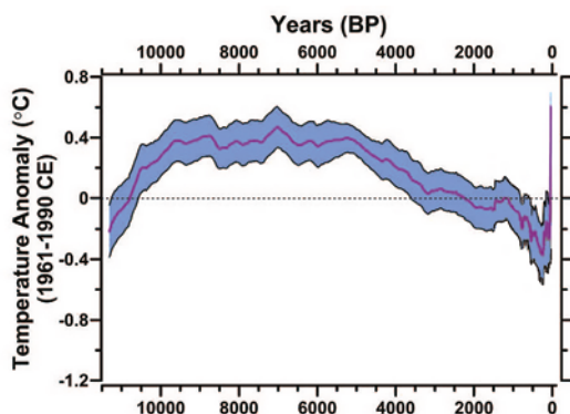
Figure 3-2. Globally stacked surface temperature anomalies with respect to the period 1961–1990 AD (purple line) with one standard deviation uncertainty (blue band). Modified from Marcott et al. (2013).
