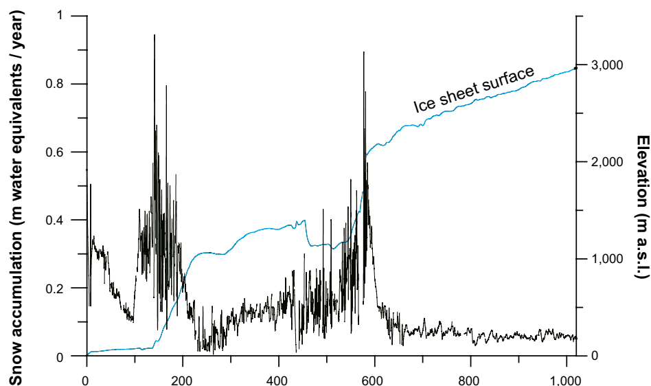
Figure 2-44. Accumulation rates and ice surface elevations along a profile in over the East Antarctic ice sheet. The accumulation is high in the coastal area and low in the interior. Due to wind redistribution of snow, exceptionally high values with strong variations are found in areas of nunataks and steep surface slope. From Richardson (2004).
