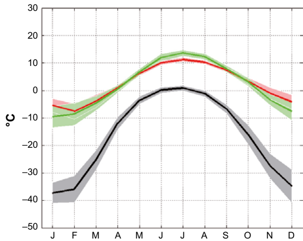
Figure 3-8. Annual temperature range in Sweden for MIS 3 (black), simulated present climate (red) and according to the CRU (Climate Research Unit, East Anglia) observational data for the time period 1961–1990 (green). Shaded areas in corresponding colours indicate the \pm 1 standard deviation range of individual monthly averages in the three data sets. From Kjellström et al. (2009).
