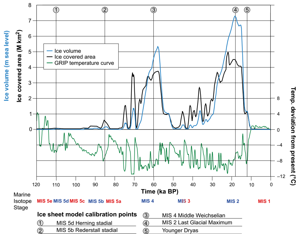
Figure 2-49. GRIP proxy temperature and reconstructed ice-covered area and ice volume for the reconstruction of the Weichselian ice sheet. Times of model calibration are shown, as well as Marine Isotope Stages (MIS) (warm stages in red and cold stages in blue).
