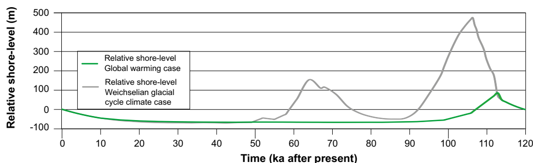
Figure 2-37. Shore-level evolution at Forsmark for a future warm climate. For comparison, the shore-level evolution for the reconstructed last glacial cycle, projected into the future as in the Weichselian glacial cycle climate case, see Section 4.4, is also shown. Negative numbers indicate that the area is situated above the contemporary sea-level. The curve was constructed by GIA modelling combined with results from observations of present-day uplift rates (Pässe 2001). There are significant uncertainties in the future shore-level development, which, in contrast to what is shown in the figure, may result in a sea transgression at Forsmark during the first thousands of years of the evolution.
