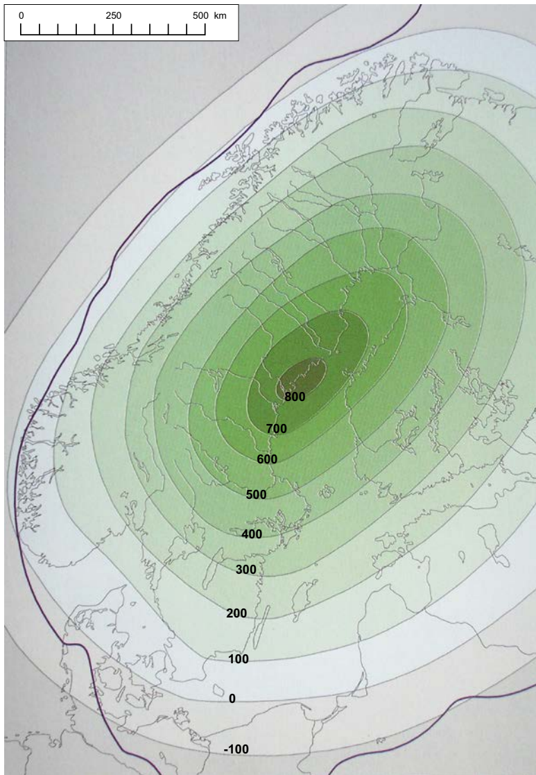
Figure 2-15. Total amount of glacial rebound (metres) that has taken place due to the deglaciation of the Weichselian ice sheet. The bold line shows the approximate maximum extent of the Weichselian ice sheet. Note that the total amount of rebound is more than twice as large as the amount of rebound that may be inferred from raised beaches formed at the highest post-glacial sea-level (see the text). After Fredén (2002).
