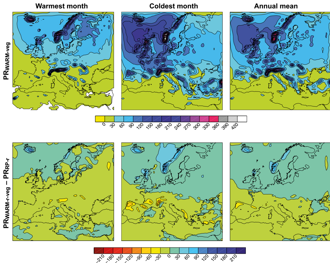
Figure 3-34. Mean precipitation of the warmest month, coldest month and annual mean in the global warming simulation. Also shown are differences between the global warming simulation and the simulated present climate (RP-r) (1961–2000). Units are mm/month. From Kjellström et al. (2009).
