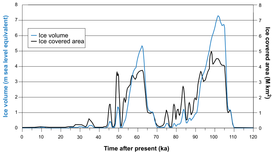
Figure 4-8. Ice sheet volume and ice covered area for the Weichselian glacial cycle climate case.
