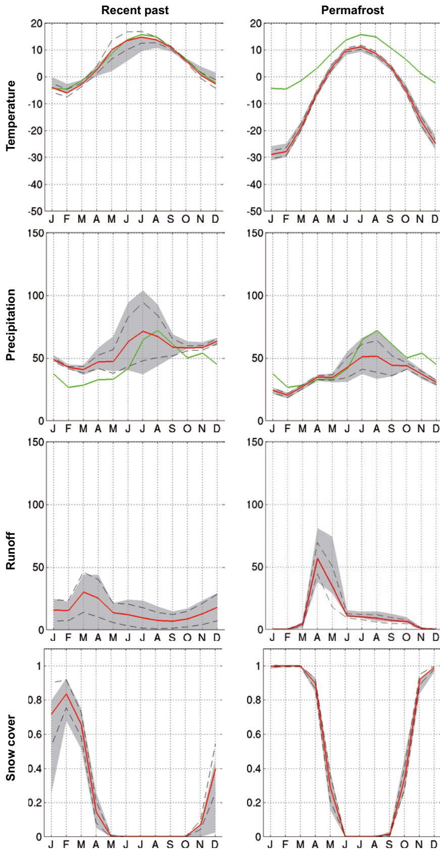
Figure 3-15. Simulated seasonal cycles of temperature (°C), precipitation (mm/month), runoff (mm/month) and snow fraction (dimensionless ranging from 0 to 1) at the grid box closest to the Forsmark site (red line). The spatial variability in the 3 × 3-grids (Figure 4-13) is displayed with the dashed lines representing \pm 1 standard deviation calculated from the 9 grid boxes, and the grey area representing the absolute maximum and minimum, of the 9 grid boxes. The green line for temperature and precipitation is the observed seasonal cycle from the CRU data set for the period 1961–1990, see Kjellström et al. (2009). From Kjellström et al. (2009).
