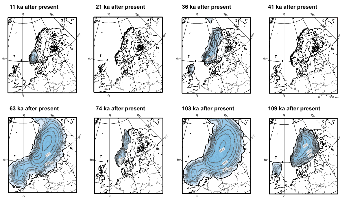
Figure 4-9. Ice-sheet configurations at stadials and interstadials for the Weichselian glacial cycle climate case. Contour lines show ice-surface elevation with a 300 m interval. All maps show present day shoreline position.
