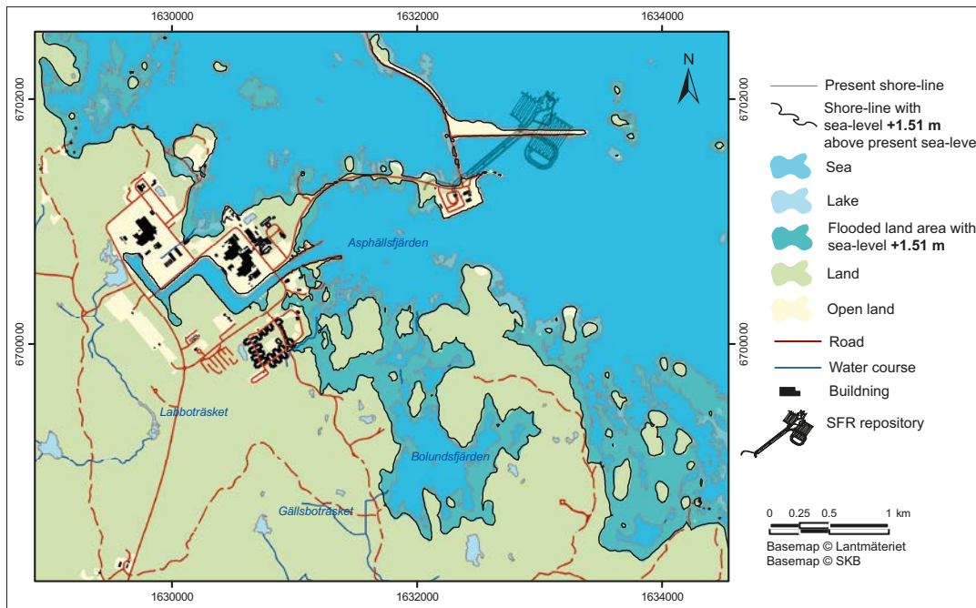
Figure 3-24. Areas at Forsmark which will be permanently flooded at 2100 AD if the sea-level reaches +1.51 m above the present-day mean sea-level (corresponding to +1.70 m in the RH2000 height system). This level represents the maximum possible mean sea-level rise due to slow long-term processes as projected by non-process based methods (+2.35 m; Table 3-3), compensated for the isostatic rebound (−0.84 m; Table 3-3). The present shore line is based on the Lantmäteriet Property map ( www.lantmateriet.se ). Note that the results describe a situation assuming cumulative worst-case effects of possible future processes spanning the global, regional and local scales.
