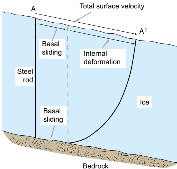
Figure 2-43. Internal deformation and basal sliding demonstrated by the deforming of a steel rod from time A to A'. Modified from Holmlund and Jansson (2003), after Sharp (1960).
