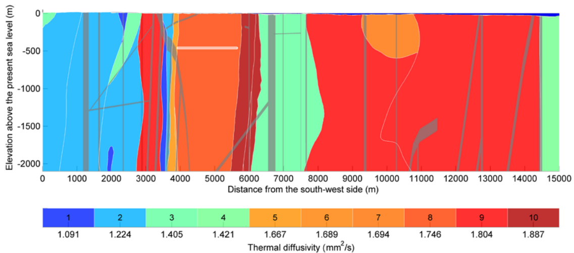
Figure 2-5. The upper 2.1 km of the 2D model domain. Colours from blue to red signify rock domains with different thermal diffusivities. Numbers from 1 to 10 indicate the rock domains of Table 2-2 in Hartikainen et al. (2010). The location of deformation zones is illustrated in grey and the repository for spent nuclear fuel in white, at a depth of 450 m starting at a distance of about 4,000 m along the profile. The thin blue layer on the top surface represents the present-day level of the Baltic Sea. Further description and references for these data are found in Hartikainen et al. (2010, Appendix C).
