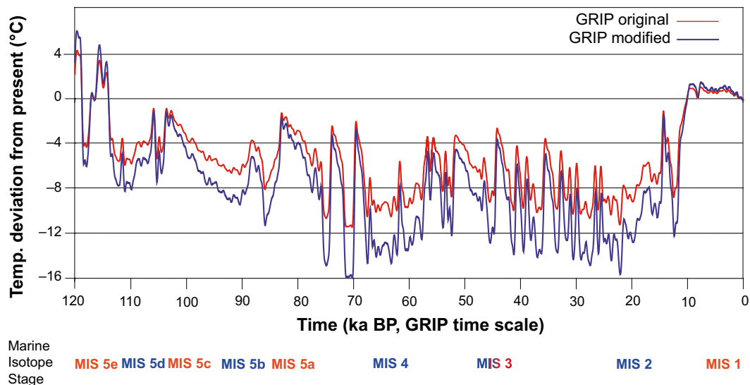
Figure 2-51. Proxy paleo-air temperature from the calibration process of the UMISM ice sheet model. The final calibrated time series used in the ice sheet modelling (blue) has larger amplitude than the original data (red), i.e. cold periods were even colder in the calibrated time series. Modifications of the temperature data set were performed for the complete time series. The temperature time series, and its uncertainties, are discussed in detail in SKB (2010a, Appendix 1).
