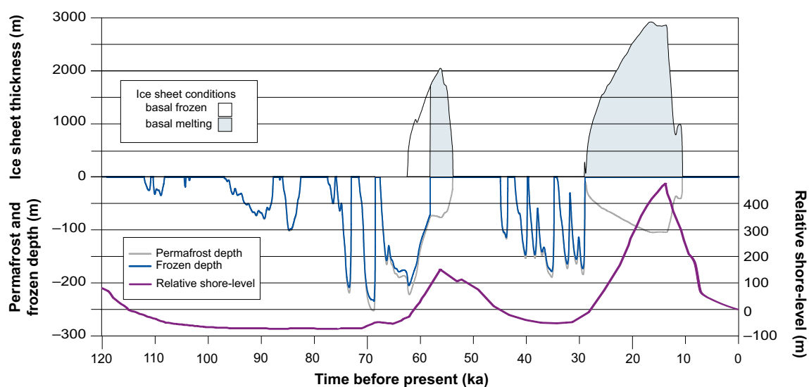
Figure 3-22. Reconstructed Weichselian evolution of ice sheet, shore-level, permafrost and frozen ground at Forsmark. This evolution was repeated and projected into the future in order to construct the SR-PSU Weichselian glacial cycle climate case .
