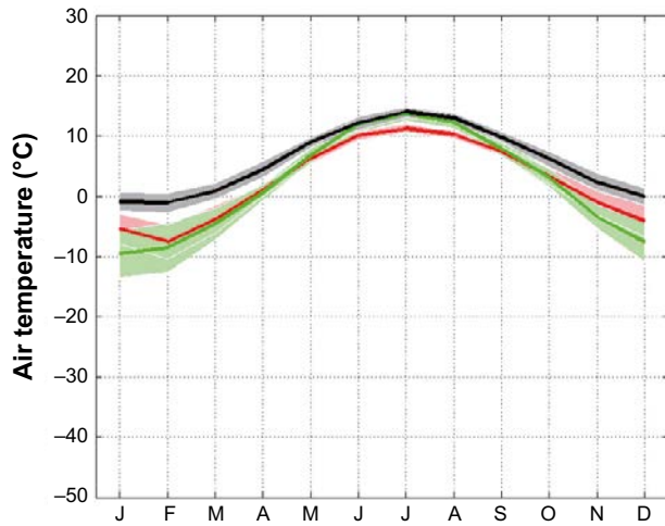
Figure 3-33. Annual cycle of temperature for Sweden in the global warming case (black line) and for the simulated present climate (1961–2000) (red line). Also shown is the CRU observational data from 1961–1990 (green line). Shaded areas in corresponding colours indicate the \pm 1 standard deviation calculated for the range of individual monthly averages in the three data sets. From Kjellström et al. (2009).
