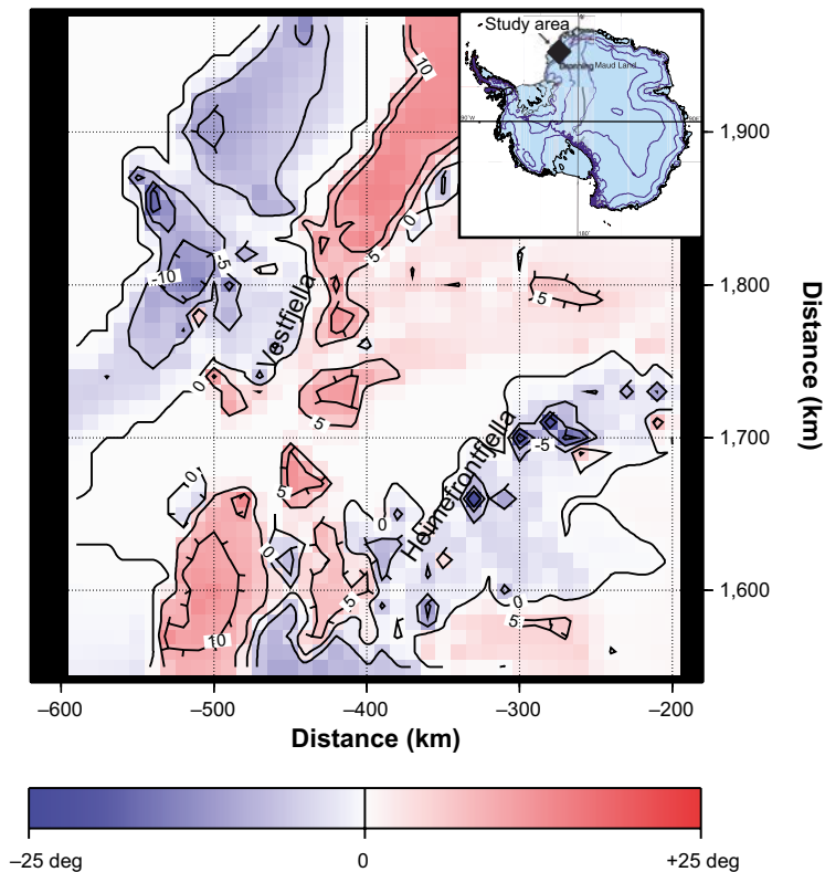
Figure 2-48. Modelled difference in basal temperature between the present-day ice configuration and a maximum Pleistocene ice sheet configuration for part of the Antarctic ice sheet. For this single change in ice configuration, ice-sheet thermodynamics induce complex changes in basal thermal pattern; some parts of the ice sheet become warmer at the bed the same time as other parts become colder. From Näslund et al. (2000).
