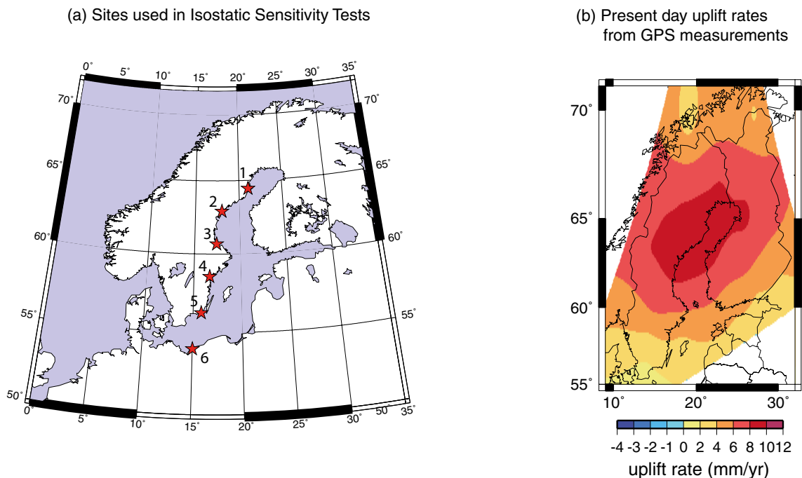
Figure 2-25. a) Map showing the location of the six sites (red stars) where the isostatic response is calculated and b) the present-day pattern of uplift in Fennoscandia from BIFROST GPS rates (Johansson et al. 2002).
