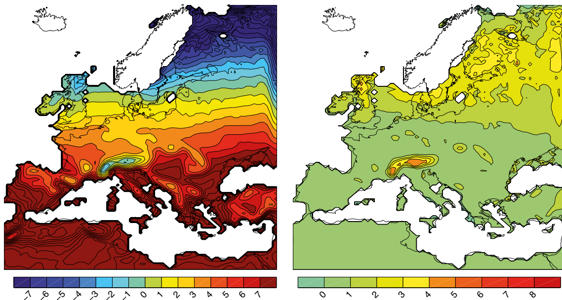
Figure 3-11. Annual mean ground temperature (left) and difference between near-surface air temperature and the ground temperature (right) in the MIS 3 simulation. Units are °C. White areas in Fennoscandia are covered by the prescribed restricted MIS 3 ice sheet. From Kjellström et al. (2009).
