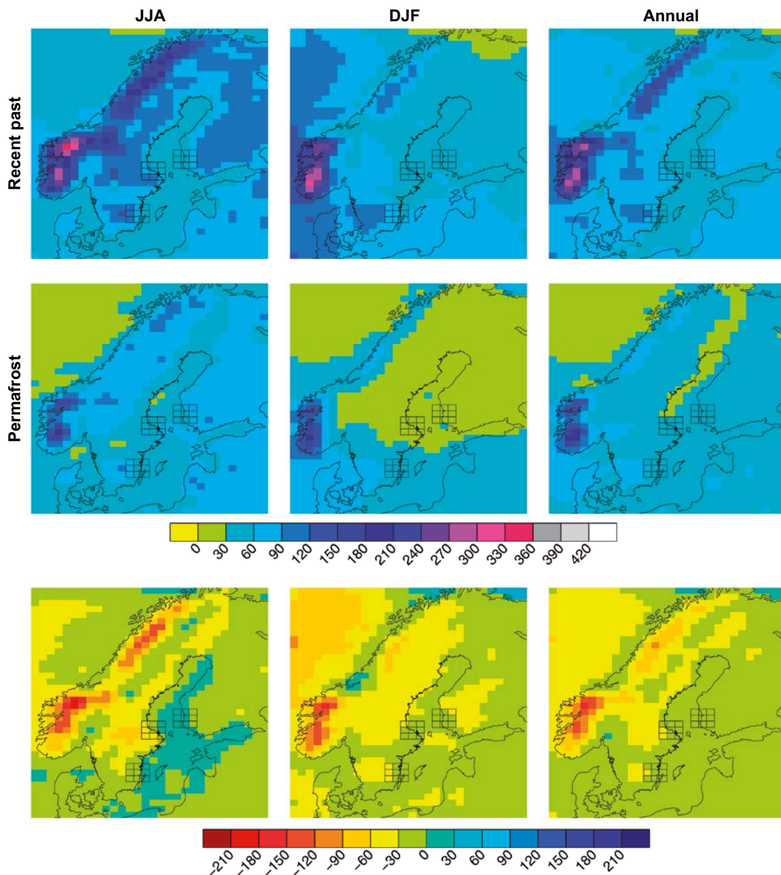
Figure 3-13. Seasonal and annual mean precipitation in the present (1961–2000) (upper row) and MIS 3 (middle row) climate simulation. The lower row shows the difference between the two. Units are mm/month. From Kjellström et al. (2009).
