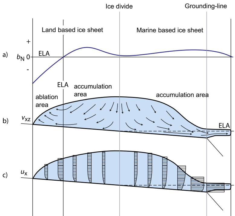
Figure 2-38. Schematic ice sheet cross section. Panel a) shows the surface net balance distribution ( b_N ), panel b) shows ice velocity trajectories ( v_{xz} ) as well as distribution of accumulation- and ablation areas, and panel c) shows the horizontal velocity component ( u_x ). ELA denotes equilibrium line altitude. Modified from Holmlund and Jansson (2003), after Denton and Hughes (1981).
