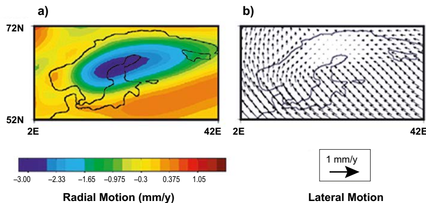
Figure 2-32. Misfit between (a) uplift rates and (b) tangential rates generated using a 3D Earth model and a 1D Earth model. 1D rates are subtracted from 3D rates.
