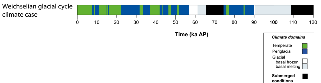
Figure 4-18. Evolution of important climate-related variables at Forsmark for the coming 120 ka in the Weichselian glacial cycle climate case .
