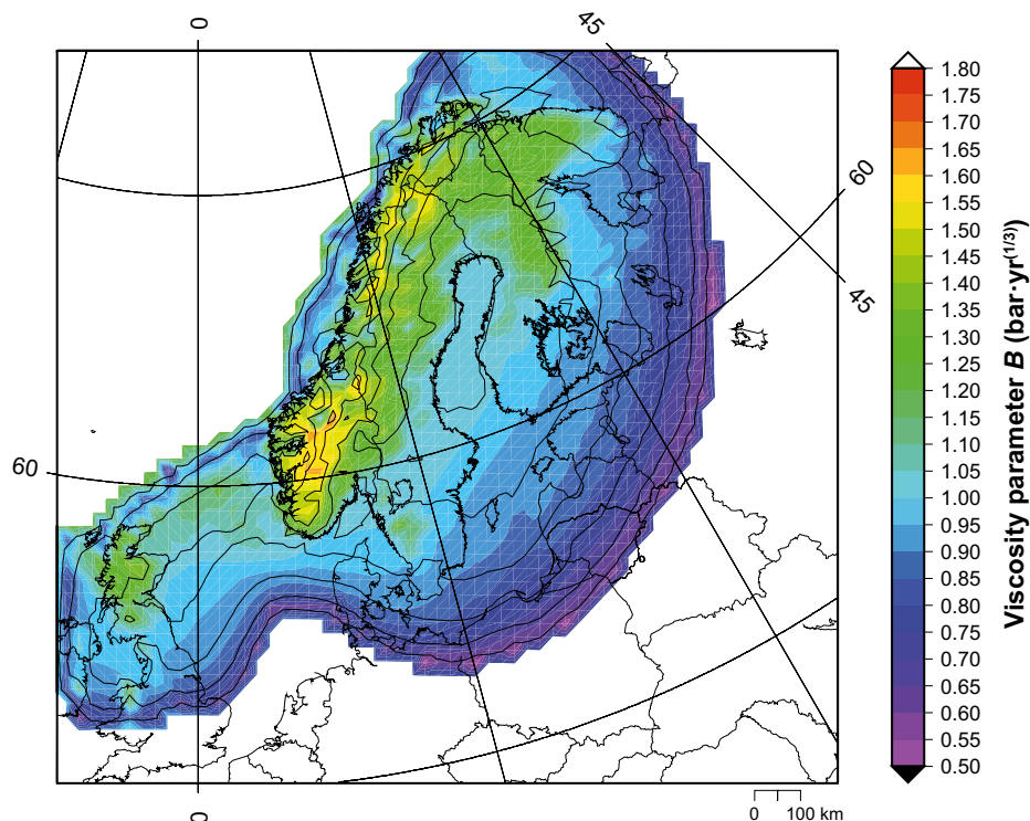
Figure 2-50. Calculated flow-law viscosity parameter B at 18.5 ka BP (at around the Last Glacial Maximum), shown as vertically integrated values up the ice column. Colder and harder ice is seen in the central parts of the ice sheet and over the Scandinavian mountain range (larger B values), while warmer and softer ice is seen closer to the ice margin (smaller B values). The black lines show ice thickness contours with a 500 m interval.
