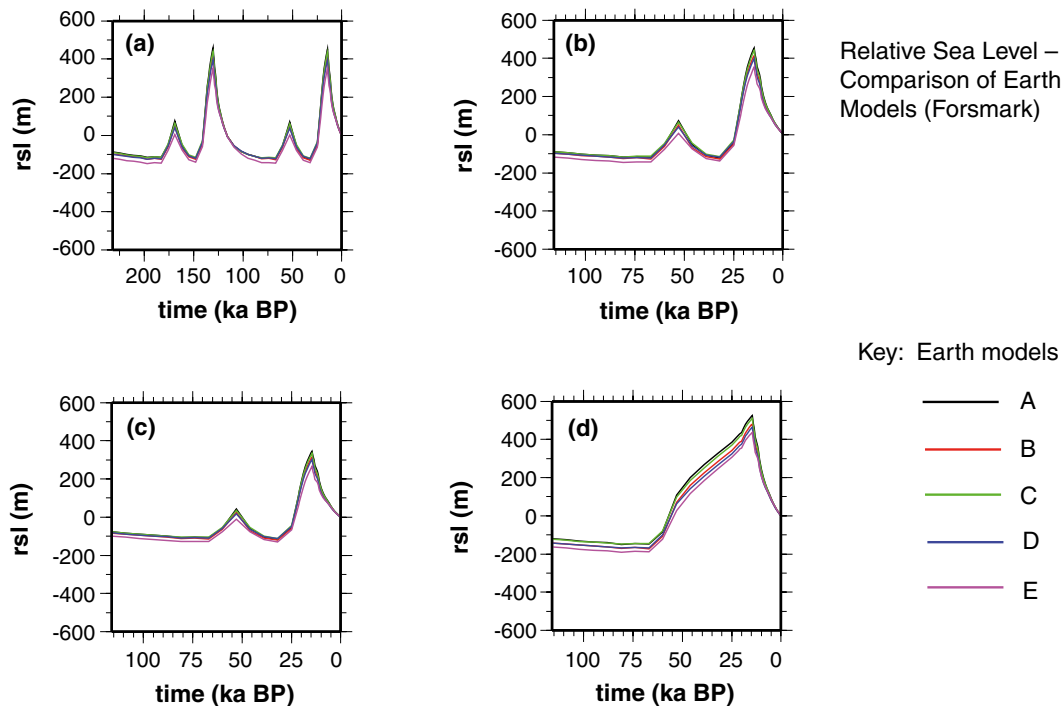
Figure 2-22. Comparison of Earth models. Predicted relative sea-level for Forsmark for all five Earth models under consideration. See Table 2-4 for details of the loading models. a): Double Weichselian glacial cycle – loading model 2. b): Single Weichselian glacial cycle – loading model 1. c): Single Weichselian glacial cycle modified with 80% ice thickness in Fennoscandia – loading model 5. d): Single Weichselian glacial cycle modified with a constant, linear increase in ice thickness in Fennoscandia between 60 ka BP and 20 ka BP – loading model 7.
