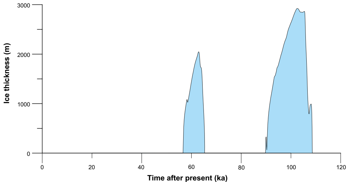
Figure 4-10. Development of ice-sheet thickness at the Forsmark site in the Weichselian glacial cycle climate case. Note that even though an ice sheet is present in Fennoscandia during most of the glacial cycle (Figure 4-8) the Forsmark site, located in south-central Sweden, is not covered by the ice sheet for the majority of the time.
