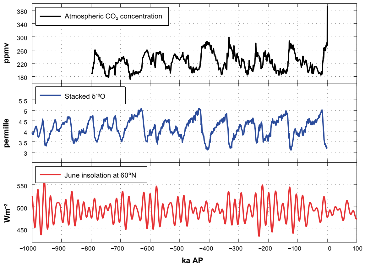
Figure 3-1. CO 2 composite record (upper panel; Lüthi et al. 2008) complemented with the observed annual average atmospheric CO 2 concentration in 2012 AD (393.8 ppmv; www.esrl.noaa.gov ). High values of CO 2 correspond to a warmer climate (interglacial state). A stack (middle panel; Lisiecki and Raymo 2005) of 57 benthic \delta^{18}\text{O} records; the \delta^{18}\text{O} is a proxy for the global ice volume. High values of \delta^{18}\text{O} correspond to a colder climate (glacial state). June insolation at 60°N (lower panel; Berger 1978, Berger and Loutre 1991).
