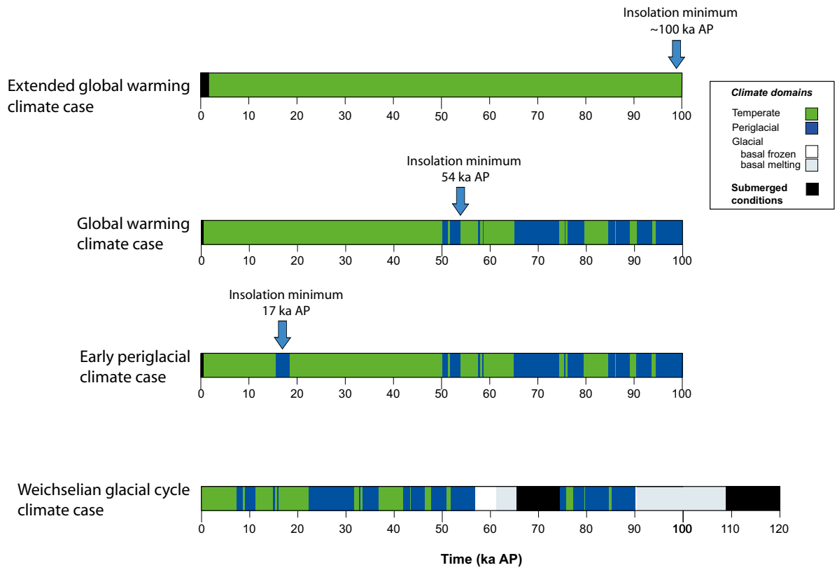
Figure 4-19. Summary of future climate cases analysed in the SR-PSU safety assessment. The cases go from warmer/wetter climates at the top to colder/dryer climates at the bottom.
