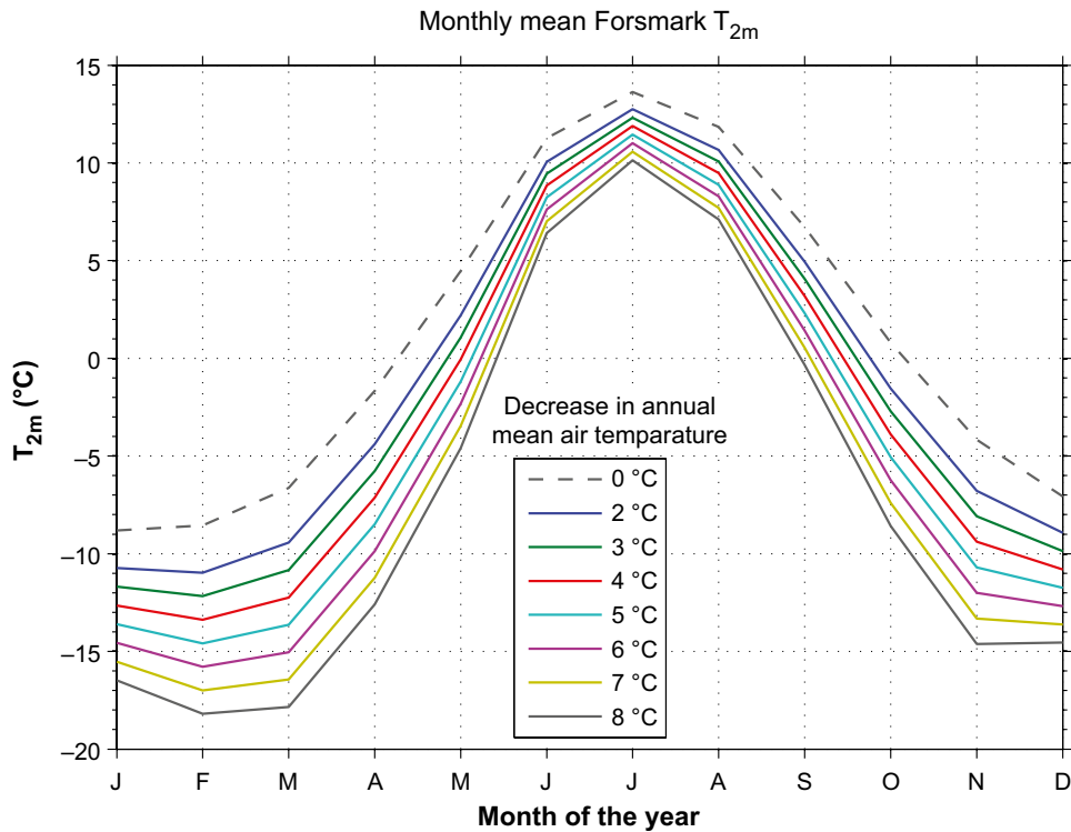
Figure 2-10. Monthly mean bias-corrected Forsmark T_{2m} (°C) in the LC_54k_180 simulation (dashed line) and in the sensitivity experiments (solid lines) performed with the permafrost model.
