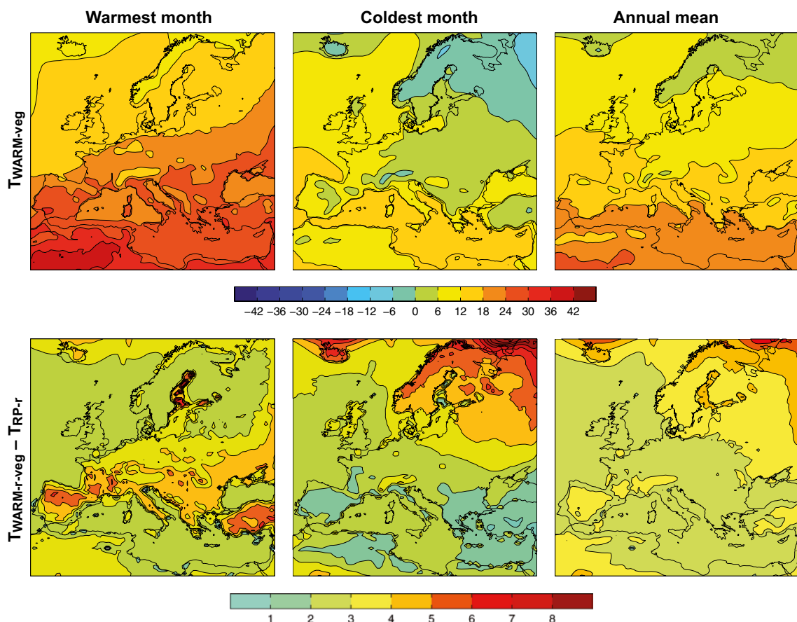
Figure 3-32. Mean near-surface air temperatures of the warmest month, coldest month and annual mean in the global warming simulation with improved vegetation (upper row). Also shown are differences between the global warming simulation and the simulations of the present climate (RP-r) (1961–2000) (lower row). Units are °C. From Kjellström et al. (2009).
