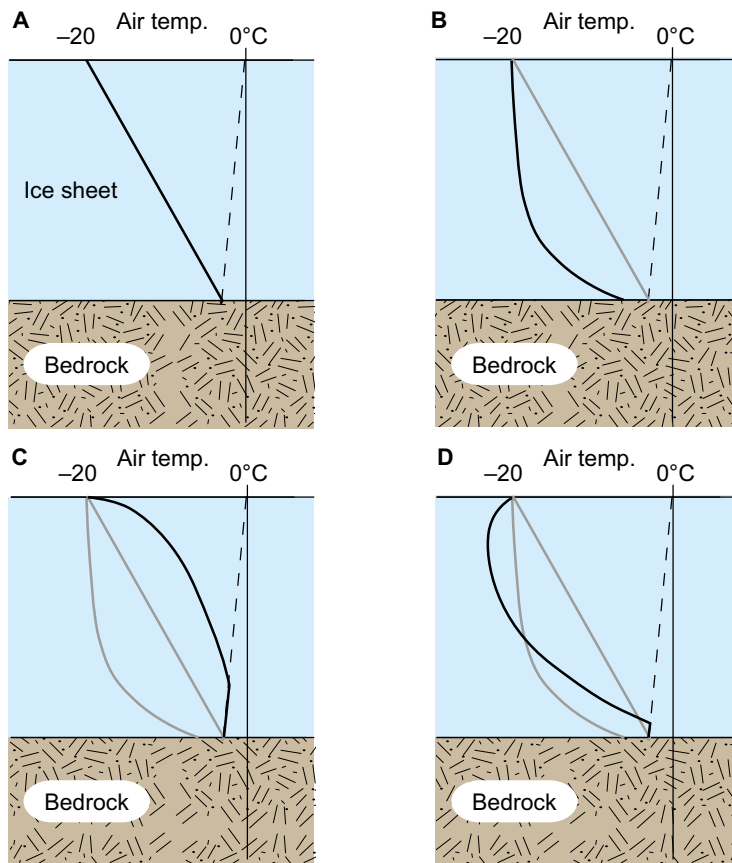
Figure 2-39. Vertical temperature profiles through a 2,000 m thick theoretical polar ice sheet. The dashed line denotes the pressure melting point temperature. a) No ice flow (dead-ice body), b) Vertical ice flow only – accumulation area (reflecting only a surface accumulation rate), and c) Vertical ice flow only – ablation area, d) Horizontal and vertical ice flow – accumulation area. Grey lines show the cases from the previous plates. Modified from Holmlund and Jansson (2003), after Sharp (1960).
