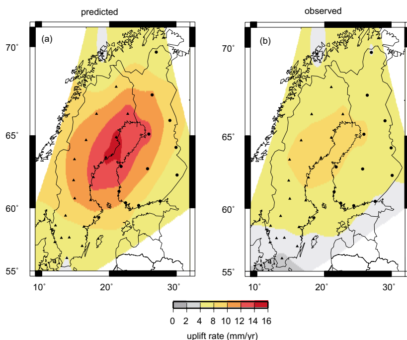
Figure 2-21. Comparison of predicted and observed present-day uplift rates. a) Predicted present-day uplift rates interpolated at GPS sites (black dots and triangles). Data generated using the Weichselian glacial cycle loading model (model 1 in Table 2-4) and an Earth model consisting of a 96 km-thick elastic lithosphere, an upper mantle of viscosity 0.5 \cdot 10^{21} Pa s, and a lower mantle of viscosity 1 \cdot 10^{22} Pa s (model A in Table 2-5). b) Observed present-day uplift rates interpolated at GPS sites. Data from the BIFROST project (Johansson et al. 2002).
