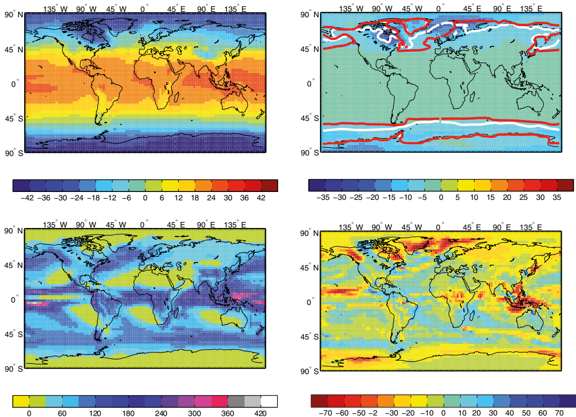
Figure 3-6. Annual mean near-surface air temperature in the MIS 3 simulation (upper left) and the difference compared with a simulated pre-industrial climate (upper right). Units are °C. Also shown is the annual mean sea ice edge (defined at 10% areal sea ice cover) for the pre-industrial simulation (white; upper right) and the MIS 3 simulation (red; upper right). The lower panels show the simulated precipitation (lower left) and the difference compared with the simulated pre-industrial climate (lower right). Units are mm/month. From Kjellström et al. (2009).
