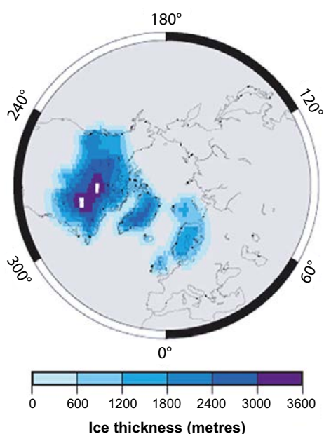
Figure 2-30. Ice thicknesses in the Northern Hemisphere at the LGM (20 ka BP). From the models of Tushingham and Peltier (1991) and Lambeck et al. (1998).
