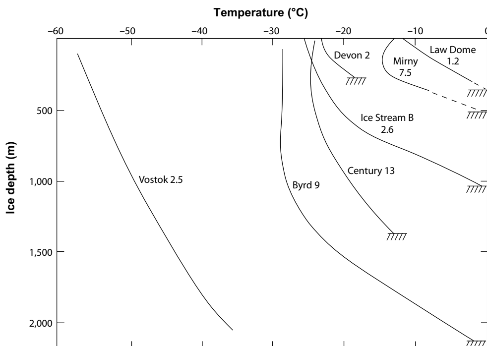
Figure 2-40. Borehole temperature data from the Greenland and Antarctic ice sheets. Modified from Holmlund and Jansson (2003), after Paterson (1994).
