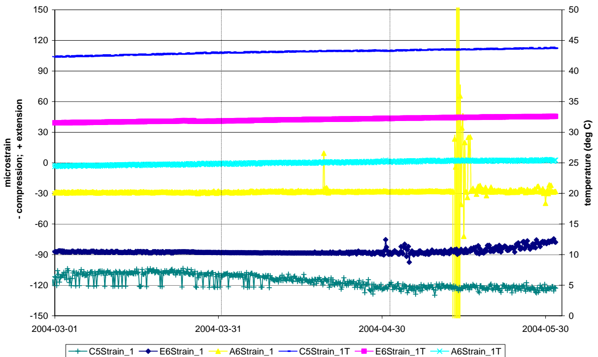
Vertical strain adjacent to Deposition Holes 5 and 6
