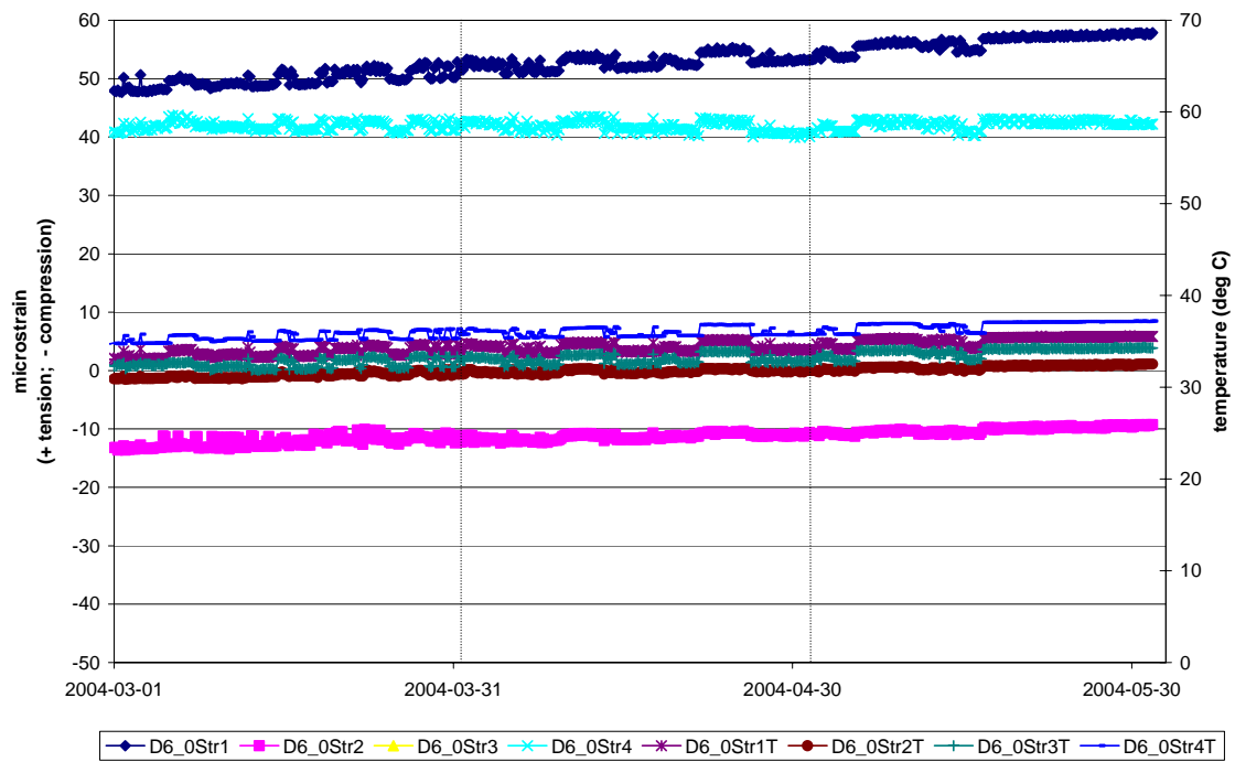
Strain measurements Borehole D6 (0)
