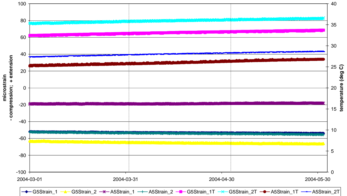
Vertical strain adjacent to Deposition Hole 5
