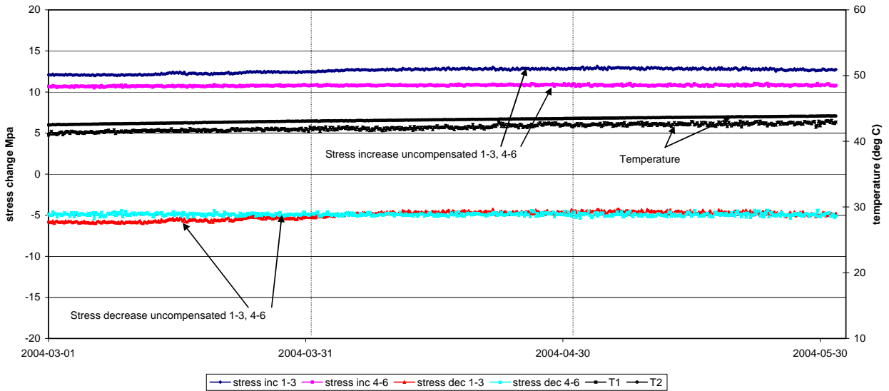
Biaxial stressmeter G5 Maximum stress increase and stress decrease in plane perpendicular to borehole axis
