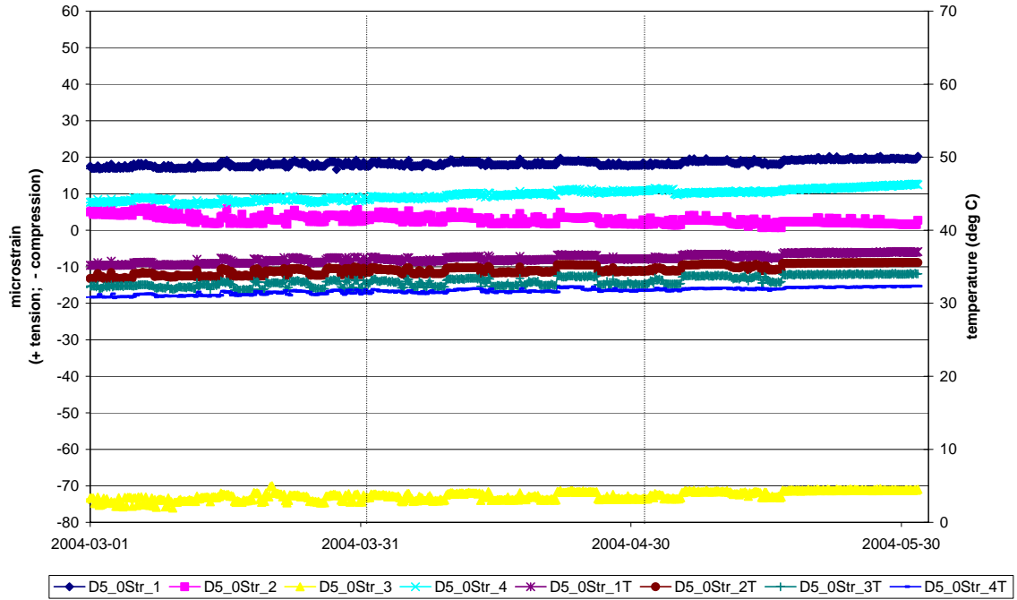
Strain measurements Borehole D5 (0)
