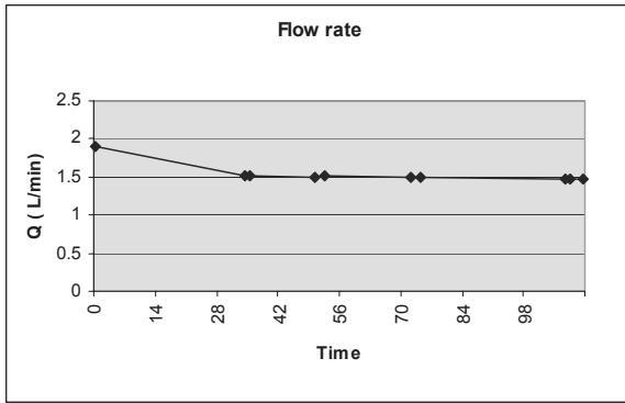
Figure 6-2 Flow rates during draw down in KA3554G01:2. Time in minutes.
