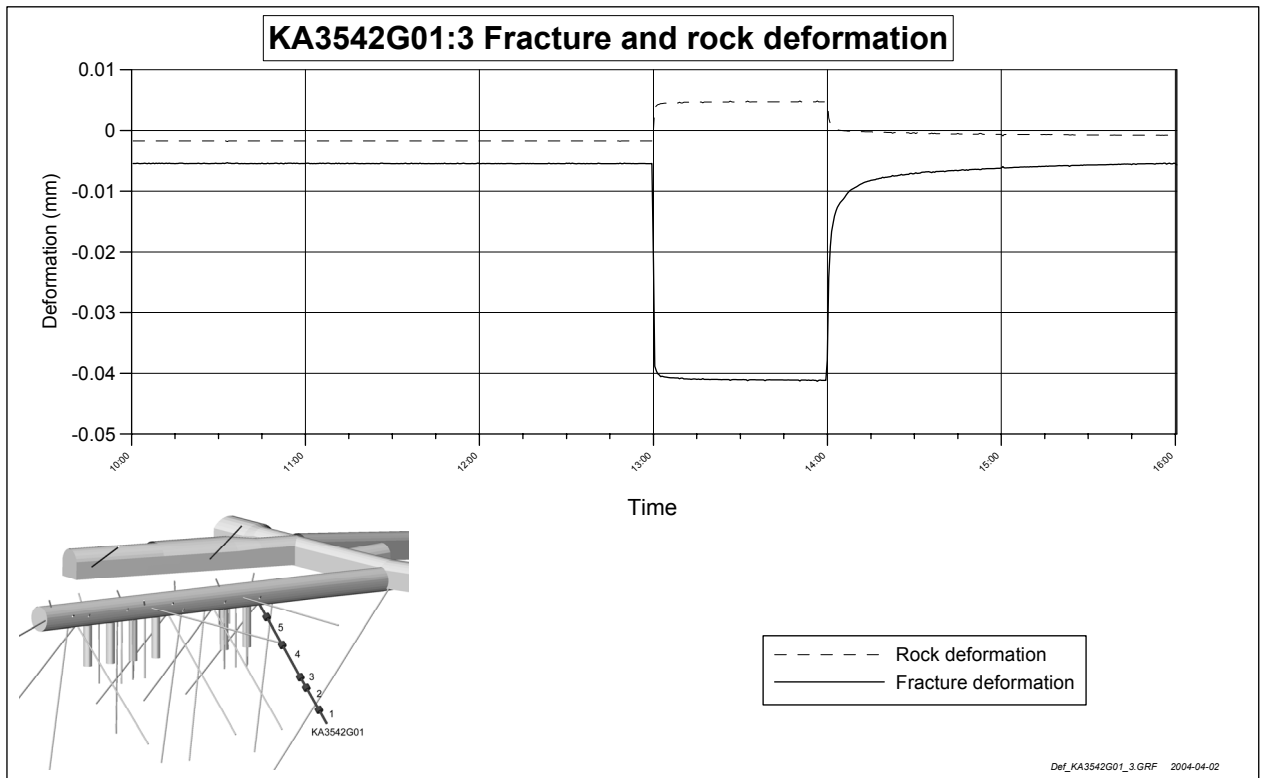
Figure 6-10 Deformation measurements in KA3542G01:3 (Test 3:5).
