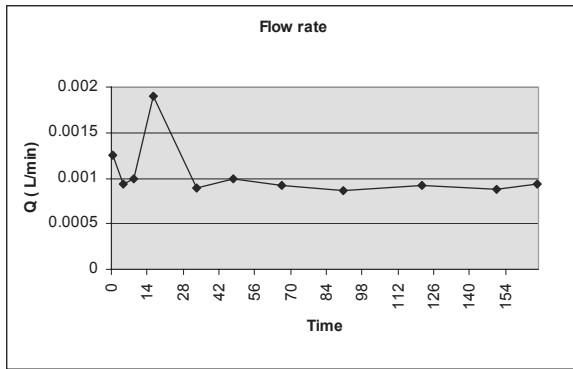
Figure 6-7 Flow rate during draw down in KA3546G01:2. Time in minutes.
