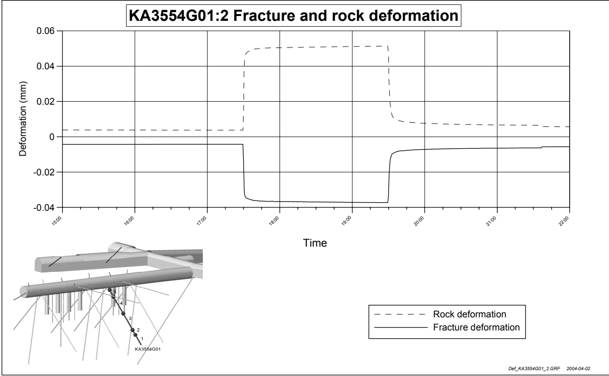
Figure 6-9 Deformation measurements in KA3554G01:2 (Test 3:2).
