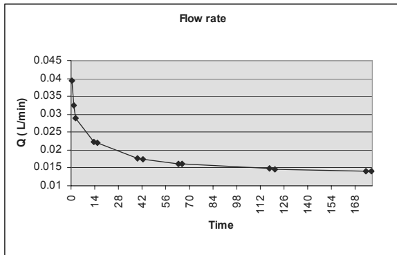
Figure 6-6 Flow rate during draw down in KA3542G02:2. Time in minutes.
