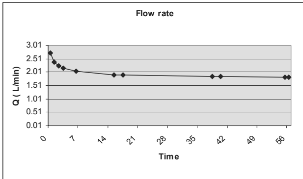
Figure 6-4 Flow rates during draw down in KA3548A01:3. Time in minutes.
