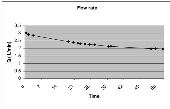
Figure 6-8 Flow rate during draw down in KA3539G:2. Time in minutes.
