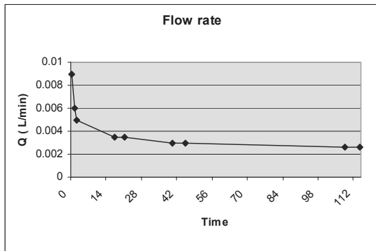
Figure 6-1 Flow rates during draw down in KA3552G01:2. Time in minutes.
