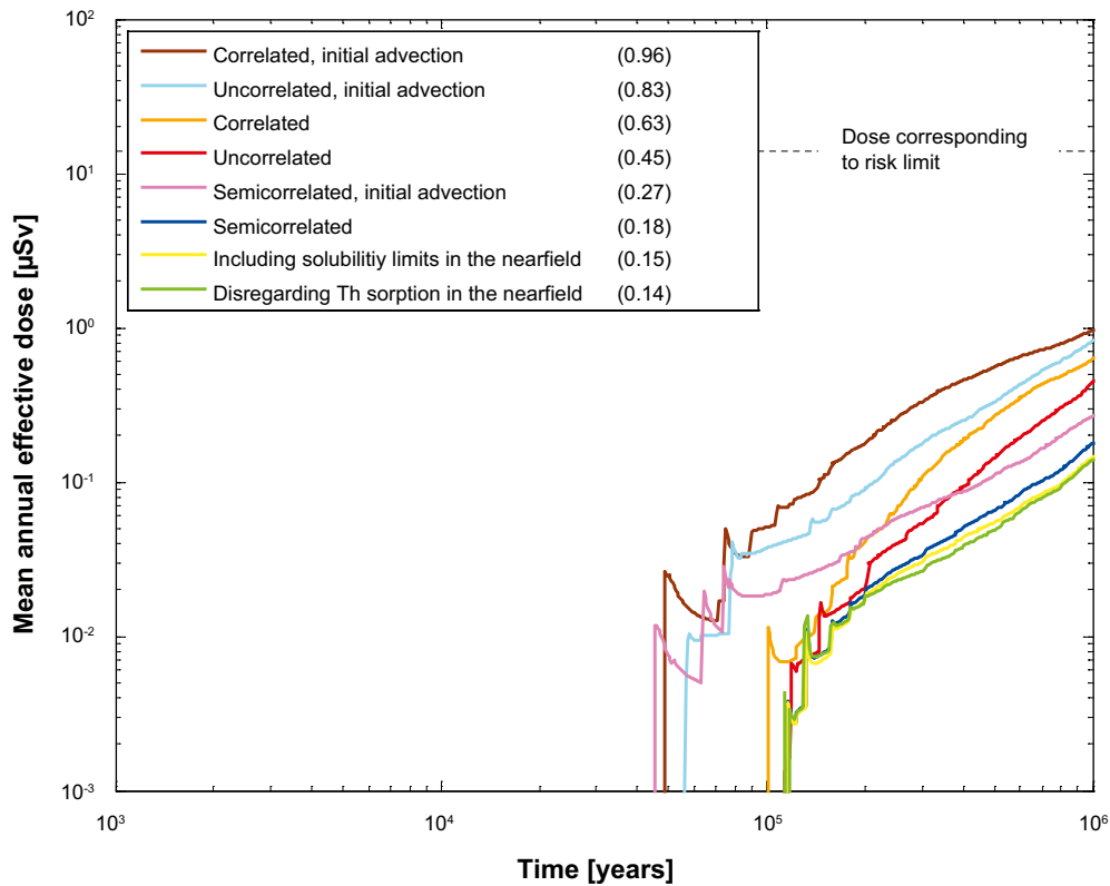
Figure 4-59. Far-field annual effective dose for probabilistic corrosion cases calculated with FARF31. The legend is sorted by peak (in the one-million year period) of the mean annual effective dose. The values in brackets are peak dose in units of \mu\text{Sv} .
