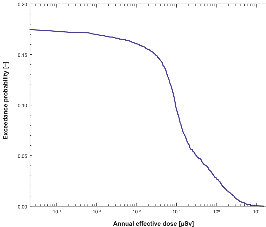
Figure 6-51. Exceedance probability for a given dose rate ( \mu\text{Sv}/\text{yr} ) for the pinhole Q1 release. A 1-million year time window was used to calculate the exceedance probability. Thus, for a given dose rate, the exceedance probability is the probability that the dose rate exceeds that value at some time during the 1-million year period.
