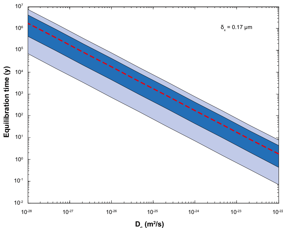
Figure B-18. Typical equilibration times for diffusive uptake to a solid-solution as a function of solid state diffusivity for a limited penetration depth of 1.7 \cdot 10^{-7} m estimated for calcite fracture mineralisations at Forsmark. The broken red line shows the time required for 50% equilibration of the assumed slab geometry while the limits of the dark band represent the time for 25%–75% equilibration. The limits of the outer lightly shaded band show the range of times required for 10%–90% diffusive equilibration.
