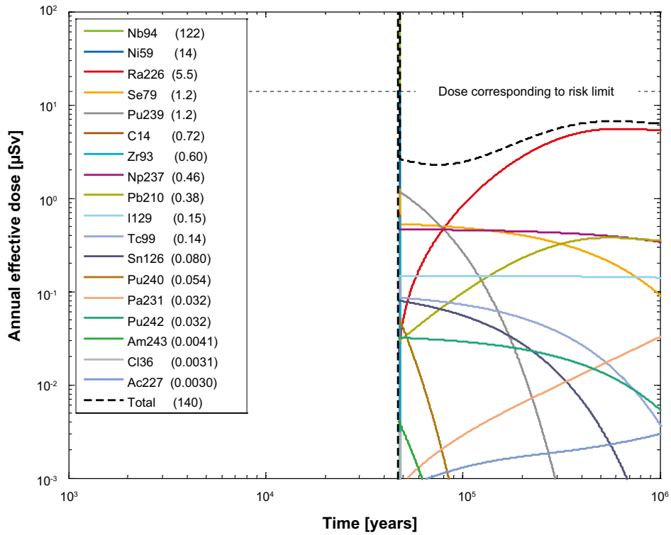
Figure 4-36. Near-field dose equivalent release for a deterministic calculation of the corrosion scenario, with hydrogeological data from the uncorrelated model and initial advection in the erosion/corrosion model. The legend is sorted by peak (in the one-million year period) of the annual effective dose. The values in brackets are peak dose in units of \mu\text{Sv} . Note that the dose equivalent release for Nb-94 is 122 \mu\text{Sv}/\text{year} , i.e. above the end of the y-axis.
