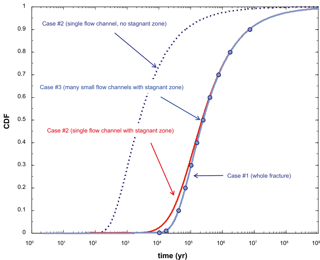
Figure A-6. Residence time distribution for a weakly sorbing solute ( K_d = 0.001 \text{ m}^3/\text{kg} ) for the channelling scenario involving 10 smaller flow channels although for the same total flow-wetted surface (10% of fracture surface area). The same channelling scenarios as in the previous Figures are also shown for comparison. The reference F -factor for Case #1 is 5 \cdot 10^5 \text{ yr/m} . Results are shown as a cumulative probability density function (CDF).
