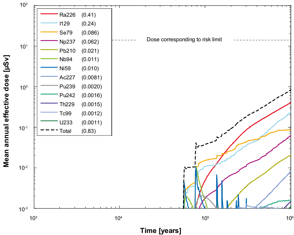
Figure 4-39. Far-field mean annual effective dose for the probabilistic calculation of the corrosion scenario, with hydrogeological data from the uncorrelated model and initial advection in the erosion/corrosion model. The legend is sorted by peak (in the one-million year period) of the mean annual effective dose. The values in brackets are peak dose in units of \mu\text{Sv} .
