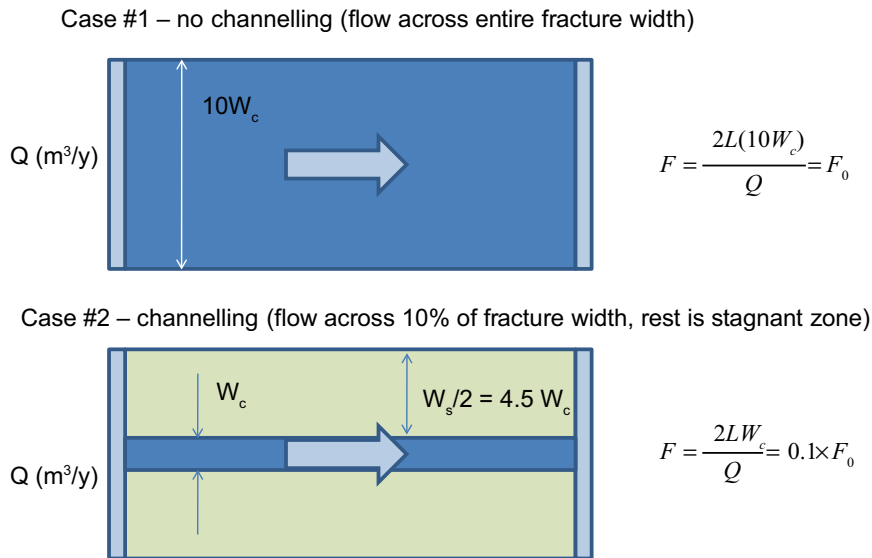
Figure A-2. Idealised example of a simple flow channel of width W_c equal to 10% of the fracture width hosted in a fracture of length L (Case 2 – bottom) as compared with the null case of a fracture where flow contacts the entire surface (Case 1 – top). Case 2 approximately corresponds to the F -factor scaling assumption used previously in SR-Can /SKB 2006/.
