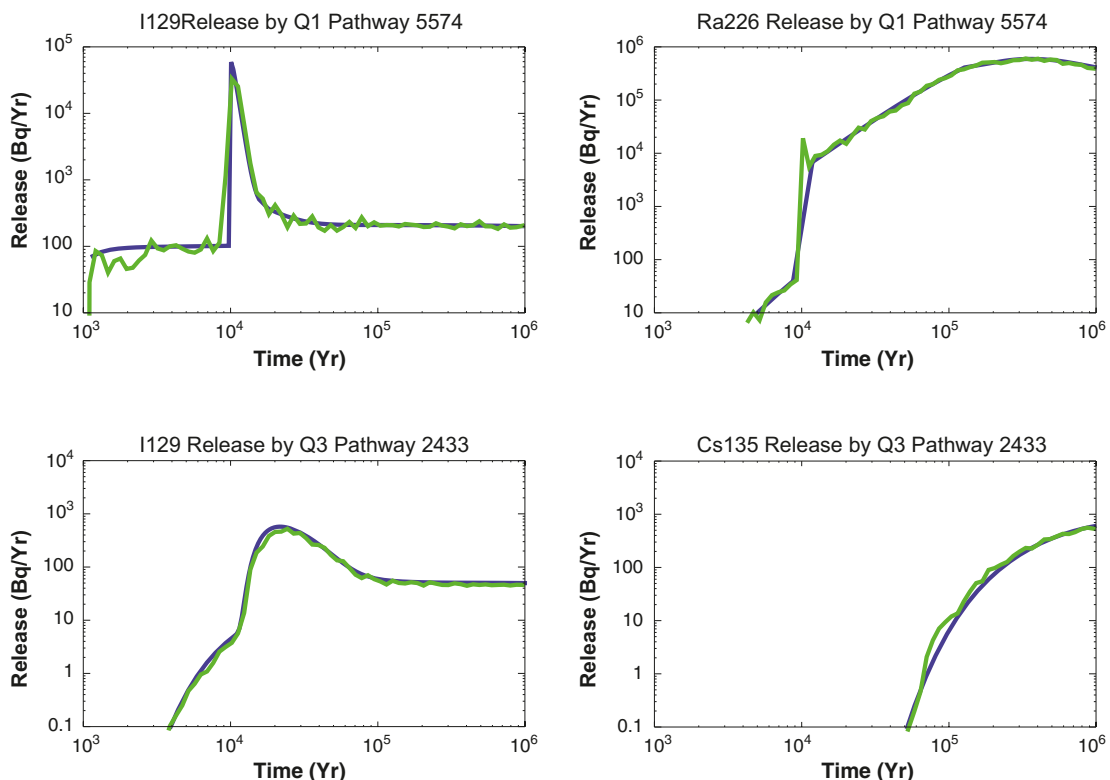
Figure C-1. Comparison between MARFA and FARF31 for two release points in the growing pinhole case.
