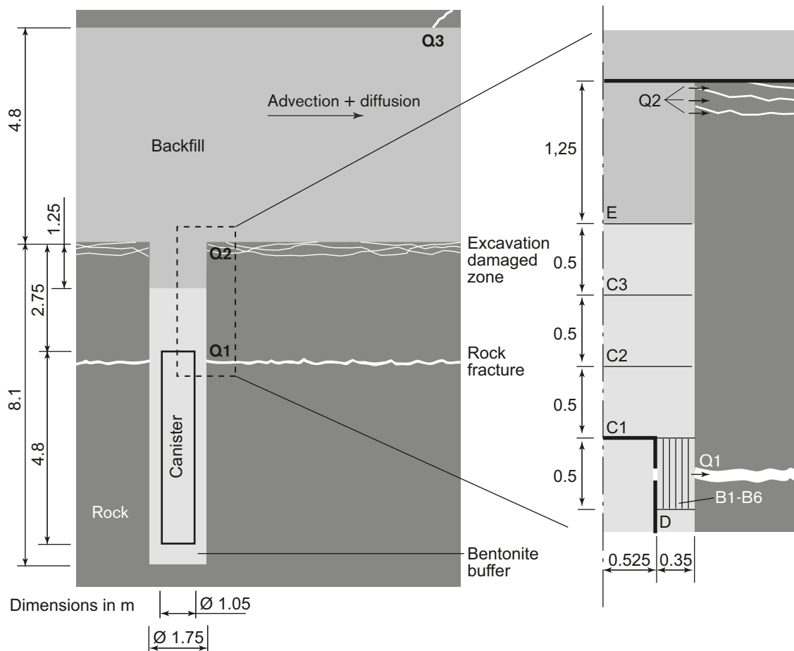
Figure G-3. Schematic picture of the compartments (including sub-compartments) B1-B6, C1-C3, D and E in the case with growing pinhole failure. The transport paths Q1, Q2 and Q3 to a fracture intersecting the deposition hole, to the excavation damaged zone, and to a fracture intersecting the deposition tunnel, respectively, are also shown.
