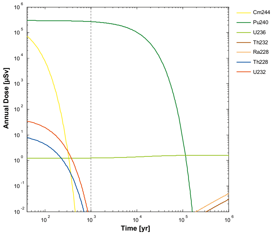
Figure D-4. Calculated annual dose in the hypothetical case supporting the selection of radionuclides for radionuclide transport calculations of the 4n chain. The vertical black dashed line denotes 1,000 years after closure.
