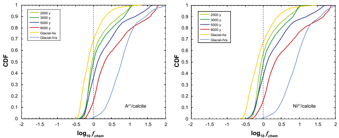
Figure B-8. Estimated groundwater chemistry correction factors ( f_{chem} ) for calcite solid solutions relative to the reference groundwater used in the scoping calculations. Data are plotted as a cumulative distribution function (CDF) for groundwater compositions at different times during repository evolution. The left-hand figure shows the approximate generic correction factor calculated using Equation B-24; the right-hand figure shows the nuclide specific correction factor for Ni^{2+} calculated using Equation B-23. The vertical broken line indicates the relative location of the reference groundwater composition (i.e. median Ca^{2+} concentration at 3,000 y).
