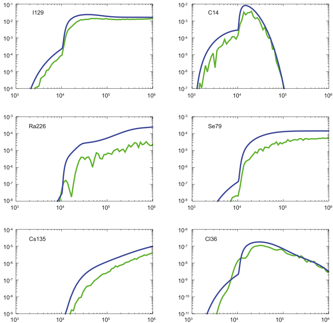
Figure 6-49. Near-field (blue) and far-field (green) releases for the top six contributors (by far-field release) for the Q3 release path. Units are \mu\text{Sv}/\text{yr} on the y-axis and year on the x-axis for each plot. Note the scale on the y-axis is different for different radionuclides.
