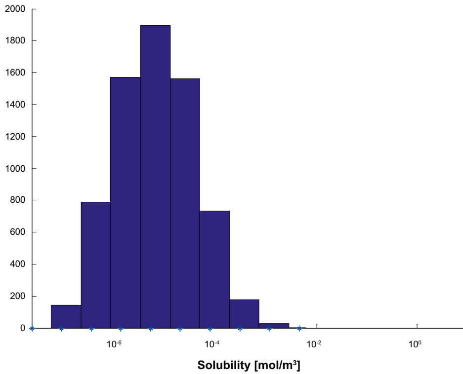
Figure F-29. Solubility limits for Se used as input data for COMP23 in SR-Site. The y-axis shows the number of realisations in each bin.
