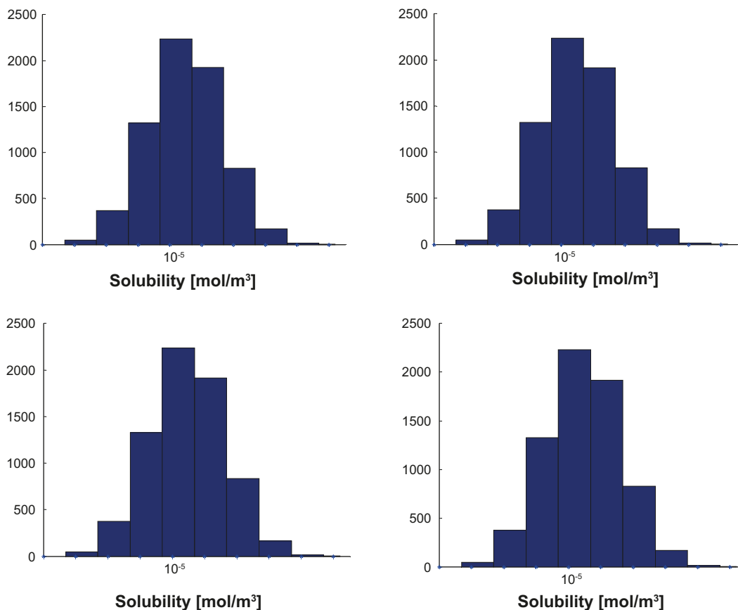
Figure F-8. Solubility limits for Zr using groundwater data from temperate conditions (upper left), permafrost conditions (upper right), glacial conditions (lower left) and submerged conditions (lower right). The y-axis shows the number of realisations in each bin.
