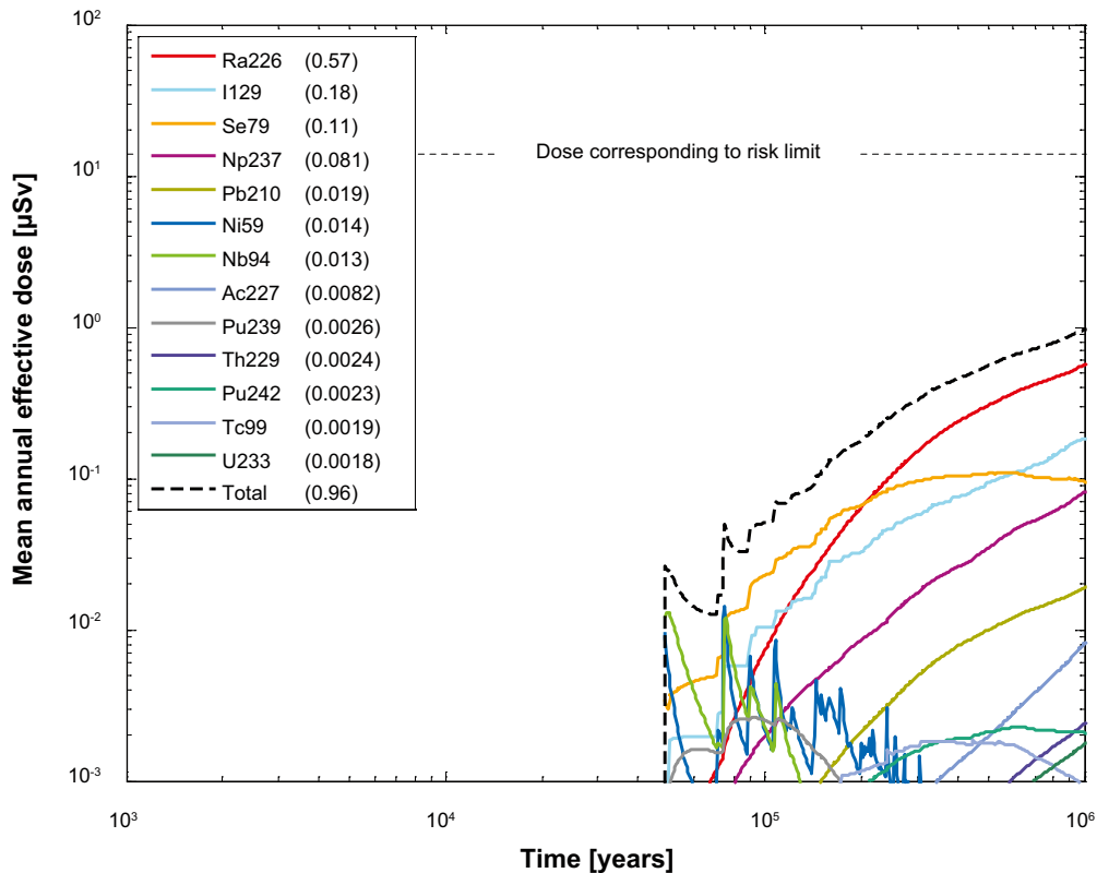
Figure 4-47. Far-field mean annual effective dose for the probabilistic calculation of the corrosion scenario, with hydrogeological data from the fully correlated model and initial advection in the corrosion model. The legend is sorted by peak (in the one-million year period) of the mean annual effective dose. The values in brackets are peak dose in units of \mu\text{Sv} .
