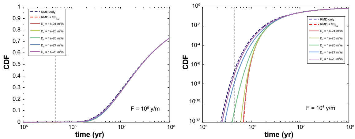
Figure B-23. Simulated residence time distribution curves for trivalent actinide transport assuming an F -factor of 10^6 yr/m and calcite solid solution for solid state diffusivities ranging from 10^{-28} m^2/s to 10^{-24} m^2/s . In the left-hand figure, data are plotted on a log-linear axis and on a log-log axis in the right-hand figure. The broken blue curve is the limiting case where only matrix diffusion and equilibrium sorption in the rock matrix is considered. The vertical broken line indicates the equilibrium retardation time for the solid solution, and the accompanying broken red curve shows the theoretical residence time distribution for matrix diffusion coupled with equilibrium retention by the solid solution.
