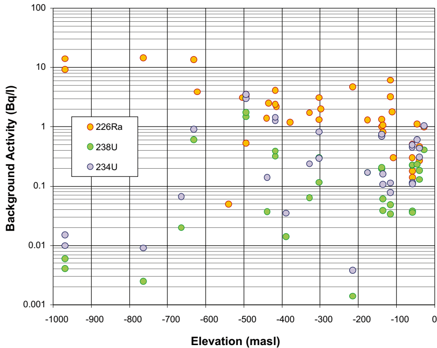
Figure 2-6. Typical background activities of the main naturally occurring radionuclides of interest in groundwater at the Forsmark site /Laaksoharju et al. 2008/ (numerical values are taken from the SKB SIMON database). Rn-222 is neglected on account of its gaseous form and consequent rapid dilution in the biosphere (it is also neglected in the calculation of far-field dose rates calculated in SR-Site owing to its low relative contribution to radiological risk).
