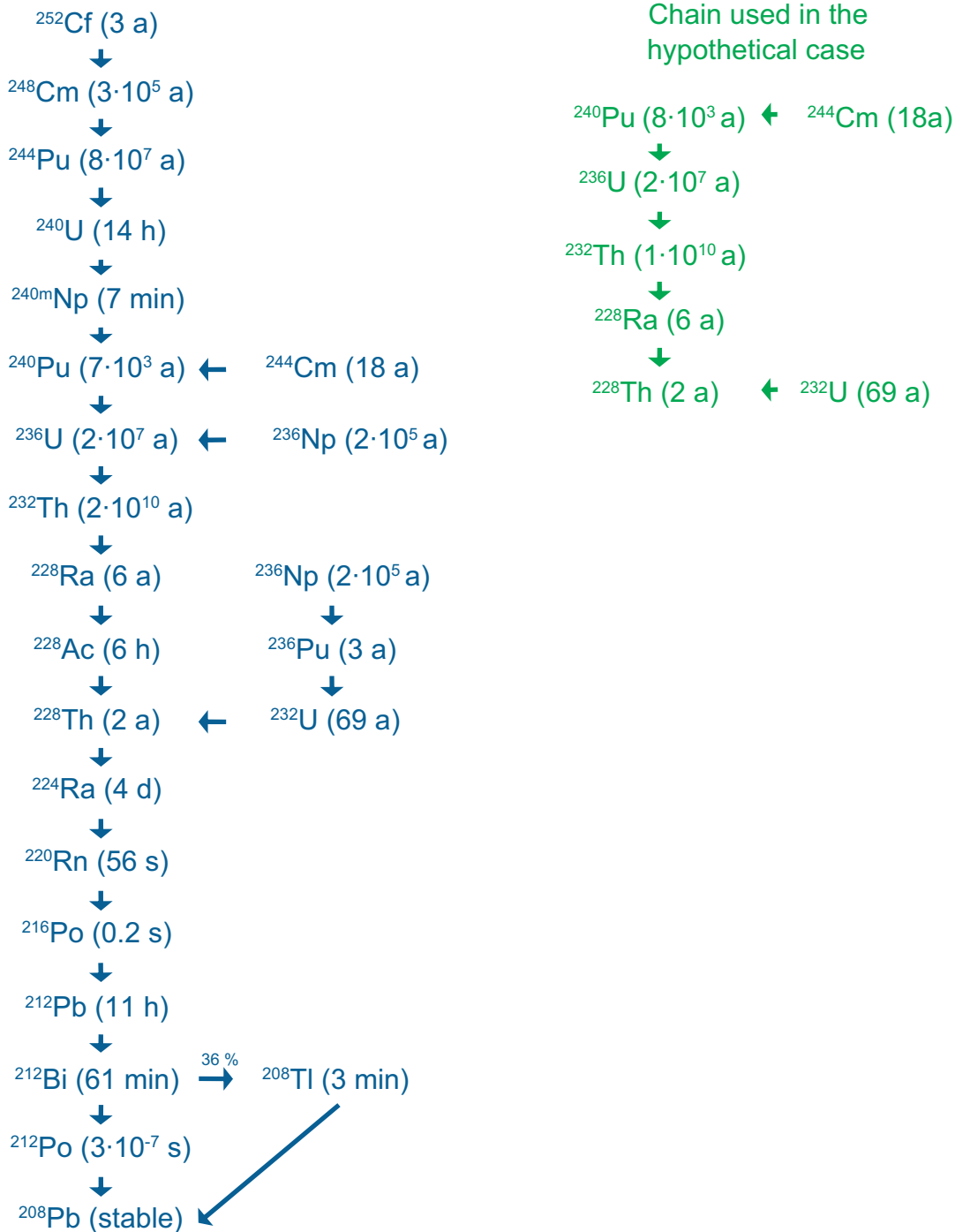
Figure D-3. The 4n chain. The half-lives are given within brackets. The simplified chain is used in the hypothetical calculation case to support the selection of radionuclides for the radionuclide transport calculations. Nuclides at the beginning of the chain without any inventory have been excluded in the simplified chain as have nuclides with a half-life shorter than 1 year. Approximate half-lives shown are derived from Table D-1.
