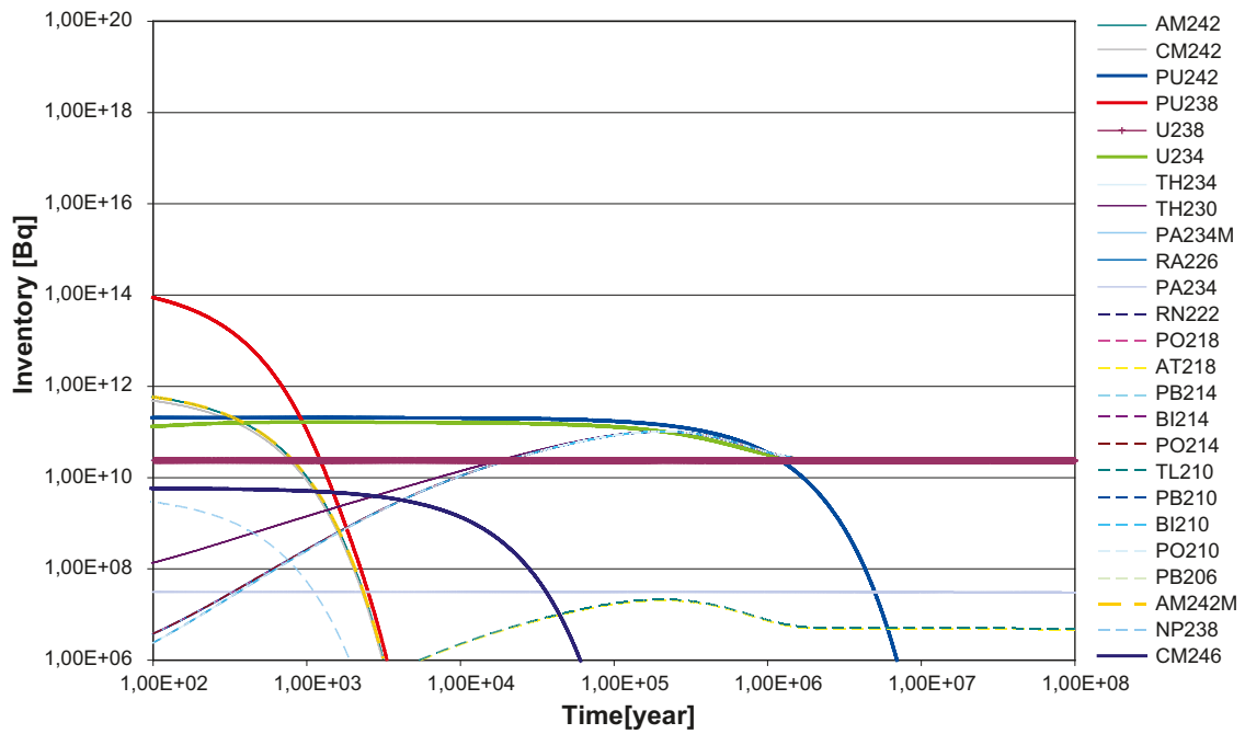
Figure D-13. Activity (Bq/tU) as a function of time for radionuclides in chain 4N+2. Initial inventory from /Håkansson 2000/.
