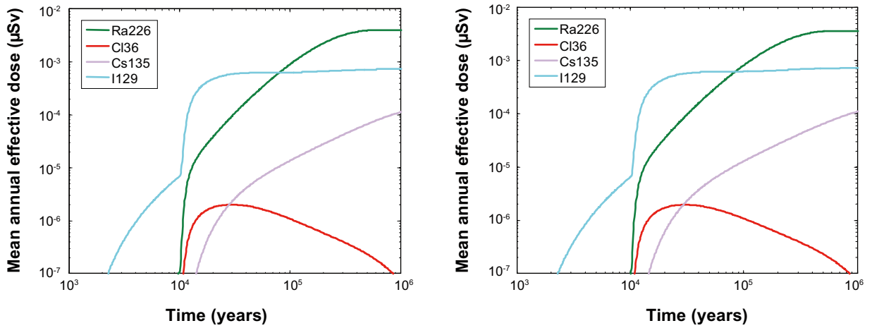
Figure G-11. Probabilistic near-field releases from Q3 for the growing pinhole case. The new tunnel discretisation used in SR-Site to the left and the old discretisation used in SR-Can to the right.
