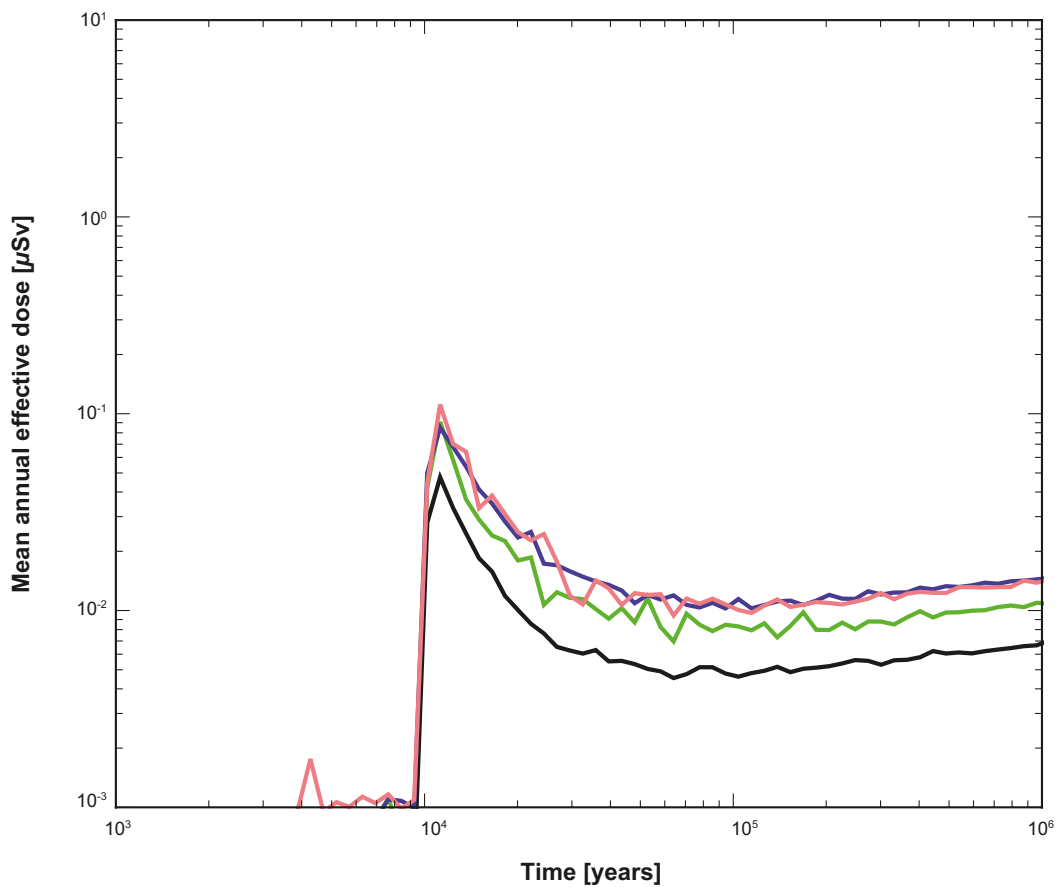
Figure 6-58. Expected far-field release as equivalent dose for pinhole Q1 release path and different assumptions about the EDZ. The blue curve is the Q1 base case, which has EDZ transmissivity of 10^{-8} m 2 /s. The black is the case for no EDZ. The green and pink curves are results for EDZ transmissivity of 10^{-6} m 2 /s and 10^{-7} m 2 /s, respectively.
