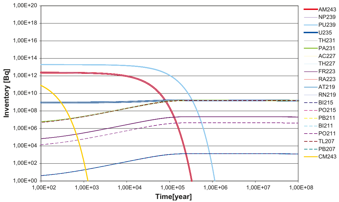
Figure D-17. Activity (Bq/tU) as a function of time for radionuclides in the 4n+3 chain. Initial inventory from /Håkansson 2000/.
