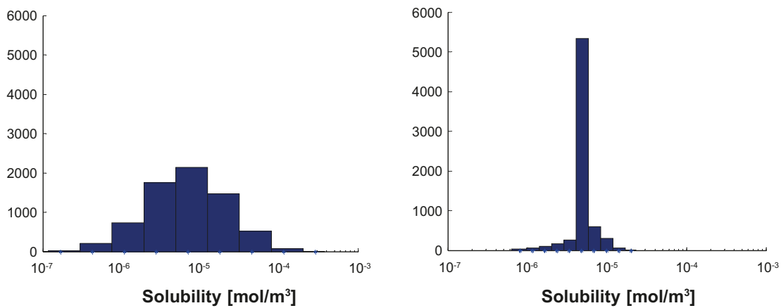
Figure F-13. Solubility limits for Se using groundwater data from temperate conditions. Fixed groundwater composition and varying thermodynamic data (left). Varying groundwater composition and fixed thermodynamic data (right). The y-axis shows the number of realisations in each bin.
