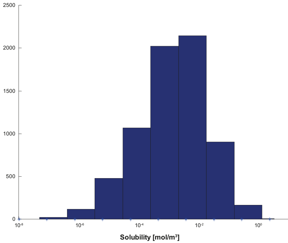
Figure F-27. Solubility limits for Pu used as input data for COMP23 in SR-Site. The y-axis shows the number of realisations in each bin.
