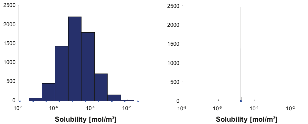
Figure F-16. Solubility limits for Zr using groundwater data from temperate conditions. Fixed groundwater composition and varying thermodynamic data (left). Varying groundwater composition and fixed thermodynamic data (right). The y-axis shows the number of realisations in each bin.
