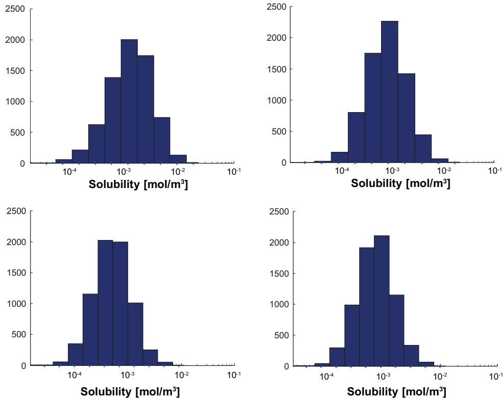
Figure F-2. Solubility limits for Pb using groundwater data from temperate conditions (upper left), permafrost conditions (upper right), glacial conditions (lower left) and submerged conditions (lower right). The y-axis shows the number of realisations in each bin.
