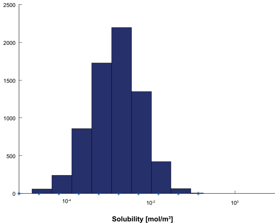
Figure F-19. Solubility limits for Cm used as input data for COMP23 in SR-Site. The y-axis shows the number of realisations in each bin.
