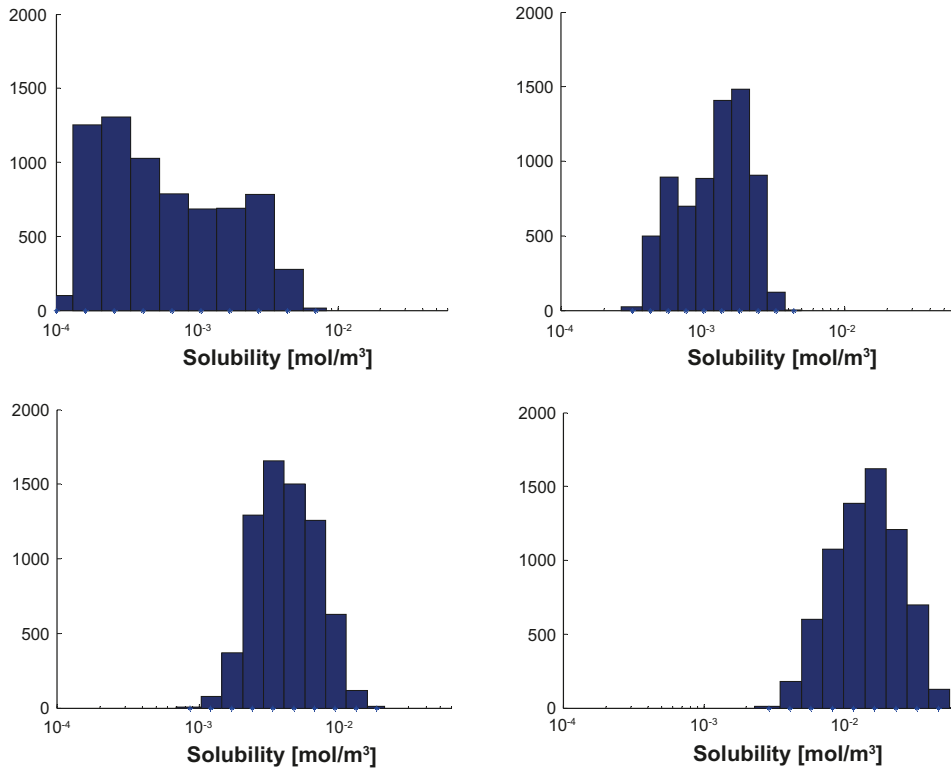
Figure F-4. Solubility limits for Ra using groundwater data from temperate conditions (upper left), permafrost conditions (upper right), glacial conditions (lower left) and submerged conditions (lower right). The y-axis shows the number of realisations in each bin.
