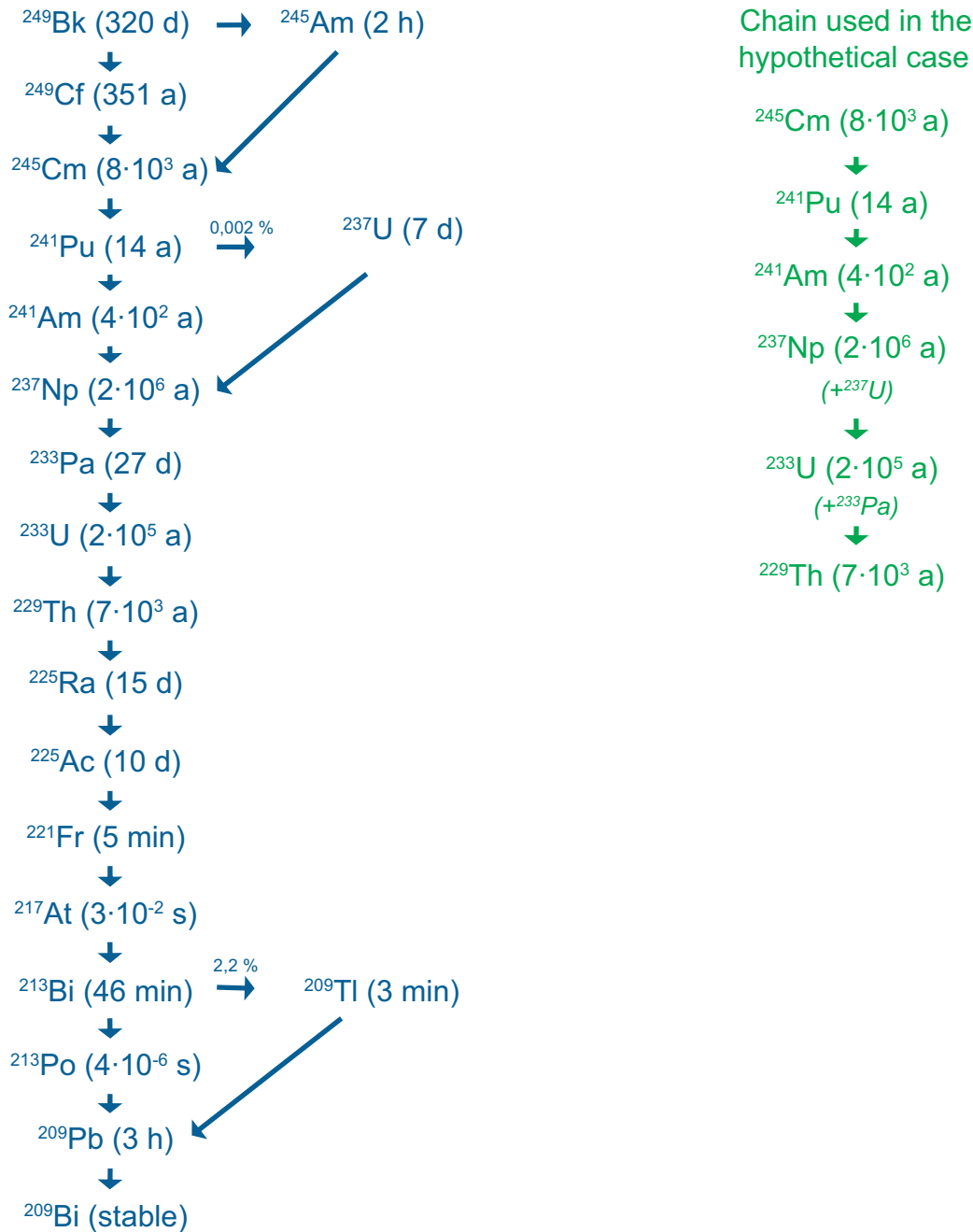
Figure D-7. The 4n+1 chain. The simplified chain is used in the hypothetical case to support the selection of radionuclides for the radionuclide transport calculations. Nuclides at the beginning of the chain without any inventory have been excluded in the simplified chain as have nuclides with a half-life shorter than 1 year but their inventories have been included in those of their daughters. Approximate half-lives shown are derived from Table D-2.
