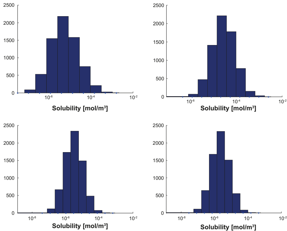
Figure F-6. Solubility limits for Th using groundwater data from temperate conditions (upper left), permafrost conditions (upper right), glacial conditions (lower left) and submerged conditions (lower right). The y-axis shows the number of realisations in each bin.
