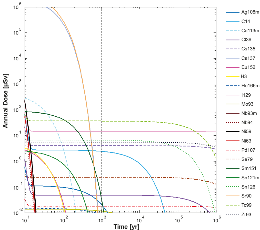
Figure D-2. Calculated annual dose in the hypothetical case to support the selection of radionuclides for the radionuclide transport calculations of fission and activation products. The vertical black dashed line denotes 1,000 years after closure.
