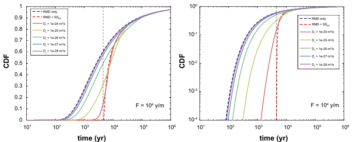
Figure B-21. Simulated residence time distribution curves for trivalent actinide transport assuming an F-factor of 10^4 yr/m and calcite solid solution for solid state diffusivities ranging from 10^{-28} m 2 /s to 10^{-24} m 2 /s. In the left-hand figure, data are plotted on a log-linear axis and on a log-log axis in the right-hand figure. The broken blue curve is the limiting case where only matrix diffusion and equilibrium sorption in the rock matrix is considered. The vertical broken line indicates the equilibrium retardation time for the solid solution, and the accompanying broken red curve shows the theoretical residence time distribution for matrix diffusion coupled with equilibrium retention by the solid solution.
