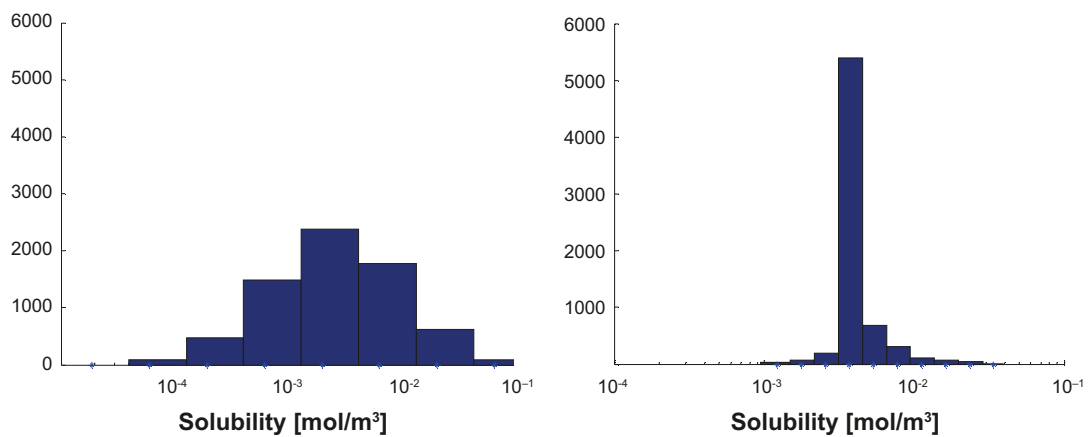
Figure F-11. Solubility limits for Pu using groundwater data from temperate conditions. Fixed groundwater composition and varying thermodynamic data (left). Varying groundwater composition and fixed thermodynamic data (right). The y-axis shows the number of realisations in each bin.
