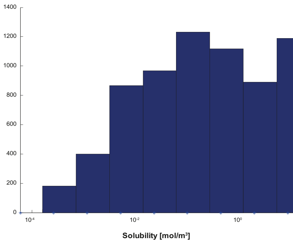
Figure F-22. Solubility limits for Ni used as input data for COMP23 in SR-Site. The y-axis shows the number of realisations in each bin.
