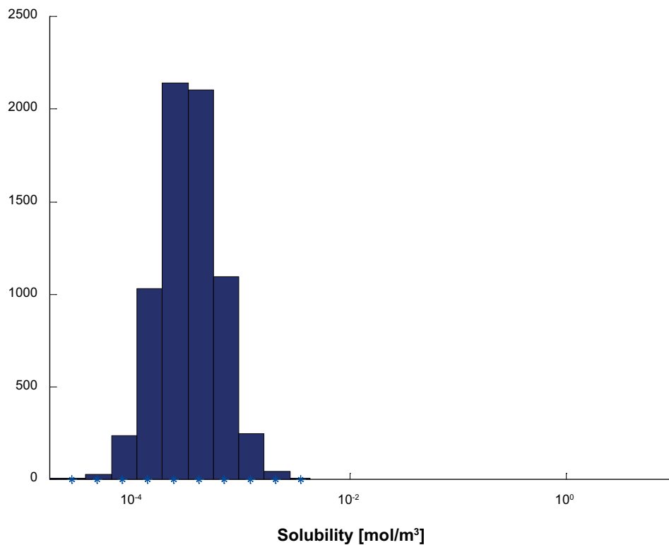
Figure F-24. Solubility limits for Pa used as input data for COMP23 in SR-Site. The y-axis shows the number of realisations in each bin.
