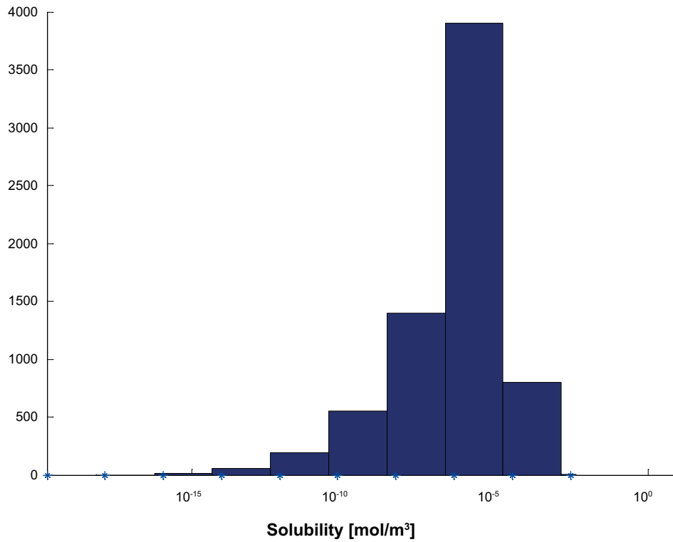
Figure F-35. Solubility limits for U used as input data for COMP23 in SR-Site. The y-axis shows the number of realisations in each bin.
