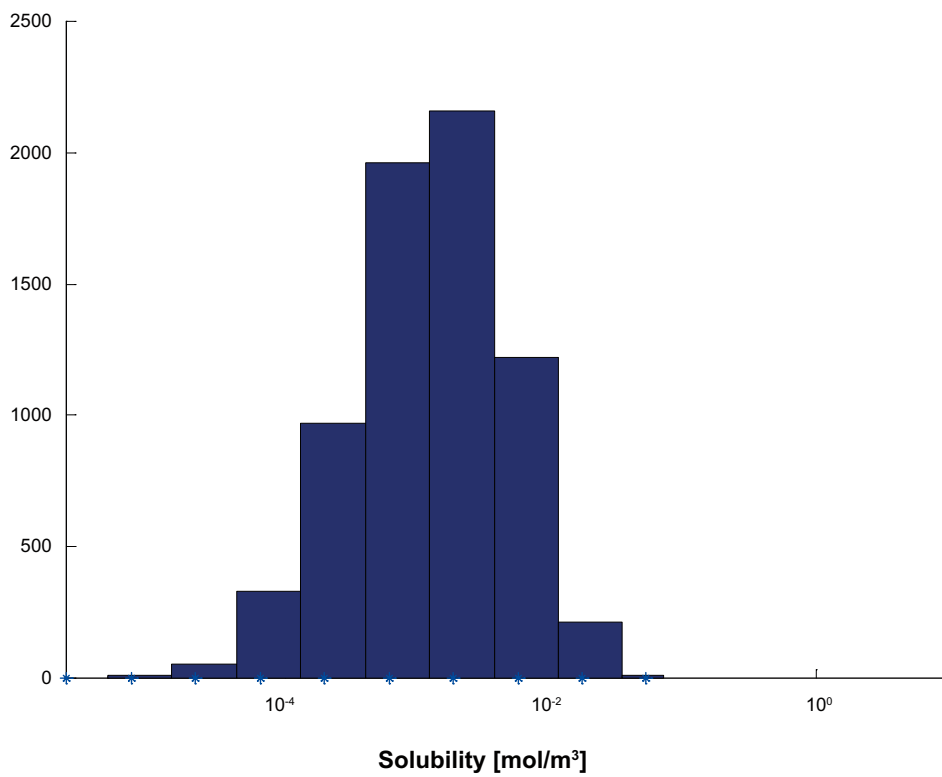
Figure F-18. Solubility limits for Am used as input data for COMP23 in SR-Site. The y-axis shows the number of realisations in each bin.
