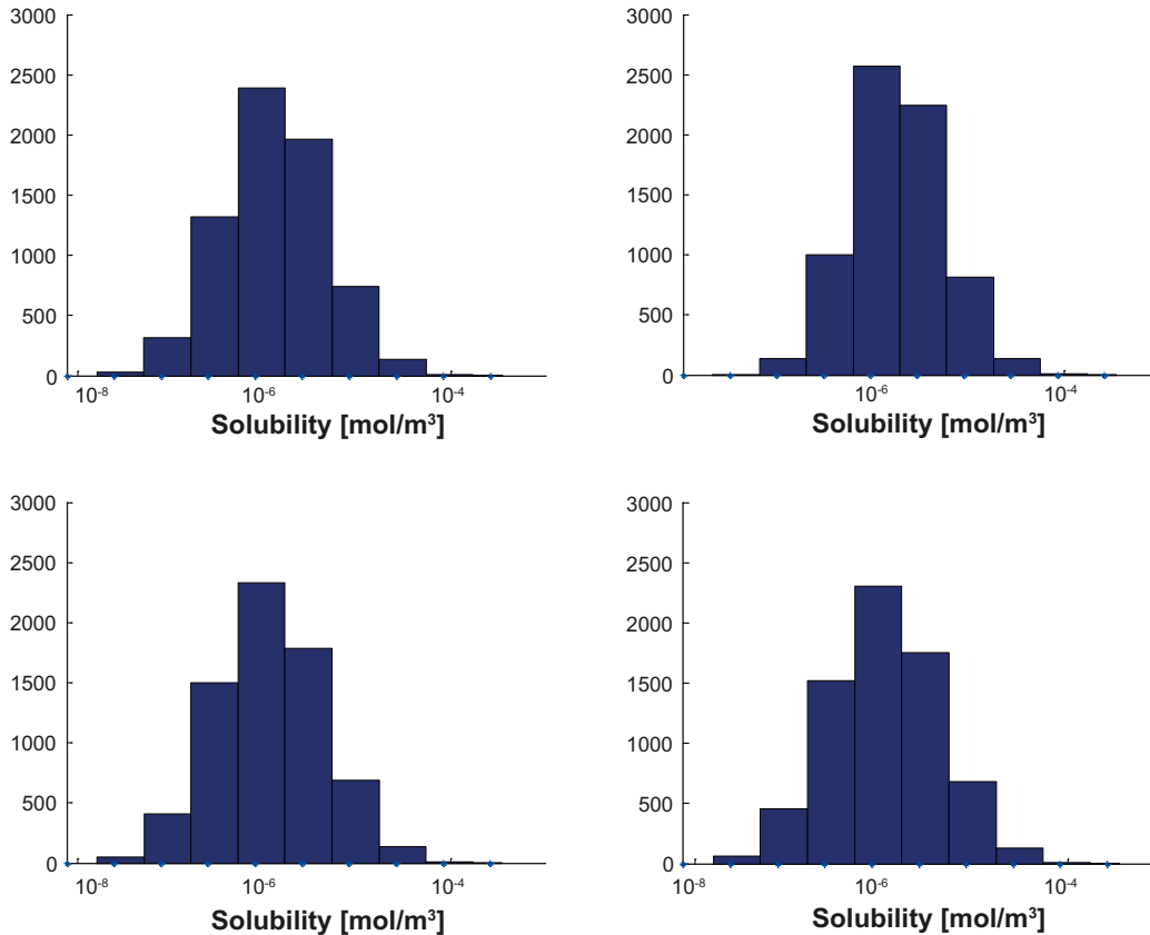
Figure F-1. Solubility limits for Np using groundwater data from temperate conditions (upper left), permafrost conditions (upper right), glacial conditions (lower left) and submerged conditions (lower right). The y-axis shows the number of realisations in each bin.
