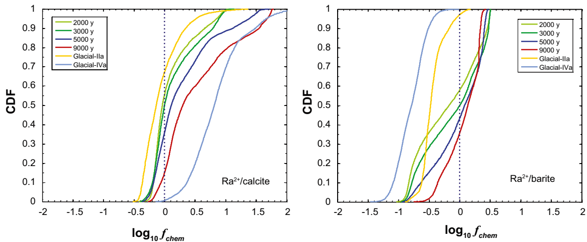
Figure B-9. Estimated groundwater chemistry correction factors ( f_{chem} ) for calcite (left) and barite (right) solid solutions relative to the reference groundwater used in the scoping calculations. Data are plotted as a cumulative distribution function (CDF) for groundwater compositions at different times during repository evolution. The correction factor for Ra^{2+} in both figures is calculated using Equation B-23. The vertical broken line indicates the relative location of the reference groundwater composition (i.e. median Ca^{2+} or Ba^{2+} concentration at 3,000 y).
