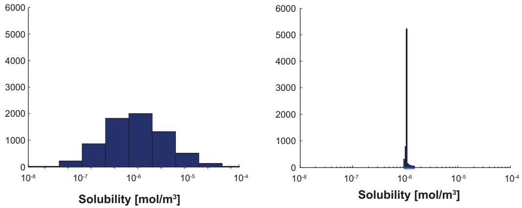
Figure F-9. Solubility limits for Np using groundwater data from temperate conditions. Fixed groundwater composition and varying thermodynamic data (left). Varying groundwater composition and fixed thermodynamic data (right). The y-axis shows the number of realisations in each bin.
