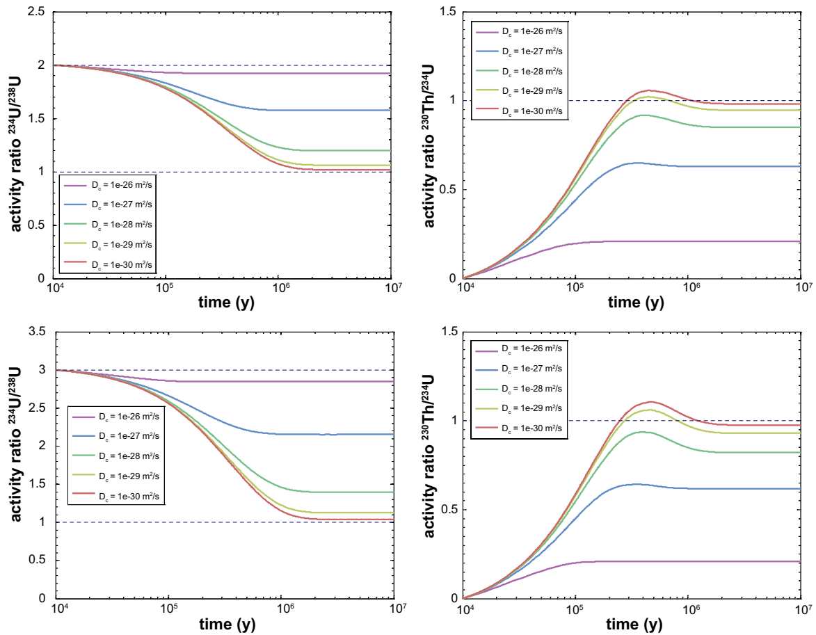
Figure B-13. Evolution of ^{234}\text{U}/^{238}\text{U} (left) and ^{230}\text{Th}/^{234}\text{U} (right) disequilibrium as a function of time for different solid state diffusivities in the range of 10^{-26} \text{m}^2/\text{s} to 10^{-30} \text{m}^2/\text{s} and for a constant groundwater ^{234}\text{U}/^{238}\text{U} activity ratio of 2 (top) and 3 (bottom) indicated by the upper broken line in each of the plots on the left-hand side. Calculations assume a calcite crystal with an accessible diffusion depth of 0.17 \mu\text{m} . A steady-state is typically achieved after roughly 2 Ma although not necessarily corresponding to secular equilibrium (activity ratio = 1 indicated by the lower broken line). Secular equilibrium is only achieved for very low solid-state diffusivities ( < 10^{-30} \text{m}^2/\text{s} ).
