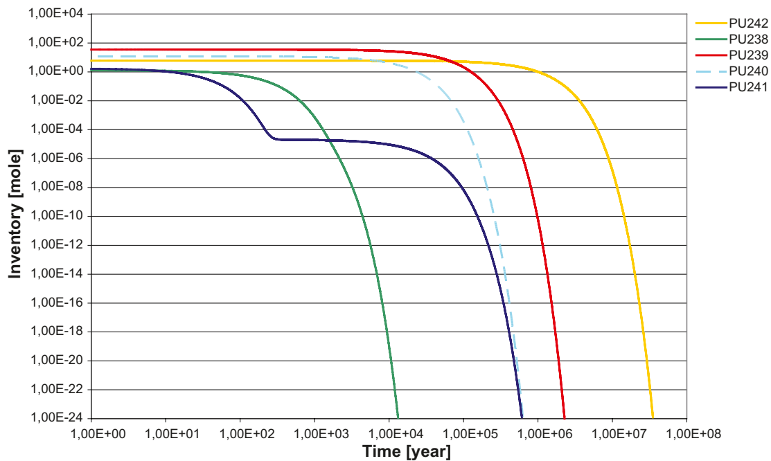
Figure D-20. Inventory (mole/canister) of plutonium isotopes.
