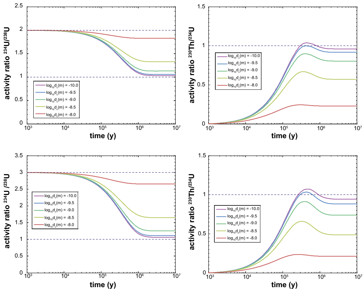
Figure B-20. Evolution of ^{234}\text{U}/^{238}\text{U} (left) and ^{230}\text{Th}/^{234}\text{U} (right) disequilibrium as a function of time for different surface entrapment zone widths in the range of 0.1 nm to 10 nm and for a constant groundwater ^{234}\text{U}/^{238}\text{U} activity ratio of 2 (top) and 3 (bottom) indicated by the upper broken line in each of the plots on the left-hand side. Calculations assume a calcite crystal with an accessible diffusion depth of 0.17 \mu\text{m} . A steady-state is typically achieved after roughly 2 Ma although not necessarily corresponding to secular equilibrium (activity ratio = 1 indicated by the lower broken line). Secular equilibrium is only achieved for very low surface entrapment zone widths ( d_c \sim 0.1 nm).
