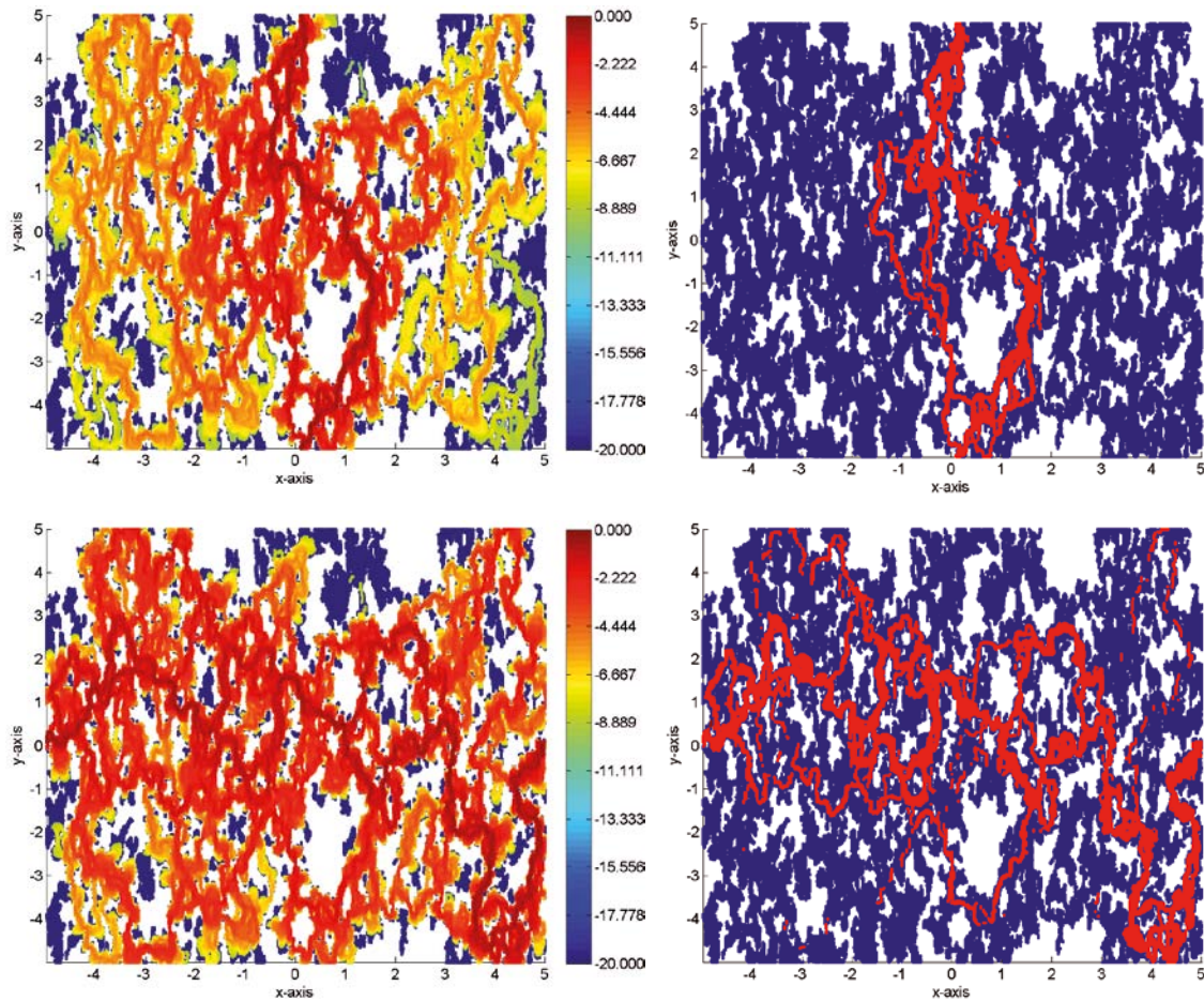
Figure A-1. Example of typical dynamic flow channels arising in a self-affine, variable aperture fracture with a surface asperity contact fraction of 40% and hydraulic gradient applied vertically (top) and horizontally (bottom) for a simple line source/sink dipole boundary condition of limited extent. Hydraulically inaccessible regions of the fracture are non-coloured. The left-hand images indicate the flow magnitude normalised with respect to the maximum flowrate ( \log_{10} units). The right-hand images show flow channels featuring flow > 1\% (arithmetic units) of the maximum flowrate highlighted in red.
