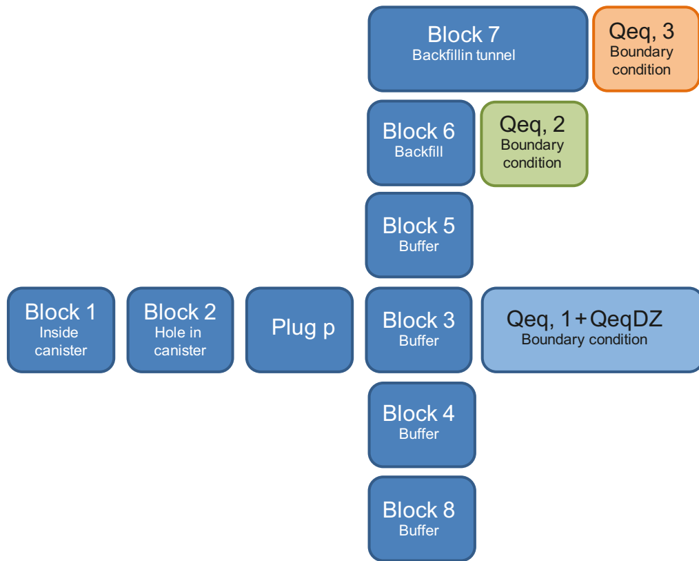
Figure G-5. Schematic picture of the blocks, plugs and boundary conditions in the case with growing pinhole failure including the effect of spalling.
