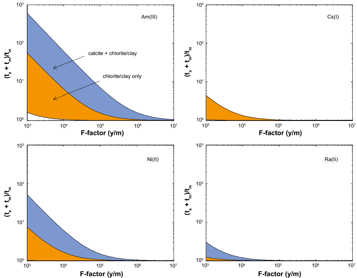
Figure B-5. Estimated relative enhancement ( \chi as defined by Equation B-30 plotted versus F-factor) of retardation effect for Am(III), Cs(I), Ni(II), and Ra(II) owing to equilibrium sorption on fracture minerals. Calculations assume a mix of chlorite, assorted clay minerals, and calcite where sorptivity is assumed to be linearly additive. Sorption on chlorite and clay minerals is assumed to occur by way of ion-exchange and surface complexation. Sorption in association with calcite is modelled assuming solid solution formation and a Henry law partitioning mechanism. Orange shaded regions indicate the retardation effect of chlorite and clay minerals only where the coloured region represents the approximate range of uncertainty. Blue shaded regions indicate the additional retardation effect potentially achievable if calcite forms a solid solution.
