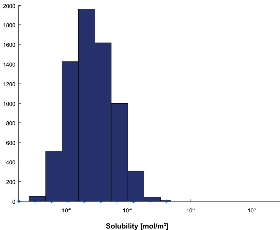
Figure F-34. Solubility limits for Th used as input data for COMP23 in SR-Site. The y-axis shows the number of realisations in each bin.
