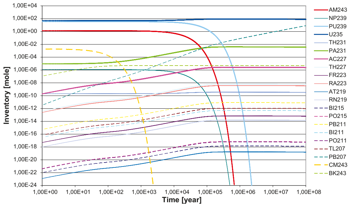
Figure D-18. Radionuclide content (mol/canister) as a function of time for radionuclides in chain 4n+3. Initial inventory from /Håkansson 2000/.
