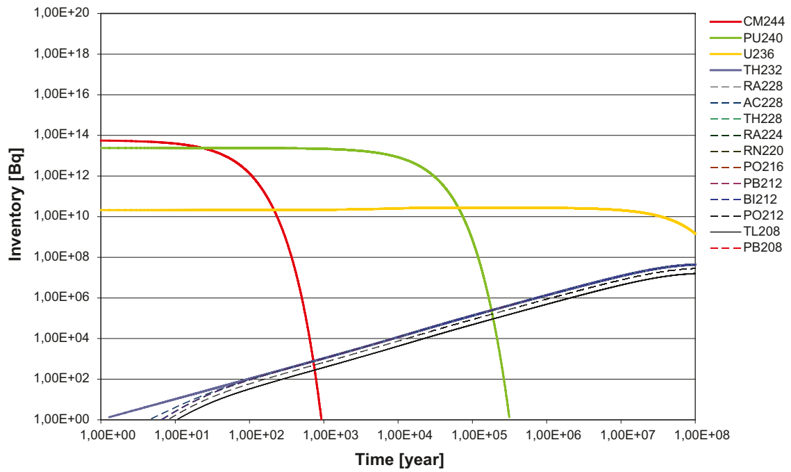
Figure D-5. Activity (Bq/tU) as a function of time for radionuclides in the 4n chain. Initial inventory from /Håkansson 2000/.
