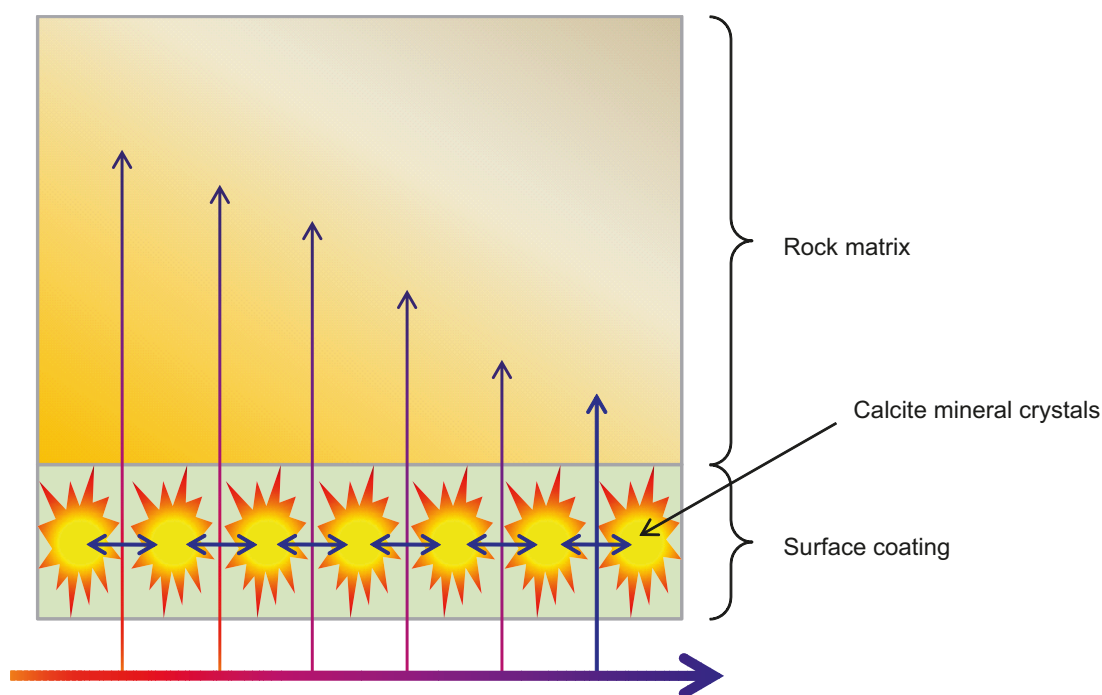
Figure B-12. Illustration of transport problem where diffusive uptake to solid solution forming surface minerals (principally calcite) is considered as a parallel retardation sink for migrating radionuclides. The arrows indicate the notional direction of solute flux in the system.
