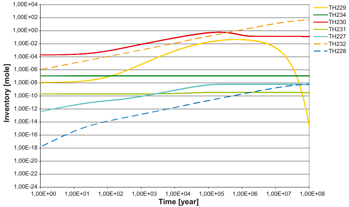
Figure D-21. Inventory (mole/canister) of thorium isotopes.
