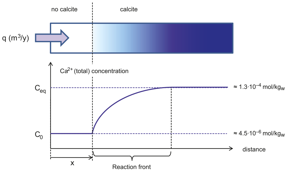
Figure B-10. Illustration of calcite mobilisation process for a flowpath where infiltrating dilute, glacial groundwater (with concentration, C_0 ) dissolves calcite. The dissolution products eventually reach their equilibrium concentration ( C_{eq} ) over a distance determined by the particular chemical kinetics of the dissolution reaction (and diffusion kinetics), the reactive surface area, and advective travel time. The transient concentration region separating the initial and equilibrium states is referred to as the reaction front.
