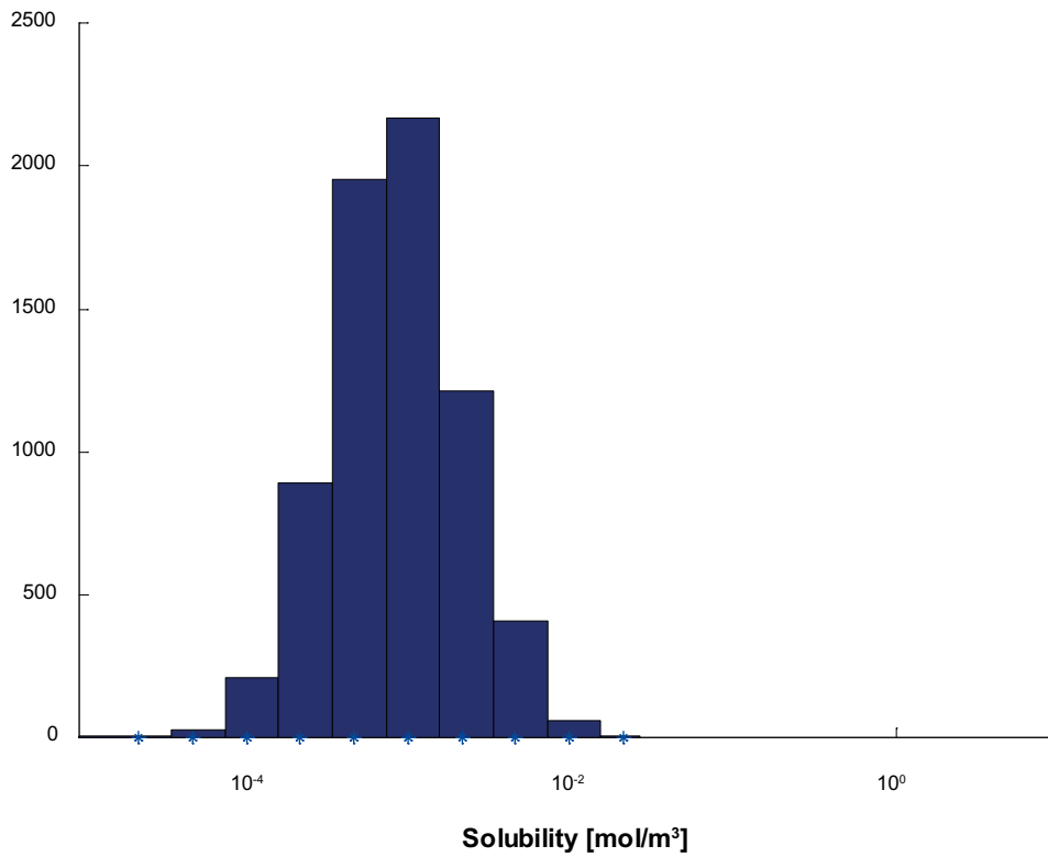
Figure F-25. Solubility limits for Pb used as input data for COMP23 in SR-Site. The y-axis shows the number of realisations in each bin.
