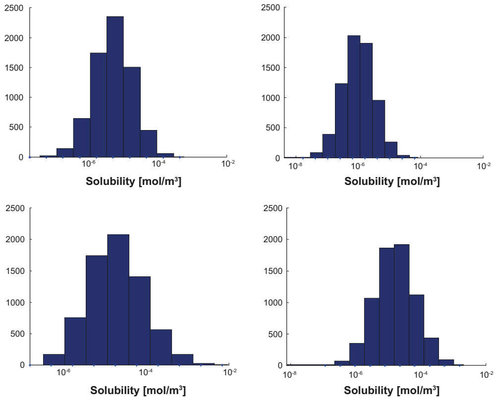
Figure F-5. Solubility limits for Se using groundwater data from temperate conditions (upper left), permafrost conditions (upper right), glacial conditions (lower left) and submerged conditions (lower right). The y-axis shows the number of realisations in each bin.
