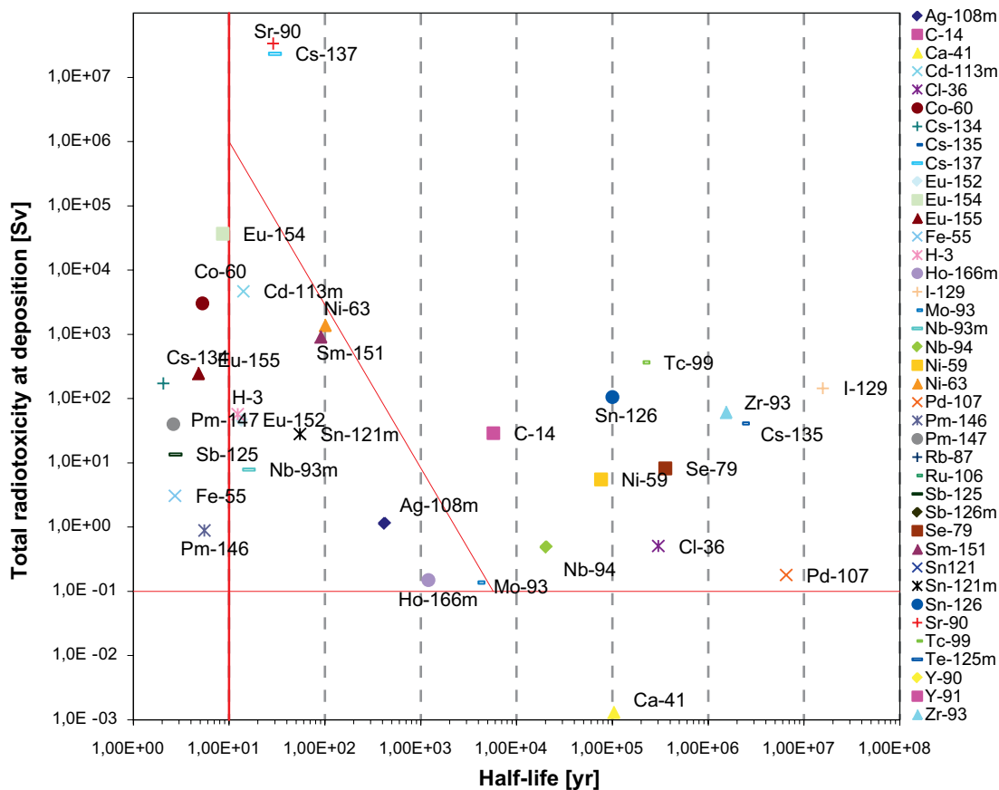
Figure D-1. Radiotoxicity as a function of half-life for all fission and activation products in the spent fuel. All nuclides considered are shown in the list to the right, whereas only some of them has a sufficiently long half-life and a sufficiently high radiotoxicity to appear in the plot.
