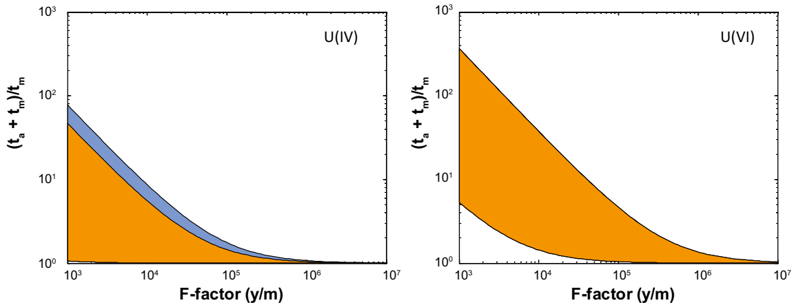
Figure B-6. Estimated relative enhancement ( \chi as defined by Equation B-30 plotted versus F-factor) of retardation effect for U(IV) and U(VI) owing to equilibrium sorption on fracture minerals. Calculations assume a mix of chlorite, assorted clay minerals, and calcite where sorptivity is assumed to be linearly additive. Sorption on chlorite and clay minerals is assumed to occur by way of ion-exchange and surface complexation. Sorption in association with calcite is modelled assuming solid solution formation and a Henry law partitioning mechanism. Orange shaded regions indicate the retardation effect of chlorite and clay minerals only where the coloured region represents the approximate range of uncertainty. Blue shaded regions indicate the additional retardation effect potentially achievable if calcite forms a solid solution.
