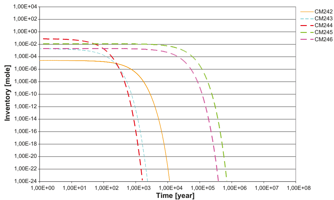
Figure D-23. Inventory (mole/canister) of curium isotopes.
