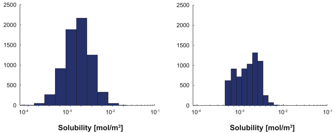
Figure F-10. Solubility limits for Pb using groundwater data from temperate conditions. Fixed groundwater composition and varying thermodynamic data (left). Varying groundwater composition and fixed thermodynamic data (right). The y-axis shows the number of realisations in each bin.
