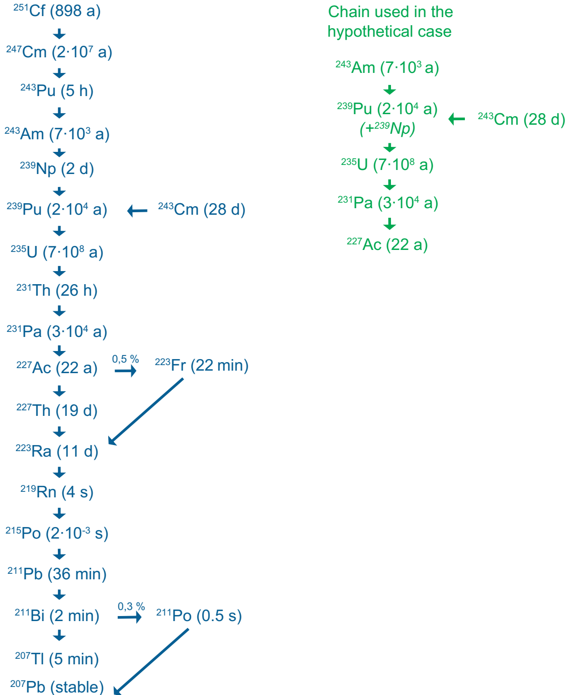
Figure D-15. Chain 4N+3. The simplified chain is used in the hypothetical case to support the selection of radionuclides for the radionuclide transport calculations. Nuclides in the beginning of the chain without any inventory have been excluded in the simplified chain as have nuclides with a half-life shorter than 1 year, but their inventories have been added to their daughter's inventory. Approximate half-lives shown are derived from Table D-4.
