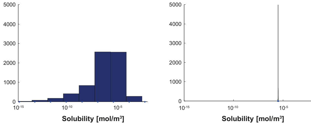
Figure F-15. Solubility limits for U using groundwater data from temperate conditions. Fixed groundwater composition and varying thermodynamic data (left). Varying groundwater composition and fixed thermodynamic data (right). The y-axis shows the number of realisations in each bin.
