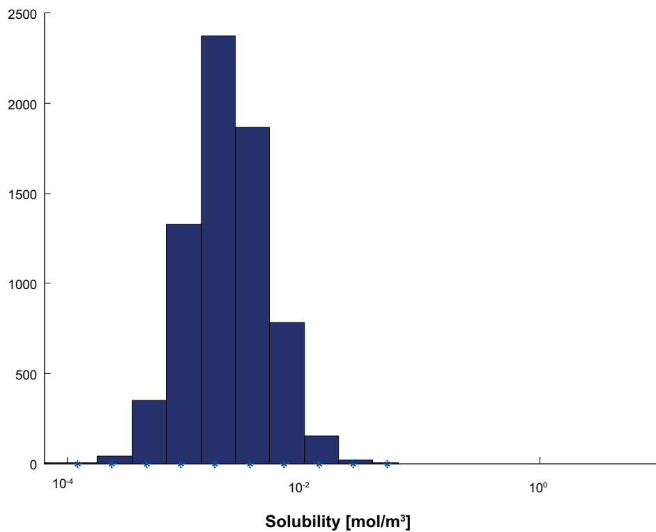
Figure F-20. Solubility limits for Ho used as input data for COMP23 in SR-Site. The y-axis shows the number of realisations in each bin.
