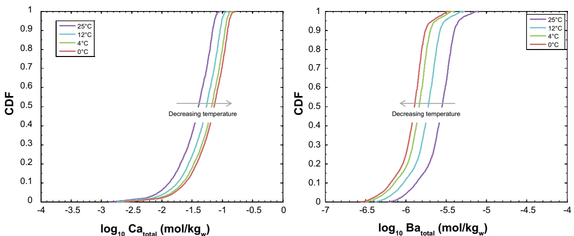
Figure B-4. Effect of temperature on calcite ( \text{Ca}^{2+} ) and barite ( \text{Ba}^{2+} ) equilibrium for the glacial IIa case plotted as a cumulative distribution function (CDF) for different temperatures in the range 0^\circ\text{C} to 25^\circ\text{C} . Calculations assume simultaneous barite/calcite equilibrium re-estimated for the groundwater compositional ranges initially calculated by /Salas et al. 2010/. The data show an increase in solubility of calcite and decrease in solubility of barite with decreasing temperature as expected.
