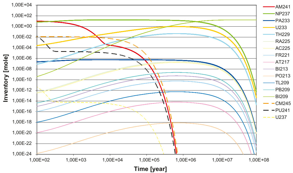
Figure D-10. Radionuclide content (mol/canister) as a function of time for radionuclides in chain 4N+1. Initial inventory from /Håkansson 2000/.
