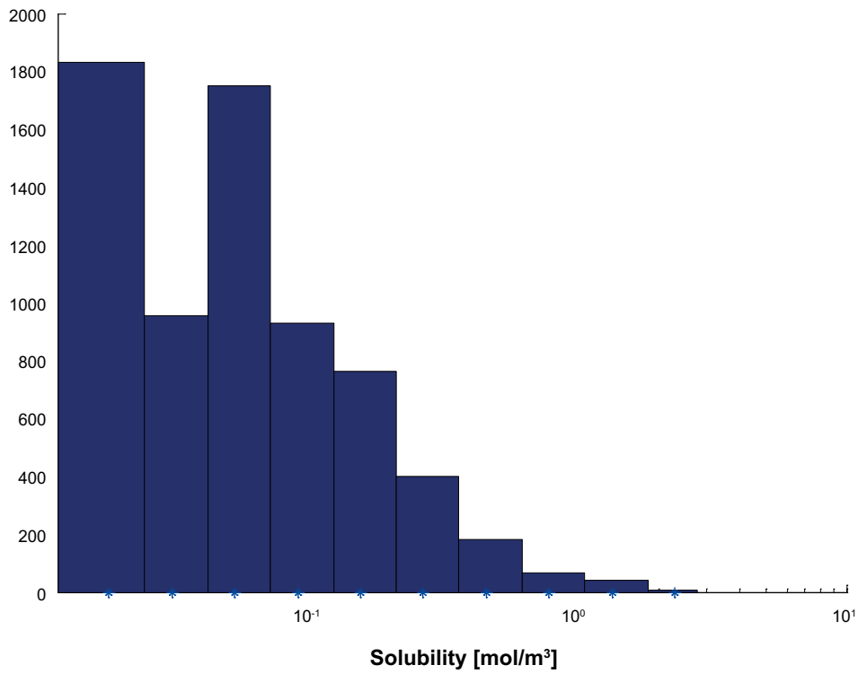
Figure F-21. Solubility limits for Nb used as input data for COMP23 in SR-Site. The y-axis shows the number of realisations in each bin.
