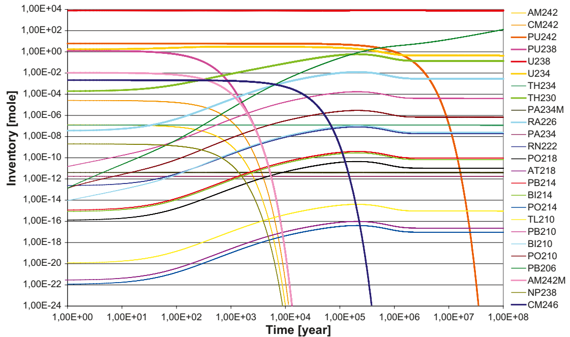
Figure D-14. Radionuclide content (mol/canister) as a function of time for radionuclides in chain 4N+2. Initial inventory from /Håkansson 2000/.
