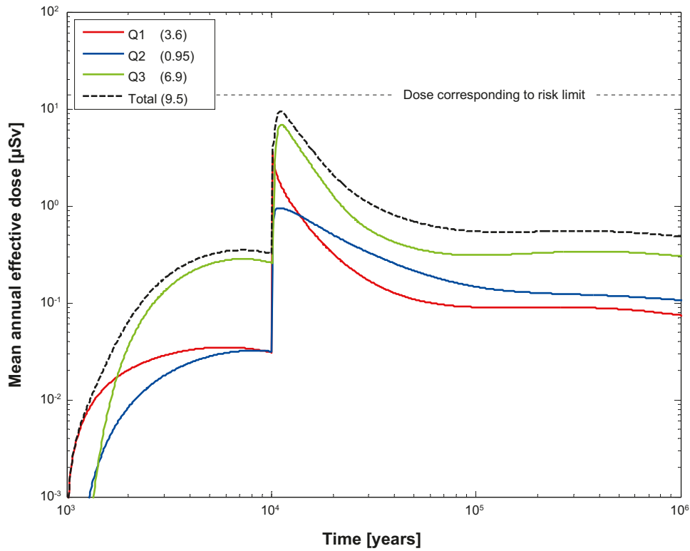
Figure 6-32. Near-field dose equivalent release for the probabilistic calculation of the pinhole case, with lost swelling pressure in tunnel backfill. Doses decomposed into Q1 , Q2 and Q3 . The legend is sorted by peak (in the one-million year period) of the mean annual effective dose. The values in brackets are peak dose in units of \mu\text{Sv} .
