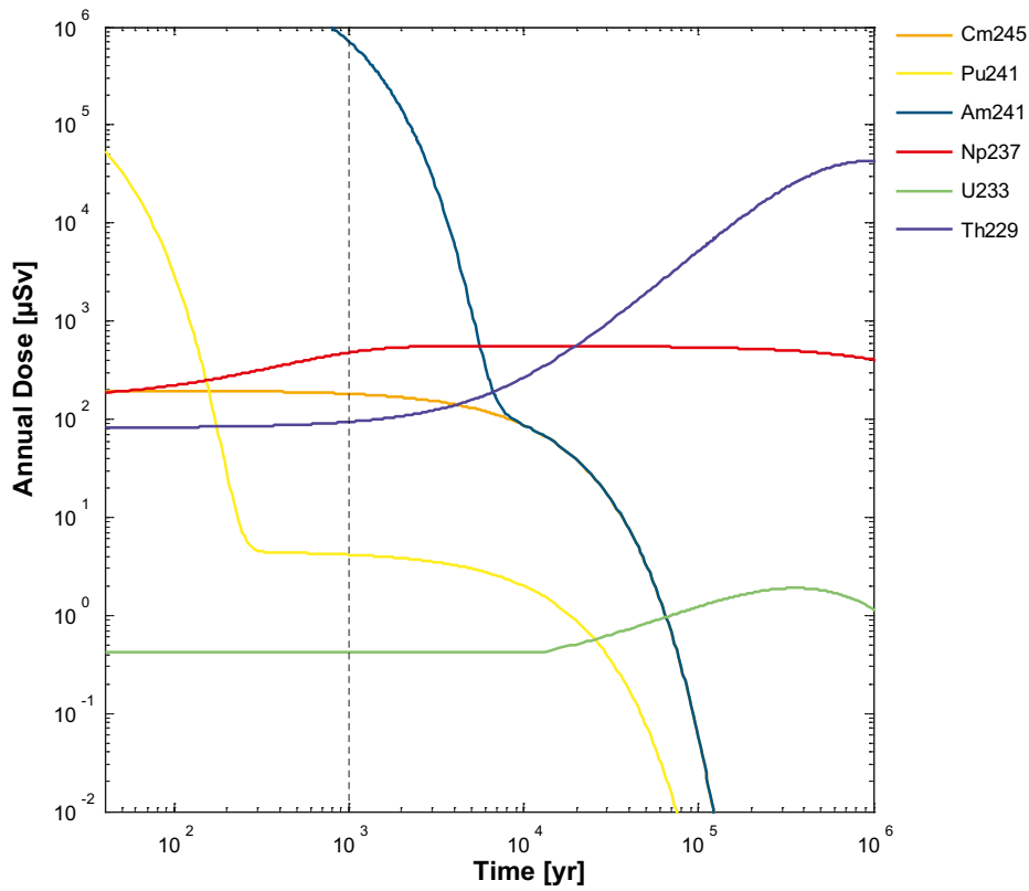
Figure D-8. Calculated annual dose in the hypothetical case supporting the selection of radionuclides for the radionuclide transport calculations of 4n+1 chain. The vertical black dashed line denotes 1,000 years after closure.
