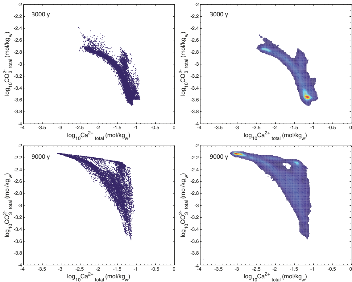
Figure B-2. Groundwater compositional data (total carbonate vs. total calcium) visualised in scatterplot form (left) and in the form of a smoothed 2D histogram (right) for the temperate 3,000 y and 9,000 y epochs. Warmer colours in the histogram plots correspond to a greater frequency of the indicated composition.
