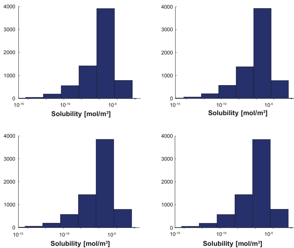
Figure F-7. Solubility limits for U using groundwater data from temperate conditions (upper left), permafrost conditions (upper right), glacial conditions (lower left) and submerged conditions (lower right). The y-axis shows the number of realisations in each bin.
