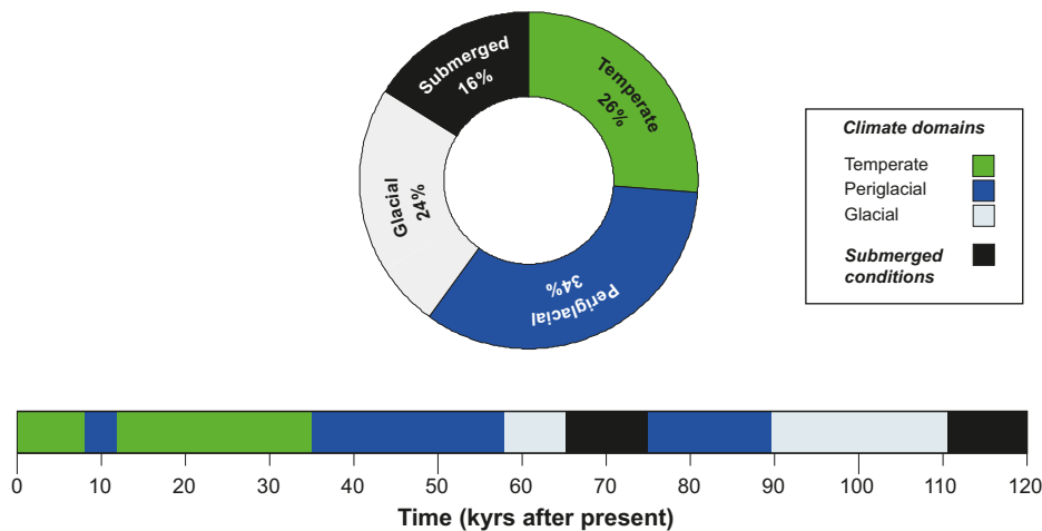
Figure 2-1. Simplified glacial cycle for use in the geosphere transport assessment /Climate report/.
