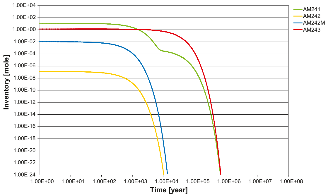
Figure D-22. Inventory (mole/canister) of americium isotopes.
