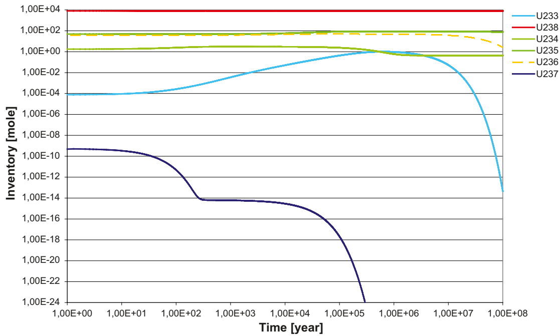
Figure D-19. Inventory (mole/canister) of uranium isotopes.
