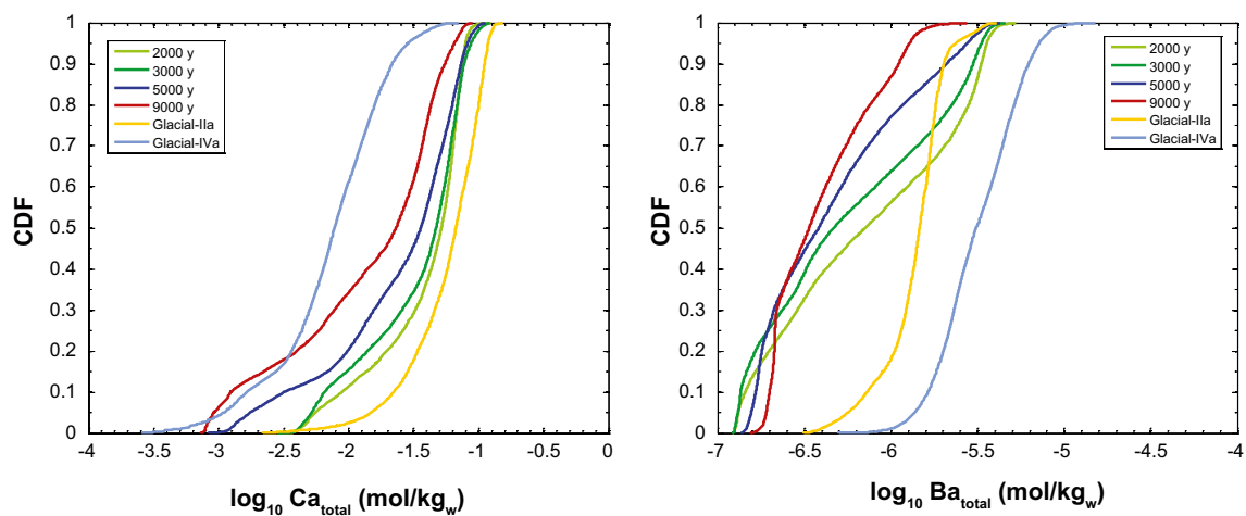
Figure B-3. Total concentration of \text{Ca}^{2+} and \text{Ba}^{2+} plotted as a cumulative distribution function (CDF) for groundwater compositions at different times during repository evolution. Calculations assume simultaneous barite/calcite equilibrium re-estimated for the groundwater compositional ranges initially calculated by /Salas et al. 2010/. An average temperature of 12°C is assumed for the temperate groundwaters and 4°C for the glacial IIa and IVa groundwaters.
