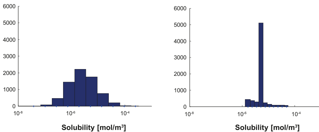
Figure F-14. Solubility limits for Th using groundwater data from temperate conditions. Fixed groundwater composition and varying thermodynamic data (left). Varying groundwater composition and fixed thermodynamic data (right). The y-axis shows the number of realisations in each bin.
