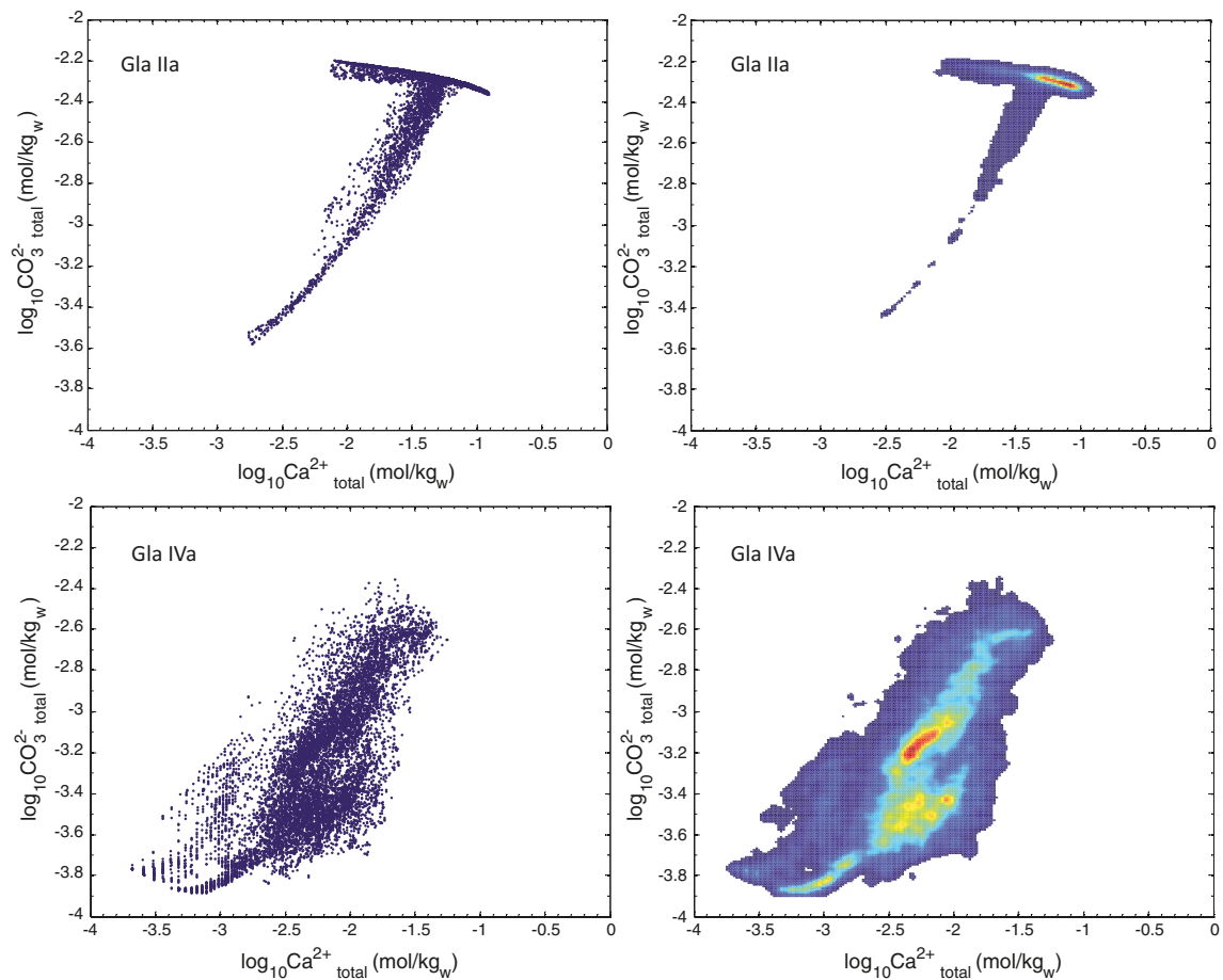
Figure B-1. Groundwater compositional data (total carbonate vs. total calcium) visualised in scatterplot form (left) and in the form of a smoothed 2D histogram (right) for the glacial IIa and IVa epochs. Warmer colours in the histograms correspond to a greater frequency of the indicated composition. Aliasing in the lower left hand figure is due to round-off errors owing to the number of significant figures in the data sets calculated by /Salas et al. 2010/.
