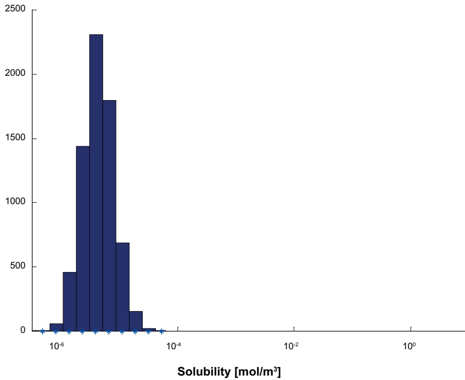
Figure F-33. Solubility limits for Tc used as input data for COMP23 in SR-Site. The y-axis shows the number of realisations in each bin.
