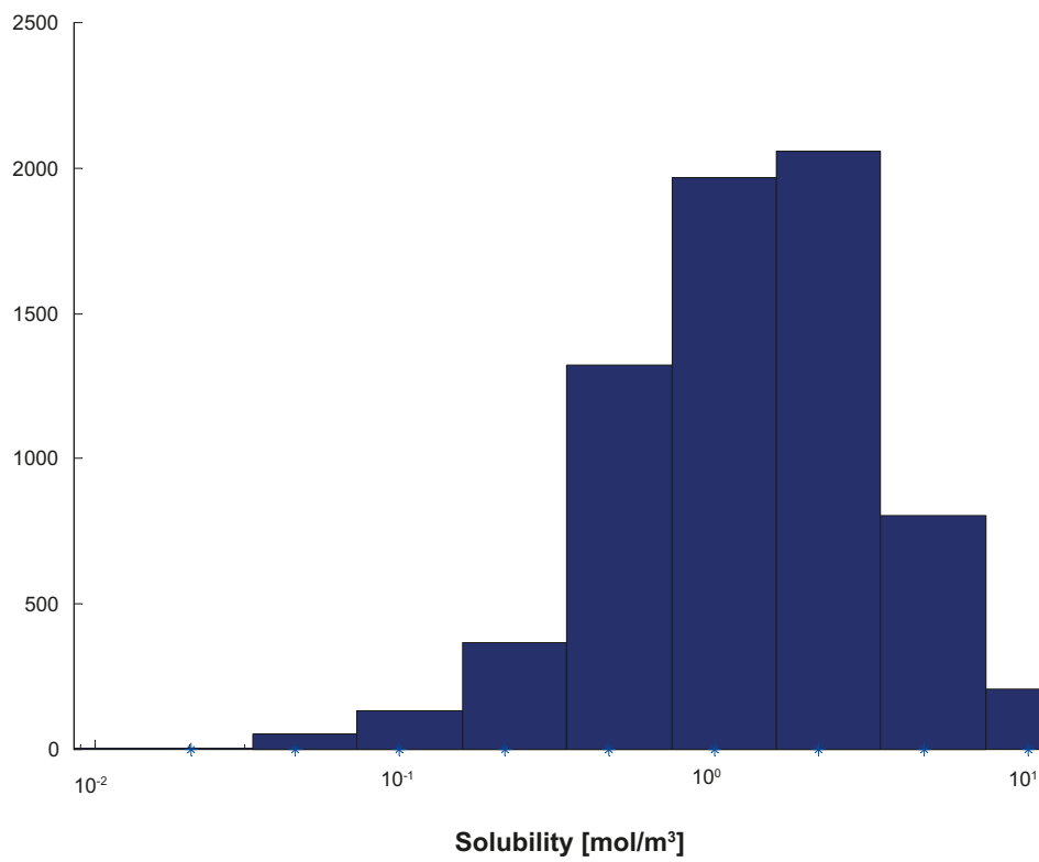
Figure F-32. Solubility limits for Sr used as input data for COMP23 in SR-Site. The y-axis shows the number of realisations in each bin.
