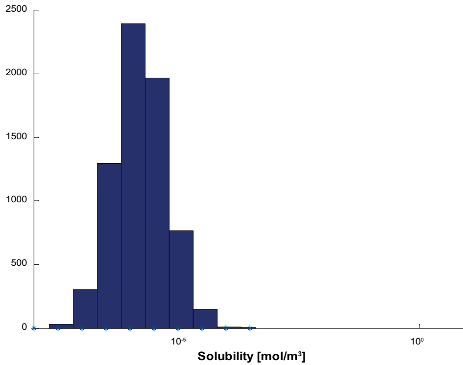
Figure F-23. Solubility limits for Np used as input data for COMP23 in SR-Site. The y-axis shows the number of realisations in each bin.
