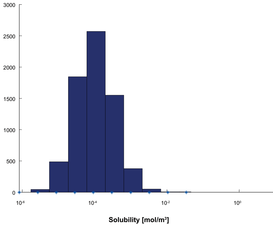
Figure F-31. Solubility limits for Sn used as input data for COMP23 in SR-Site. The y-axis shows the number of realisations in each bin.
