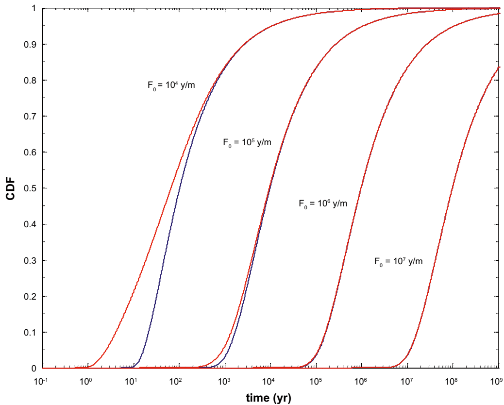
Figure A-8. Residence time distribution for a weakly sorbing solute ( K_d = 0.001 \text{ m}^3/\text{kg} ) for the simplified channeling scenario (red curves, Case 2) as compared to the reference scenario (blue curves, Case 1). Results are shown as a cumulative probability density function (CDF) for different reference case F -factors as indicated.
