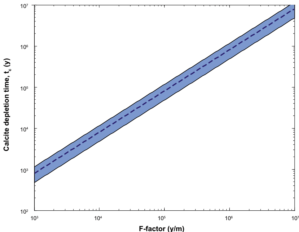
Figure B-11. Time to deplete calcite from an advective flowpath as a function of F-factor. Calculations assume estimated specific mass of calcite given in Table B-2 and only calcite residing along the main flowpath. The shaded region represents the minimum-maximum range and the broken line is the best estimate. Additional calcite buffering capacity may reside in stagnant zones of the fracture or in partially annealed sections flanking the flowpath.
