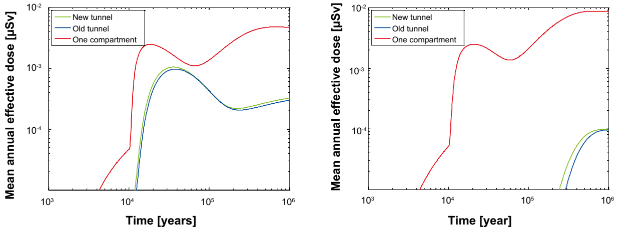
Figure G-10. Comparison between the tunnel discretisation used in SR-Can and SR-Site for two different path lengths (10.1 m to the left and 93.5 m to the right). In addition results for a calculation with one single compartment are shown.
