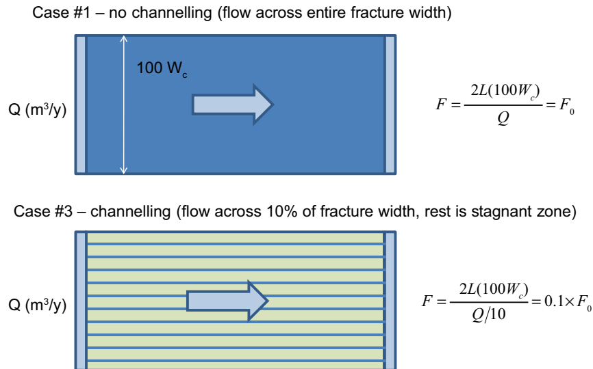
Figure A-5. Idealised example of 10 flow channels of width W_c equal to 1% of the fracture width hosted in a fracture of length L (Case 3 – bottom) as compared with the null case of a fracture where flow contacts the entire surface (Case 1 – top). Case 3 approximately corresponds to the F -factor scaling assumption used previously in SR-Can /SKB 2006/.
