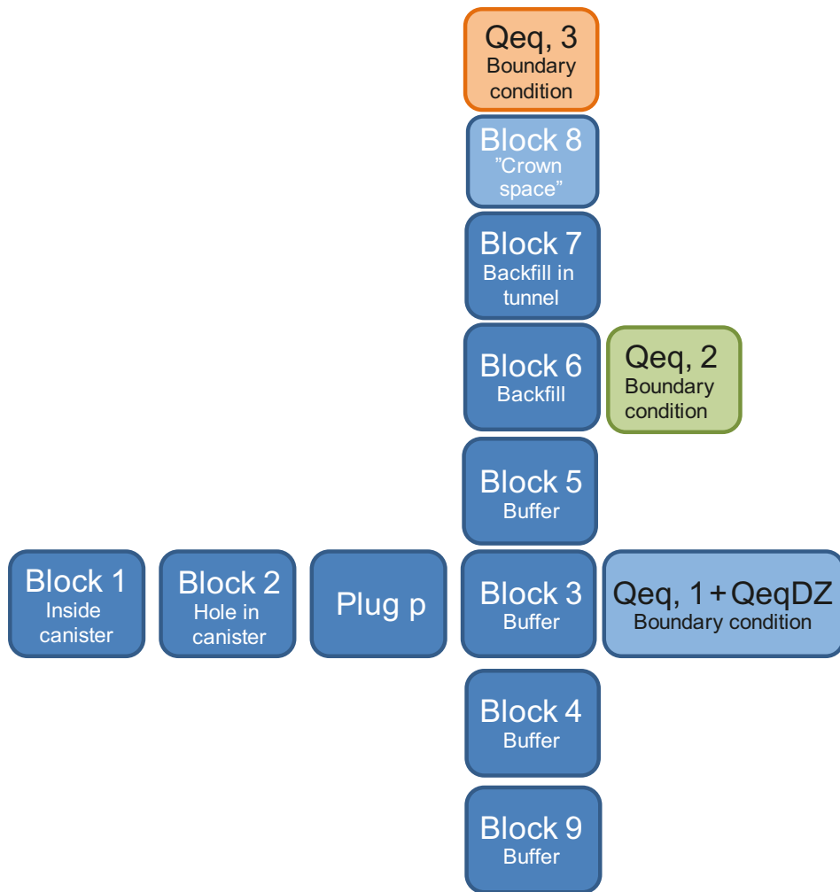
Figure G-6. Schematic picture of the blocks, plugs and boundary conditions in the case with lost swelling pressure in the backfill in the tunnel.
