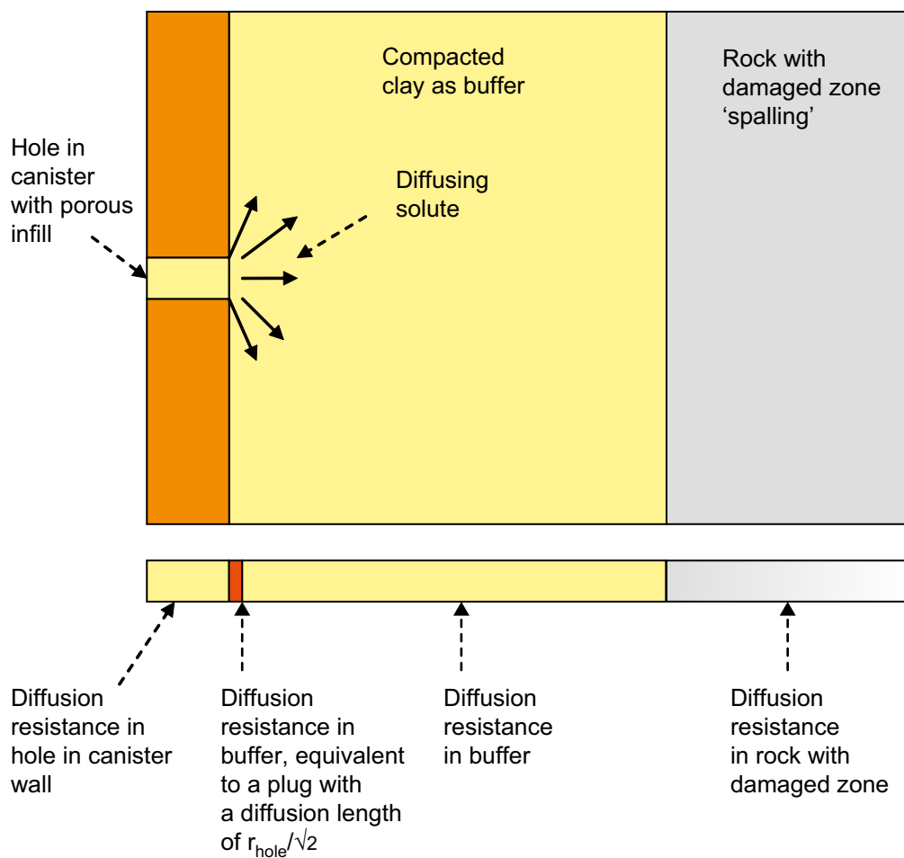
Figure G-4. Transport from a defect canister through the buffer and into the damaged zone in the case with growing pinhole failure including the effect of spalling (modified from Neretnieks 2006/).
