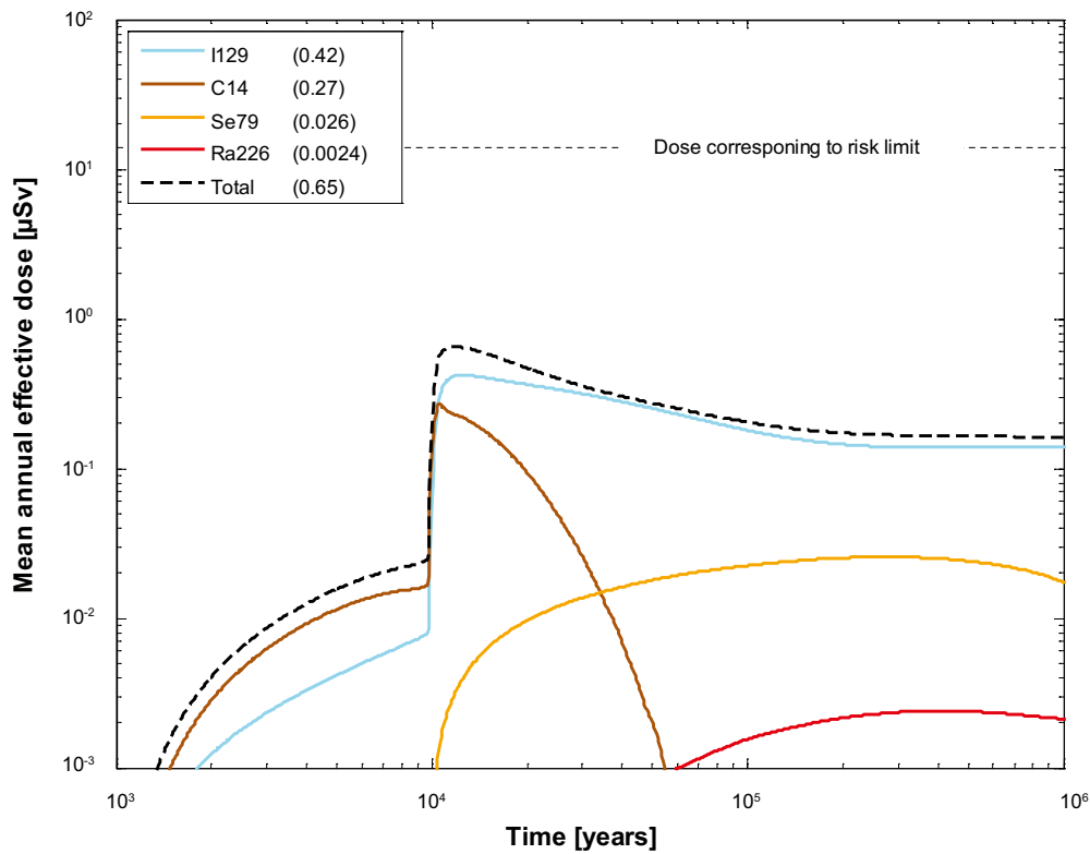
Figure 6-17. Far-field mean annual mean effective dose for the probabilistic calculation of the pinhole case, including the effect of spalling. Summed doses for all release paths ( Q1+Q2+Q3 ). The legend is sorted by peak (in the one-million year period) of the mean annual effective dose. The values in brackets are peak dose in units of \mu\text{Sv} .
