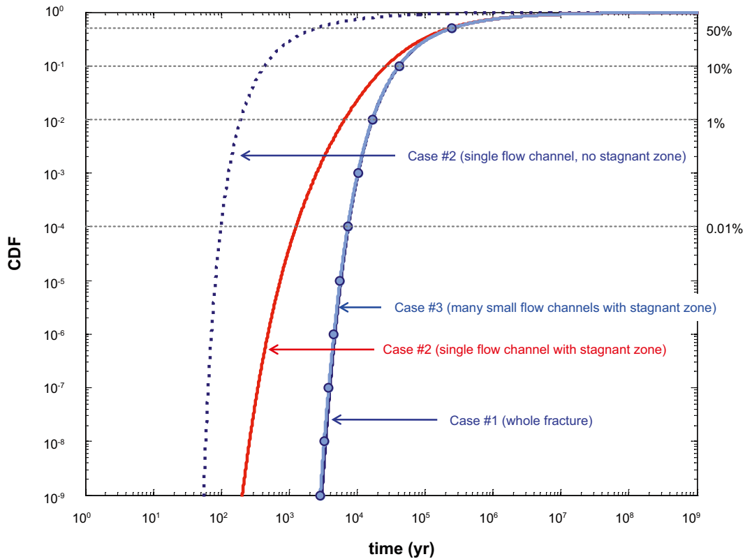
Figure A-7. Same results as in the previous Figure although plotted on a log-log axis. Different recovery fractions corresponding to 0.01% - 50% of released solute are also indicated by the horizontal broken lines for reference purposes.
