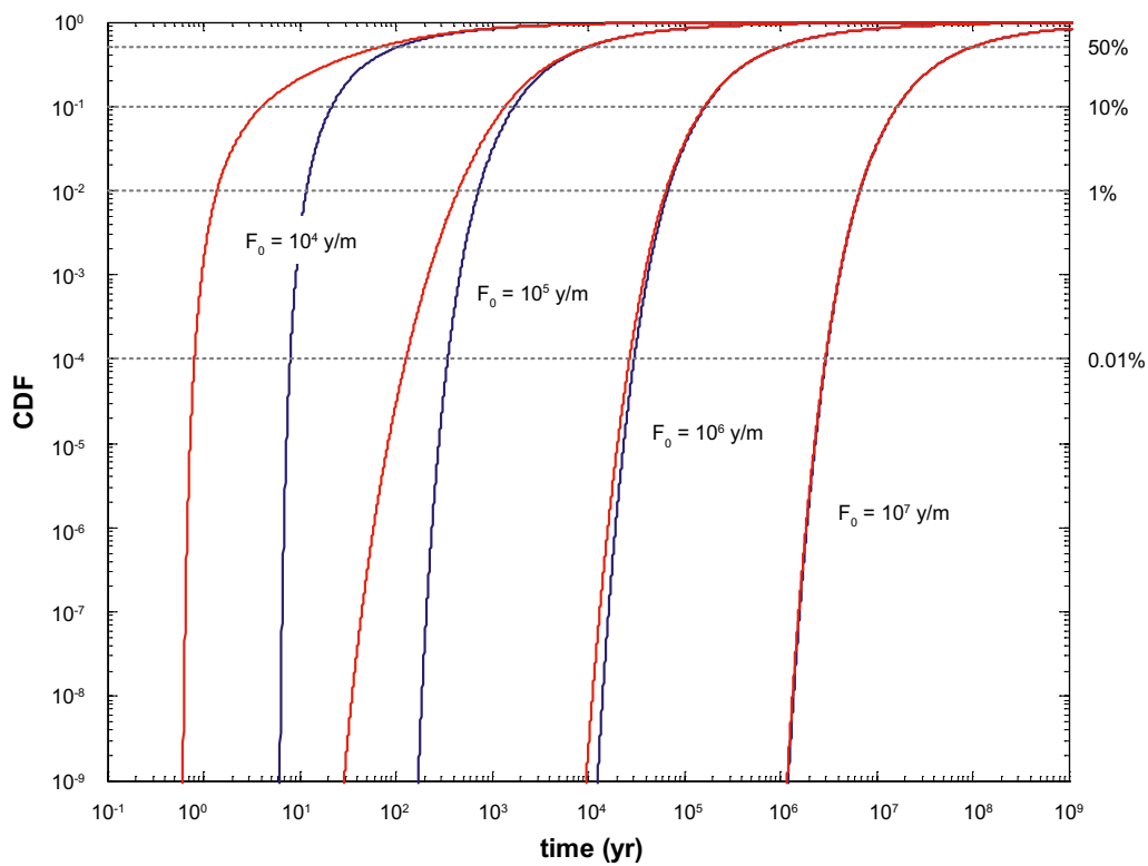
Figure A-9. Same results as in the previous Figure although plotted on a log-log axis. Different recovery fractions corresponding to 0.01% - 50% of released solute are also indicated by the horizontal broken lines for reference purposes.
