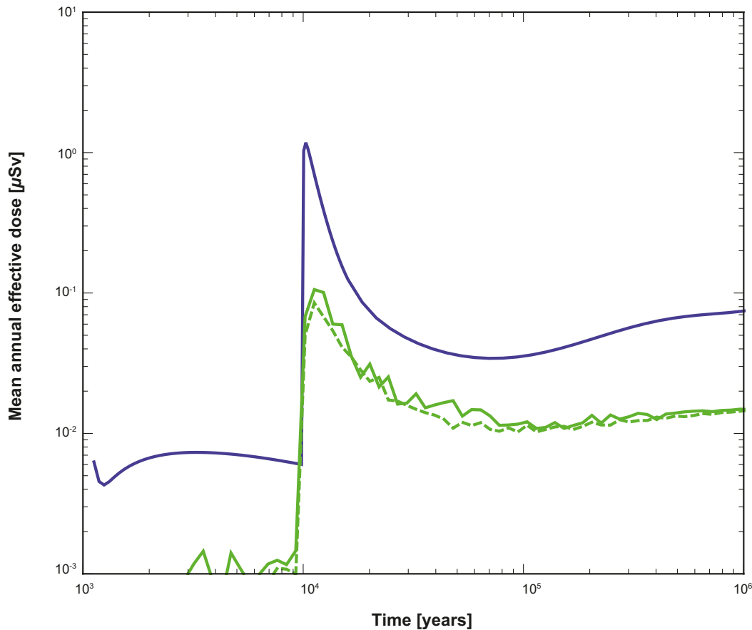
Figure 6-52. Effect of having multiple Q1 pathways per release point. The blue curve is near-field release. The solid green curve is the base case far-field release. The dashed green curve is the far-field release for the case with 10 pathways per release point.
