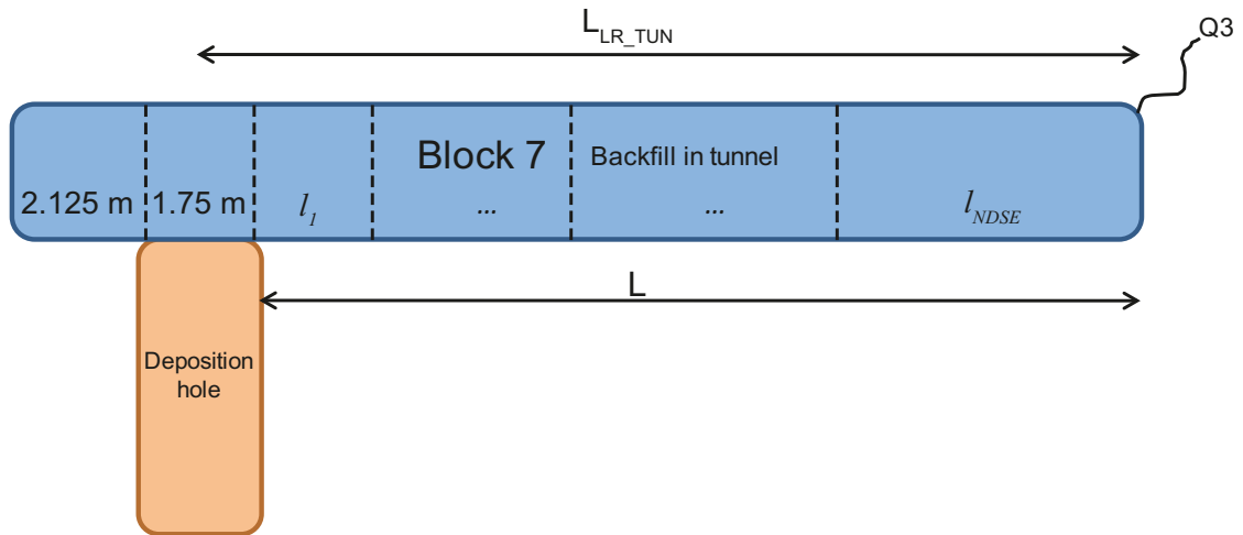
Figure G-9. Discretisation for the tunnel block, Block 7. The sink Q3 is located at the first fracture in the tunnel.
