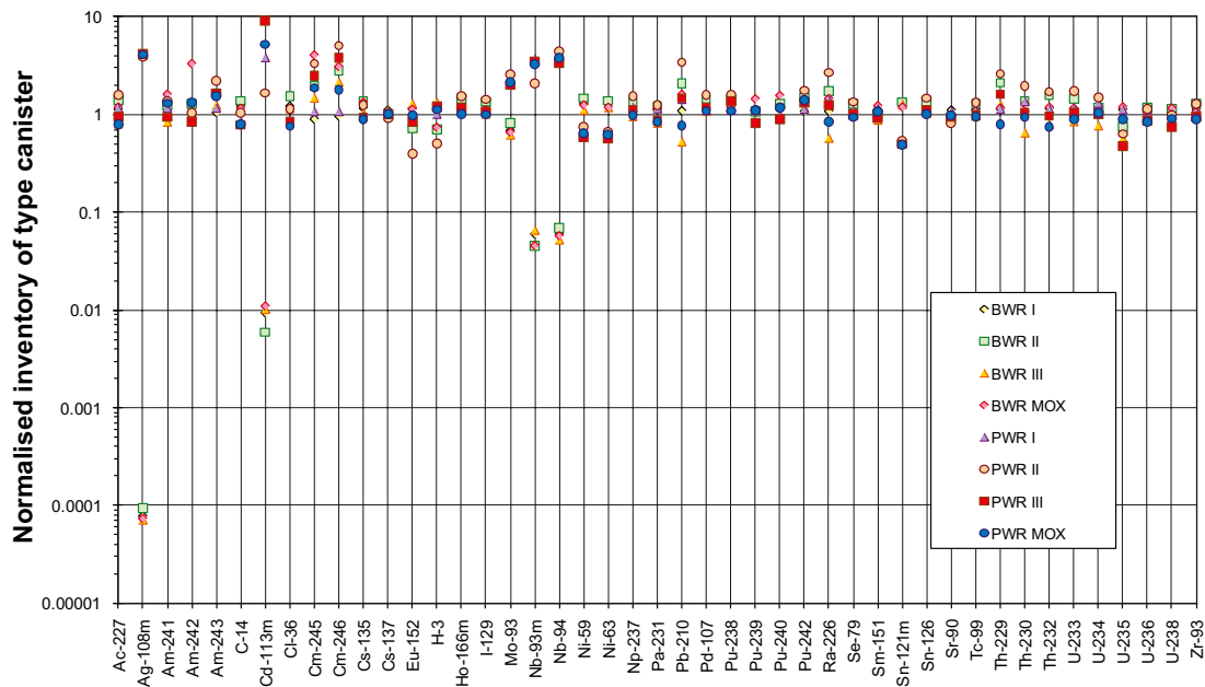
Figure E-1. Spread in data of inventory per type canister, as normalised with the inventory per average canister. All data taken from the Data report , i.e. data for the corrected inventory.
