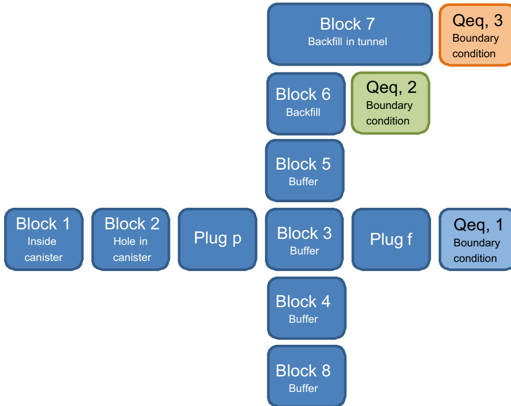
Figure G-2. Schematic picture of the blocks, plugs and boundary conditions in the case with growing pinhole failure without including the effect of spalling.
