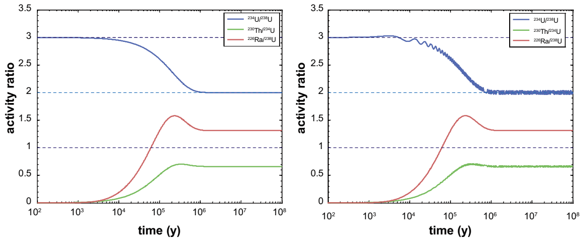
Figure B-15. Evolution of U-series disequilibrium as a function of time for a solid state diffusivity of 7 \cdot 10^{-28} \text{ m}^2/\text{s} and for a groundwater ^{234}\text{U}/^{238}\text{U} activity ratio varying in the range 2–4. The left-hand figure shows the result for a constant concentration boundary condition representing the average, while the right-hand figure shows the impact of a periodic variation in the activity ratio in the range 2–4 (although for constant groundwater ^{238}\text{U} activity). Calculations assume a calcite crystal with an accessible diffusion depth of 0.17 \text{ }\mu\text{m} as in previous calculations and an initial ^{234}\text{U}/^{238}\text{U} activity ratio of 3.
