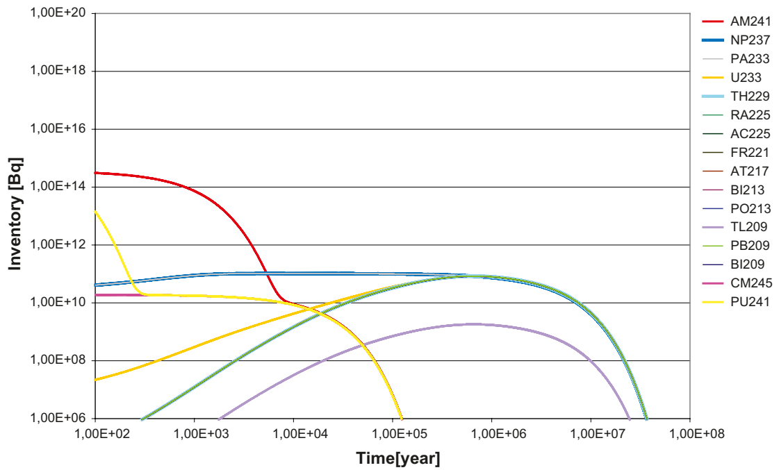
Figure D-9. Activity (Bq/tU) as a function of time for radionuclides in chain 4N+1. Initial inventory from /Håkansson 2000/.
