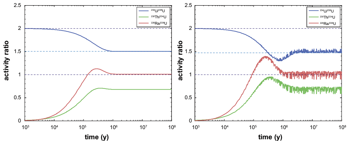
Figure B-14. Evolution of U-series disequilibrium as a function of time for a solid state diffusivity of 7 \cdot 10^{-28} \text{ m}^2/\text{s} and for a constant groundwater ^{234}\text{U}/^{238}\text{U} activity ratio of 2. The left-hand figure shows the result for a constant concentration boundary condition, while the right-hand figure shows the impact of a periodic variation in absolute U concentration (6 orders of magnitude variability with a period of 10 ka although constant ^{234}\text{U}/^{238}\text{U} activity ratio). Calculations assume a calcite crystal with an accessible diffusion depth of 0.17 \mu\text{m} as in previous calculations.
