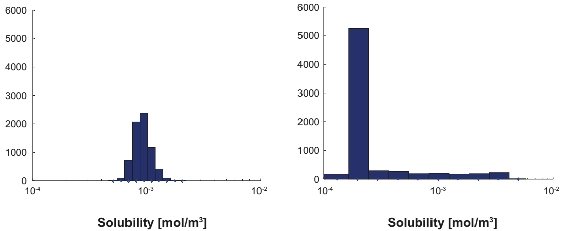
Figure F-12. Solubility limits for Ra using groundwater data from temperate conditions. Fixed groundwater composition and varying thermodynamic data (left). Varying groundwater composition and fixed thermodynamic data (right). The y-axis shows the number of realisations in each bin.
