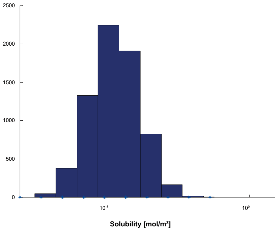
Figure F-36. Solubility limits for Zr used as input data for COMP23 in SR-Site. The y-axis shows the number of realisations in each bin.
