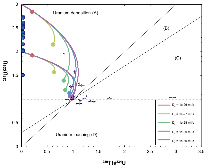
Figure B-17. Cross plot of ^{234}\text{U}/^{238}\text{U} vs. ^{230}\text{Th}/^{234}\text{U} activity ratio in the manner described by /Thiel et al. 1983/. Secular equilibrium corresponds to the intersection of the vertical and horizontal broken lines at an activity ratio of unity. The upper (A) and lower (D) sectors correspond to U deposition and leaching, respectively. Sector (B) is the forbidden sector for any single continuous process, while sector (C) is the forbidden sector for any single process. Small markers with error bars indicate measured values for Forsmark fracture minerals (data taken from /Sandström et al. 2008/) while blue markers along the vertical axis indicate approximate range of ^{234}\text{U}/^{238}\text{U} activity ratios in contemporary groundwater at Forsmark /Laaksoharju et al. 2008/. Endpoint markers of simulated curves indicate the steady state condition for the particular solid state diffusivity modelled.
