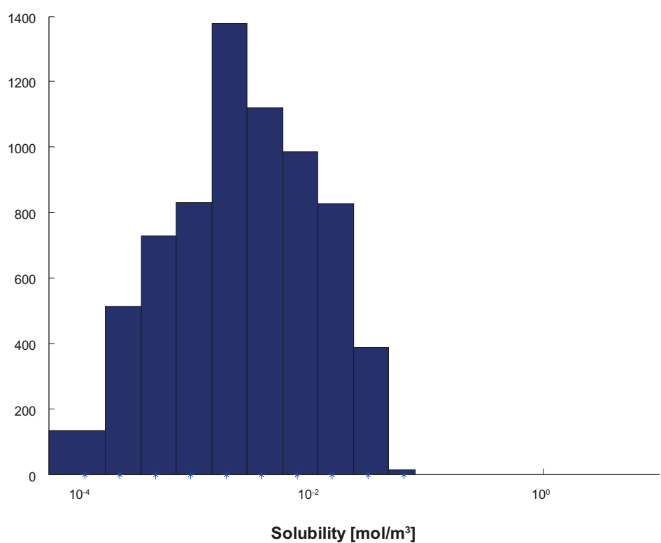
Figure F-28. Solubility limits for Ra used as input data for COMP23 in SR-Site. The y-axis shows the number of realisations in each bin.
