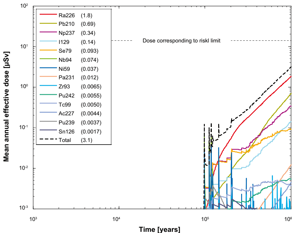
Figure 4-34. Near-field dose equivalent release for the probabilistic calculation of the corrosion scenario, with hydrogeological data from the uncorrelated model. The legend is sorted by peak (in the one-million year period) of the mean annual effective dose. The values in brackets are peak dose in units of \mu\text{Sv} .
