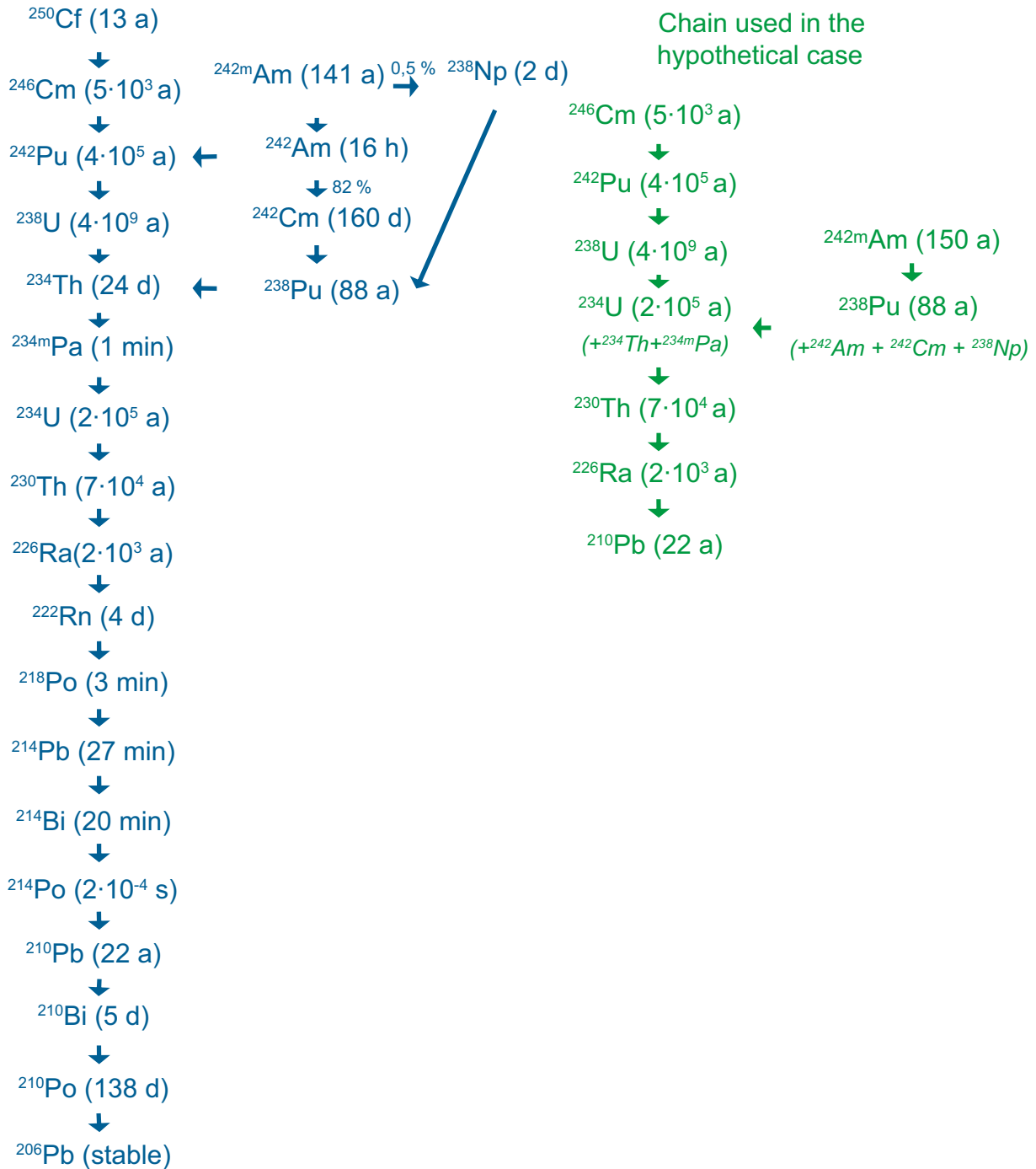
Figure D-11. The 4n+2 chain. The simplified chain is used in the hypothetical case to support the selection of radionuclides for the radionuclide transport calculations. Nuclides at the beginning of the chain without any inventory have been excluded in the simplified chain as have nuclides with a half-life shorter than 1 year but their inventories have been included in their daughter's inventory. Approximate half-lives shown are derived from Table D-3.
