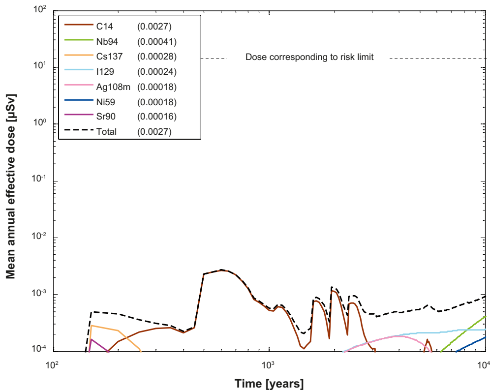
Figure 5-6. Near-field and far-field mean annual effective dose for the probabilistic calculation of the shear load scenario, with failure during the period up to 10,000 years. The legend is sorted by peak (in the one-million year period) of the mean annual effective dose. The values in brackets are peak dose in units of \mu\text{Sv} .
