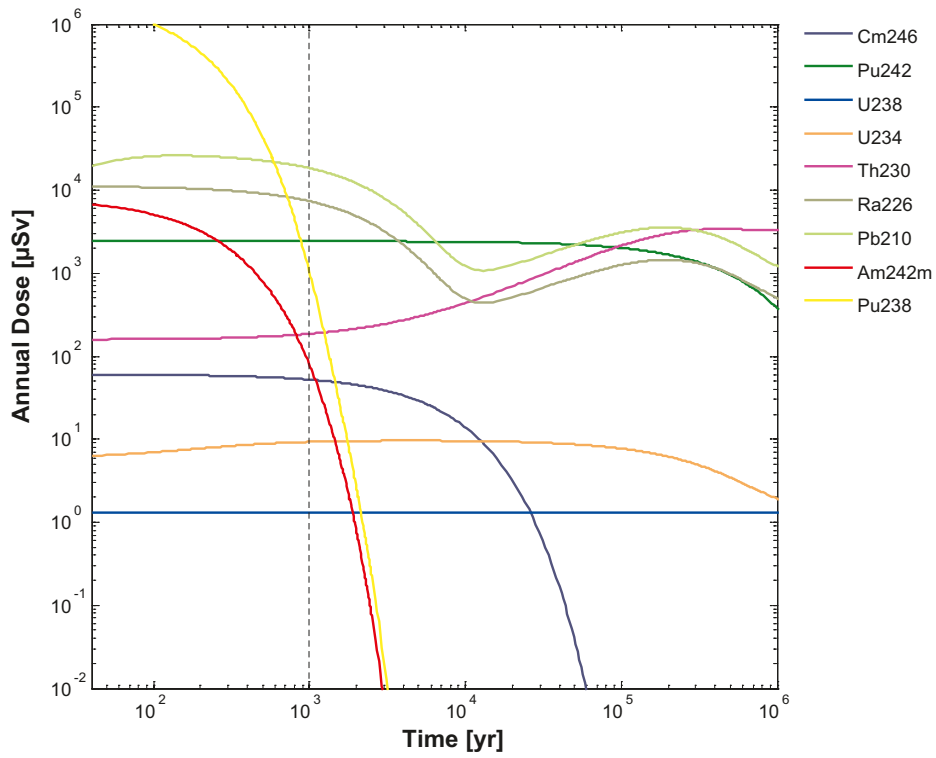
Figure D-12. Calculated annual dose in the hypothetical case supporting the selection of radionuclides for the radionuclide transport calculations of the 4n+2 chain. The vertical black dashed line denotes 1,000 years after closure.
