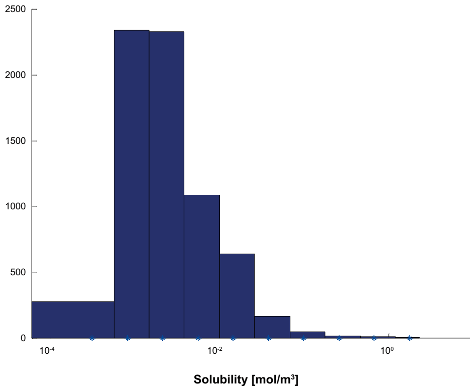
Figure F-17. Solubility limits for Ag used as input data for COMP23 in SR-Site. The y-axis shows the number of realisations in each bin.
