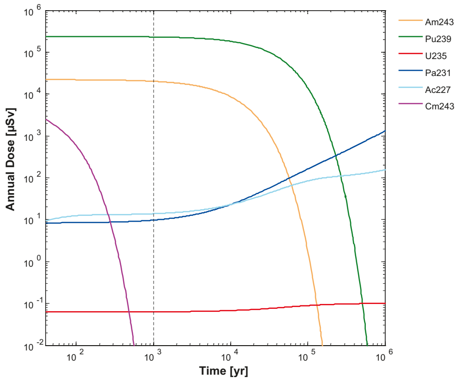
Figure D-16. Calculated annual dose in the hypothetical case supporting the selection of radionuclides for the radionuclide transport calculations of the 4n+3 chain. The vertical black dashed line denotes 1,000 years after closure.
