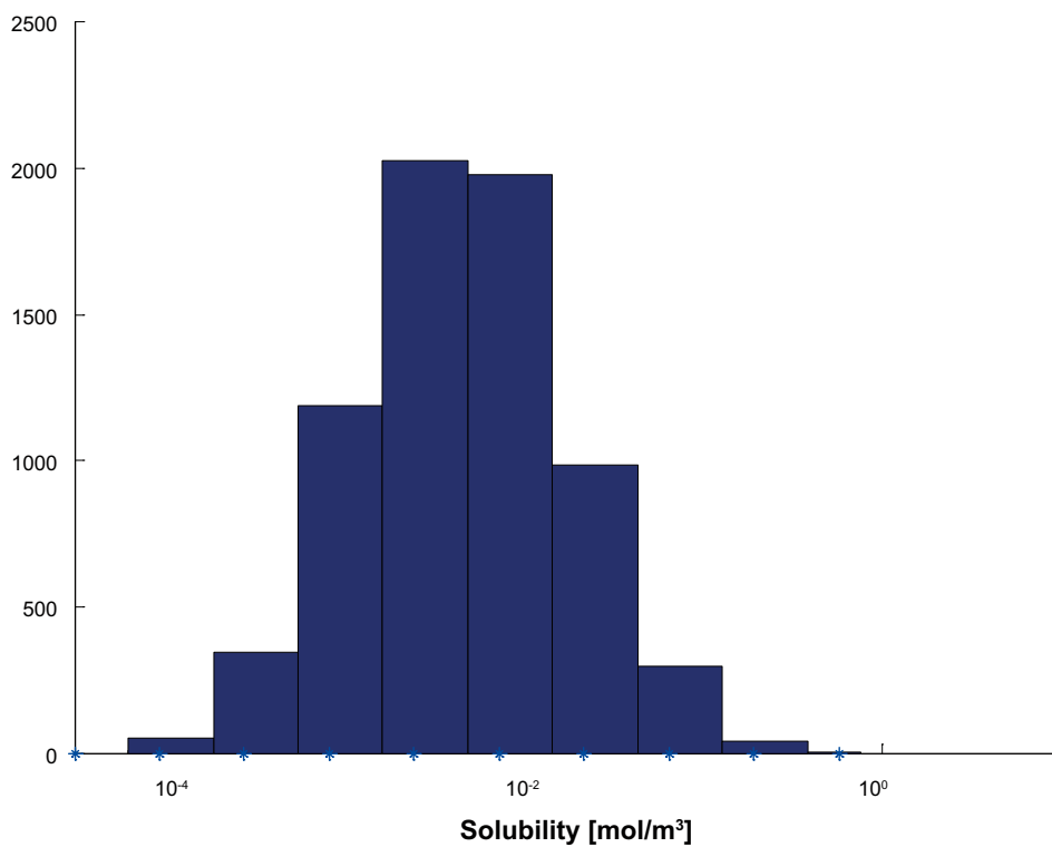
Figure F-26. Solubility limits for Pd used as input data for COMP23 in SR-Site. The y-axis shows the number of realisations in each bin.
