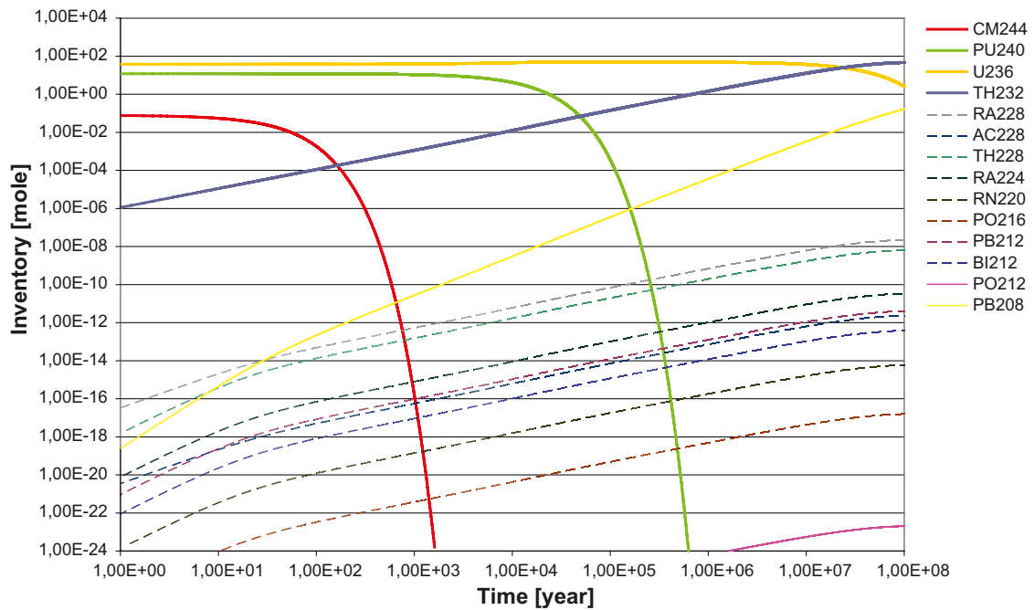
Figure D-6. Radionuclide content (mol/canister) as a function of time for radionuclides in the 4n chain. Initial inventory from /Håkansson 2000/.
