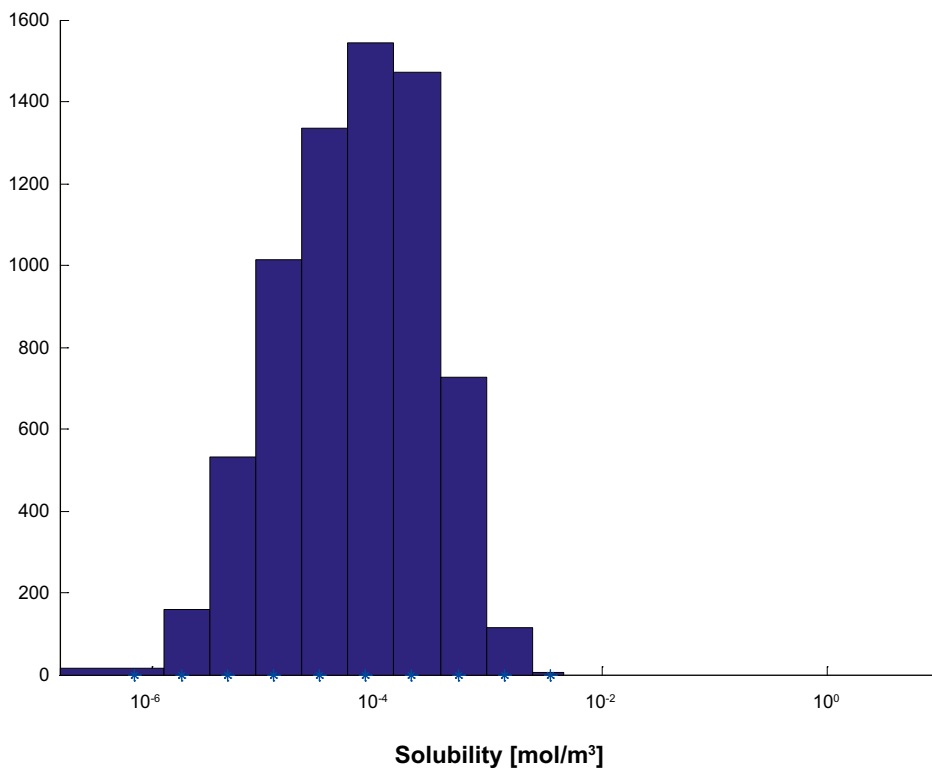
Figure F-30. Solubility limits for Sm used as input data for COMP23 in SR-Site. The y-axis shows the number of realisations in each bin.
