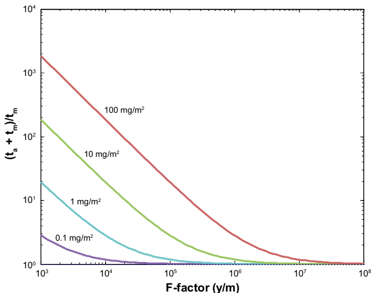
Figure B-7. Estimated relative enhancement ( \chi as defined by Equation B-30 plotted versus F-factor) of retardation effect for Ra(II) owing to solid solution equilibrium with barite. The impact of barite solid solution formation is shown for varying amounts of barite in the fracture coatings from 0.1 \text{ mg}/\text{m}^2 to 100 \text{ mg}/\text{m}^2 . Curves are calculated for the best estimate K_{ds} value for barite solid solution estimated using Equation B-25 and assume fast uptake kinetics (i.e. f_{eq} = 1 ).
