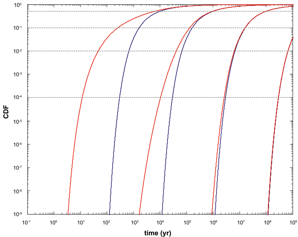
Figure A-10. Residence time distribution for a strongly sorbing solute ( K_d = 0.1 \text{ m}^3/\text{kg} ) for the simplified channelling scenario (red curves, Case 2) as compared to the reference scenario (blue curves, Case 1). Results are shown as a cumulative probability density function (CDF) for different reference case F-factors as indicated.
