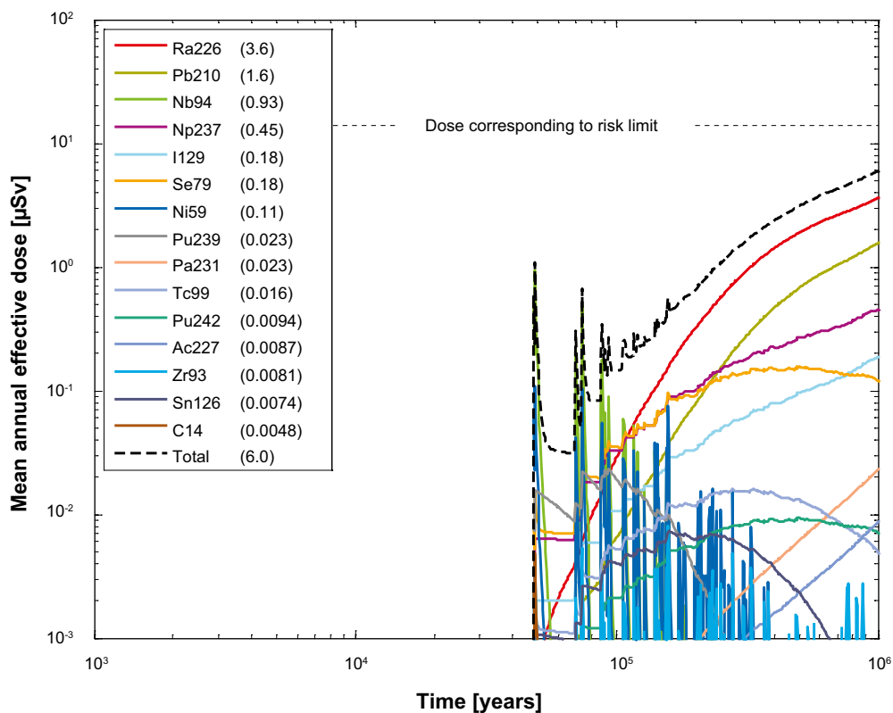
Figure 4-46. Near-field dose equivalent release for the probabilistic calculation of the corrosion scenario, with hydrogeological data from the fully correlated model and initial advection in the erosion/corrosion model. The legend is sorted by peak (in the one-million year period) of the mean annual effective dose. The values in brackets are peak dose in units of \mu\text{Sv} .
