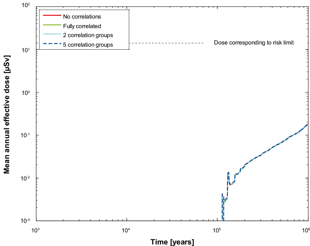
Figure 4-23. Far-field mean annual effective dose for probabilistic calculations of the central corrosion case with different correlations for K_d and D_e for rock.
