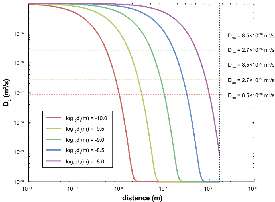
Figure B-19. Diffusivity profiles calculated using Equation B-38 assuming an exponentially decaying trend of solid state diffusivity bounded between 10^{-24} m 2 /s and 10^{-30} m 2 /s. Mean diffusivities averaged over the hypothetical maximum penetration depth of the calcite crystal ( 0.17 \mu\text{m} as indicated by the vertical broken line) are shown as horizontal broken lines and are matched by colour with the corresponding diffusivity profiles (numerical values are shown to the right hand side).
