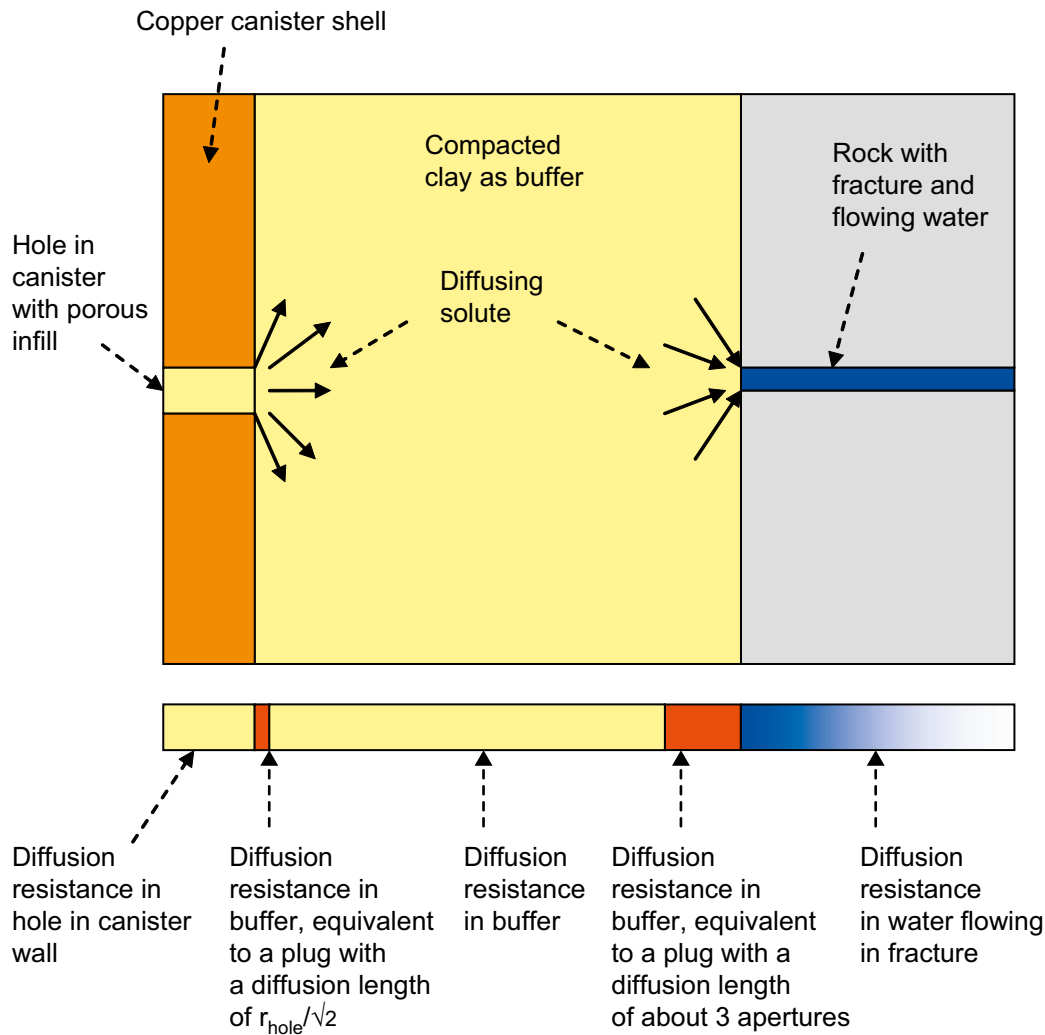
Figure G-1. Transport from a defect canister through the buffer and into a flowing water in fracture rock (modified from /Neretnieks 2006/ and /Neretnieks et al. 2010/).
