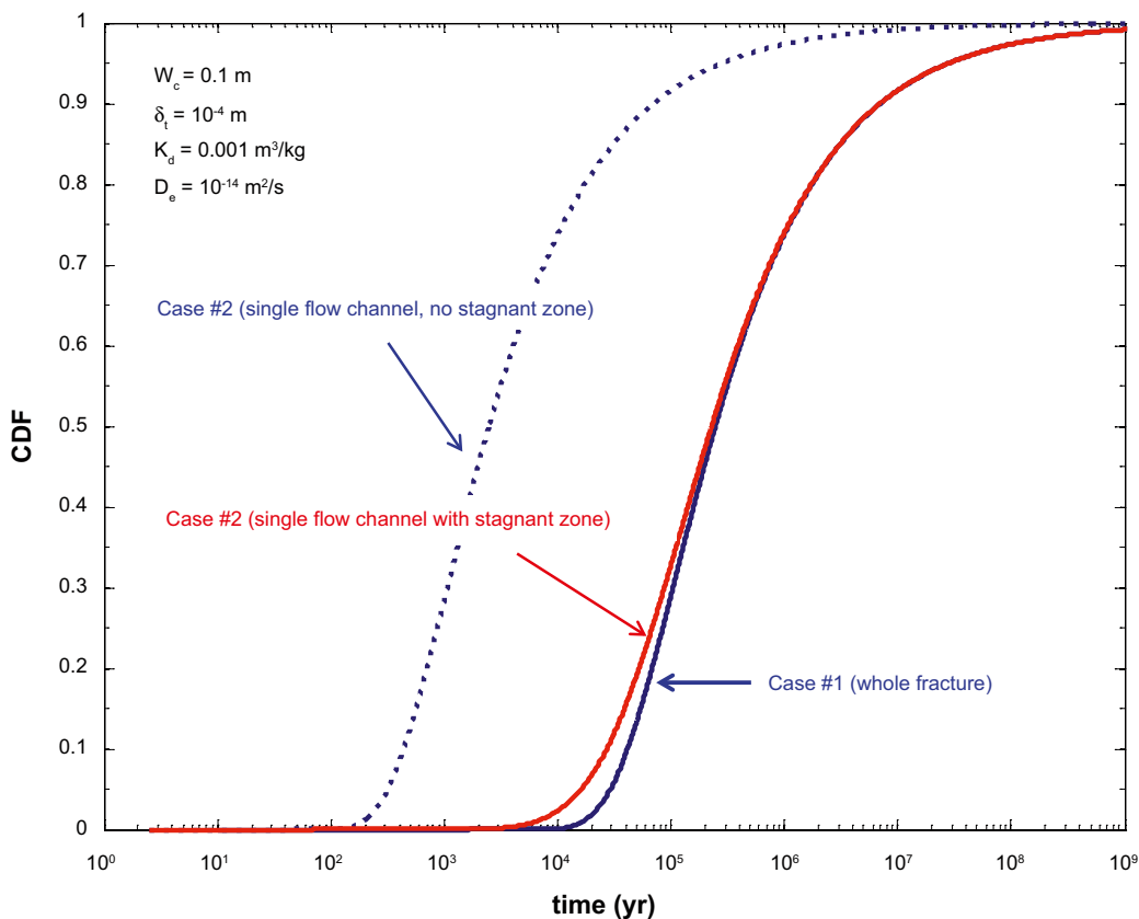
Figure A-3. Residence time distribution for a weakly sorbing solute ( K_d = 0.001 \text{ m}^3/\text{kg} ) assuming no channelling (Case 1, solid blue curve), flow channelling without stagnant zone diffusion (Case 2, broken blue curve), and flow channelling with stagnant zone diffusion (Case 2, red curve). The reference F -factor for Case #1 is 5 \cdot 10^5 \text{ yr/m} . Results are shown as a cumulative probability density function (CDF).
