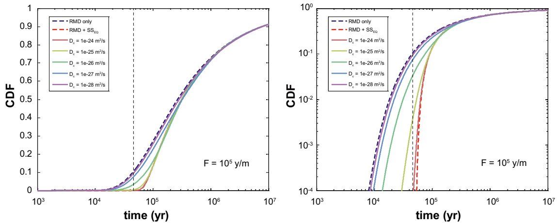
Figure B-22. Simulated residence time distribution curves for trivalent actinide transport assuming an F -factor of 10^5 yr/m and calcite solid solution for solid state diffusivities ranging from 10^{-28} m^2/s to 10^{-24} m^2/s . In the left-hand figure, data are plotted on a log-linear axis and on a log-log axis in the right-hand figure. The broken blue curve is the limiting case where only matrix diffusion and equilibrium sorption in the rock matrix is considered. The vertical broken line indicates the equilibrium retardation time for the solid solution, and the accompanying broken red curve shows the theoretical residence time distribution for matrix diffusion coupled with equilibrium retention by the solid solution.
