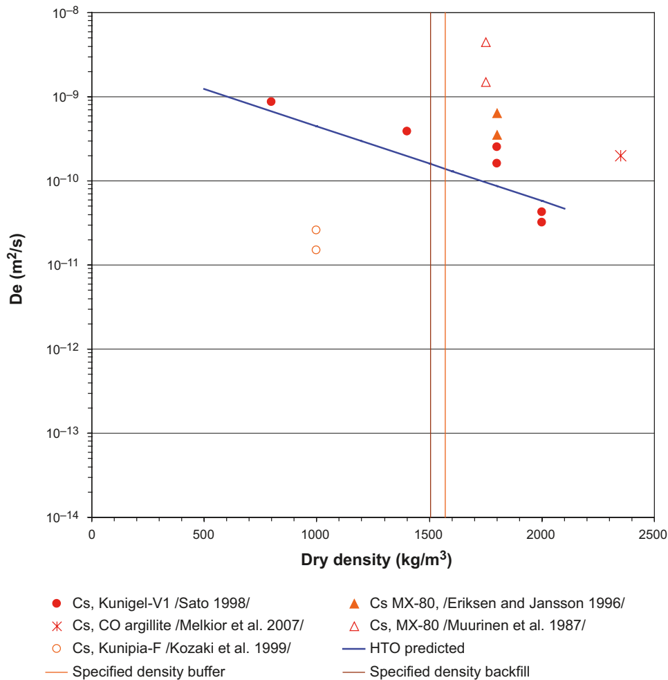
Figure 5-10. Effective diffusivities obtained in compacted clays using Cs^+ as tracer. The specified reference buffer and backfill dry densities are indicated. The regression for HTO is shown for comparison.
