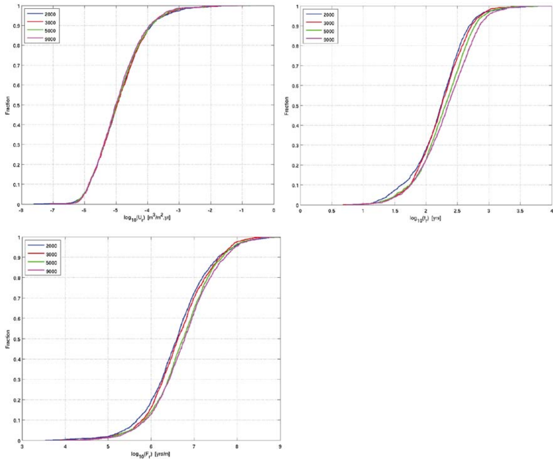
Figure 6-67. Normalised CDF plots of Darcy flux q (denoted U_r in figure caption,) t_w and F (denoted t_w and F_r in figure captions to indicate that t_w and F are calculated in the bedrock described as a DFN only) in the Hydrogeological base case model at 2000 AD, 3000 AD, 5000 AD, and 9000 AD for release path Q1. The t_w and F_r plots are based on particles successfully reaching the model top boundary (cf. /Selroos and Follin 2010, Figure 5-9/).
