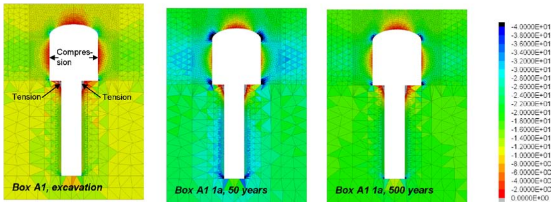
Figure 6-54. Contours of the vertical stress component after excavation (left), 50 years (middle) and 500 years (right). Stresses are plotted in the range from -40 MPa (compression) to 0 MPa. Note that stress magnitudes that fall outside the range are marked in black for compression and light grey for tension. Modified from /Hökmark et al. 2010, Figure H-9/.
