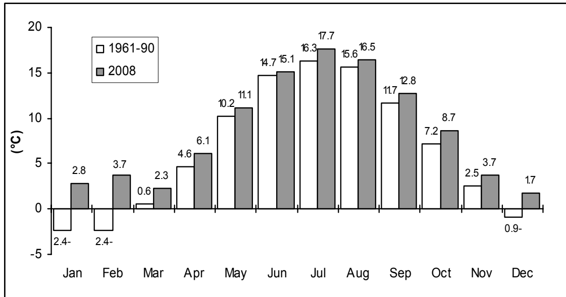
Figure 5-4. Temperature at Oskarshamn/Äspö: Monthly values for Norra Äspö 2008 and monthly means for Oskarshamn 1961 – 1990.
