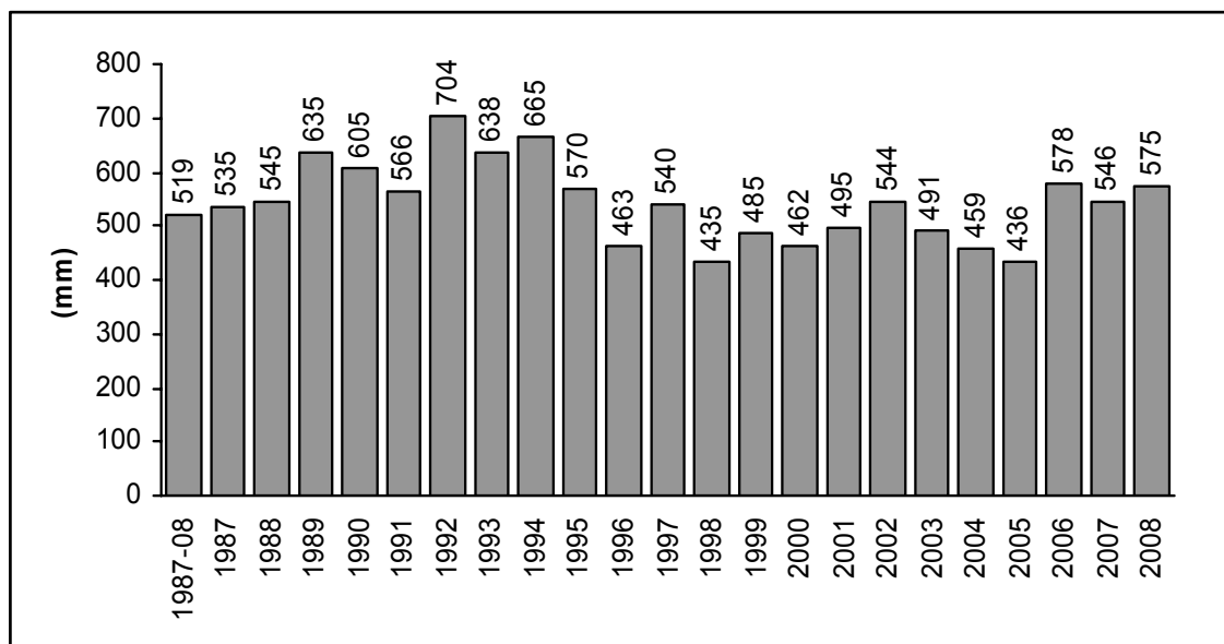
Figure 5-7. Potential evapotranspiration. Yearly values for Norra Äspö 2006 - 2008, for Gladhammar and Ölands Norra Udde 1987 - 2005 and yearly mean for the period 1987 - 2008.
