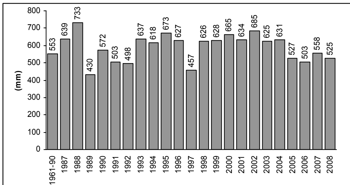
Figure 5-3. Precipitation at Oskarshamn/Äspö. Yearly values for Norra Äspö 2006 - 2008 and for Oskarshamn 1987 - 2005 and yearly mean for Oskarshamn for the period 1961 - 1990.
