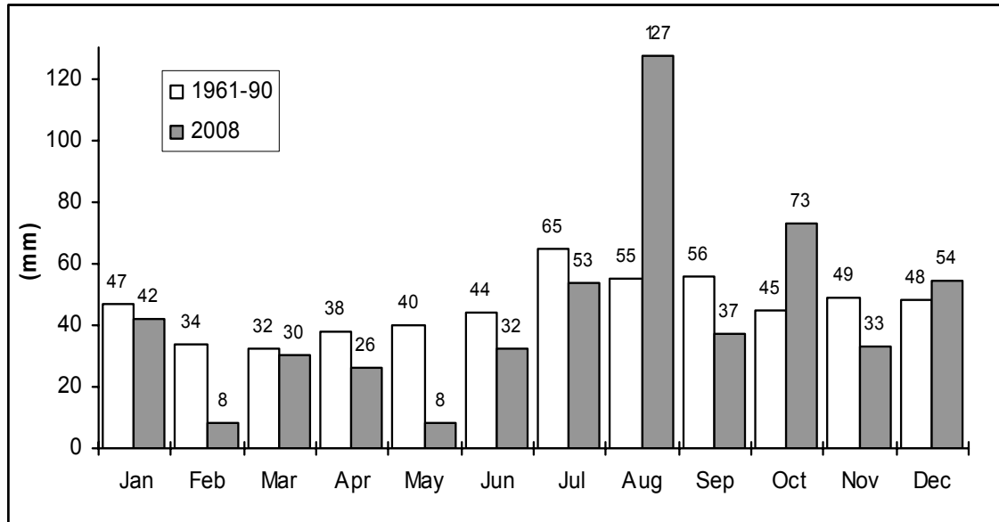
Figure 5-2. Precipitation at Oskarshamn/Äspö: Monthly values for Norra Äspö 2008 and monthly means for Oskarshamn 1961 – 1990.
