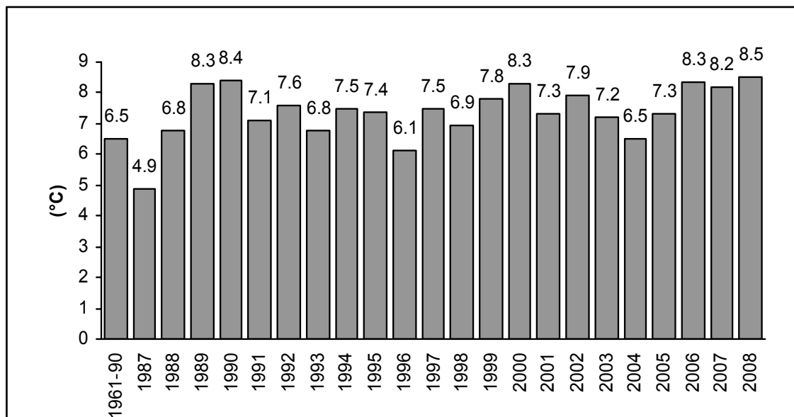
Figure 5-5. Temperature at Oskarshamn/Äspö. Yearly values for Norra Äspö 2006 - 2008 and for Oskarshamn 1987 - 2005 and yearly mean for Oskarshamn for the period 1961 - 1990.
