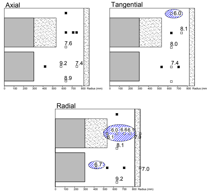
Figure 5-7. Total pressure distribution on July 1, 2008. Values in MPa. Boxes are sensor positions. Filled boxes indicate sensors out of order. Levels below 7 MPa marked blue.
