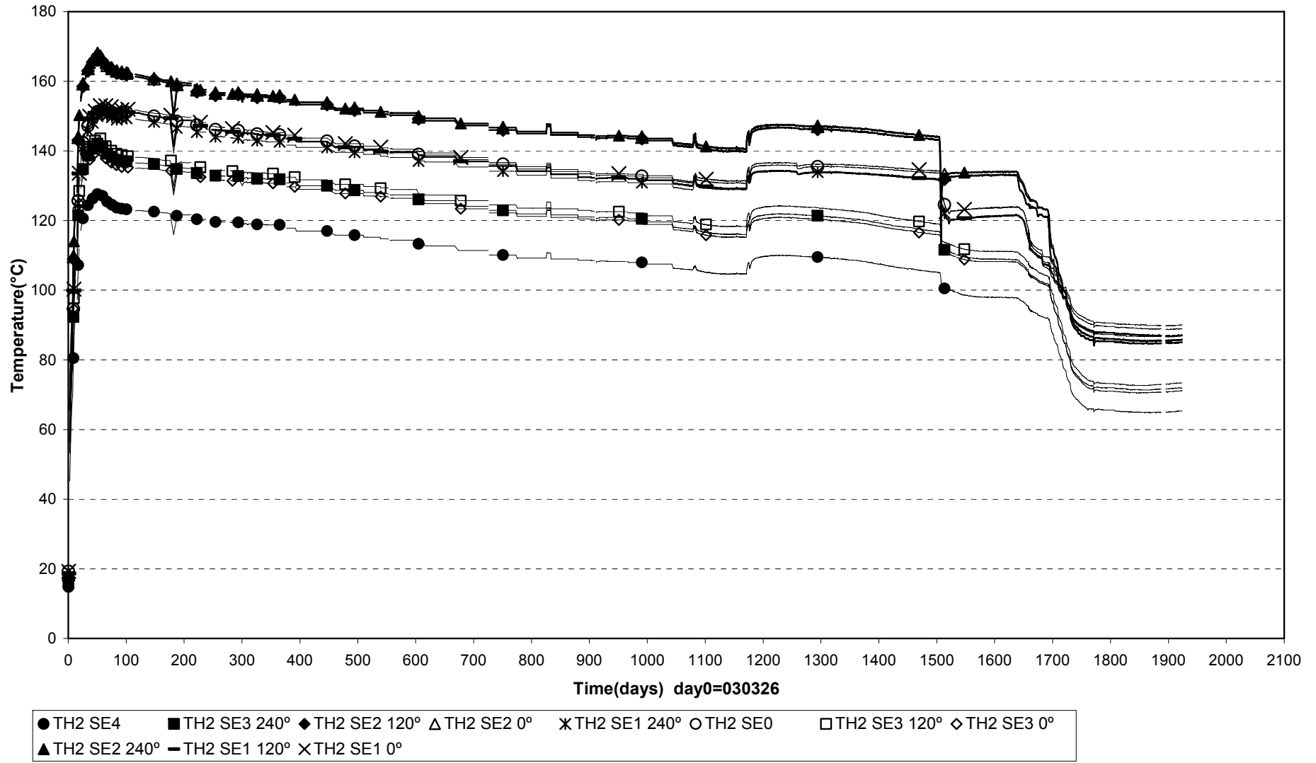
External temperatures Heater 2 (070504-080701)
