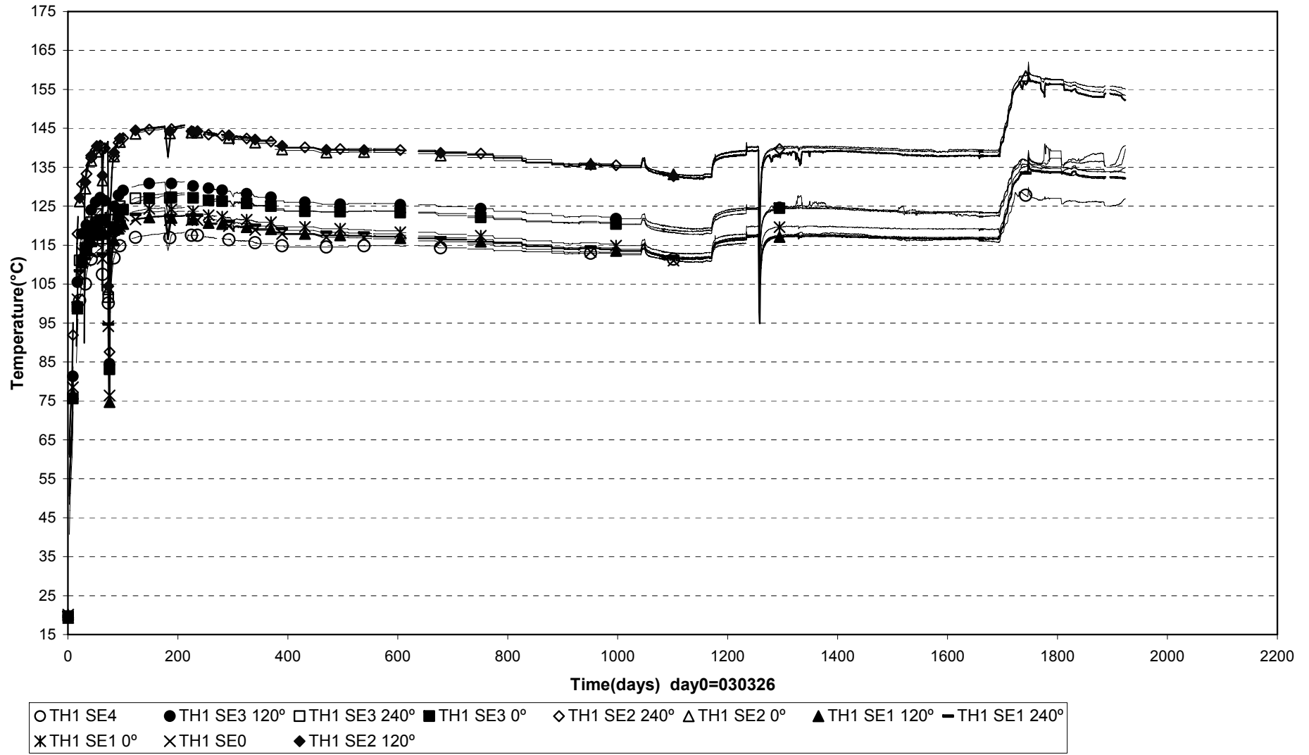
External temperatures Heater 1 (030326-080701)
