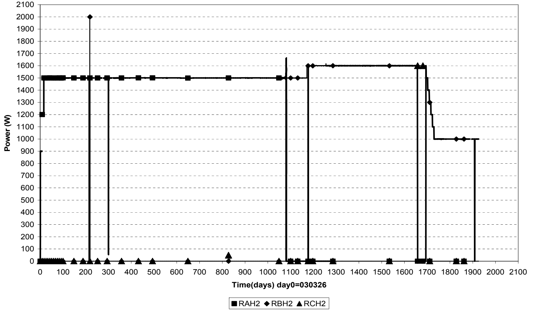
Power Heater 2 (03026-080701)
