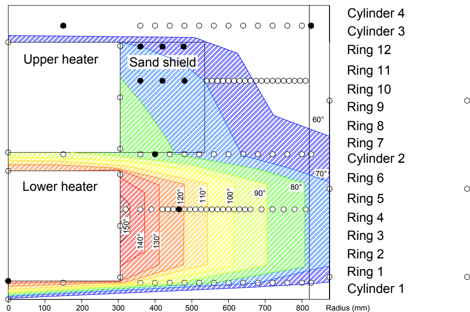
Figure 5-3. Temperature distribution on July 1, 2008. Rings indicate sensor positions. Filled rings indicate sensors out of order.
