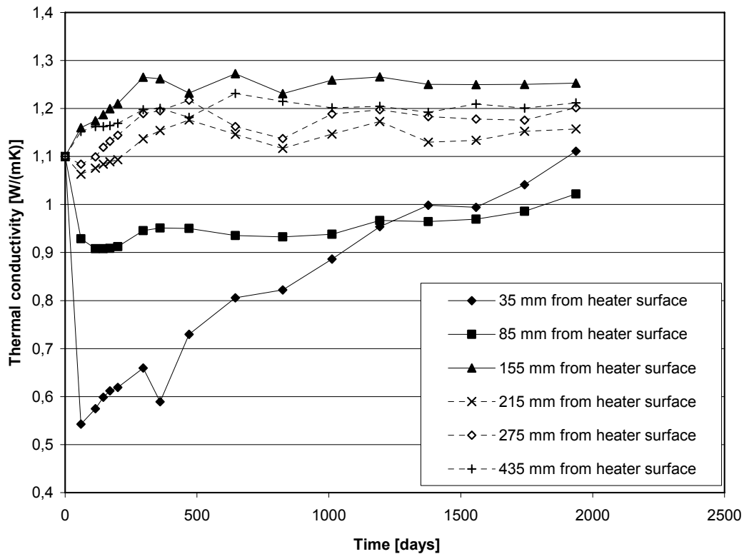
Figure 5-5. Thermal conductivity development in Ring 4.
