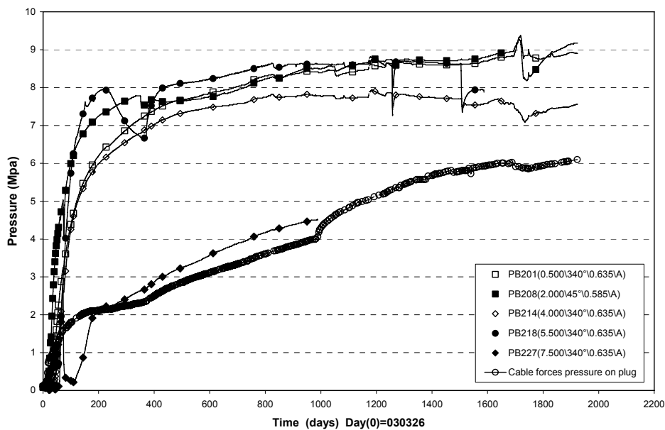
Figure 5-8. Axial pressure measured in different sections. Cable forces are shown as pressures, assuming an even distribution over the rock hole area ( 2.40 \text{ m}^2 ).
