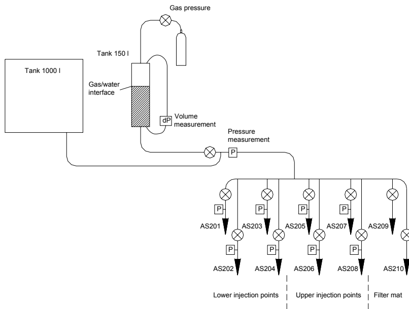
Figure 5-1. Schematic view of injection system.
