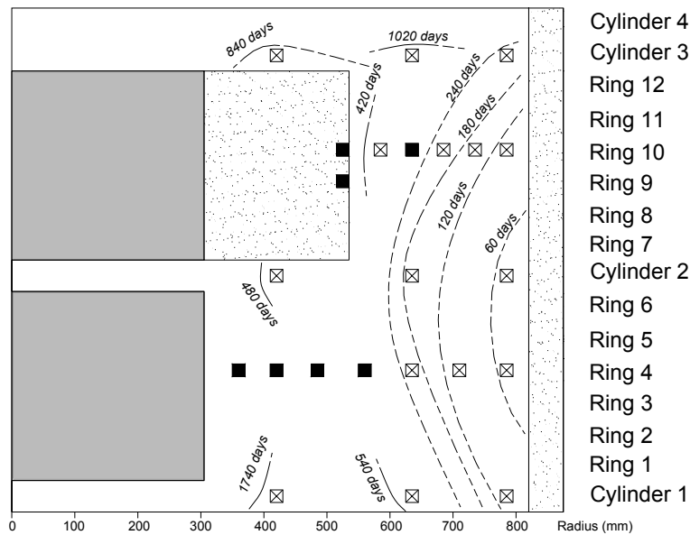
Figure 5-6. Occurrences of vapour saturation up till July 1, 2008. Boxes are sensor positions. Ticked boxes indicate saturation. Filled boxes indicate sensors out of order.
