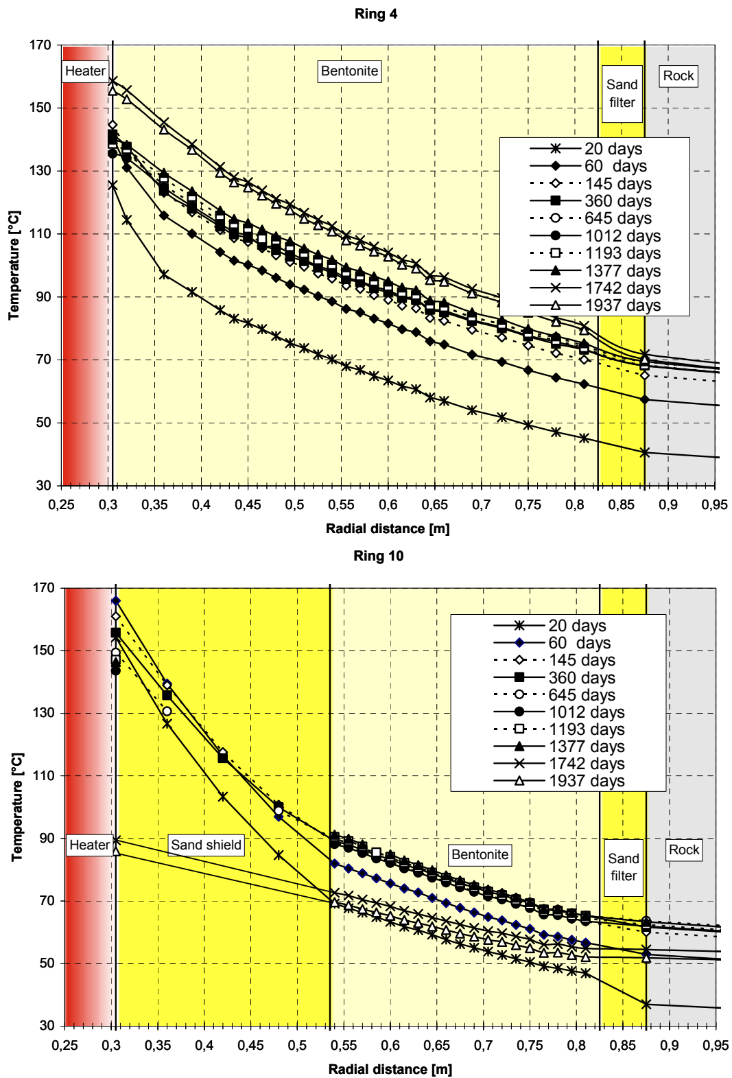
Figure 5-4. Temperatures measured at mid-height of Heater 1 (Ring 4) and Heater 2 (Ring 10).
