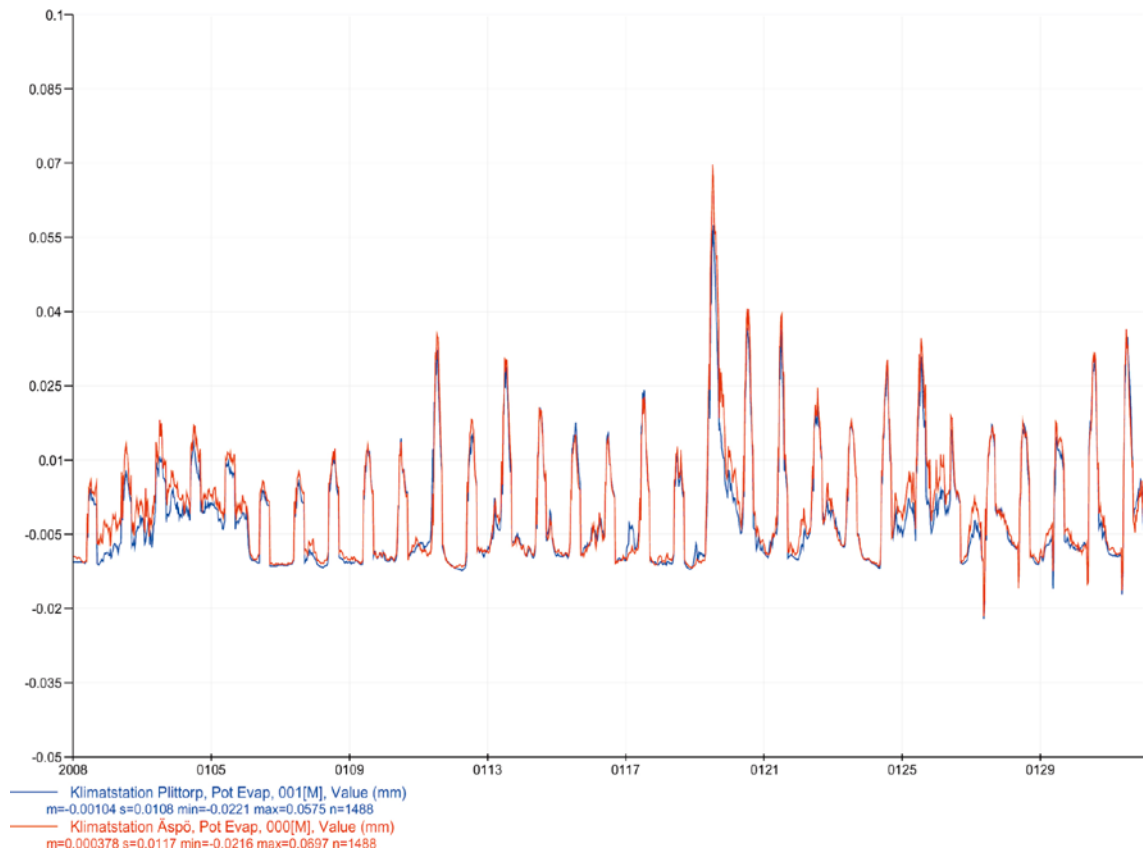
Figure A5-15. Evapotranspiration in mm, 30 min values. January 2008.
