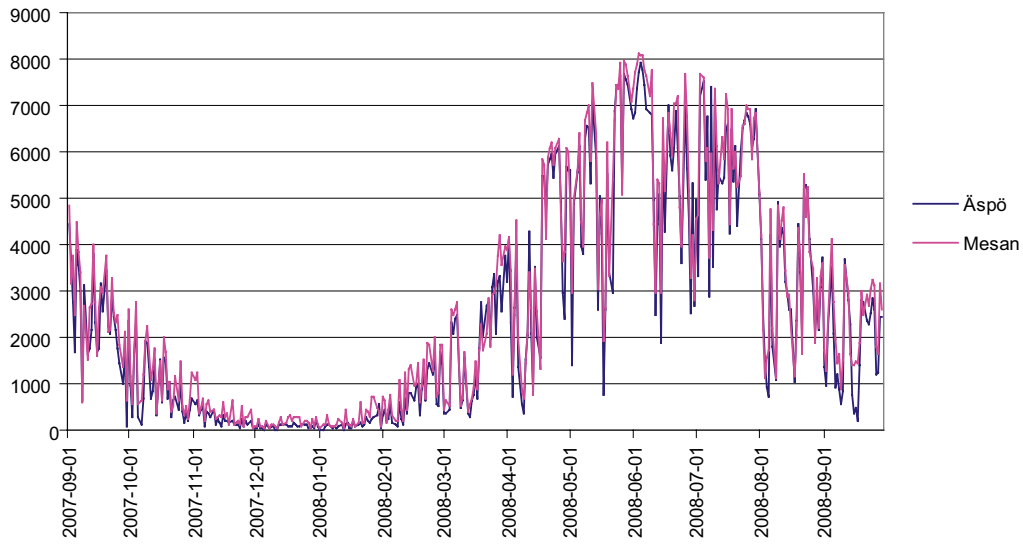
Figure A5-7. Global radiation in Wh/m 2 , daily sum. September 2007–September 2008.
