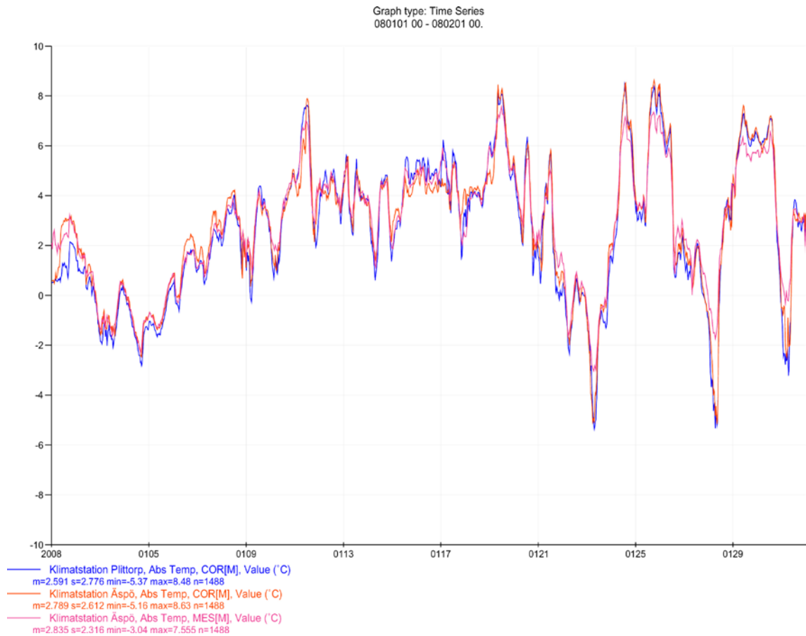
Figure A5-11. Temperature in °C, 30 min-values. January 2008.
