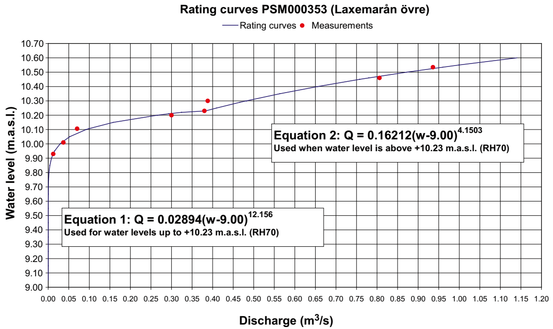
Figure A2-7. Rating curve for PSM000353 Laxemarån upper based on control measurements made up to 2006-10-01.
