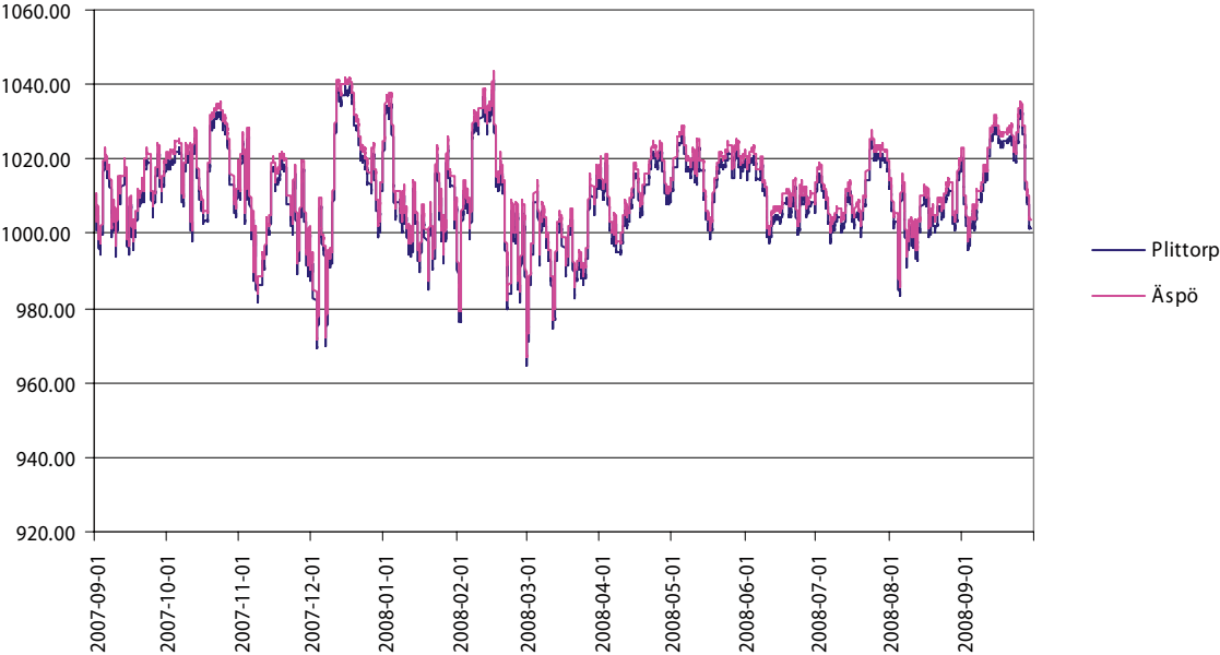
Figure A5-2. Barometric pressure in hPa, daily values. September 2007–September 2008.
