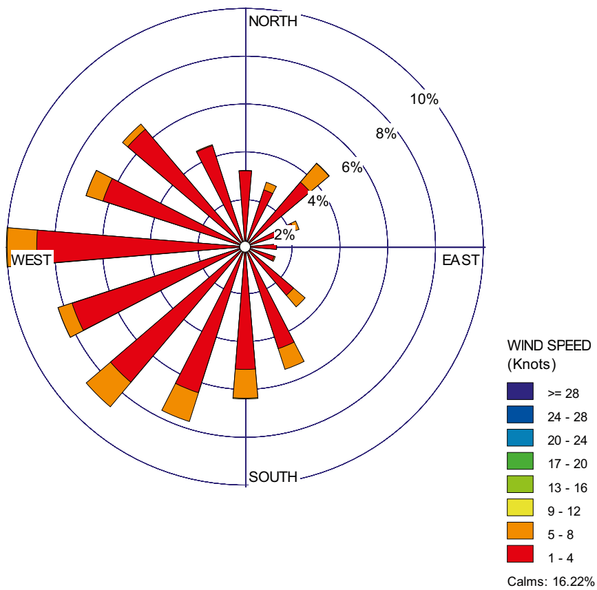
Figure A5-6. Windroses of 30-minutes values for Åspö and Plittorp. September 2007–September 2008.
