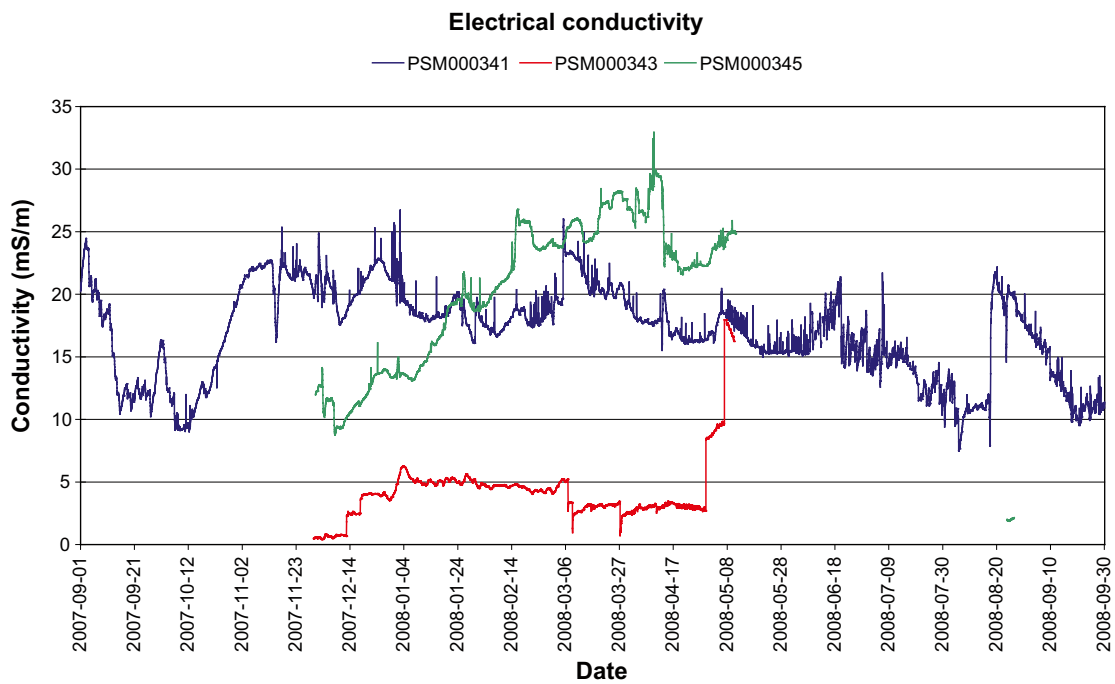
Figure 5-10. Electrical conductivity, EC, measured at stations PSM000341, PSM000343 and PSM000345. Values deleted during periods when the discharge equals zero or when the watercourse is dried up. Extremely high values at station PSM000345 corrected.
