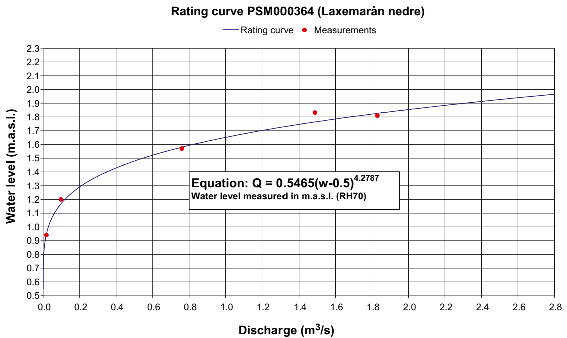
Figure A2-8. Rating curve for PSM000364 Laxemarån lower based on control measurements made up to 2006-10-01.
