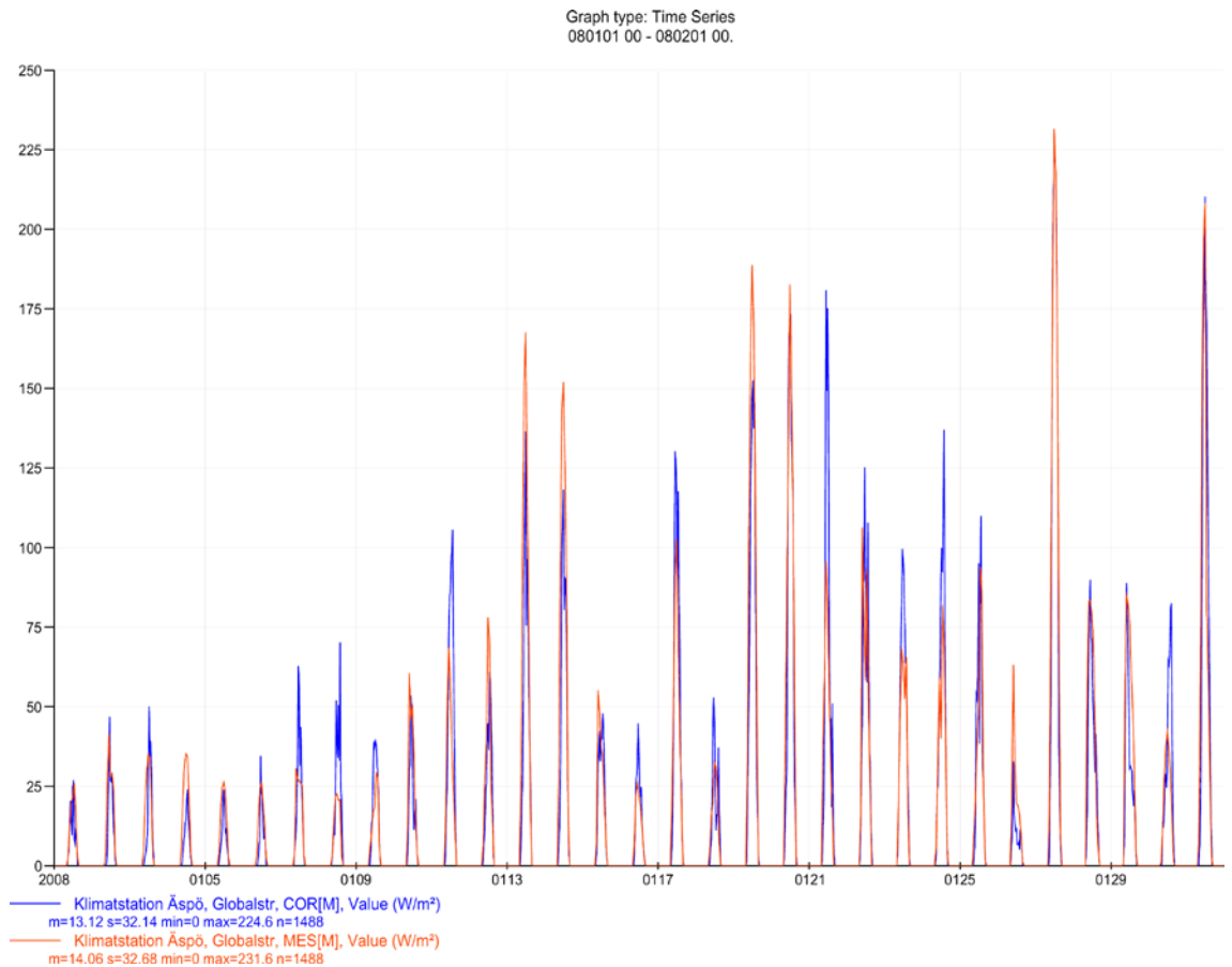
Figure A5-14. Global radiation in W/m 2 , 30 min values. January 2008.
