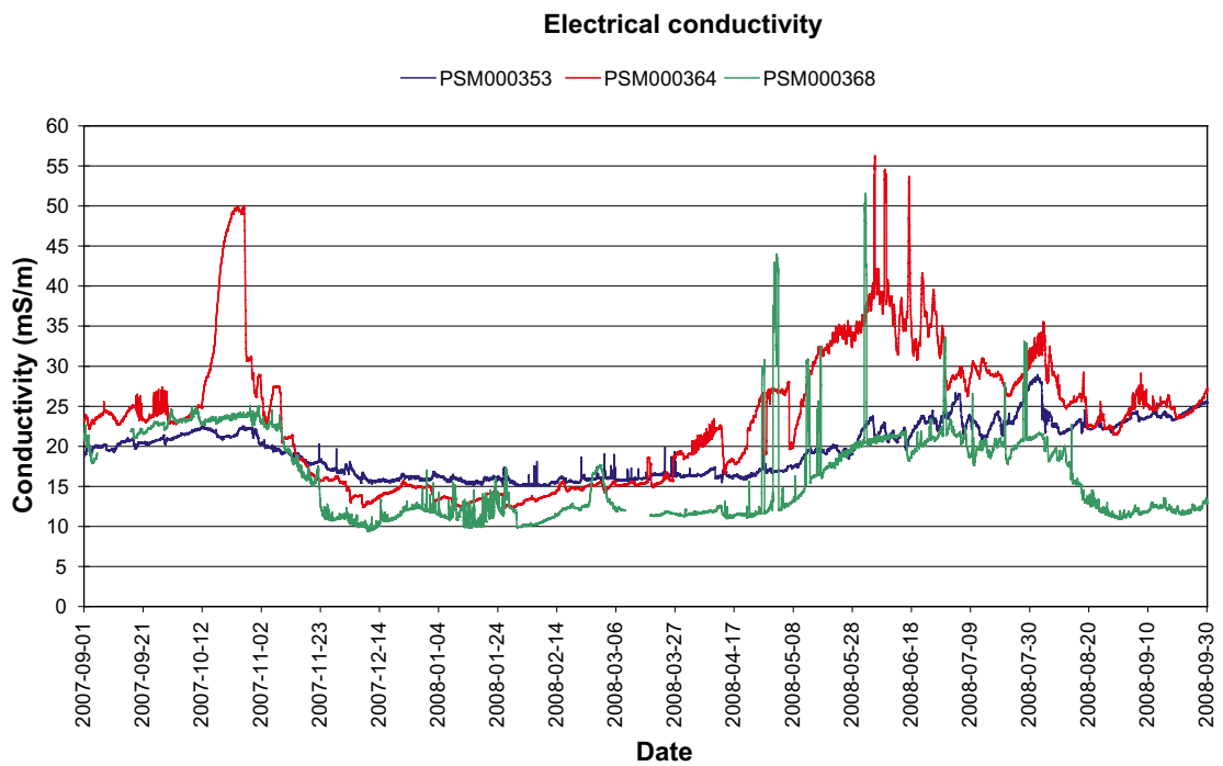
Figure 5-14. Electrical conductivity measured at station PSM000353, PSM000364 and PSM000368. Extremely high and low values corrected.
