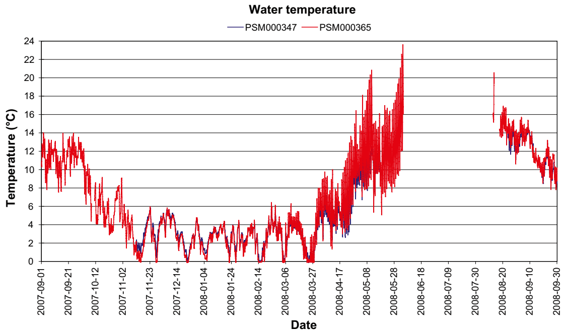
Figure 5-11. Water temperature measured at stations PSM000347 and PSM000365. Values deleted during periods when the discharge equals zero or when the watercourse is dried up.
