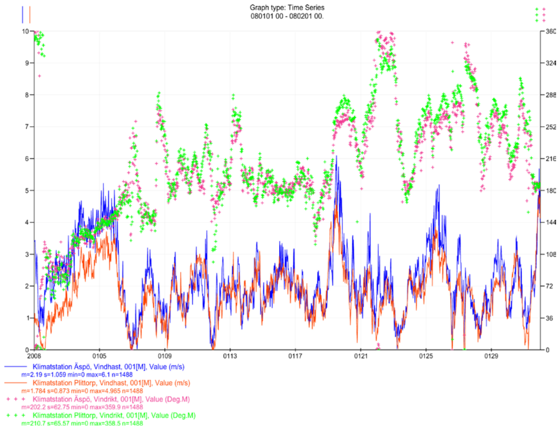
Figure A5-13. Wind speed in m/s and wind directions in ° , 30 min values. January 2008.
