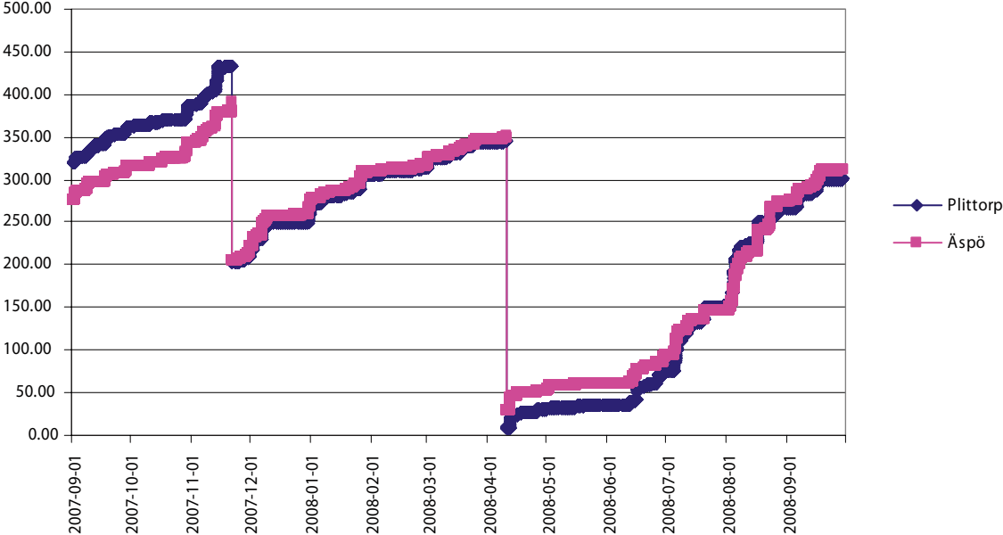
Figure A5-1. Precipitation in mm, 30 min values. September 2007–September 2008.
