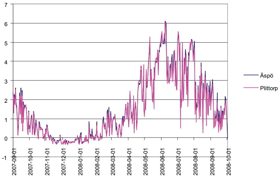
Figure A5-8. Potential evapotranspiration in mm, daily sum. September 2007–September 2008.
