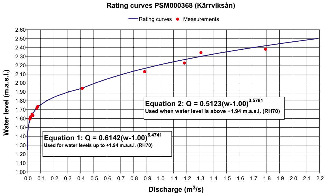
Figure A2-9. Rating curve for PSM000368 Kärrviksån based on control measurements made up to 2006-10-01.
