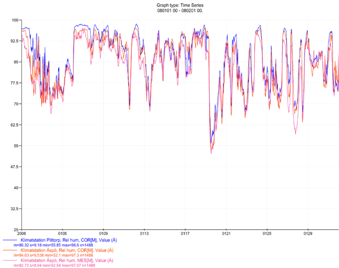
Figure A5-12. Relative humidity in %, 30 min-values. January 2008.
