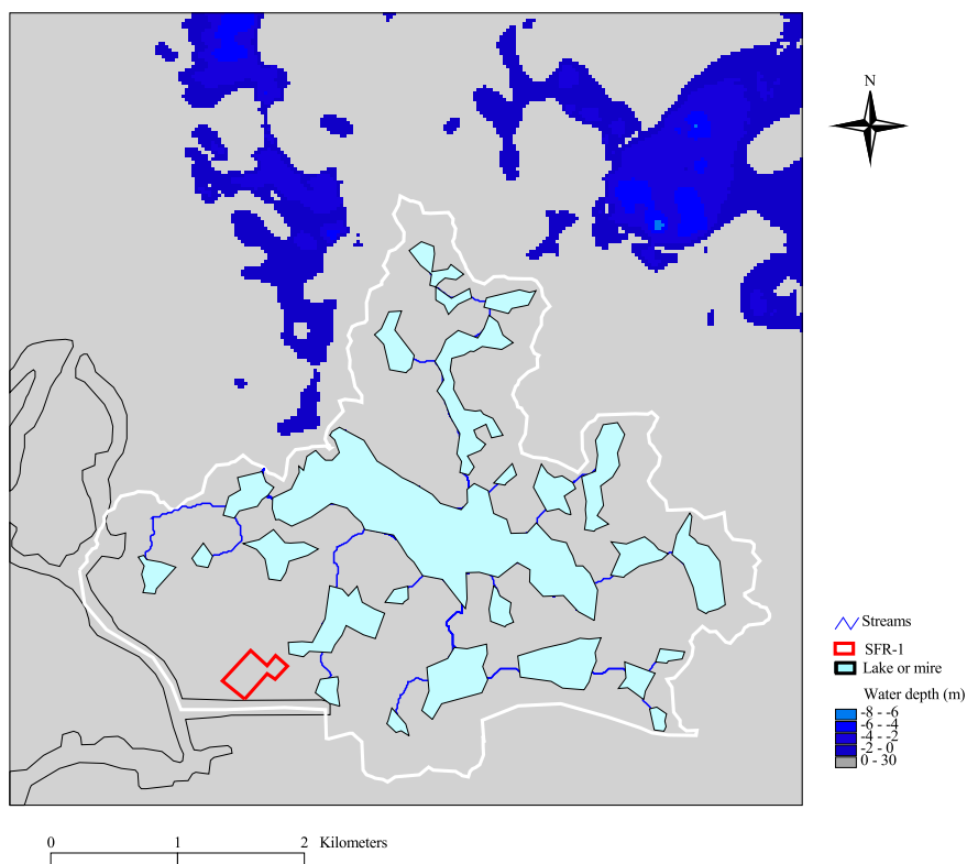
Figure 12. The water depth conditions in the inner model area 5000 AD. Notice that no brackish water occurs in the inner model area at this time. Permissions: The National Land Survey of Sweden, register number 507-96-1524 and the Swedish national administration of shipping and navigation, permission number 9709388.
