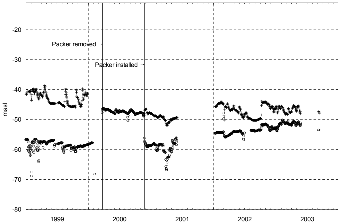
Figure 6-4 Groundwater levels in HAS04 on Äspö, 1999-2003.
