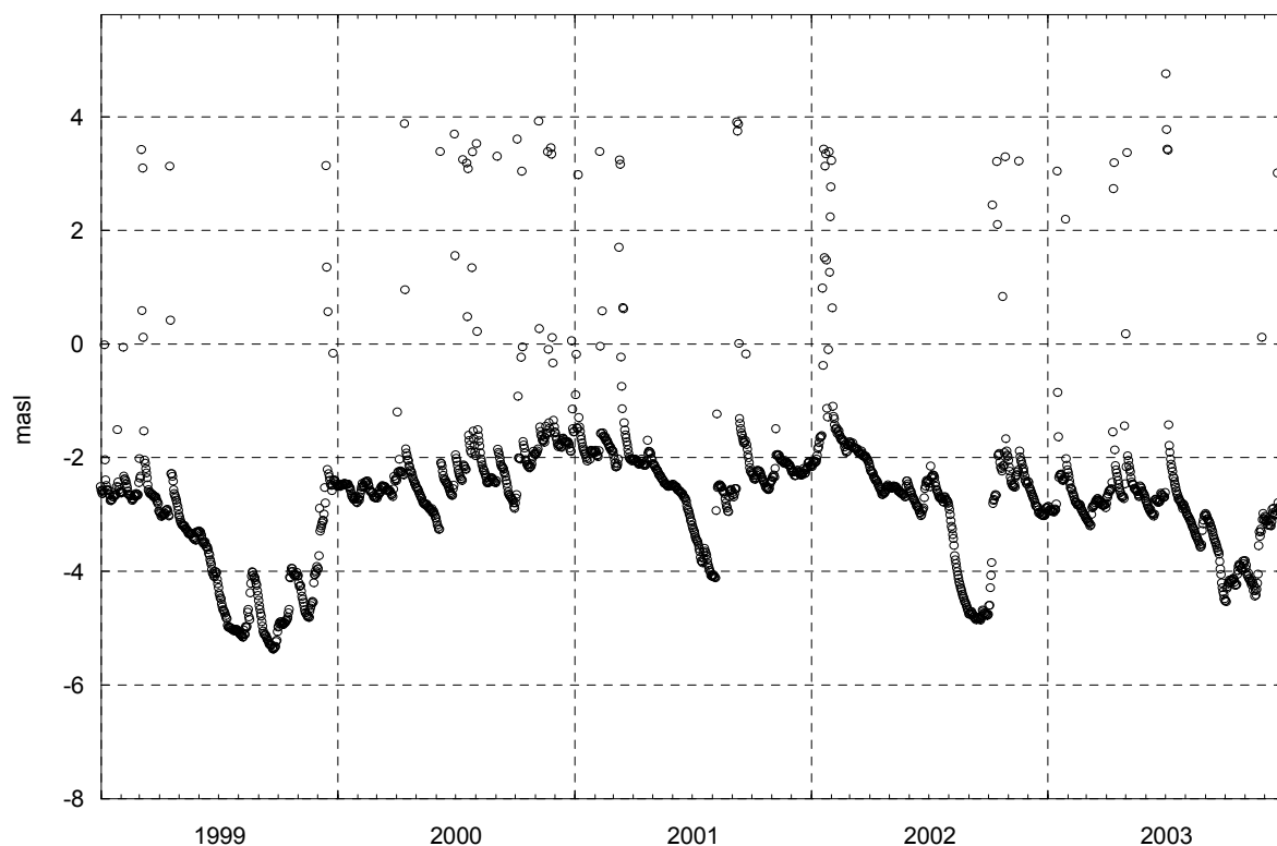
Figure 6-5 Groundwater levels in HAV08 on Ävrö, 1999-2003.
