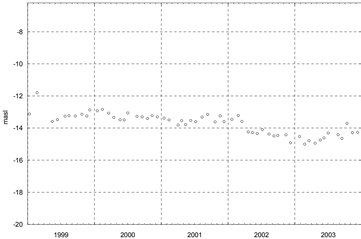
Figure 6-3 Groundwater levels in KAS14 on Äspö, 1999-2003.
