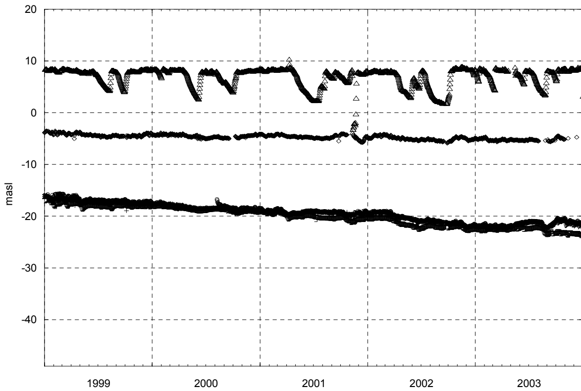
Figure 6-1 Groundwater levels in KAS03 on Äspö, 1999-2003.
