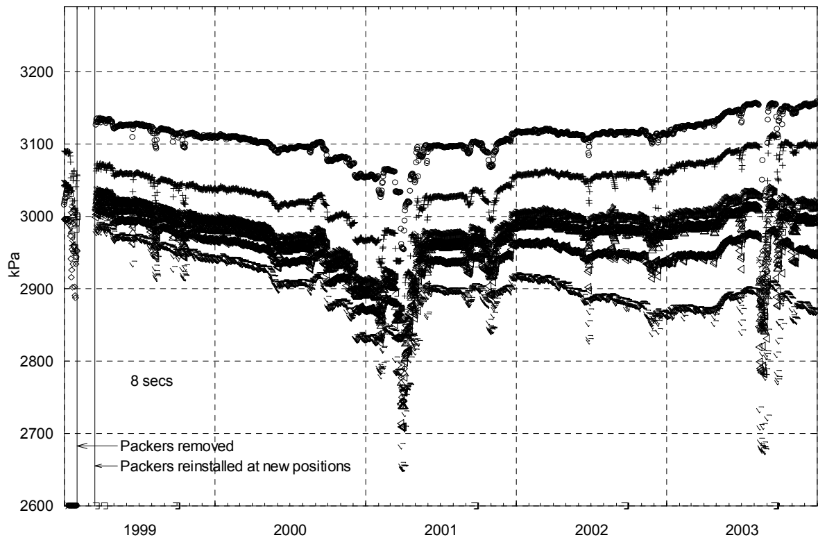
Figure 6-7 Groundwater pressure in tunnel borehole KA2511A, 1999-2003.
