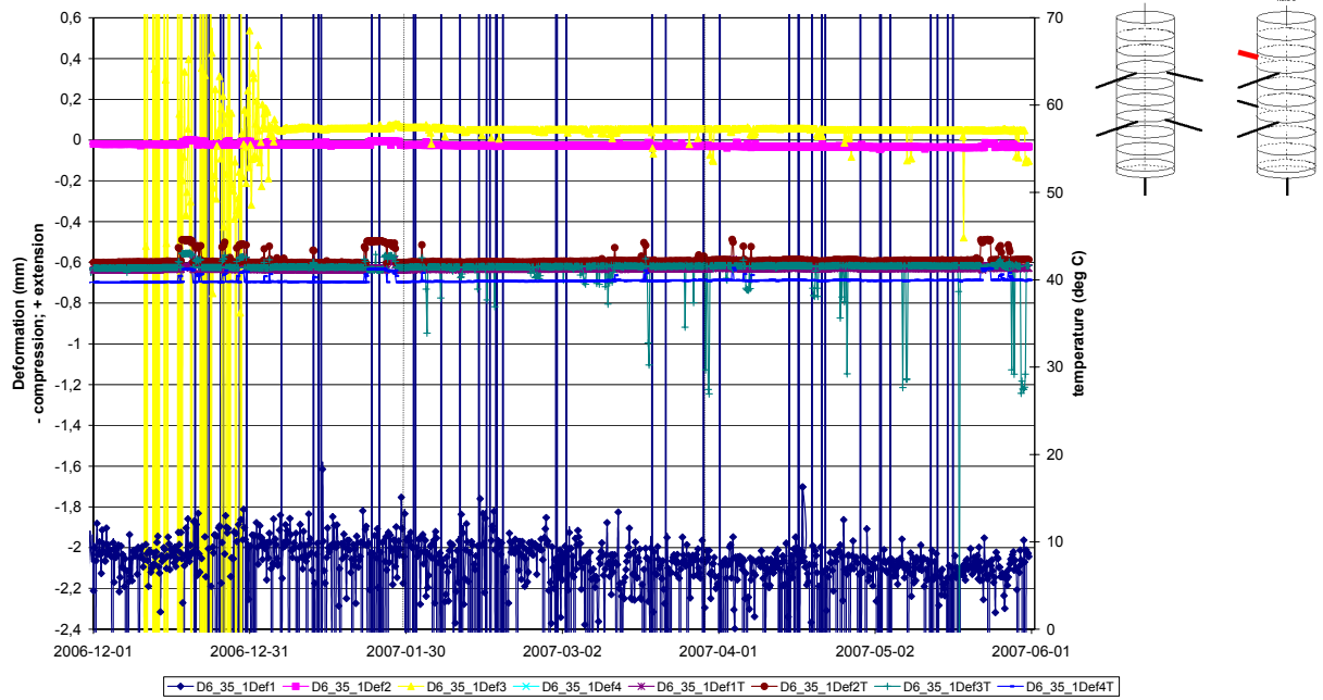
Deformation measurements Borehole D6:3.5(1)
