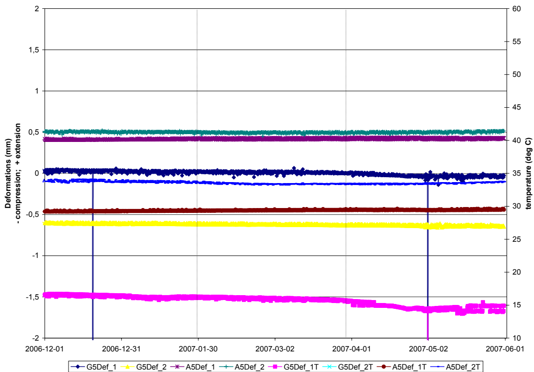
Vertical deformations adjacent to Deposition Hole 5 in Boreholes G5 and A5
