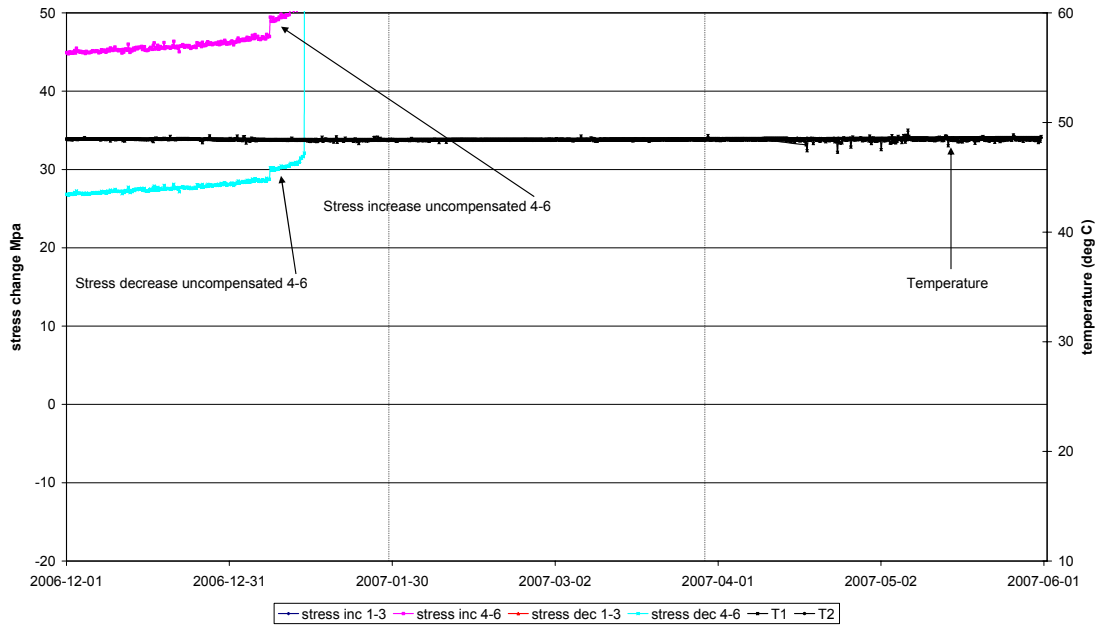
Biaxial stressmeter E5 Maximum stress increase and stress decrease in plane perpendicular to borehole axis
