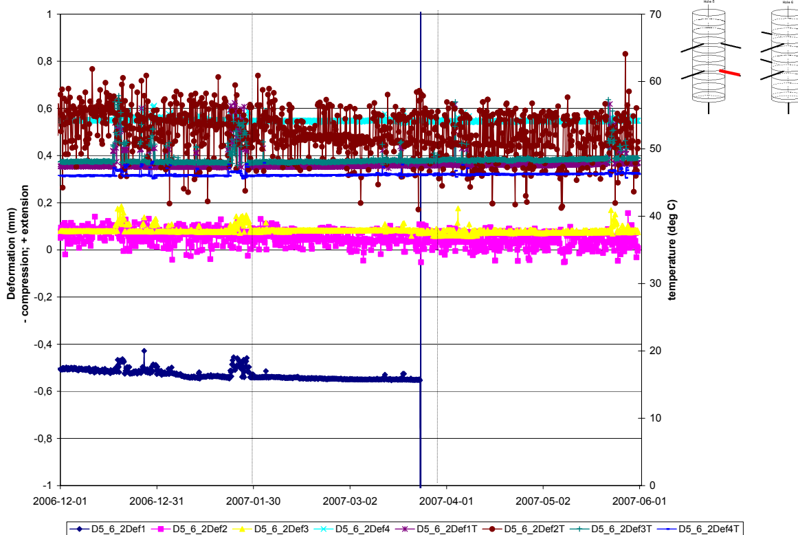
Deformation measurements Borehole D5:6(2)
