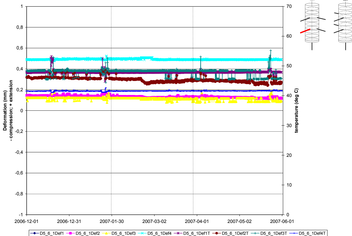
Deformation measurements Borehole D5:6(1)
