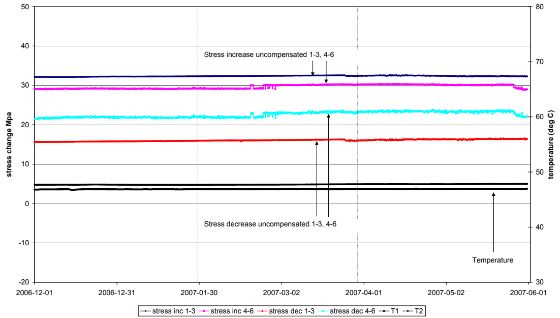
Biaxial stressmeter G5 Maximum stress increase and stress decrease in plane perpendicular to borehole axis
