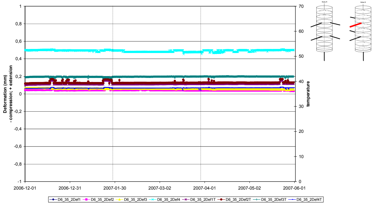
Deformation measurements Borehole D6:3.5(2)
