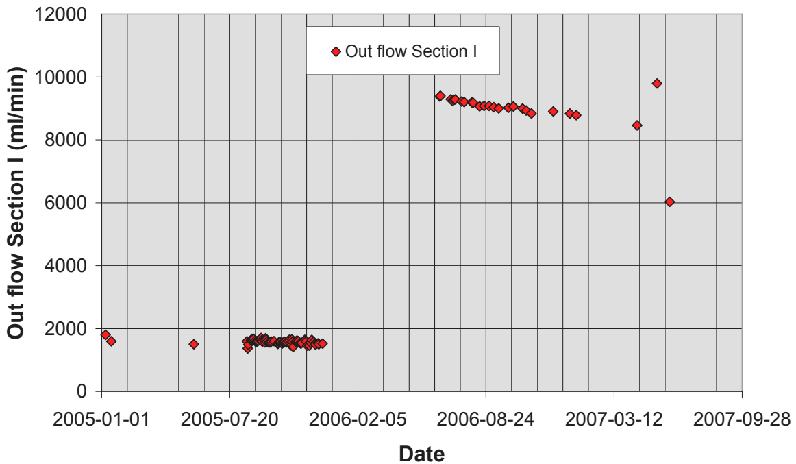
Figure 5-8. The measured outflow from the inner section of the Prototype tunnel.
