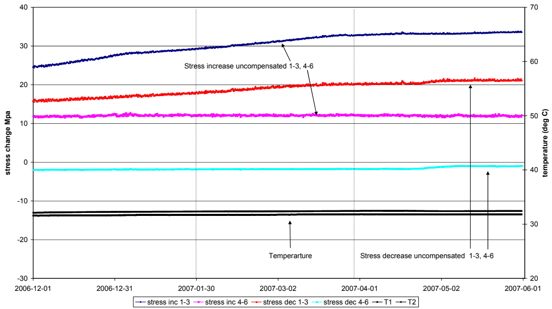
Biaxial stressmeter A6 Maximum stress increase and stress decrease in plane perpendicular to borehole axis
