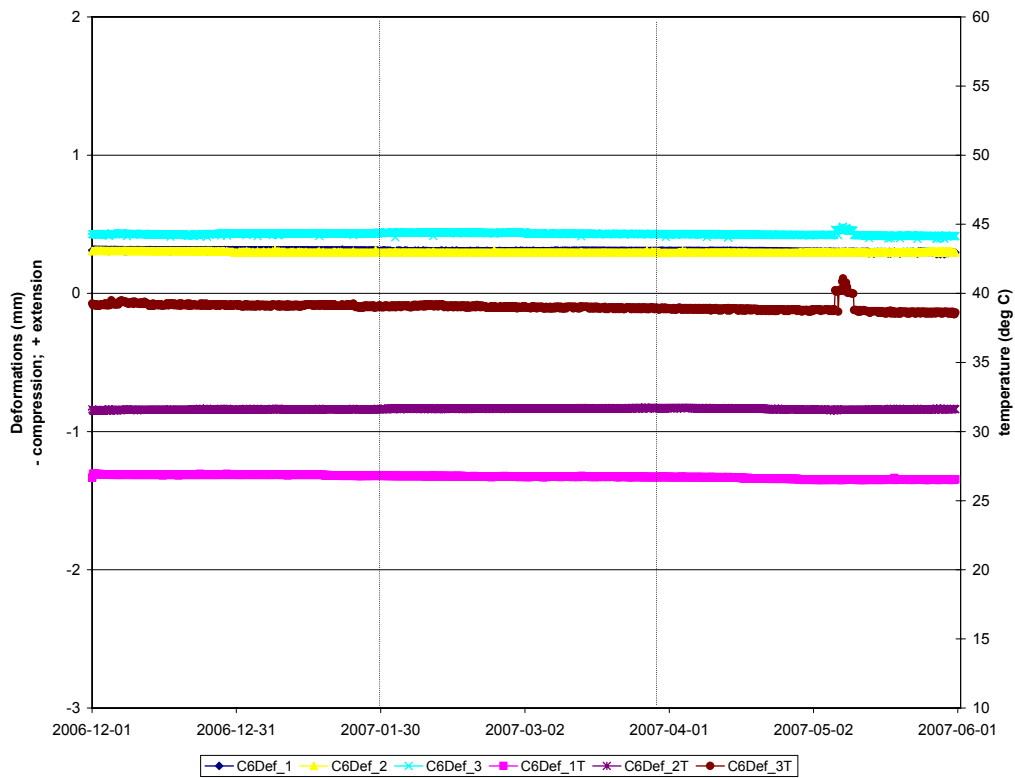
Vertical deformations adjacent to Deposition Hole 6 in borehole C6
