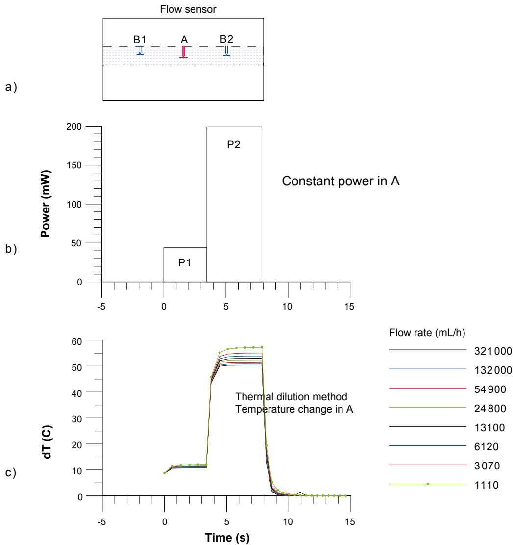
Figure 3-4. Flow measurement, flow rate > 600 mL/h.
