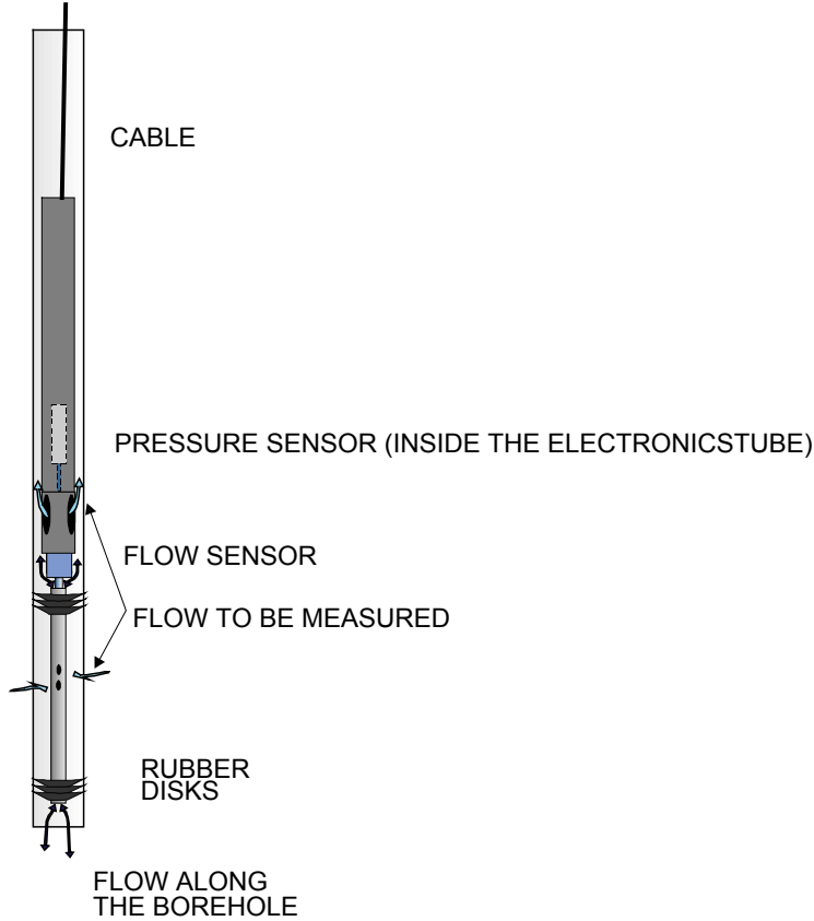
Figure 3-2. The absolute pressure sensor is located inside the electronics tube and connected through a tube to the borehole water.
