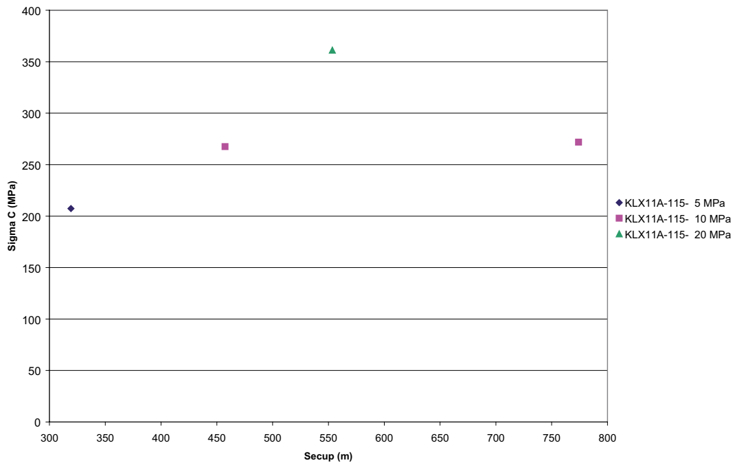
Figure 5-2. Compressive strength versus sampling level (borehole length).
