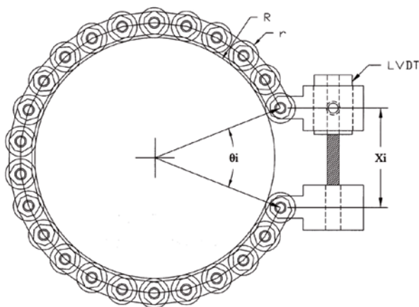
Figure A-1. Chain for radial deformation measurement.
