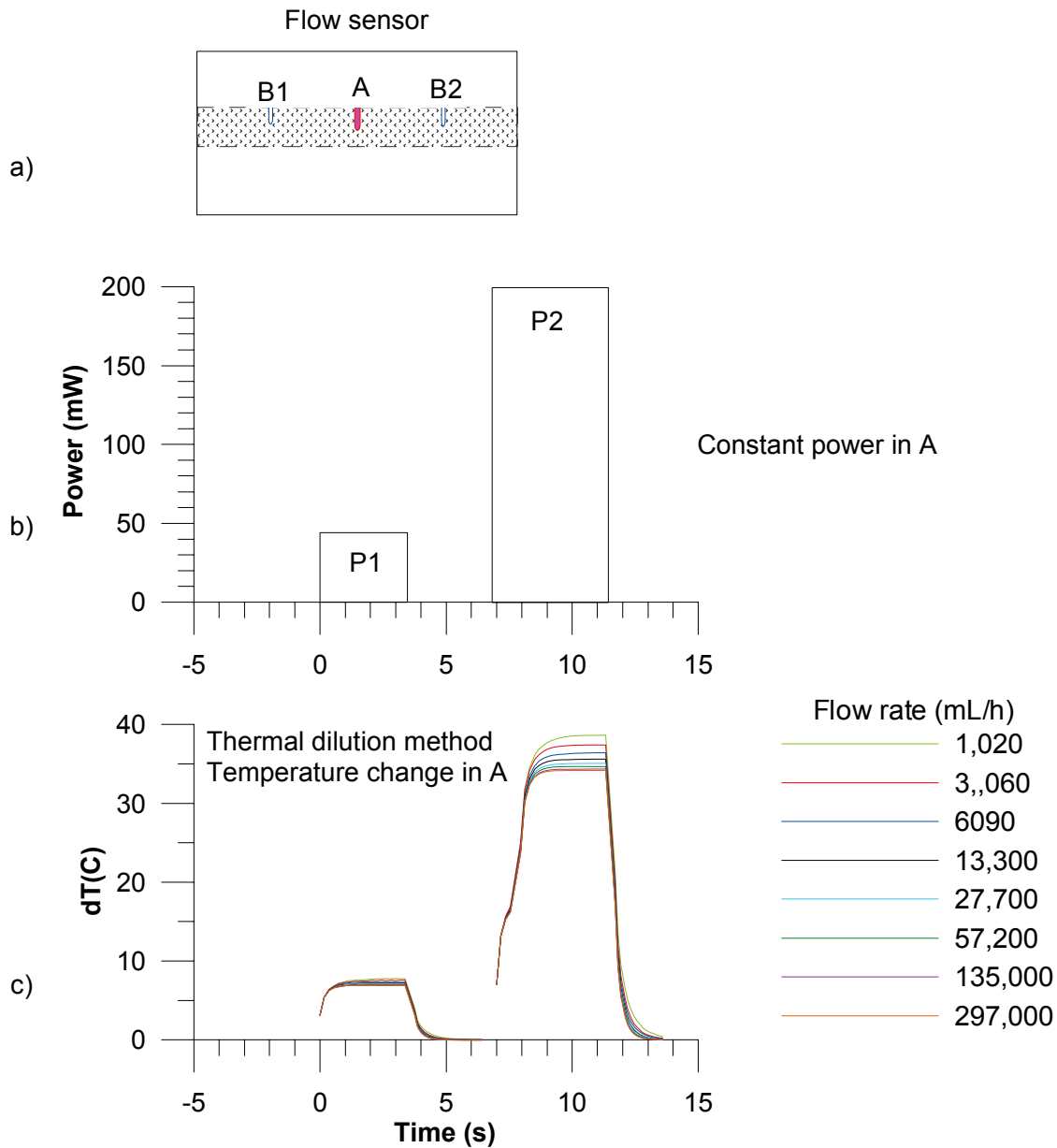
Figure 3-4. Flow measurement, flow rate > 1,200 mL/h.
