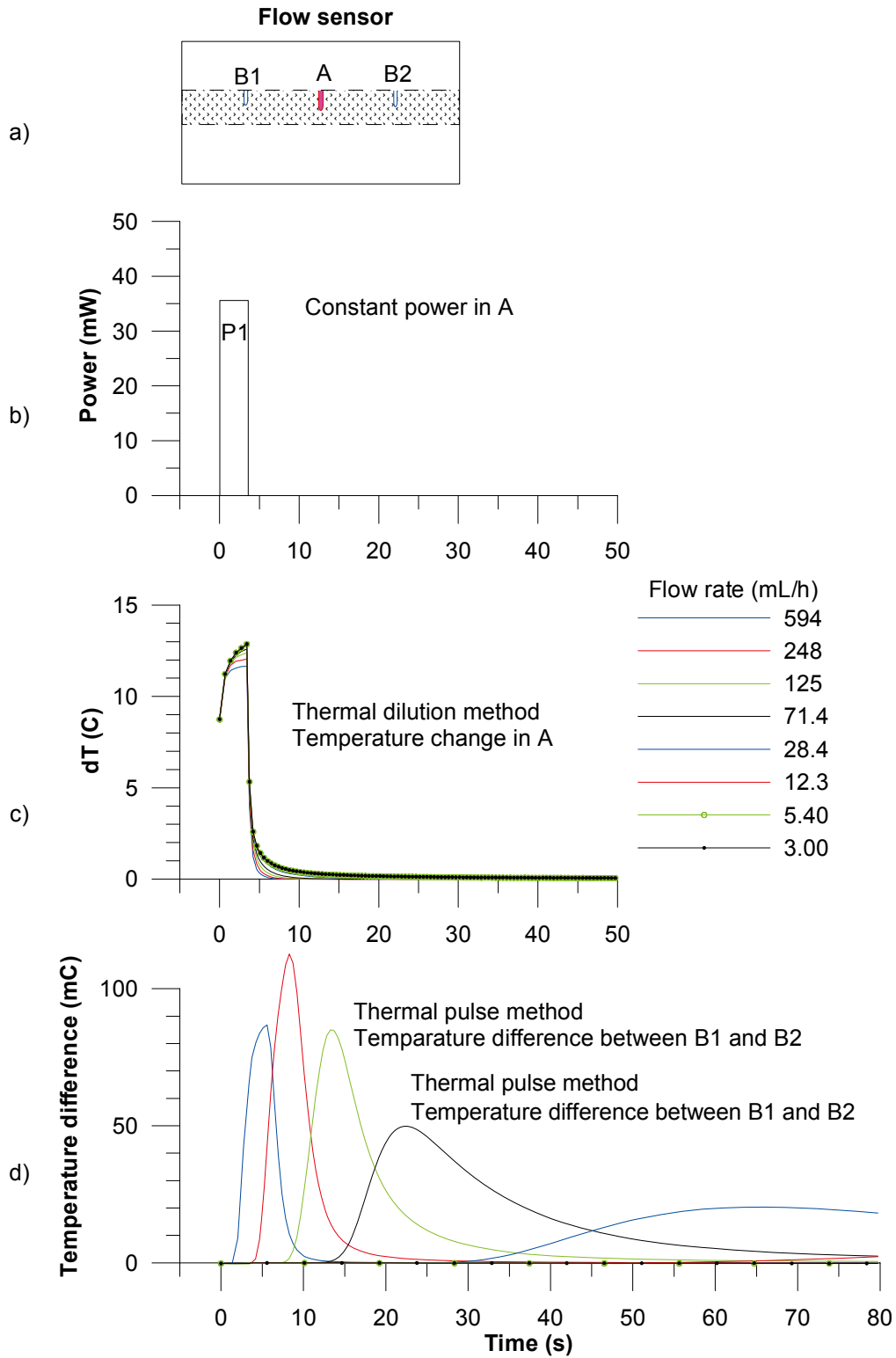
Figure 3-3. Flow measurement, flow rate < 1,200 mL/h.
