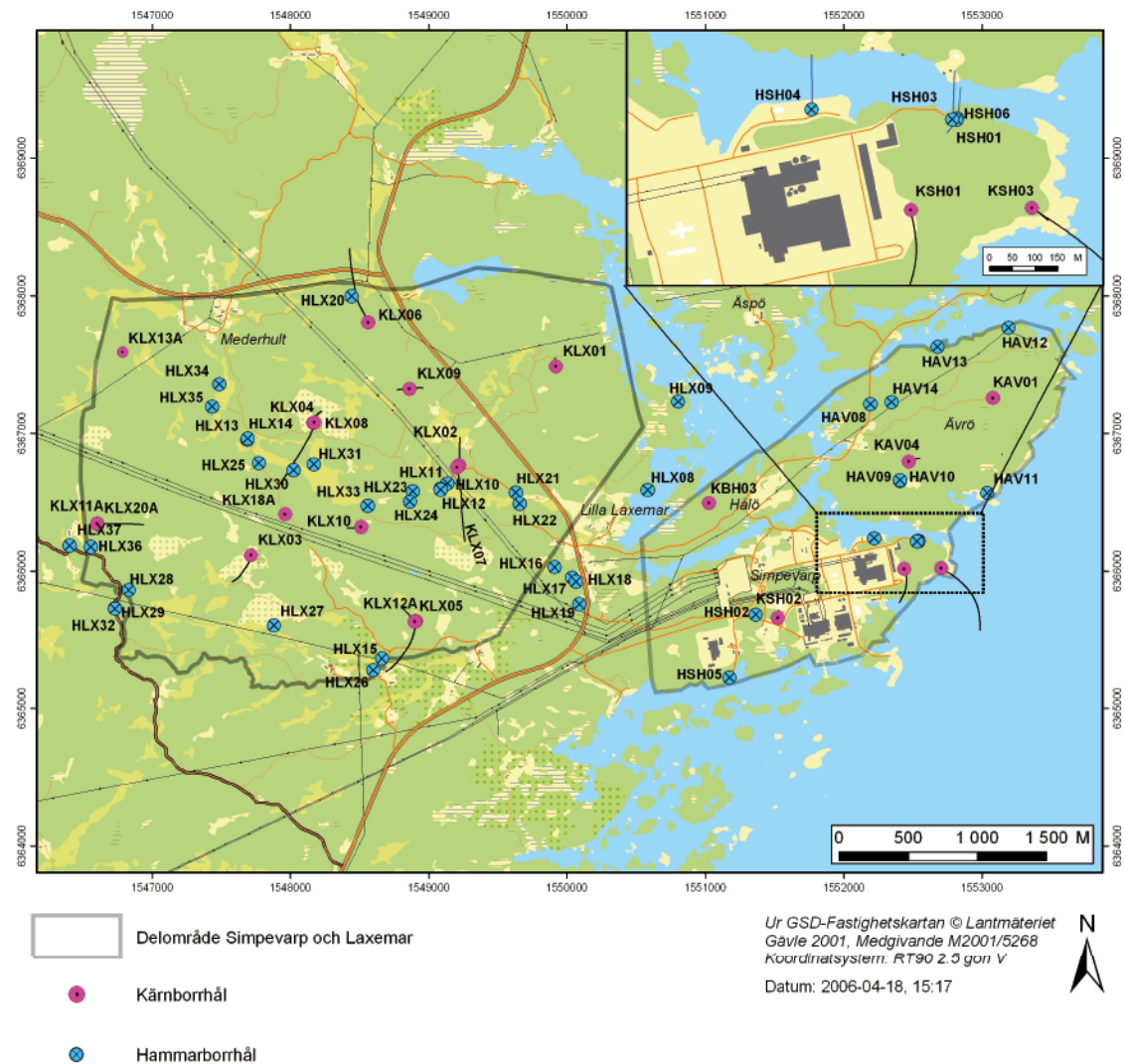
Figure 1-1. Location of all telescopic boreholes drilled up to April 2006 within or close to the Oskarshamn candidate area. The projection of each borehole on the horizontal plane at top of casing is also shown in the figure.
