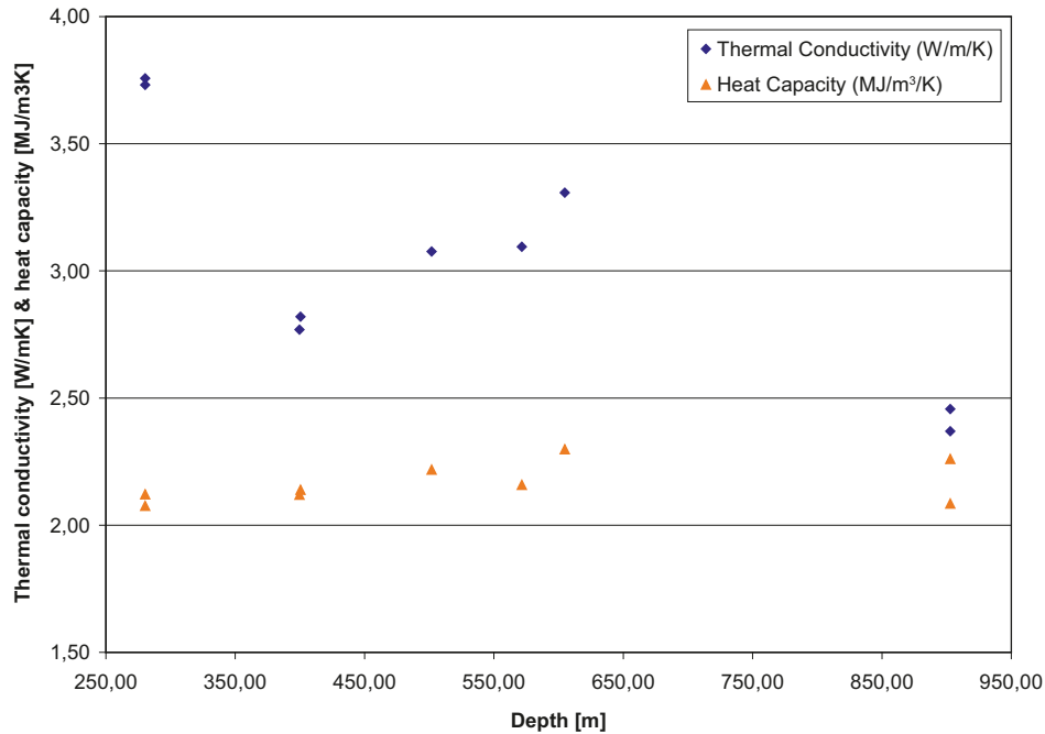
Figure 5-10. Thermal conductivity and heat capacity versus borehole length at 20°C.
