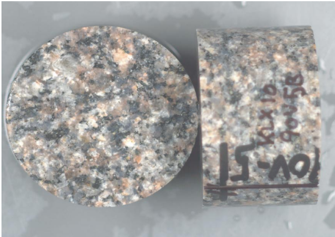
Figure 5-5. Specimens KLX10-90V-05A and B.
