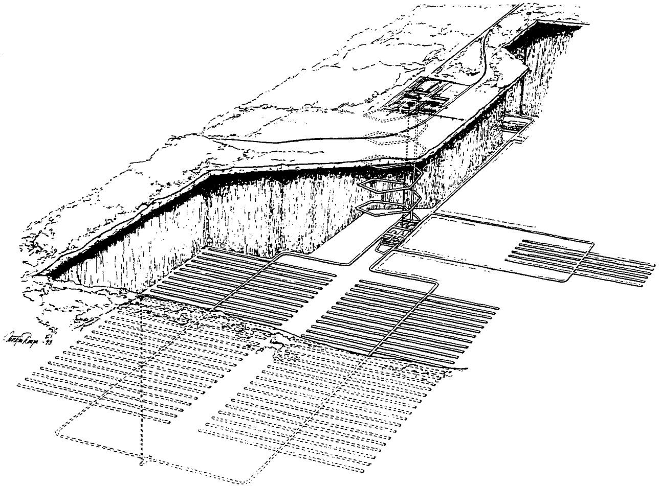
Figure 2.8 Deep repository – overview
