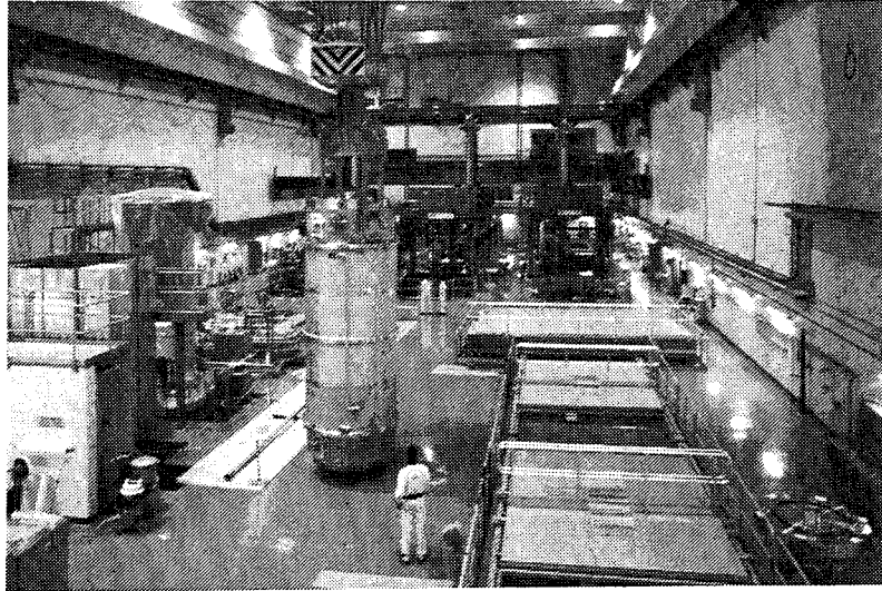
Handling of transport cask in the receiving section
