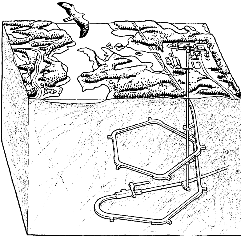
Figure 2.2 Schematic drawing of Äspö HRL
