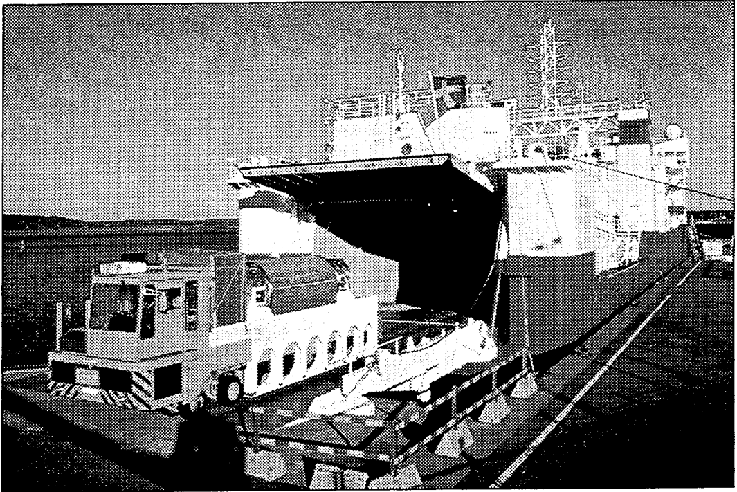
Figure 2.3 Terminal vehicle with fuel transport cask
