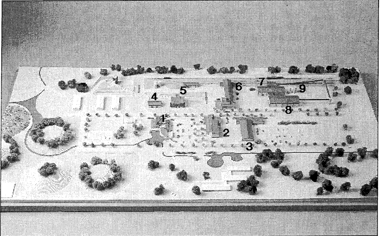
Figure 2.7. Model of the industrial area at the deep repository
