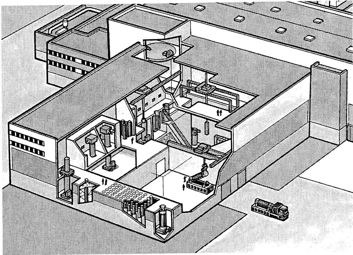
Figure 2.6 Encapsulation plant for spent fuel
