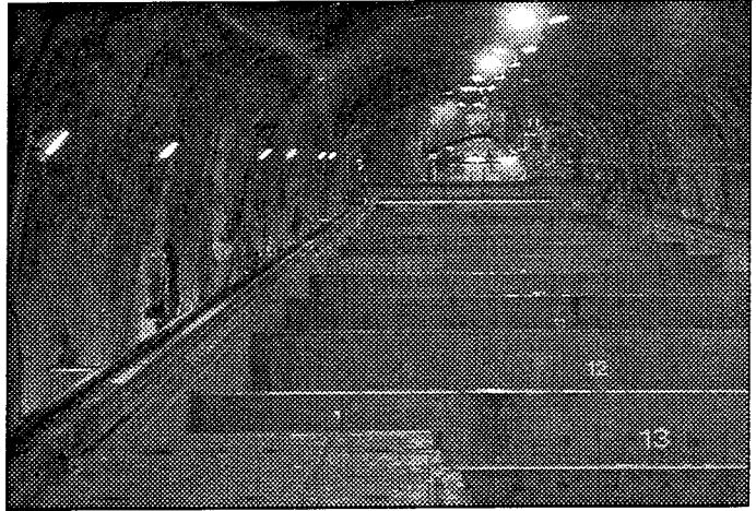
View of the rock vault for intermediate-level waste
