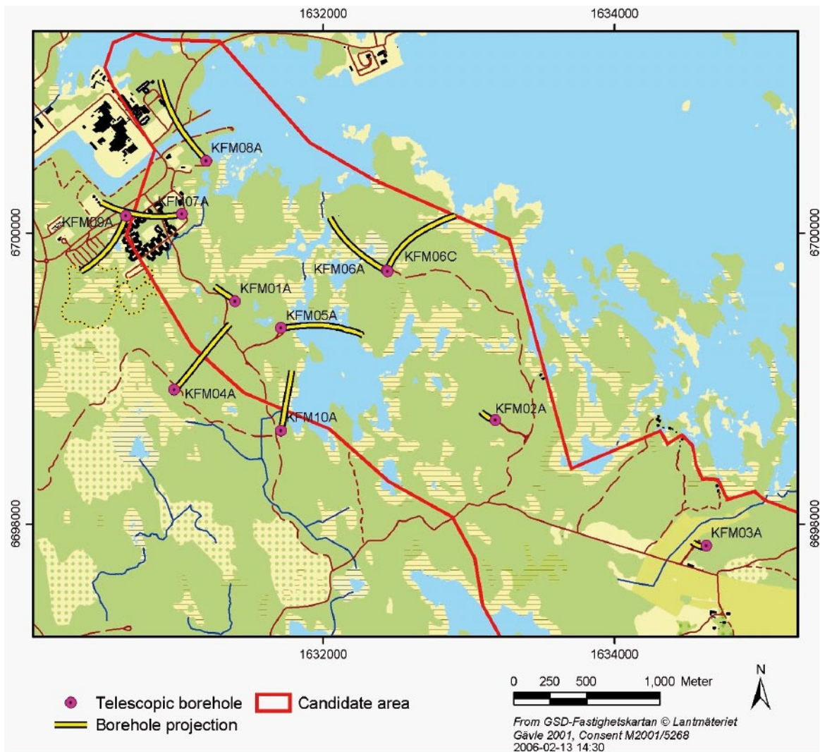
Figure 1-1. Location of all deep core drilled boreholes completed up February 2006 within or close to the Forsmark candidate area. The projection of each borehole on the horizontal plane at top of casing is also shown in the figure.
