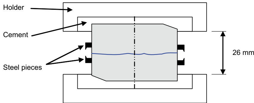
Figure 4-2. Specimen cast with cement in the specimen holder for the normal loading tests.
