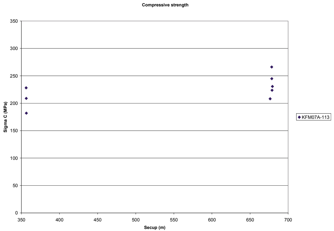
Figure 5-2. Uniaxial compressive strength versus sampling level (borehole length).
