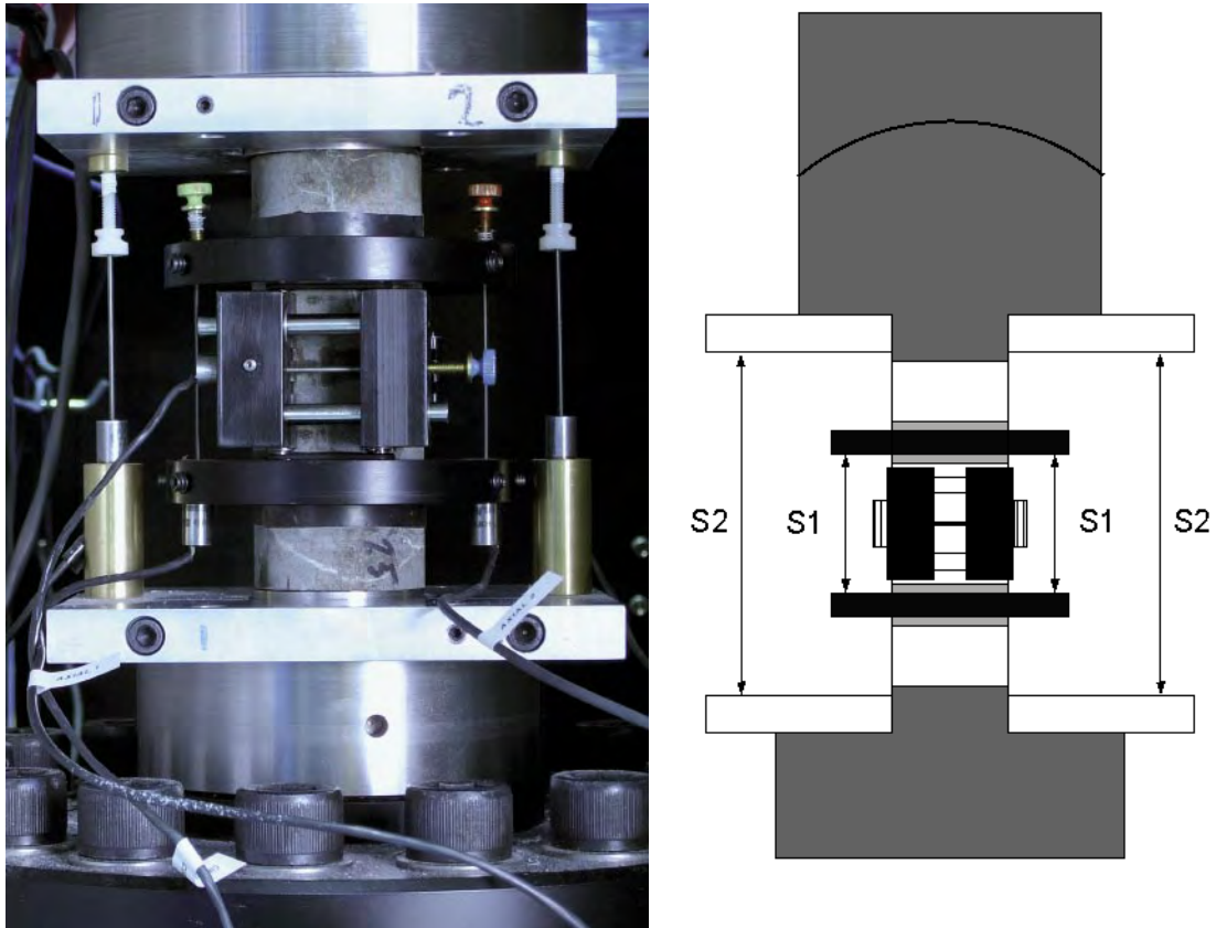
Figure 3-3. Left: Specimen inserted between the loading platens. The two separate axial deformation measurement devices can be seen: system (S1) that measures the local axial deformation (rings), and system (S2) that measures the deformation between the aluminium plates (total deformation). Right: Principal sketch showing the two systems used for the axial deformation measurements.
