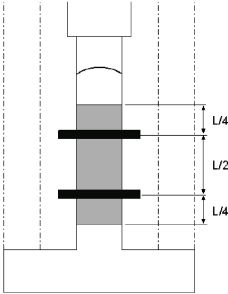
Figure 4-1. Sketch showing the triaxial cell with the rock specimen (grey) with height L and the position of the rings (black) used for the axial deformation measurements. The membrane is omitted in the figure for simplicity.
