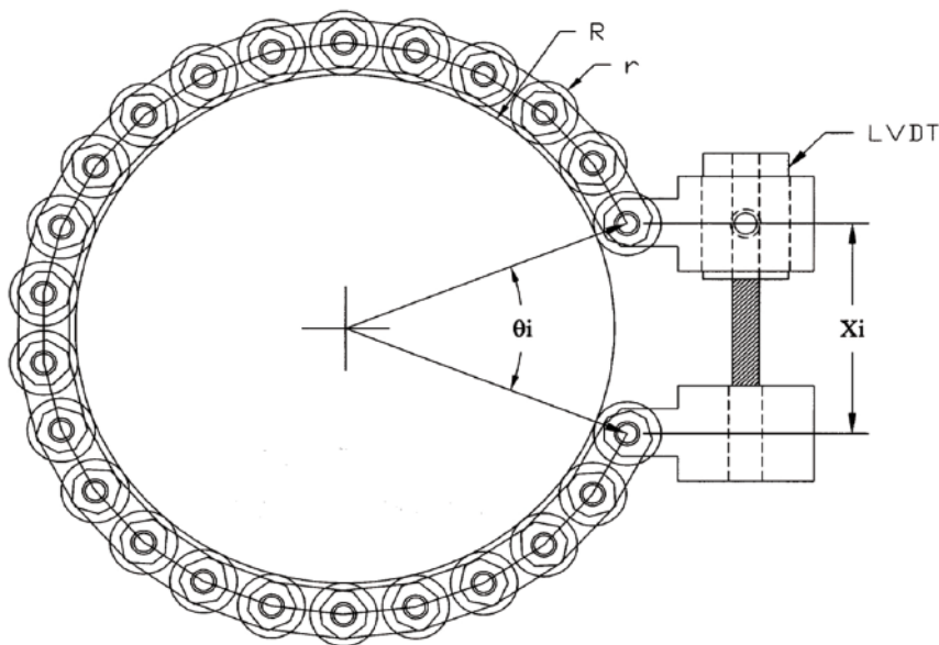
Figure A-1. Chain for radial deformation measurement.
