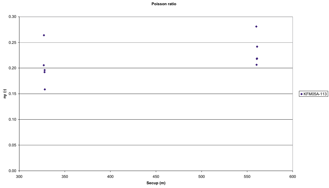
Figure 5-4. Tangent Poisson ratio versus borehole length (KFM05A is inclined c 60^\circ from the horizon).
