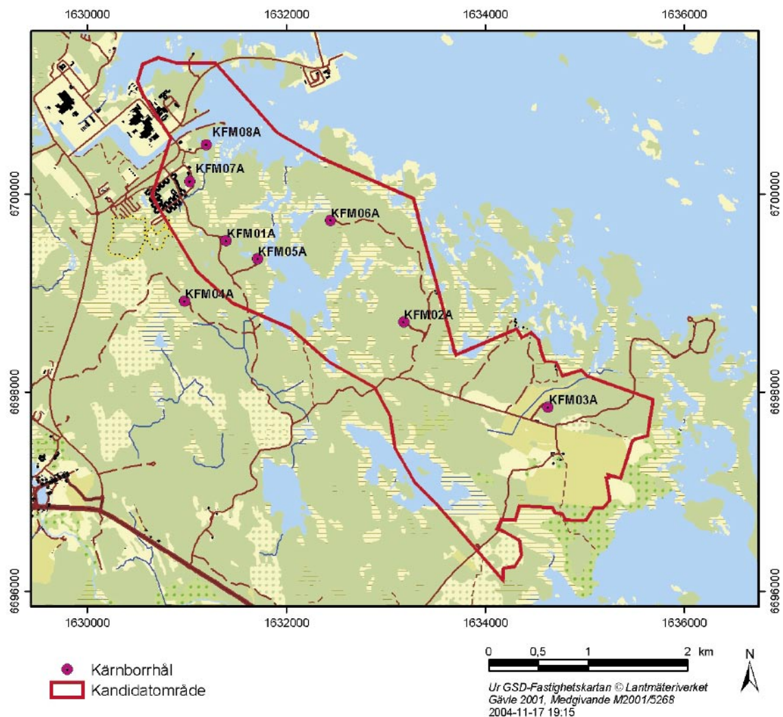
Figure 1-1. Location of borehole KFM05A at the Forsmark site.
