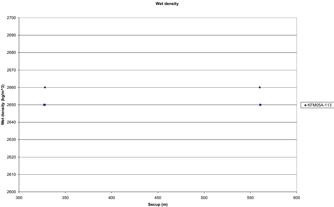
Figure 5-1. Density versus borehole length (KFM05A is inclined c 60° from the horizon).
