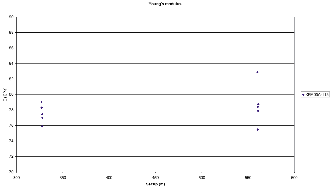
Figure 5-2. Uniaxial compressive strength versus borehole length (KFM05A is inclined c 60° from the horizon).
