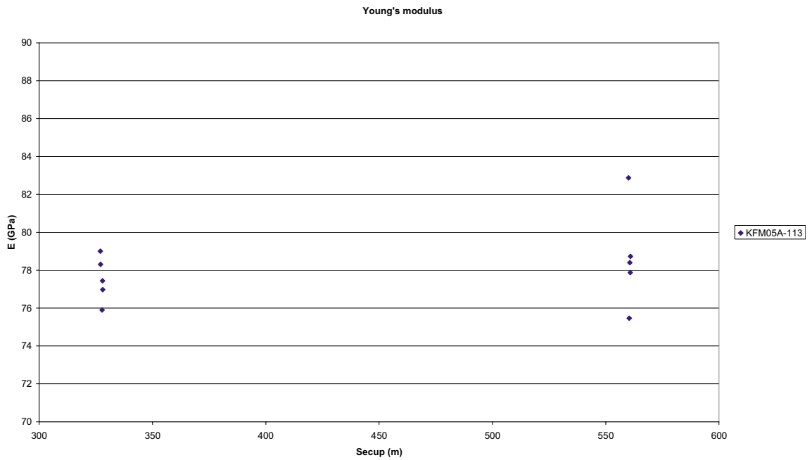
Figure 5-3. Tangent Young's modulus versus borehole length (KFM05A is inclined c 60° from the horizon).
