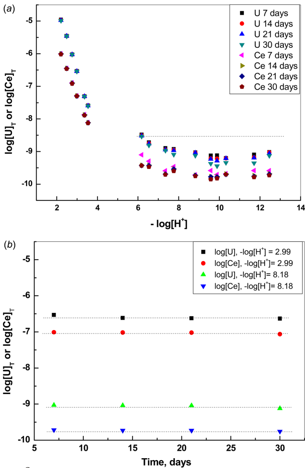
Figure 2 (a) Evolution of U and Ce total concentrations during 30 days equilibration for all pH values investigated for the solid with 1% Ce. (b) Evolution of U and Ce concentrations during 30 days equilibration for two randomly selected samples at -\log[\text{H}^+] values of 2.99 and 8.18. The dotted lines are horizontal and centered at the value of the last point.
