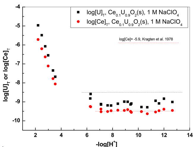
Figure 16 Concentrations of Ce and U in equilibrium with Ce_{0.10}U_{0.90} oxide coprecipitate. The dotted lines in the basic range indicate the solubility of UO_2(s) , \log [U] = -8.5 , and the horizontal part of Ce concentrations for the pure oxide and the coprecipitate.
