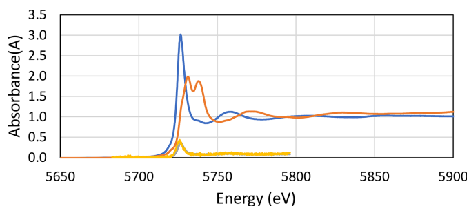
Figure 10 Normalized raw XANES spectra of cerium (III) oxide, \text{Ce}_2\text{O}_3 (light blue line) and cerium (IV) oxide, \text{CeO}_2 (brown line). Raw data, not normalized, of \text{U}_{0.90}\text{Ce}_{0.10} at two different spots (yellow and gray lines) show that cerium is present as cerium (III) in the studied samples.
