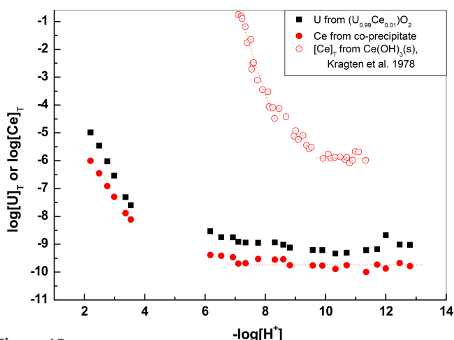
Figure 15 Concentrations of Ce and U in equilibrium with Ce_{0.01}U_{0.99} oxide coprecipitate compared with concentrations of Ce in equilibrium with Ce(OH)_3(s) (Kragten & Decnop-Weever, 1978) at 1 M NaClO_4 .
