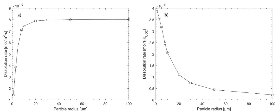
Fig. 15. –Area-specific (a) and weight specific (b) UO 2 dissolution rates modelling the Tribet fuel with UO 2 particles of radius 1–100 μm.
